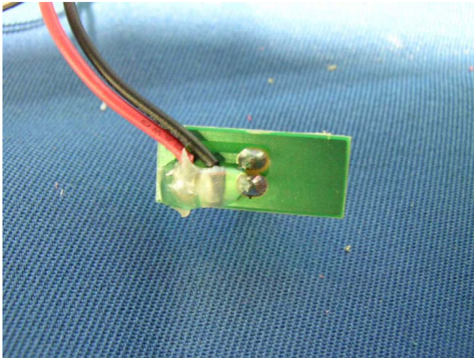
Handset rechargeable battery terminal PCB rear side
