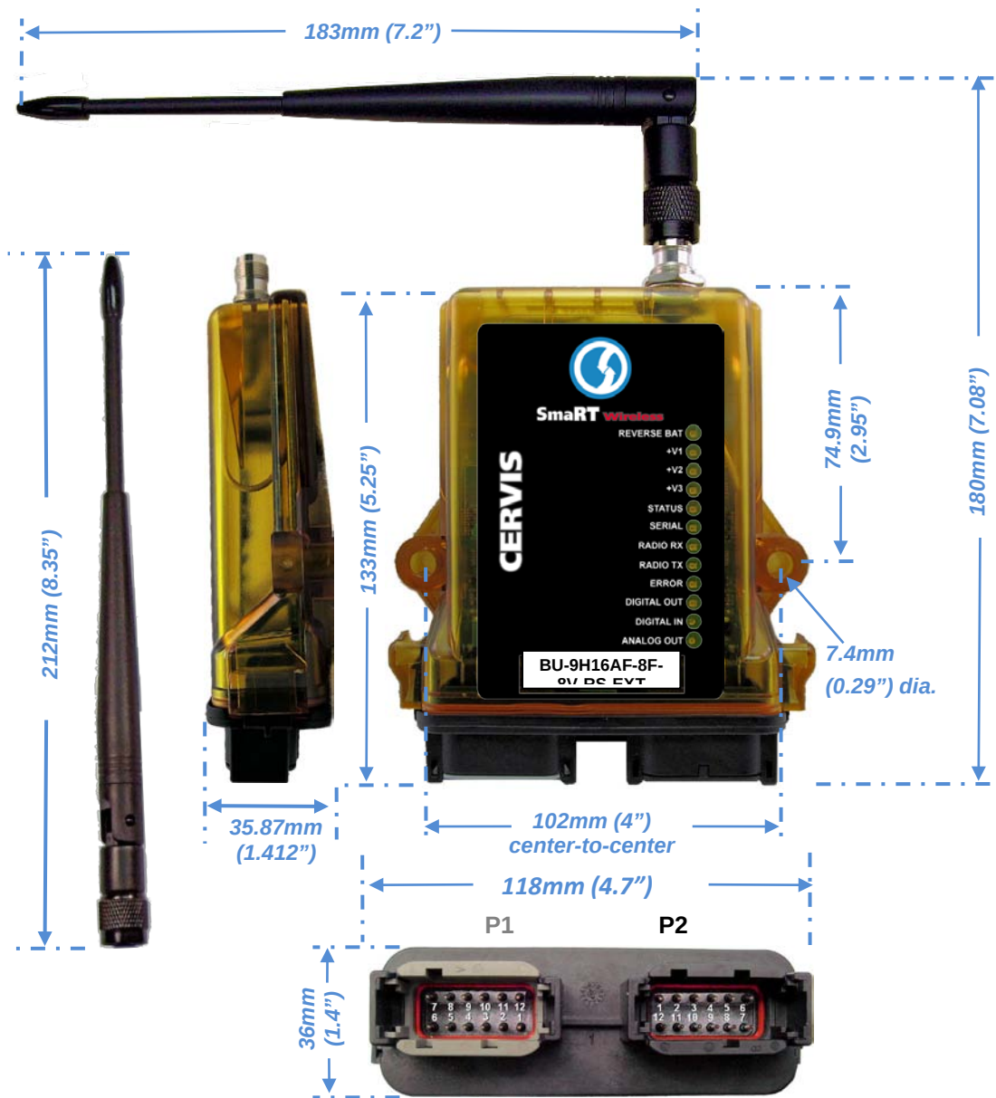
Figure 4. SmaRT BU-9H16AF-8F-8V-RS-EXT Mounting Dimensions
