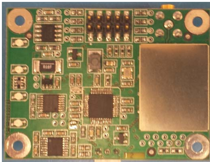
LOBMRF450, Component Side, RF Shield Installed
