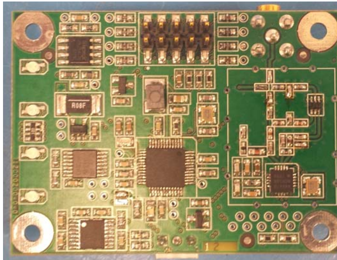
LOBMRF450, Component Side, RF Shield Removed
