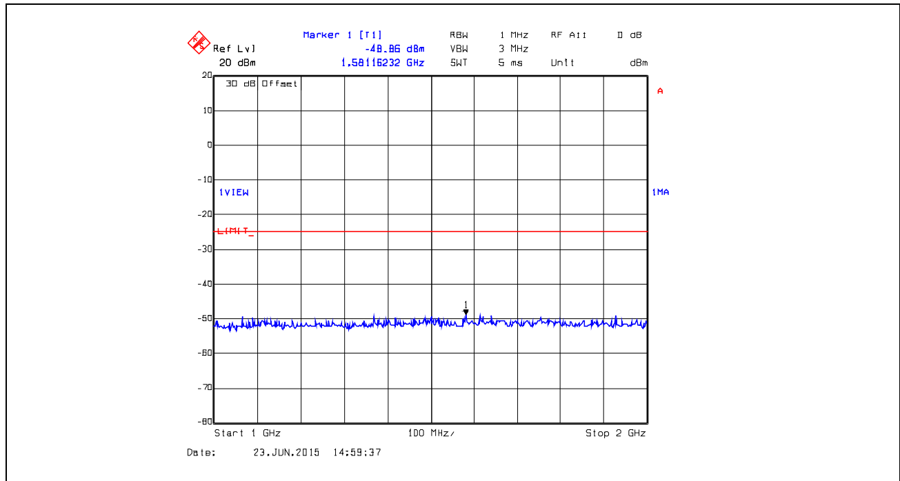
Plot 5.5.4.21. Conducted Transmitter Spurious Emissions, 173.9 MHz, High Power, 1 GHz – 2 GHz
