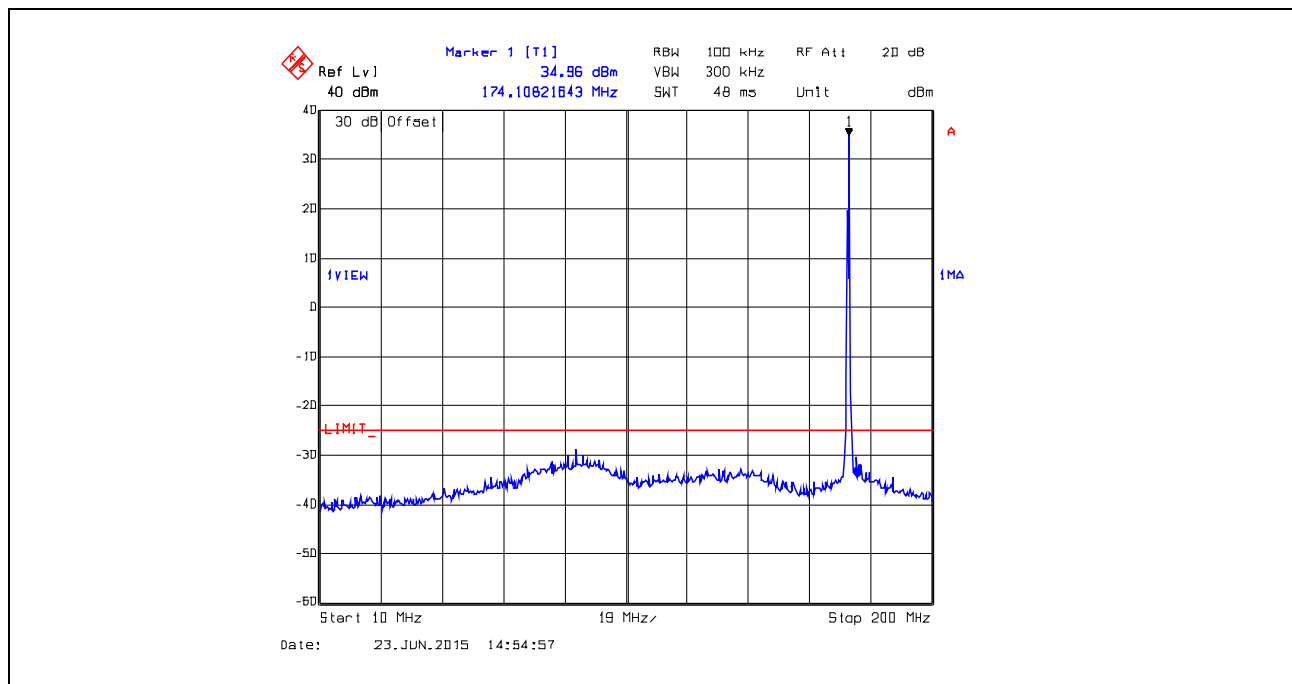
Plot 5.5.4.19. Conducted Transmitter Spurious Emissions, 173.9 MHz, High Power, 10 MHz – 200 MHz
