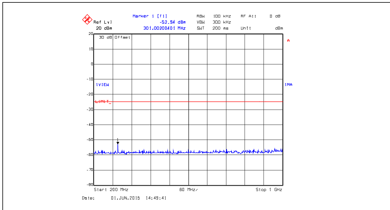
Plot 5.5.4.8. Conducted Transmitter Spurious Emissions, 151.1 MHz, High Power, 200 MHz – 1 GHz
