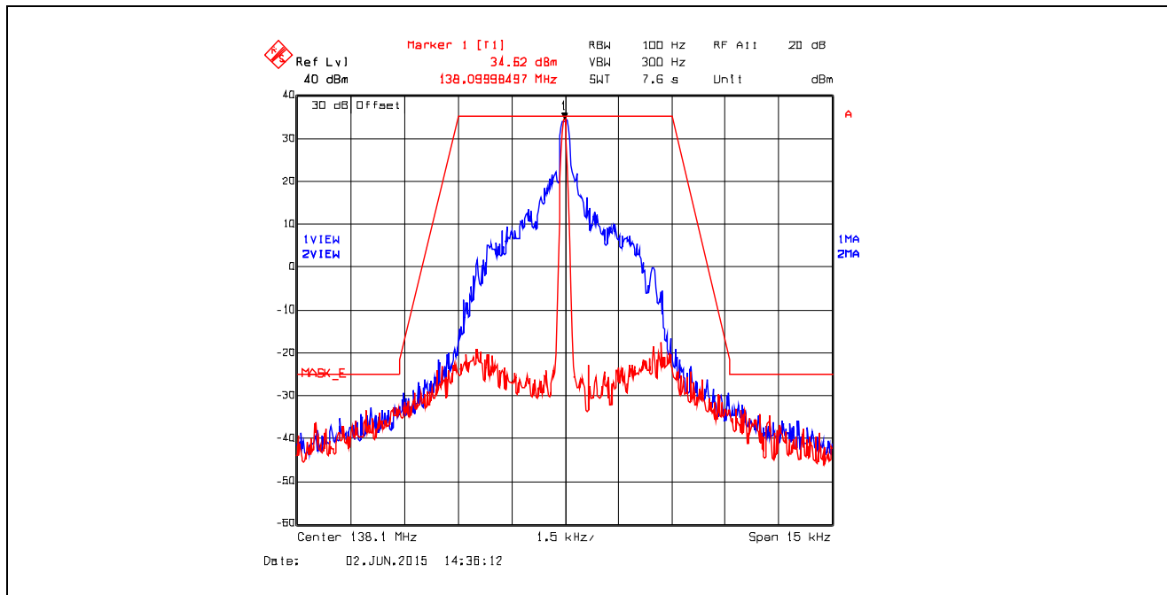
Plot 5.4.4.6.1. Emission Mask E, Digital at 4.8 kbps, 138.1 MHz, High Power
