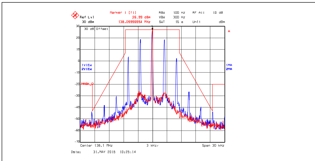
Plot 5.4.4.4.2. Emission Mask D, Analog, 138.1 MHz, Low Power
