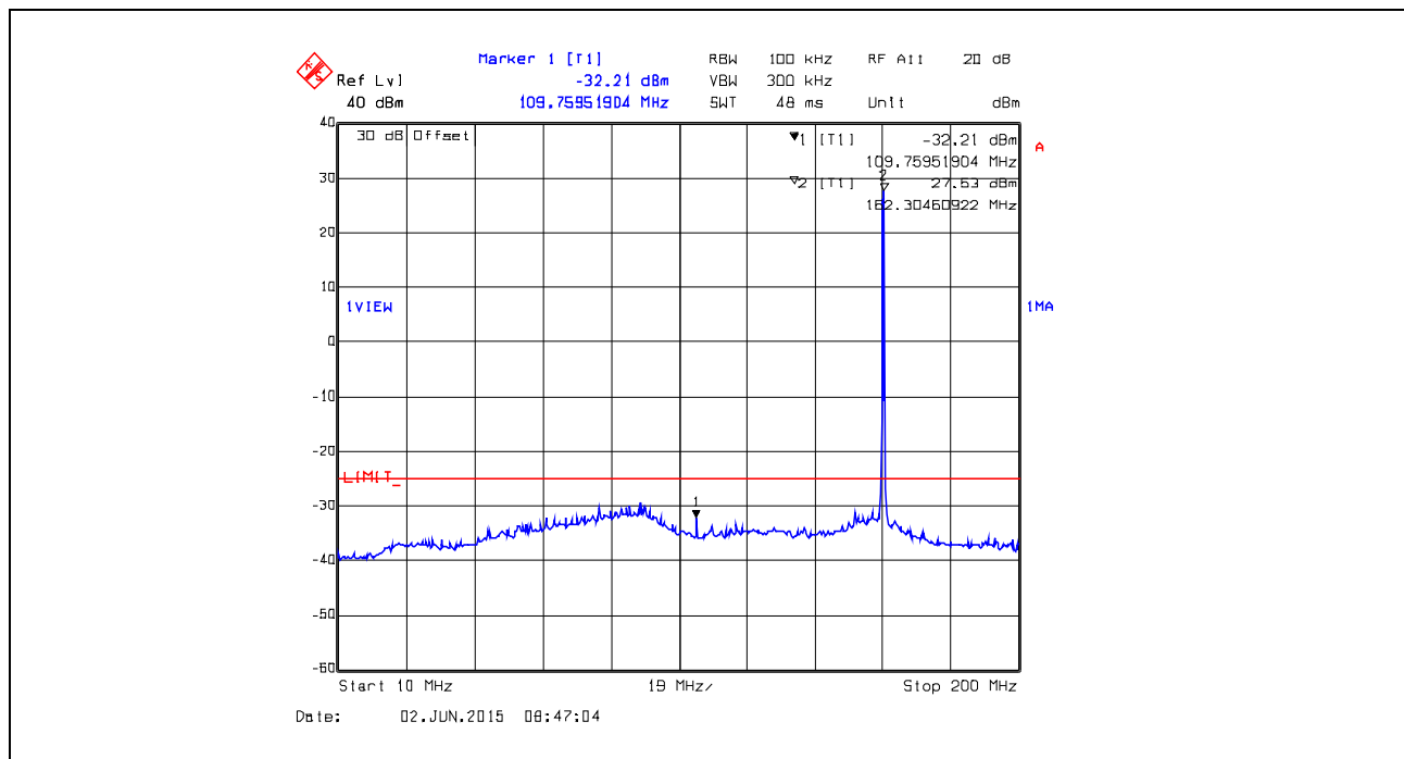
Plot 5.5.4.16. Conducted Transmitter Spurious Emissions, 162.0 MHz, Low Power, 10 MHz – 200 MHz
