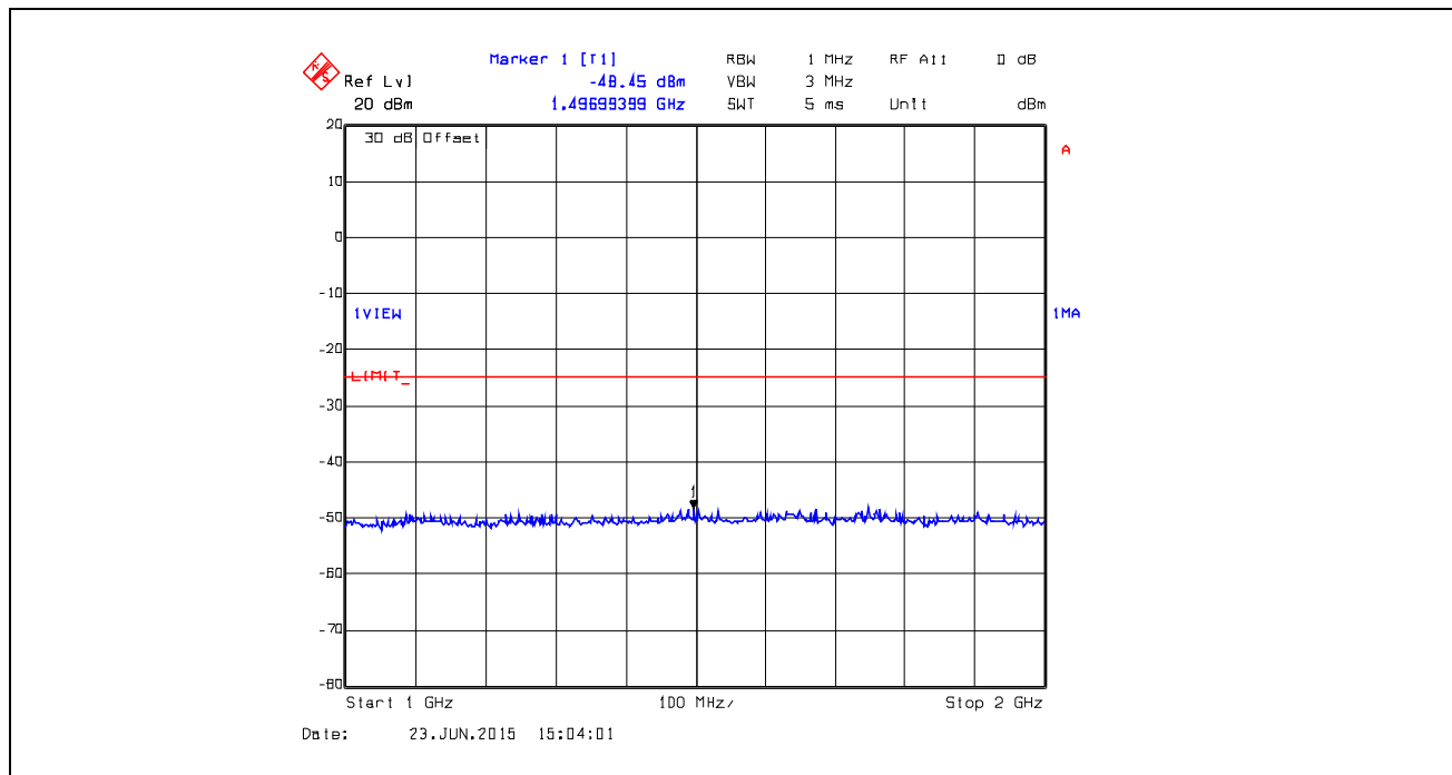
Plot 5.5.4.6. Conducted Transmitter Spurious Emissions, 138.1 MHz, Low Power, 1 GHz – 2 GHz
