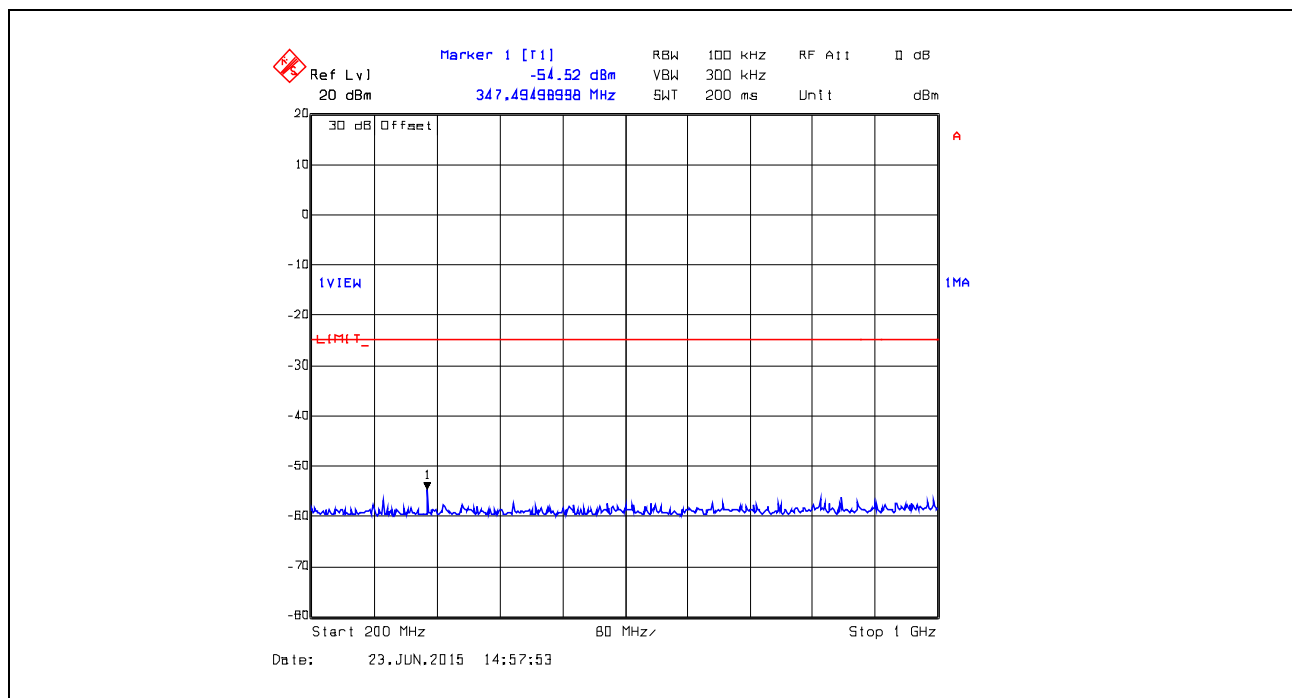
Plot 5.5.4.20. Conducted Transmitter Spurious Emissions, 173.9 MHz, High Power, 200 MHz – 1 GHz
