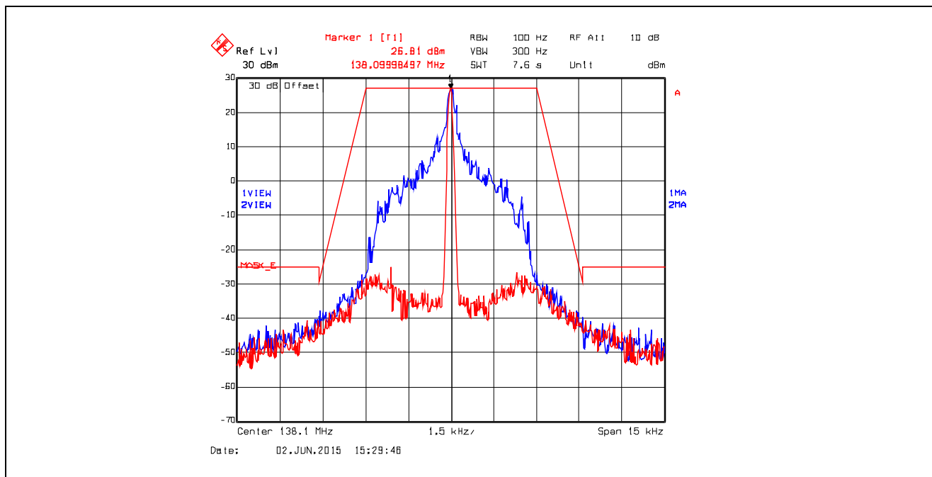
Plot 5.4.4.6.2. Emission Mask E, Digital at 4.8 kbps, 138.1 MHz, Low Power
