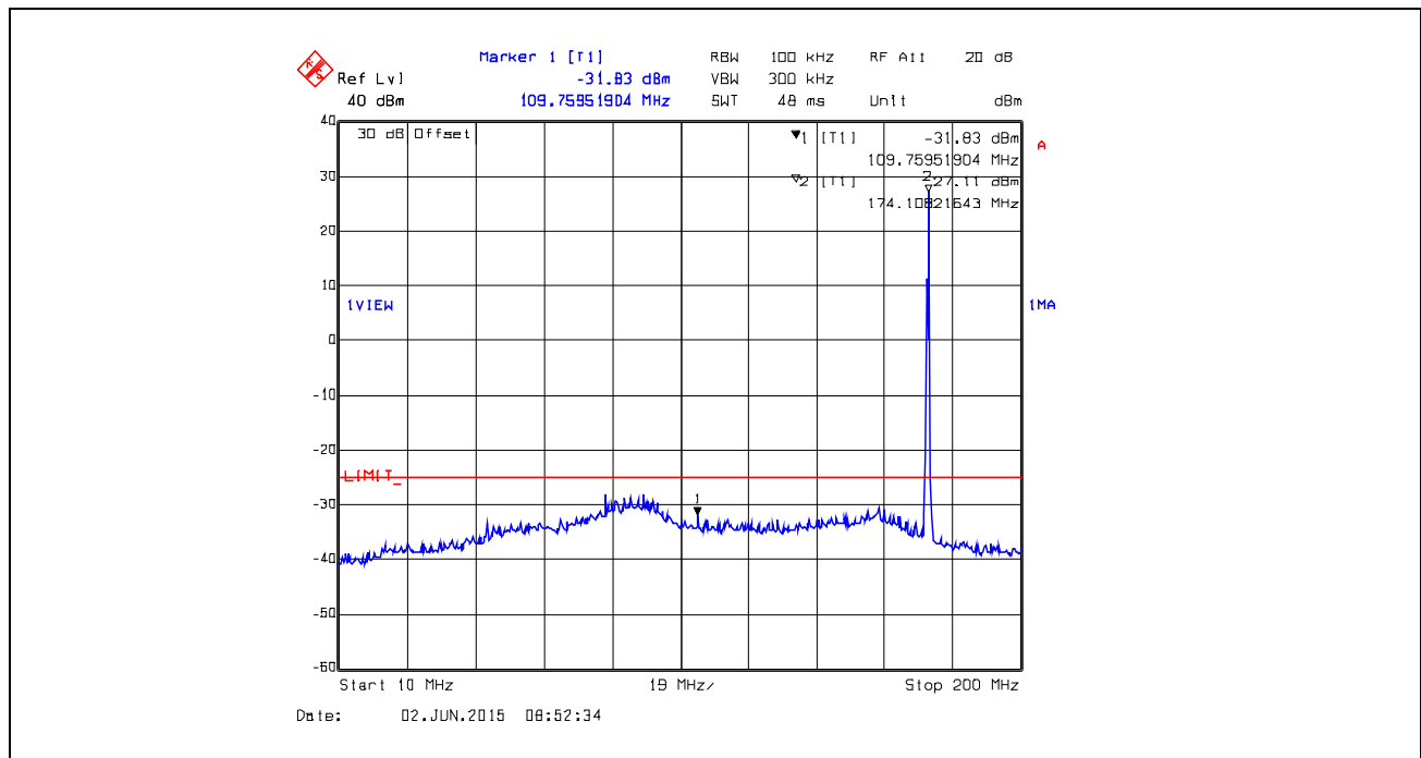
Plot 5.5.4.22. Conducted Transmitter Spurious Emissions, 173.9 MHz, Low Power, 10 MHz – 200 MHz
