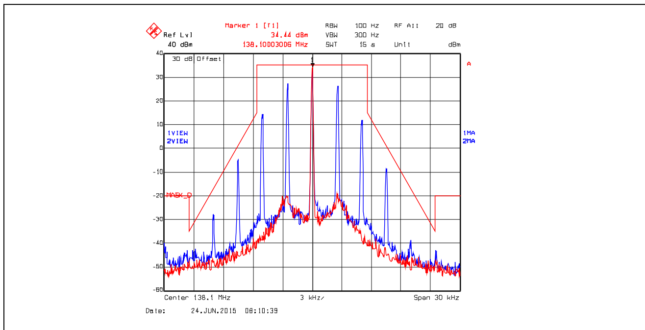
Plot 5.4.4.4.1. Emission Mask D, Analog, 138.1 MHz, High Power
