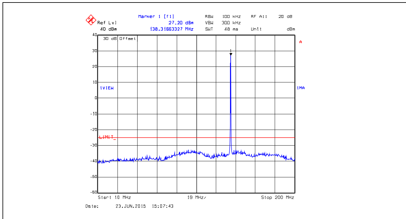
Plot 5.5.4.4. Conducted Transmitter Spurious Emissions, 138.1 MHz, Low Power, 10 MHz – 200 MHz
