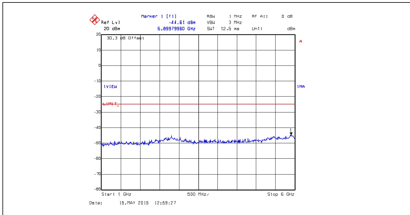
Plot 5.5.4.12. Conducted Transmitter Spurious Emissions, 390.0 MHz, Low Power, 1 GHz – 6 GHz
