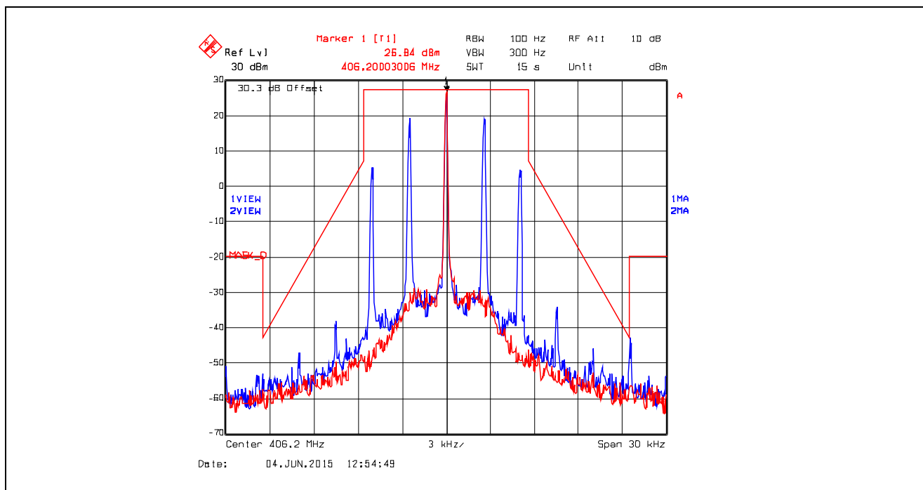
Plot 5.4.4.4.8. Emission Mask D, Analog, 406.2 MHz, Low Power
