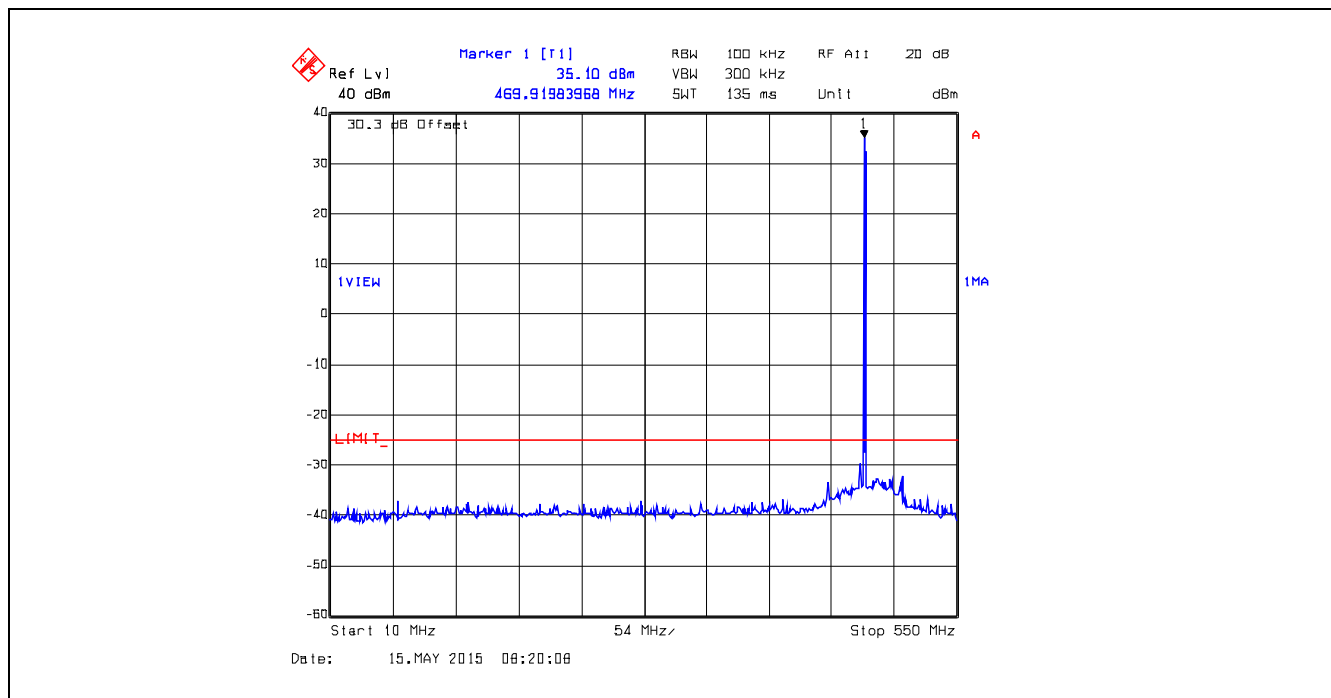
Plot 5.5.4.43. Conducted Transmitter Spurious Emissions, 470.0 MHz, High Power, 10 MHz – 550 MHz
