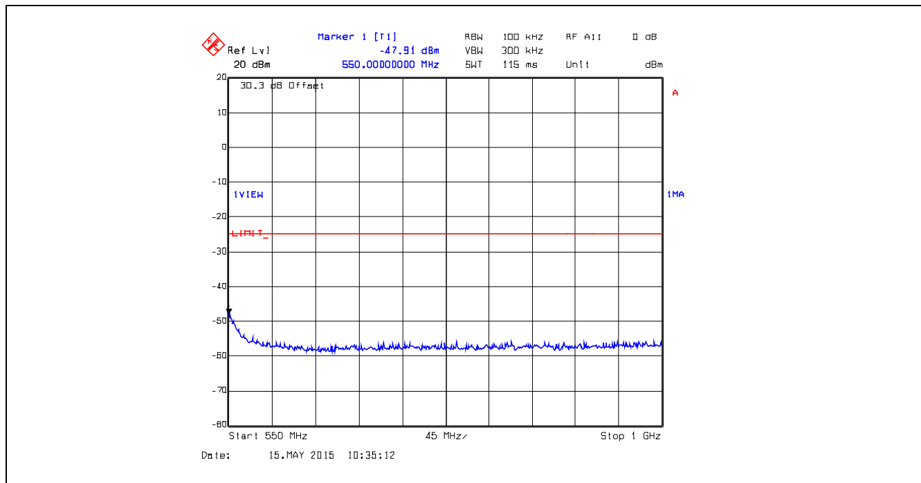
Plot 5.5.4.50. Conducted Transmitter Spurious Emissions, 511.9 MHz, High Power, 550 MHz – 1 GHz
