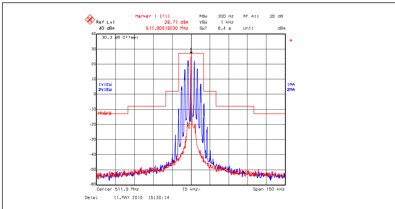
Plot 5.4.4.2.18. Emission Mask B, Analog, 511.9 MHz, Low Power
