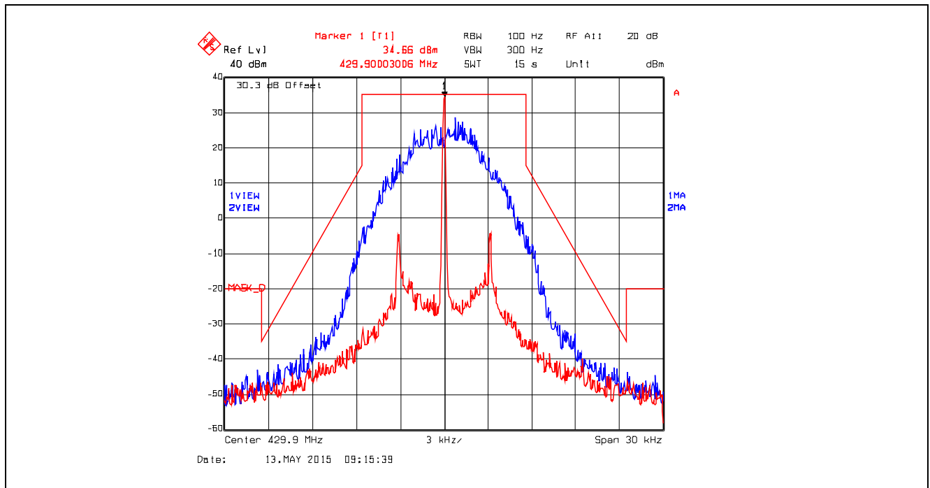
Plot 5.4.4.5.11. Emission Mask D, Digital at 9.6 kbps, 429.9 MHz, High Power
