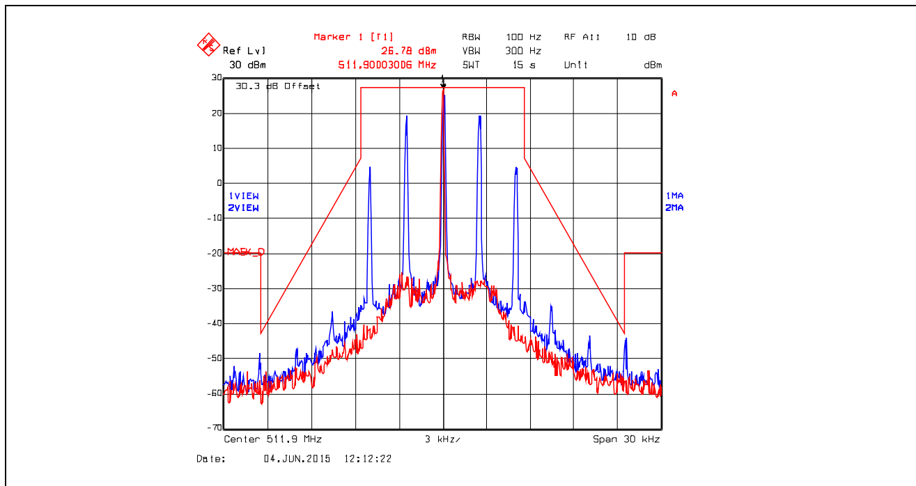
Plot 5.4.4.4.18. Emission Mask D, Analog, 511.9 MHz, Low Power
