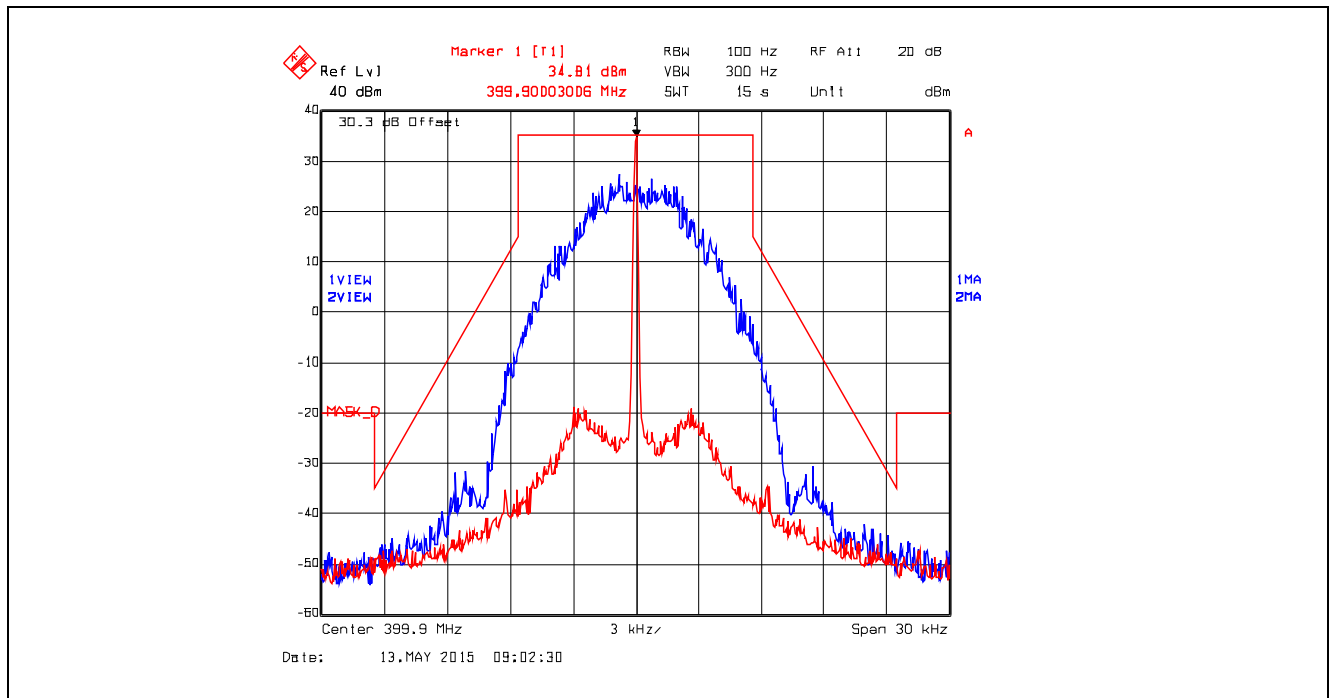
Plot 5.4.4.5.5. Emission Mask D, Digital at 9.6 kbps, 399.9 MHz, High Power
