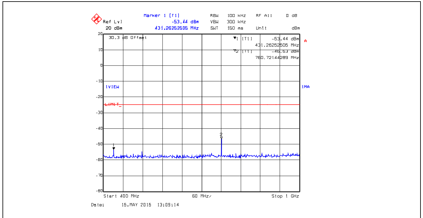
Plot 5.5.4.5. Conducted Transmitter Spurious Emissions, 380.1 MHz, Low Power, 400 MHz – 1 GHz
