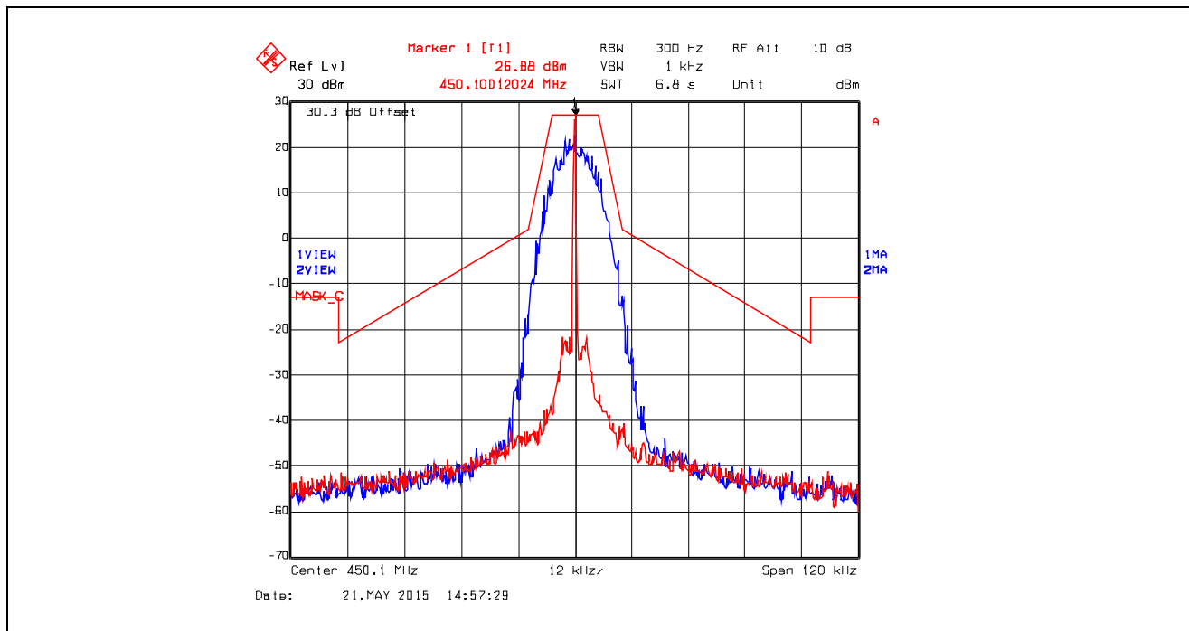
Plot 5.4.4.3.14. Emission Mask C, Digital at 19.2 kbps, 450.1 MHz, Low Power
