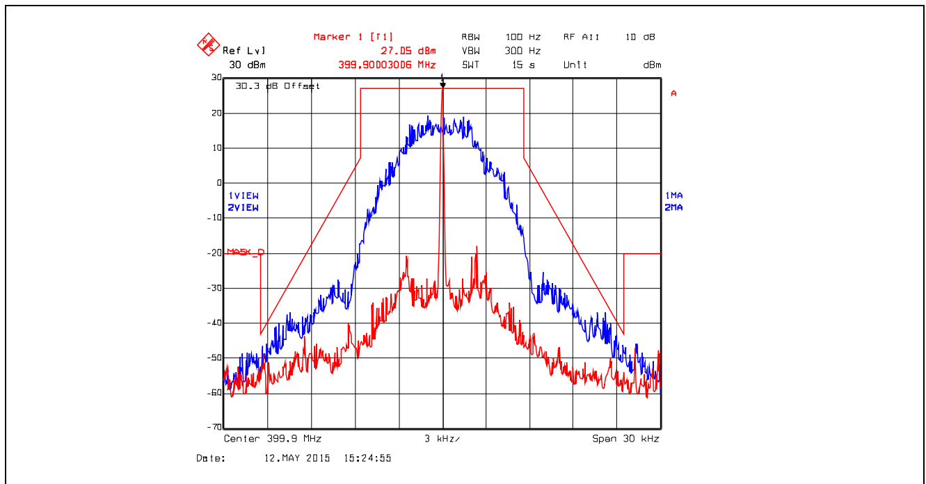
Plot 5.4.4.5.6. Emission Mask D, Digital at 9.6 kbps, 399.9 MHz, Low Power
