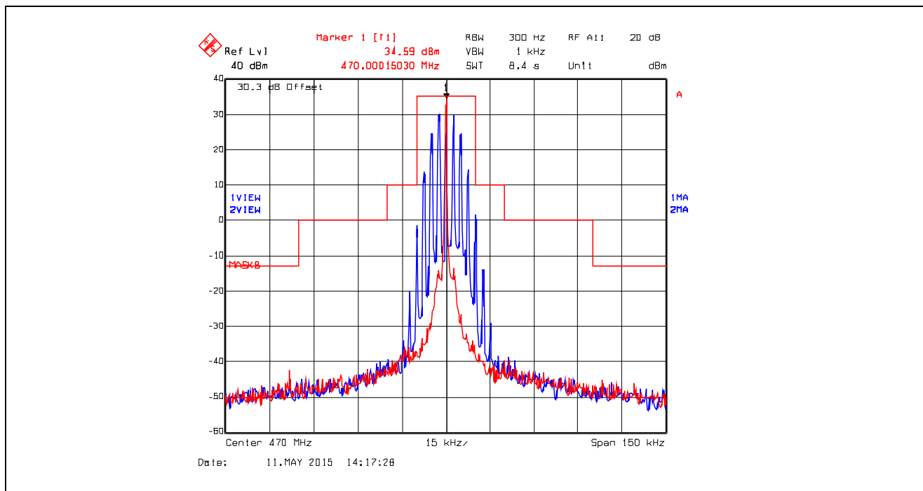
Plot 5.4.4.2.15. Emission Mask B, Analog, 470.0 MHz, High Power
