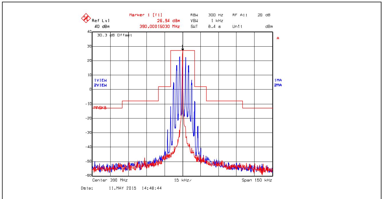
Plot 5.4.4.2.4. Emission Mask B, Analog, 390.0 MHz, Low Power
