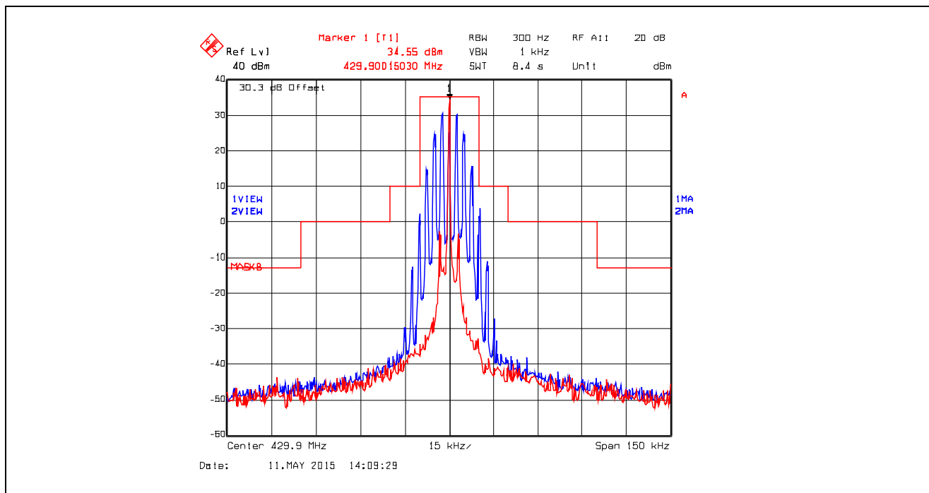
Plot 5.4.4.2.11. Emission Mask B, Analog, 429.9 MHz, High Power
