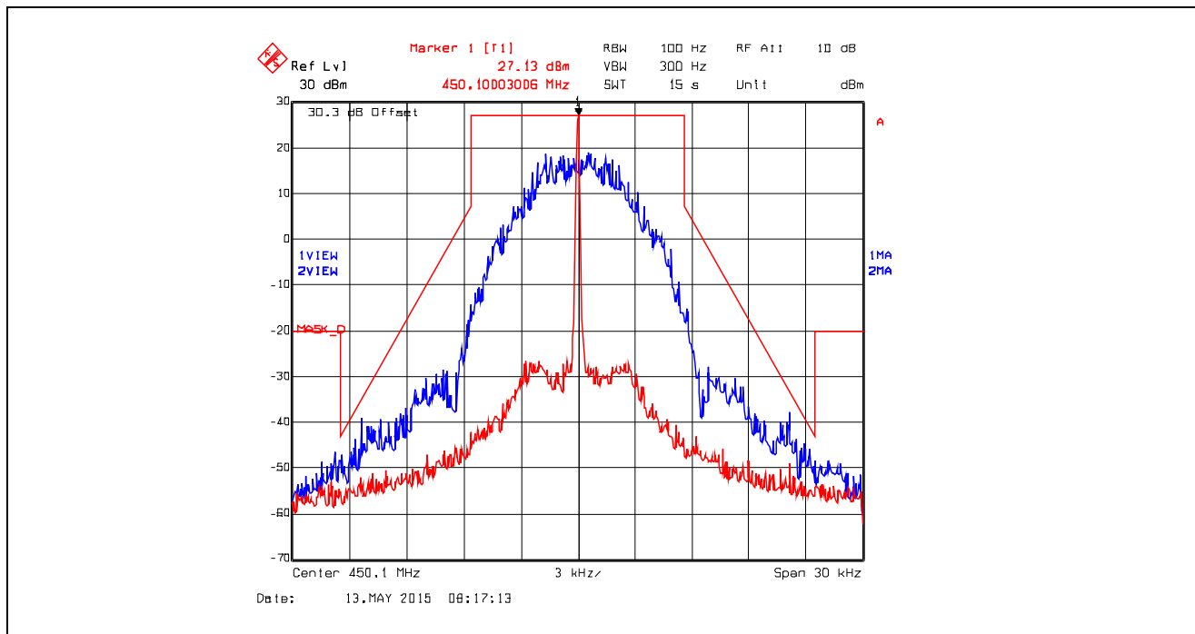
Plot 5.4.4.5.14. Emission Mask D, Digital at 9.6 kbps, 450.1 MHz, Low Power
