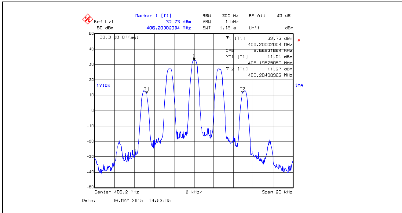
Plot 5.4.4.1.22. 99% Occupied Bandwidth, 12.5 kHz Channel Spacing, Analog, 406.2 MHz
