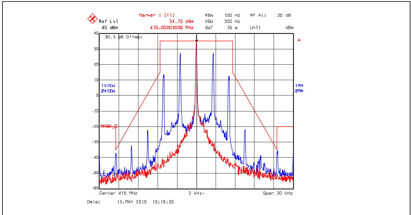
Plot 5.4.4.4.9. Emission Mask D, Analog, 415.0 MHz, High Power
