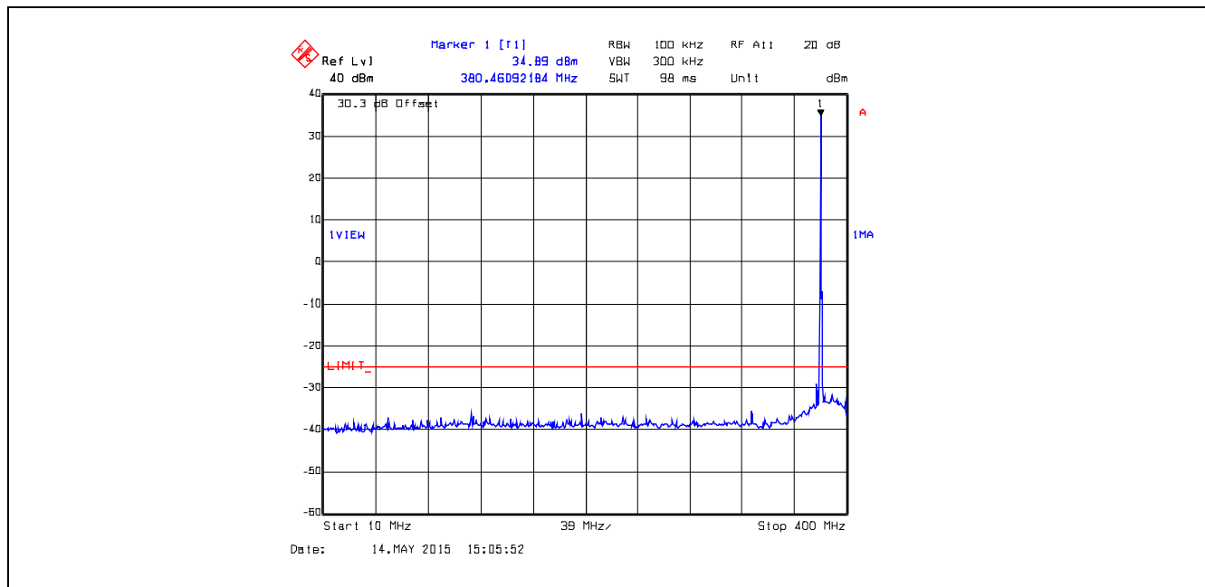
Plot 5.5.4.1. Conducted Transmitter Spurious Emissions, 380.1 MHz, High Power, 10 MHz – 400 MHz
