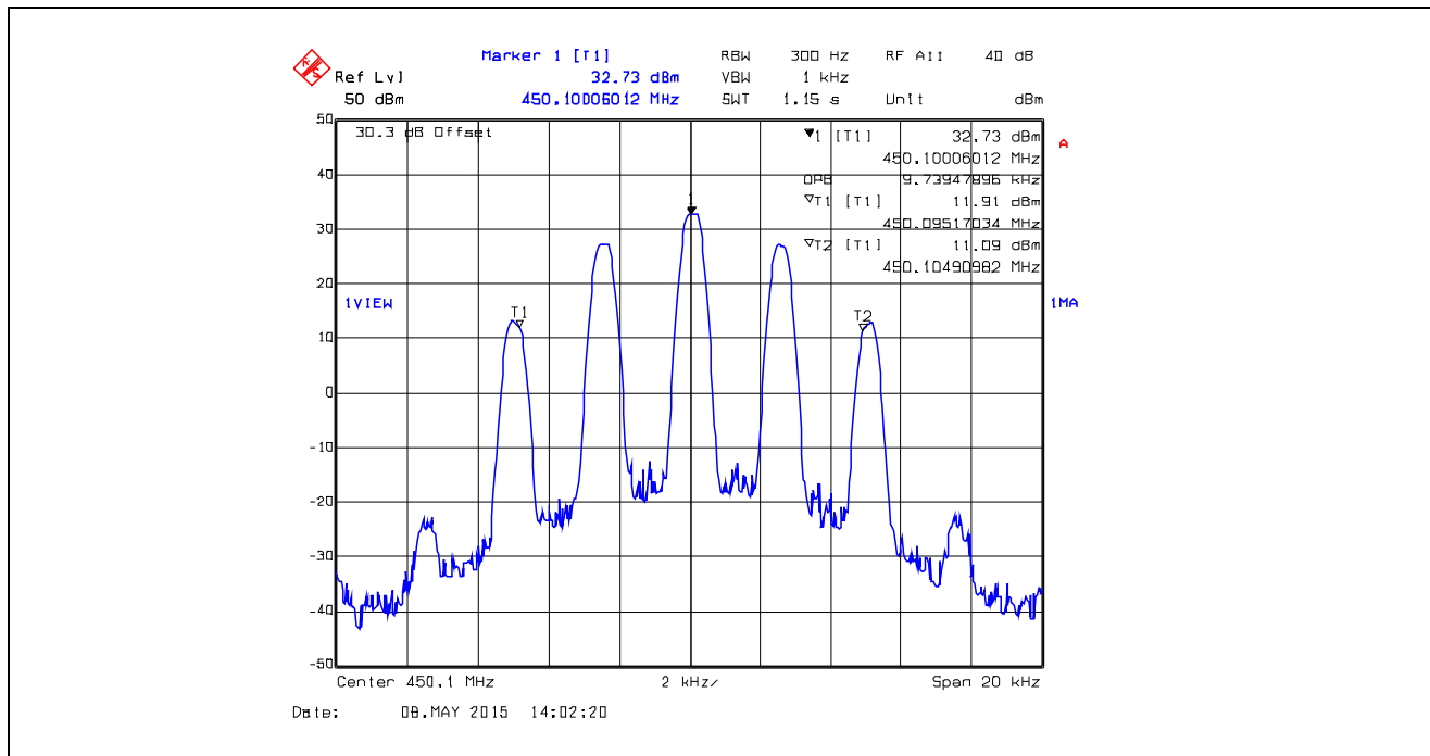
Plot 5.4.4.1.25. 99% Occupied Bandwidth, 12.5 kHz Channel Spacing, Analog, 450.1 MHz
