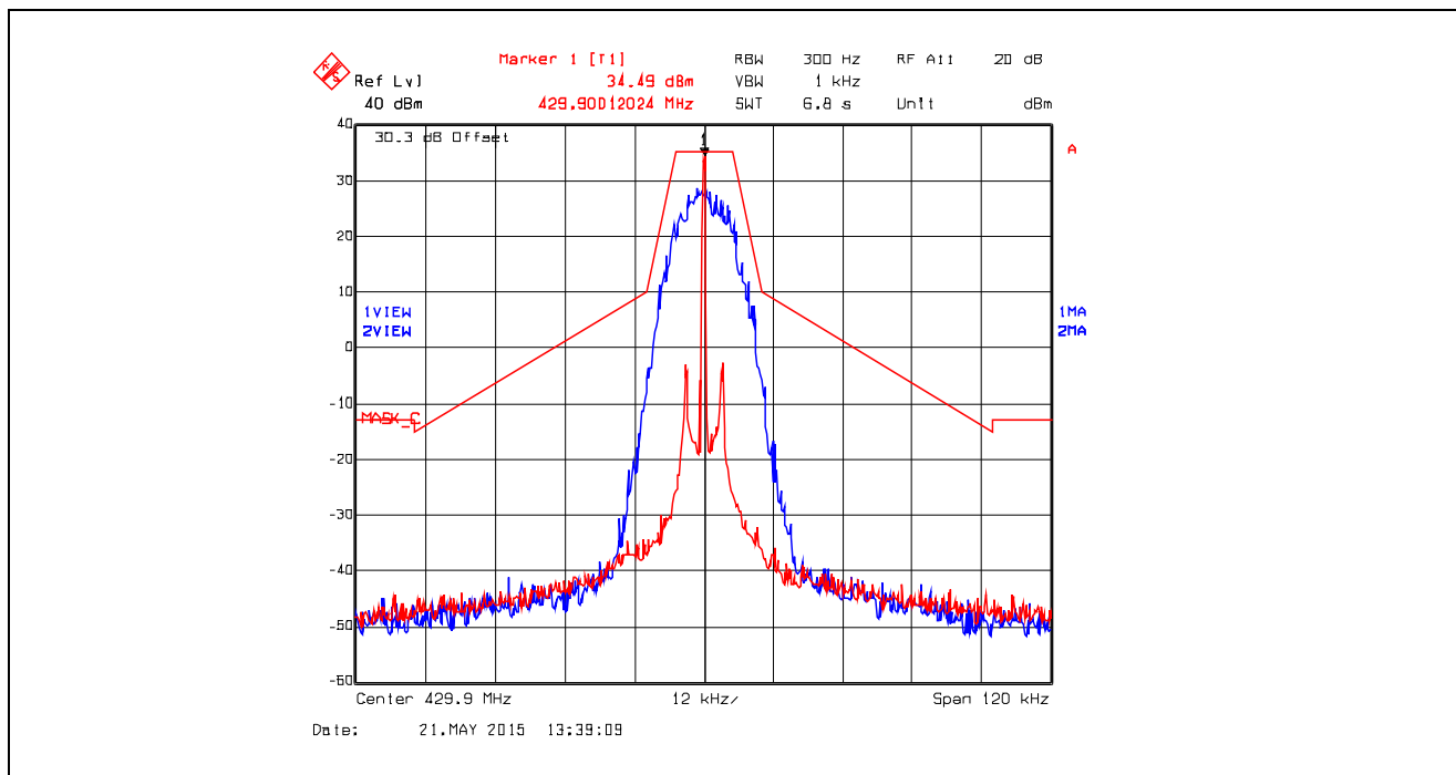
Plot 5.4.4.3.11. Emission Mask C, Digital at 19.2 kbps, 429.9 MHz, High Power
