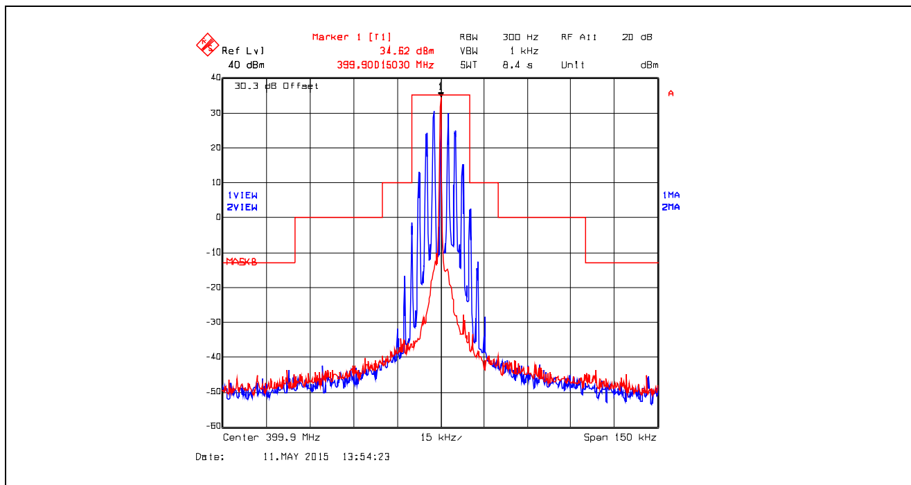
Plot 5.4.4.2.5. Emission Mask B, Analog, 399.9 MHz, High Power
