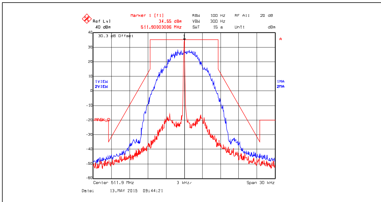
Plot 5.4.4.5.17. Emission Mask D, Digital at 9.6 kbps, 511.9 MHz, High Power
