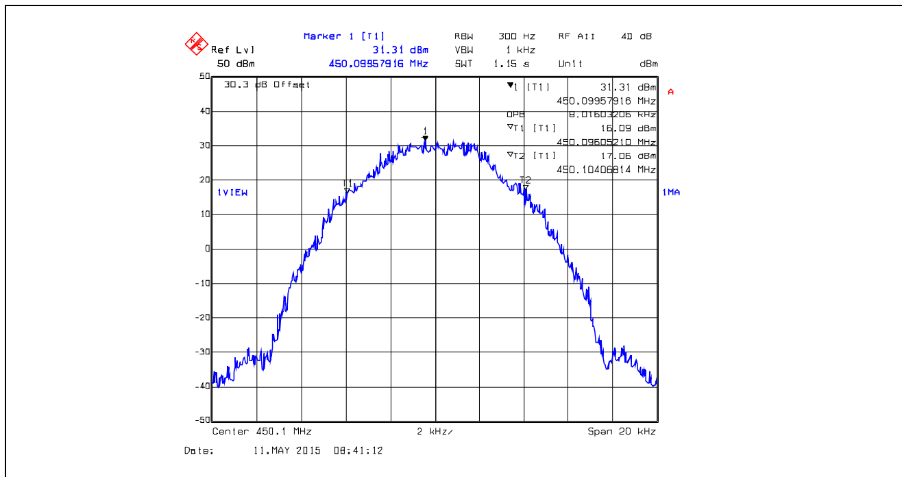
Plot 5.4.4.1.34. 99% Occupied Bandwidth, 12.5 kHz Channel Spacing, Digital 9.6 kbps, 450.1 MHz
