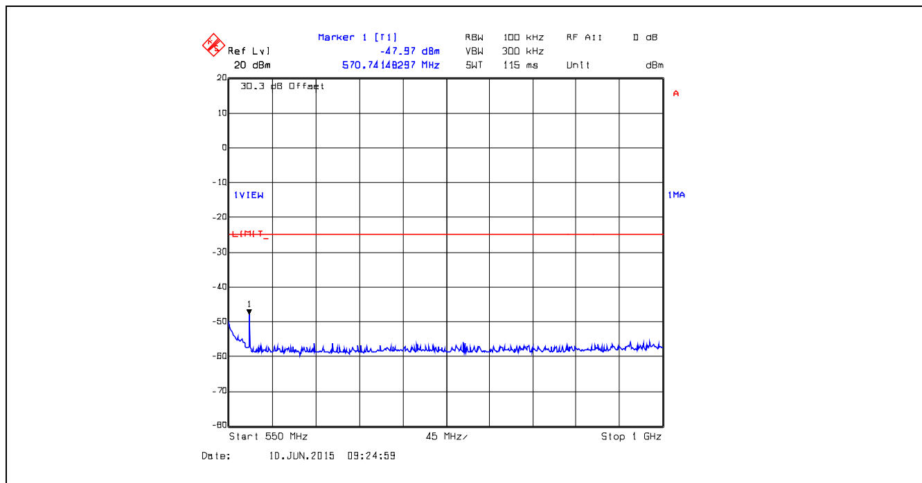
Plot 5.5.4.41. Conducted Transmitter Spurious Emissions, 450.1 MHz, Low Power, 550 MHz – 1 GHz
