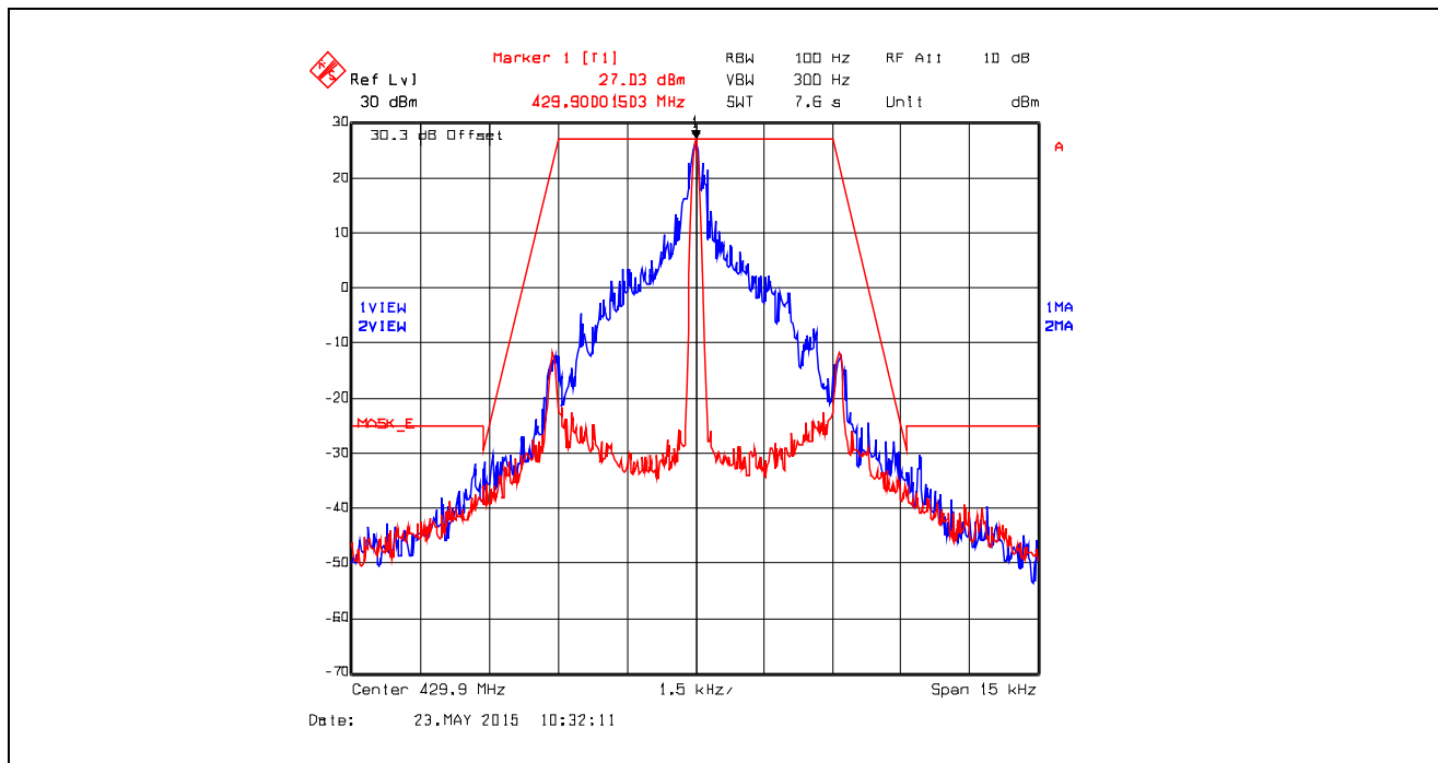
Plot 5.4.4.6.12. Emission Mask E, Digital at 4.8 kbps, 429.9 MHz, Low Power
