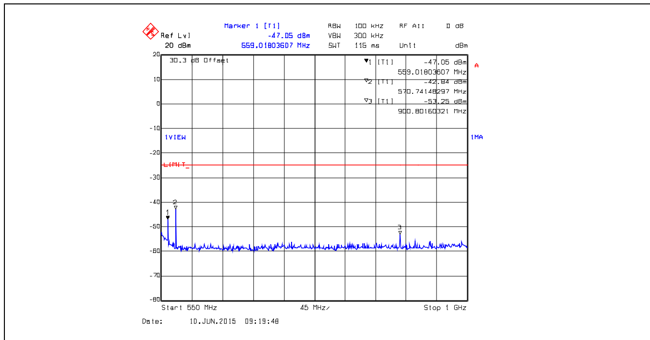
Plot 5.5.4.38. Conducted Transmitter Spurious Emissions, 450.1 MHz, High Power, 550 MHz – 1 GHz
