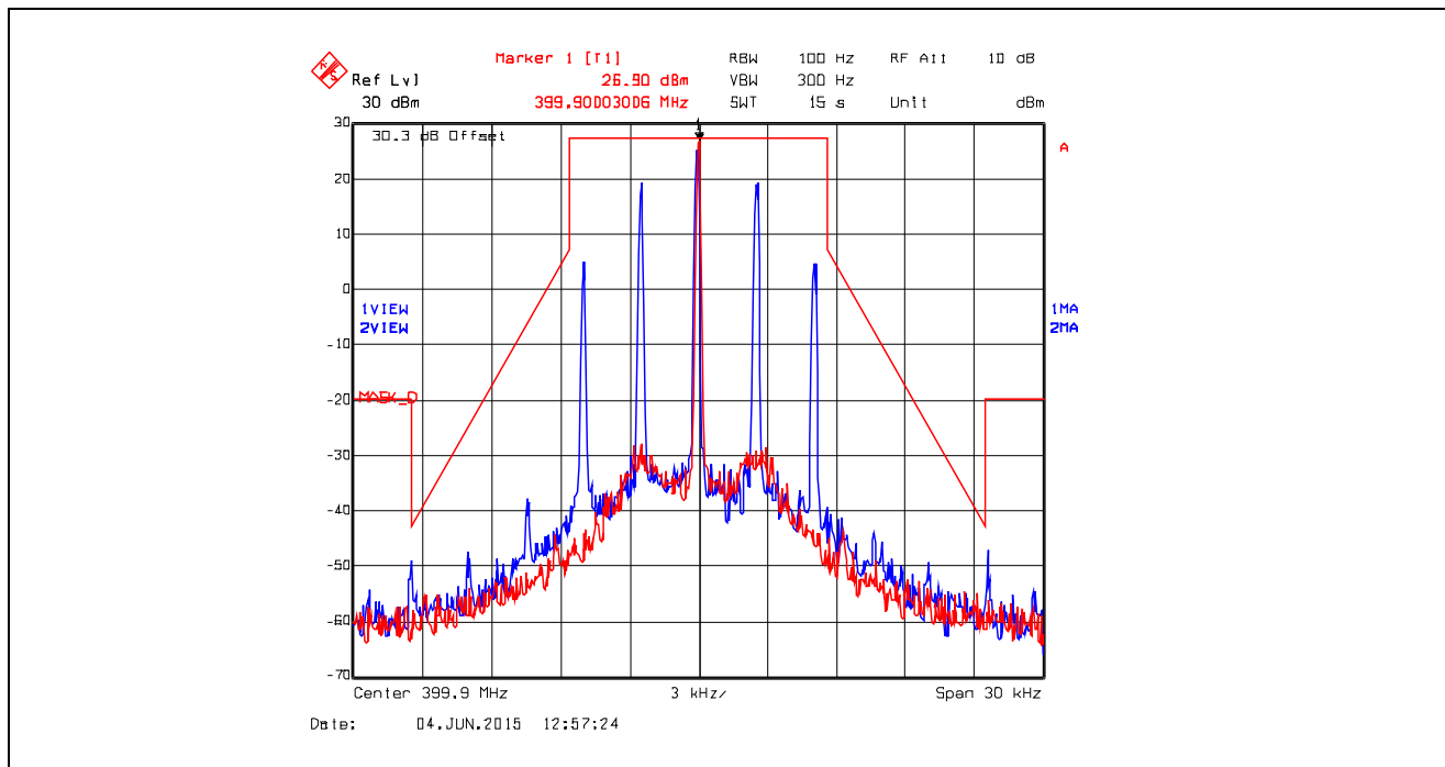
Plot 5.4.4.4.6. Emission Mask D, Analog, 399.9 MHz, Low Power
