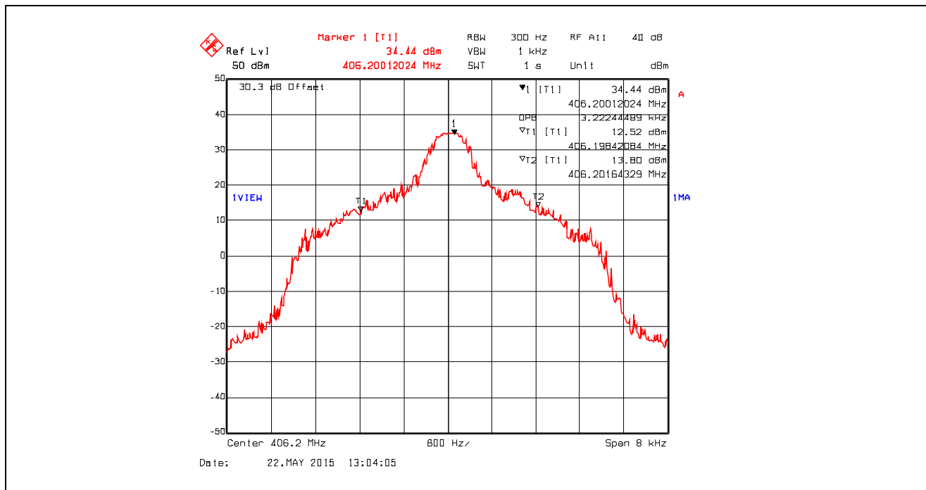
Plot 5.4.4.1.40. 99% Occupied Bandwidth, 6.25 kHz Channel Spacing, Digital 4.8 kbps, 406.2 MHz
