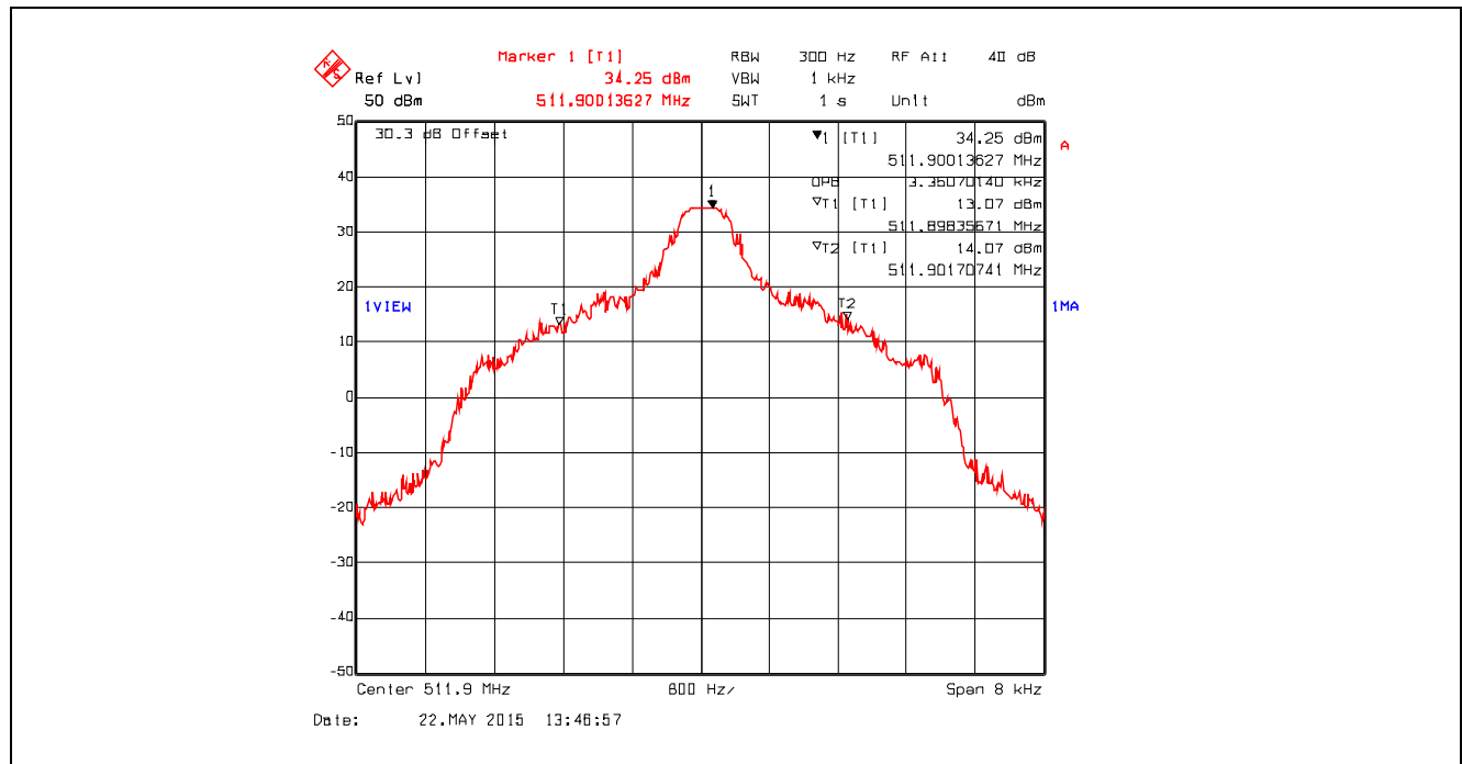
Plot 5.4.4.1.45. 99% Occupied Bandwidth, 6.25 kHz Channel Spacing, Digital 4.8 kbps, 511.9 MHz
