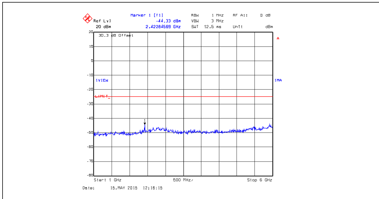
Plot 5.5.4.54. Conducted Transmitter Spurious Emissions, 511.9 MHz, Low Power, 1 GHz – 6 GHz
