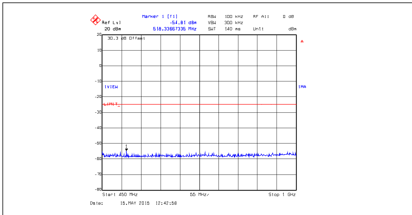
Plot 5.5.4.29. Conducted Transmitter Spurious Emissions, 415.0 MHz, Low Power, 450 MHz – 1 GHz
