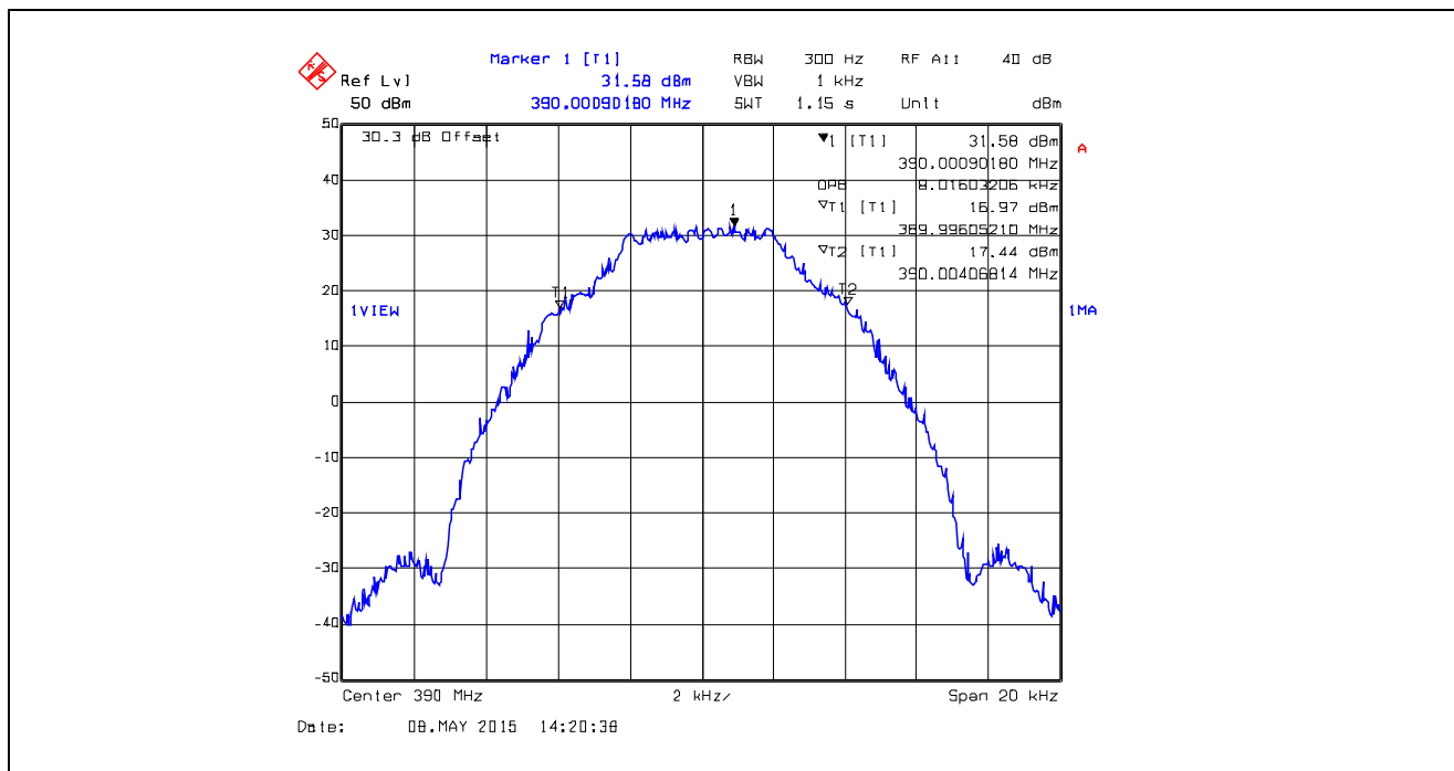
Plot 5.4.4.1.29. 99% Occupied Bandwidth, 12.5 kHz Channel Spacing, Digital 9.6 kbps, 390.0 MHz
