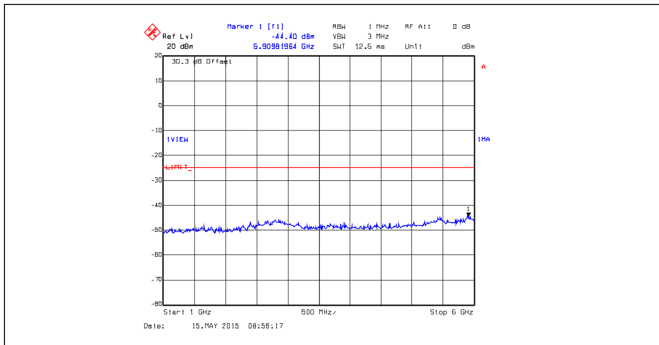
Plot 5.5.4.33. Conducted Transmitter Spurious Emissions, 429.9 MHz, High Power, 1 GHz – 6 GHz
