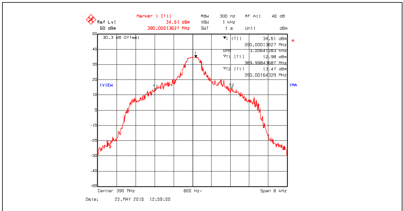
Plot 5.4.4.1.38. 99% Occupied Bandwidth, 6.25 kHz Channel Spacing, Digital 4.8 kbps, 390.0 MHz
