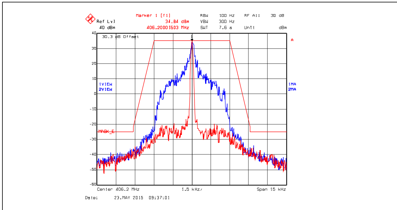
Plot 5.4.4.6.7. Emission Mask E, Digital at 4.8 kbps, 406.2 MHz, High Power
