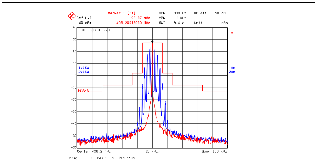
Plot 5.4.4.2.8. Emission Mask B, Analog, 406.2 MHz, Low Power
