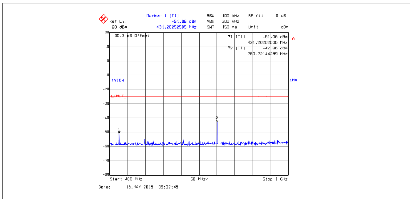
Plot 5.5.4.2. Conducted Transmitter Spurious Emissions, 380.1 MHz, High Power, 400 MHz – 1 GHz
