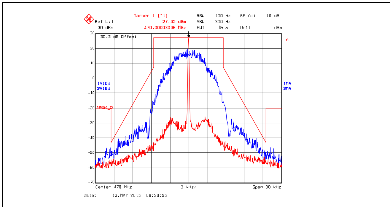
Plot 5.4.4.5.16. Emission Mask D, Digital at 9.6 kbps, 470.0 MHz, Low Power
