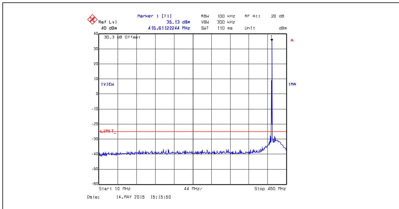
Plot 5.5.4.25. Conducted Transmitter Spurious Emissions, 415.0 MHz, High Power, 10 MHz – 450 MHz
