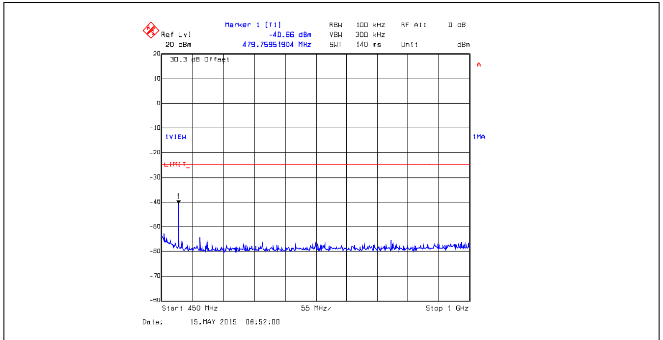
Plot 5.5.4.32. Conducted Transmitter Spurious Emissions, 429.9 MHz, High Power, 450 MHz – 1 GHz
