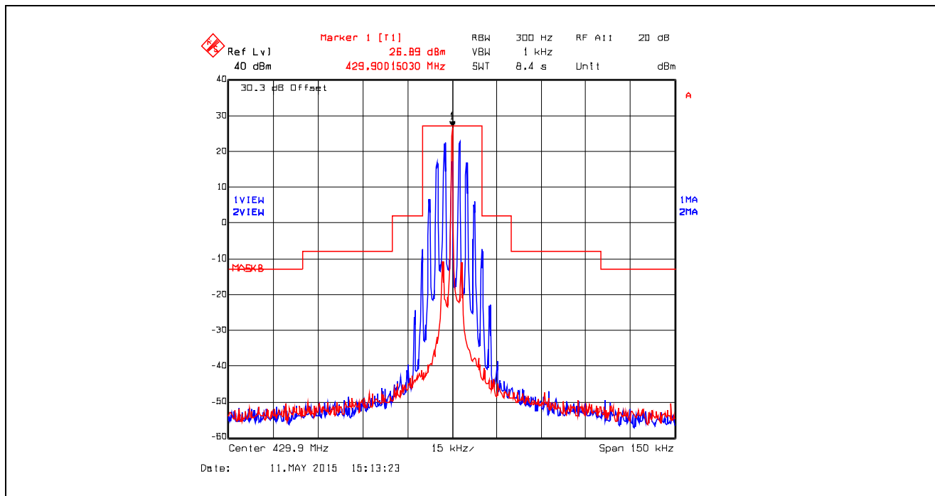
Plot 5.4.4.2.12. Emission Mask B, Analog, 429.9 MHz, Low Power
