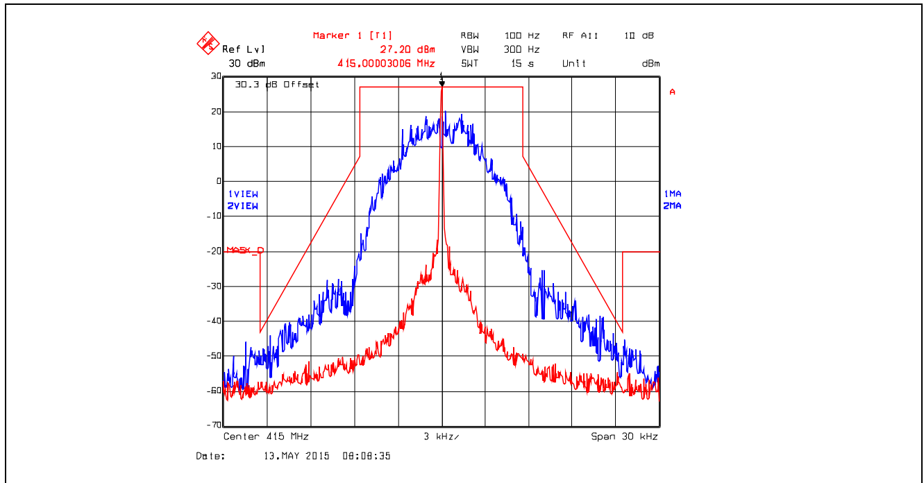
Plot 5.4.4.5.10. Emission Mask D, Digital at 9.6 kbps, 415.0 MHz, Low Power
