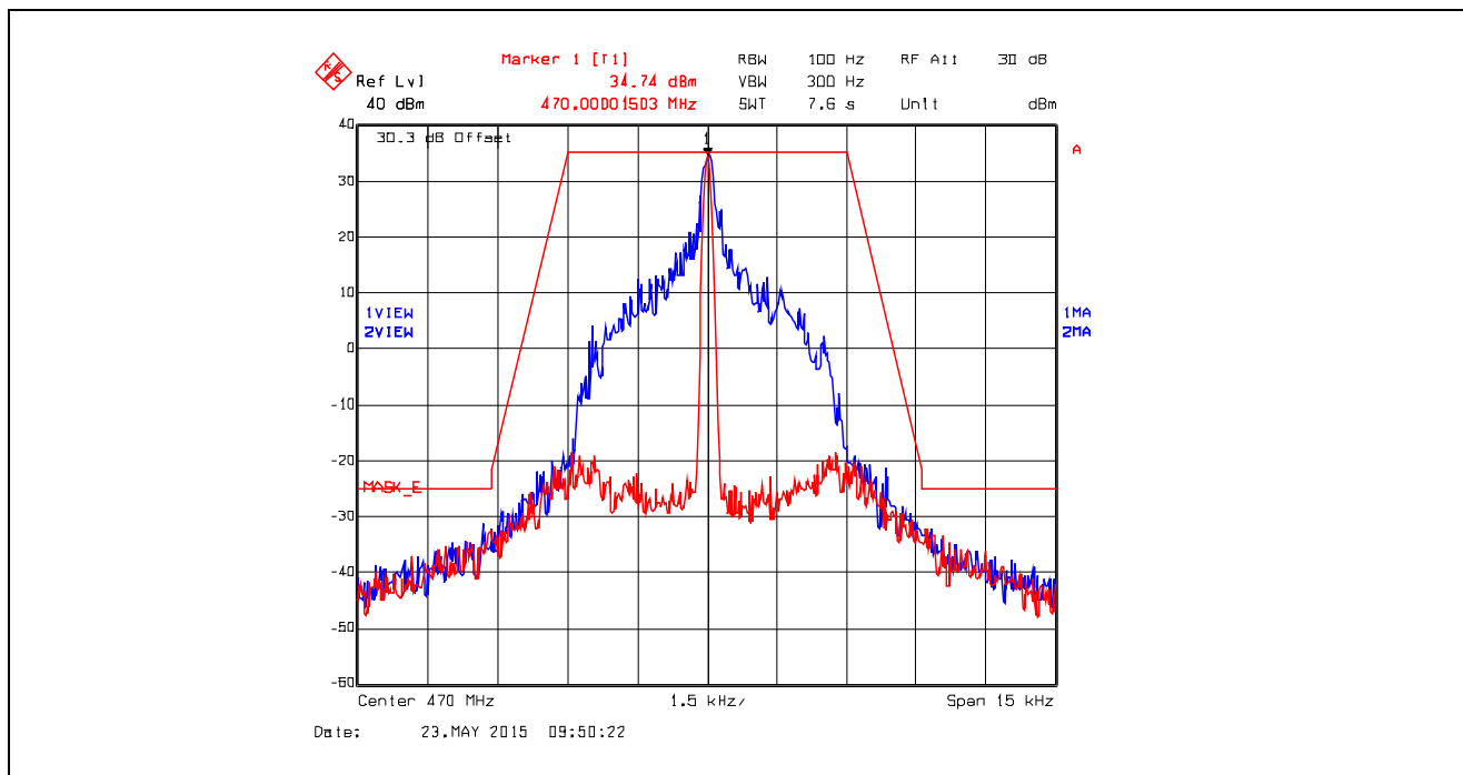
Plot 5.4.4.6.15. Emission Mask E, Digital at 4.8 kbps, 470.0 MHz, High Power
