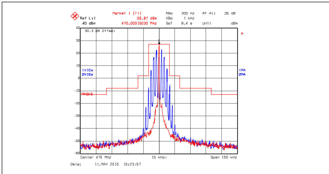
Plot 5.4.4.2.16. Emission Mask B, Analog, 470.0 MHz, Low Power
