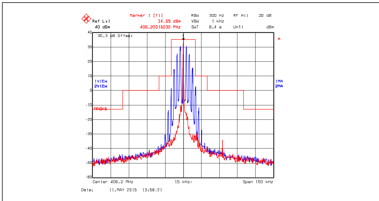
Plot 5.4.4.2.7. Emission Mask B, Analog, 406.2 MHz, High Power
