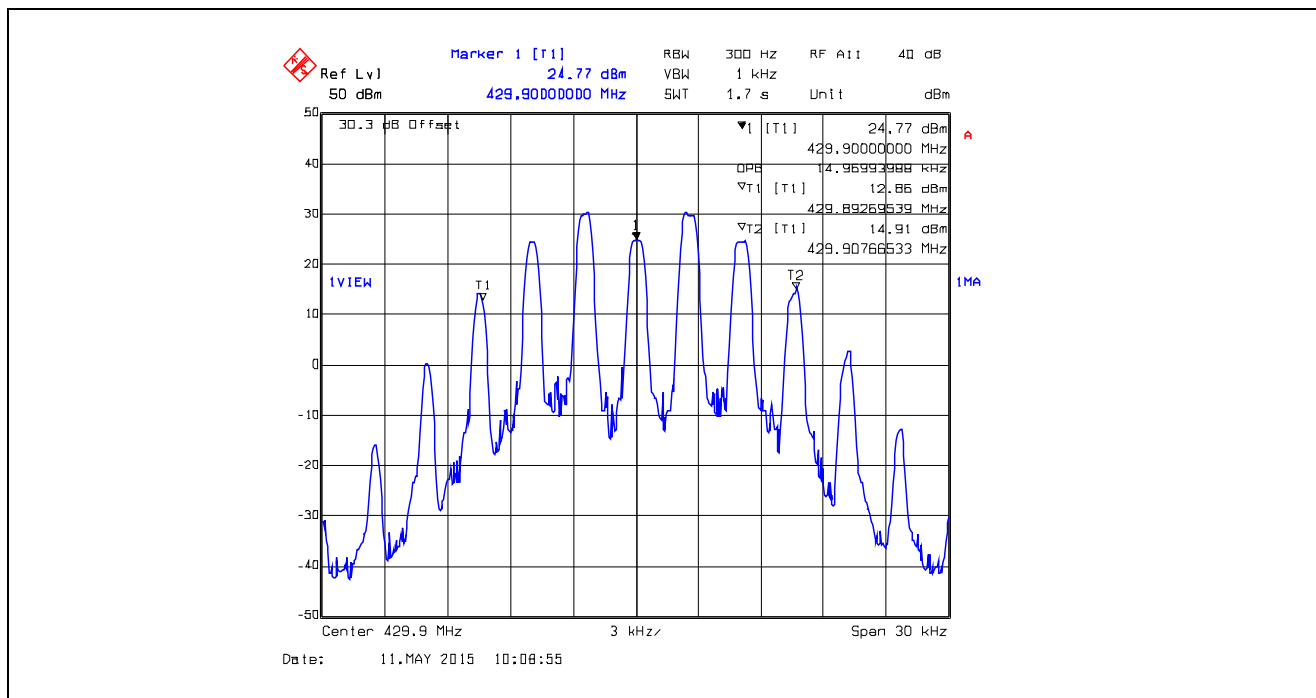
Plot 5.4.4.1.6. 99% Occupied Bandwidth, 25 kHz Channel Spacing, Analog, 429.9 MHz
