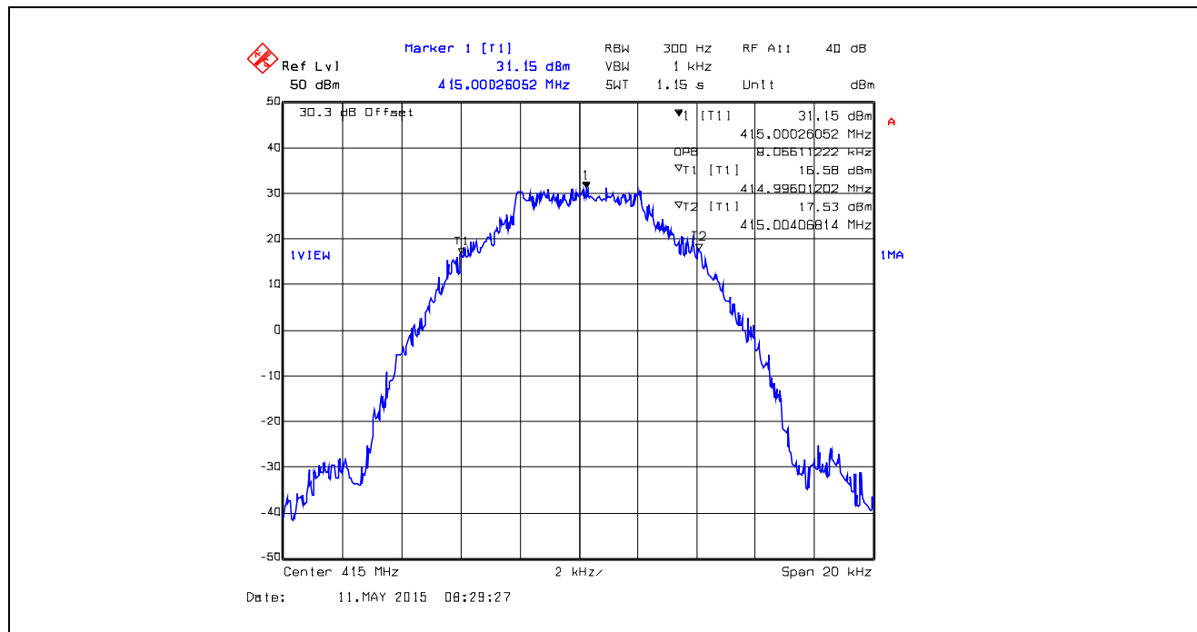
Plot 5.4.4.1.32. 99% Occupied Bandwidth, 12.5 kHz Channel Spacing, Digital 9.6 kbps, 415.0 MHz
