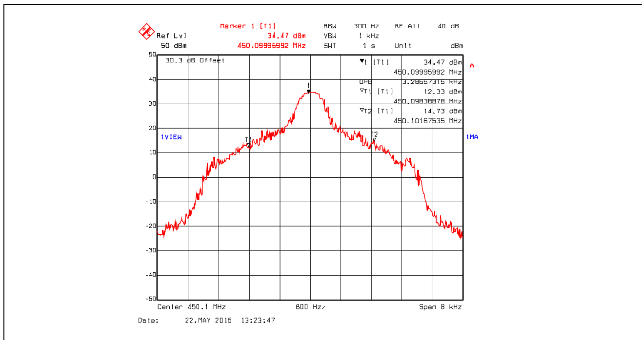
Plot 5.4.4.1.43. 99% Occupied Bandwidth, 6.25 kHz Channel Spacing, Digital 4.8 kbps, 450.1 MHz
