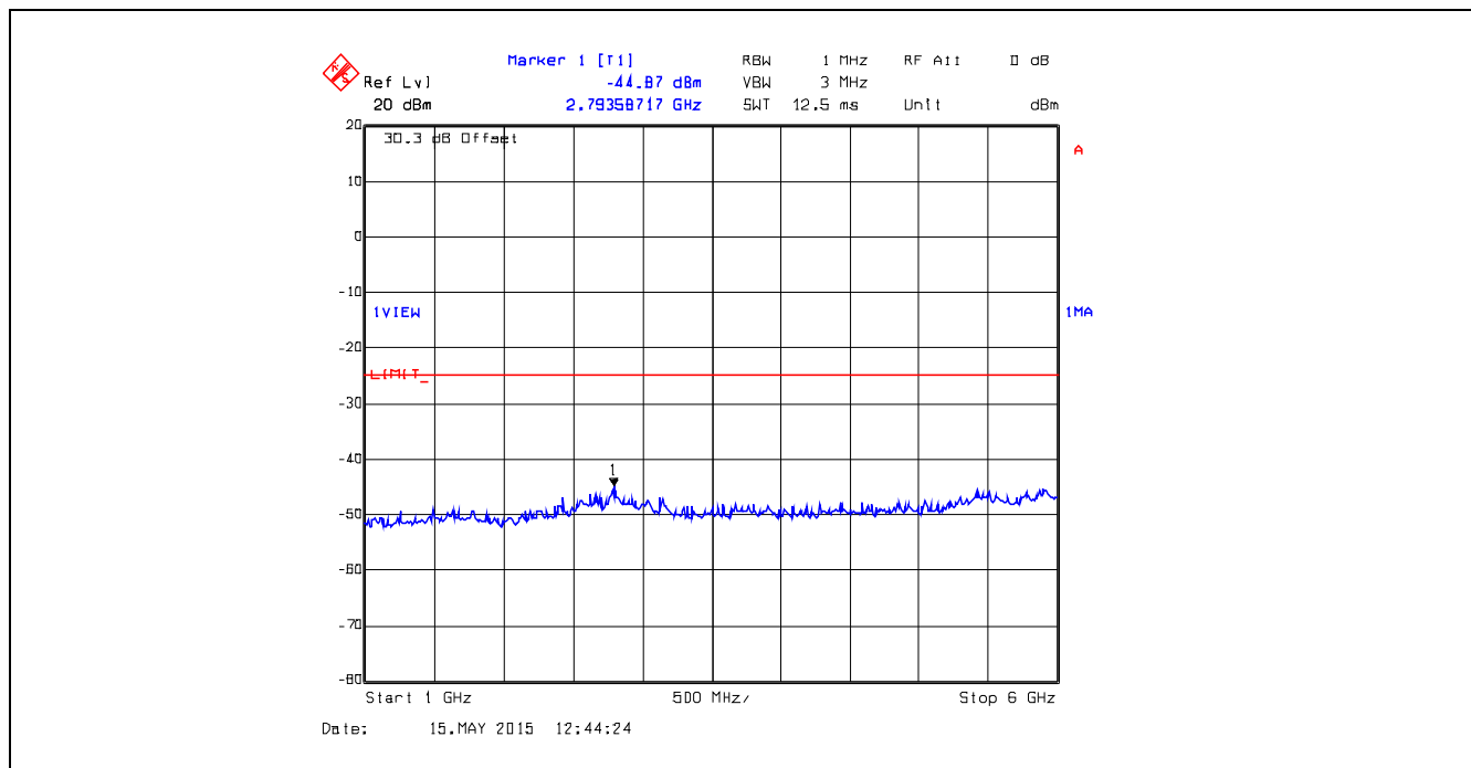
Plot 5.5.4.30. Conducted Transmitter Spurious Emissions, 415.0 MHz, Low Power, 1 GHz – 6 GHz
