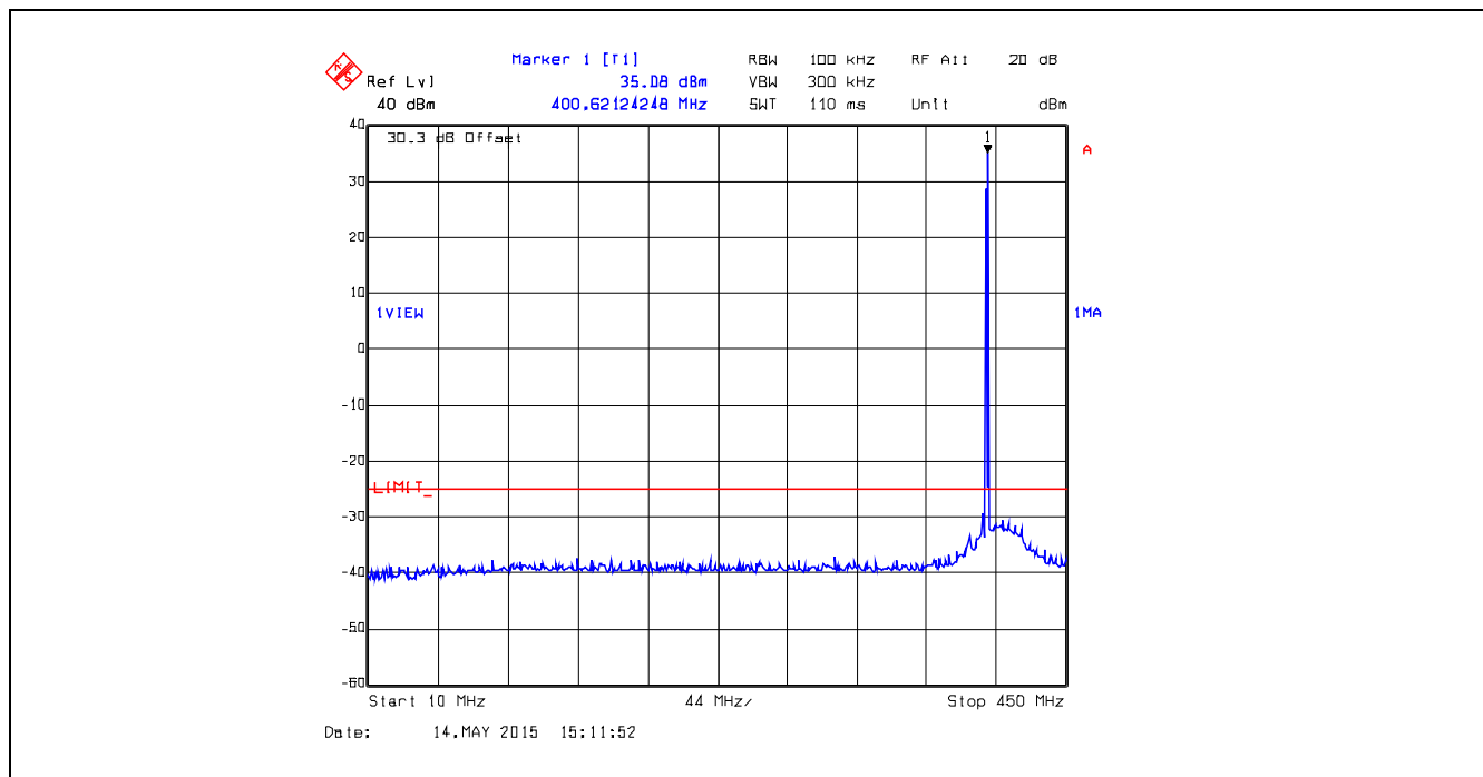
Plot 5.5.4.13. Conducted Transmitter Spurious Emissions, 399.9 MHz, High Power, 10 MHz – 450 MHz
