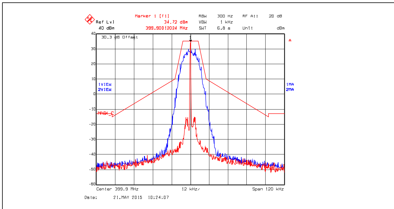
Plot 5.4.4.3.5. Emission Mask C, Digital at 19.2 kbps, 399.9 MHz, High Power
