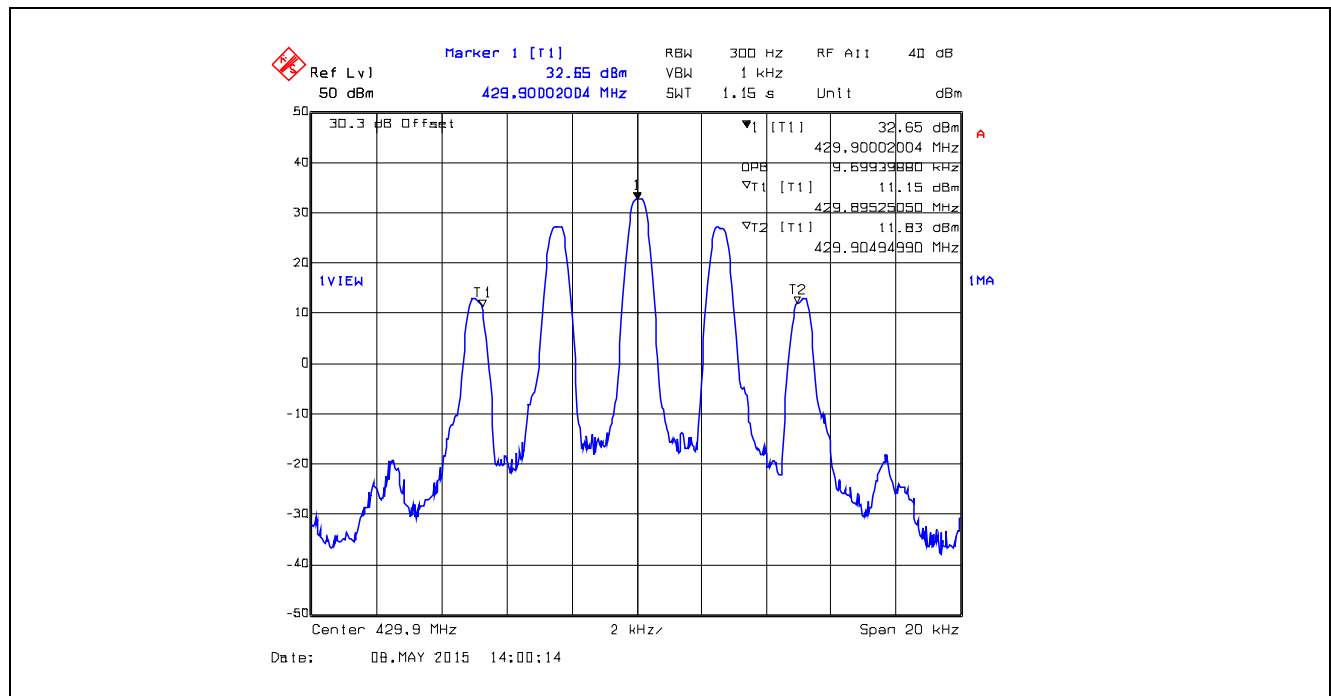
Plot 5.4.4.1.24. 99% Occupied Bandwidth, 12.5 kHz Channel Spacing, Analog, 429.9 MHz
