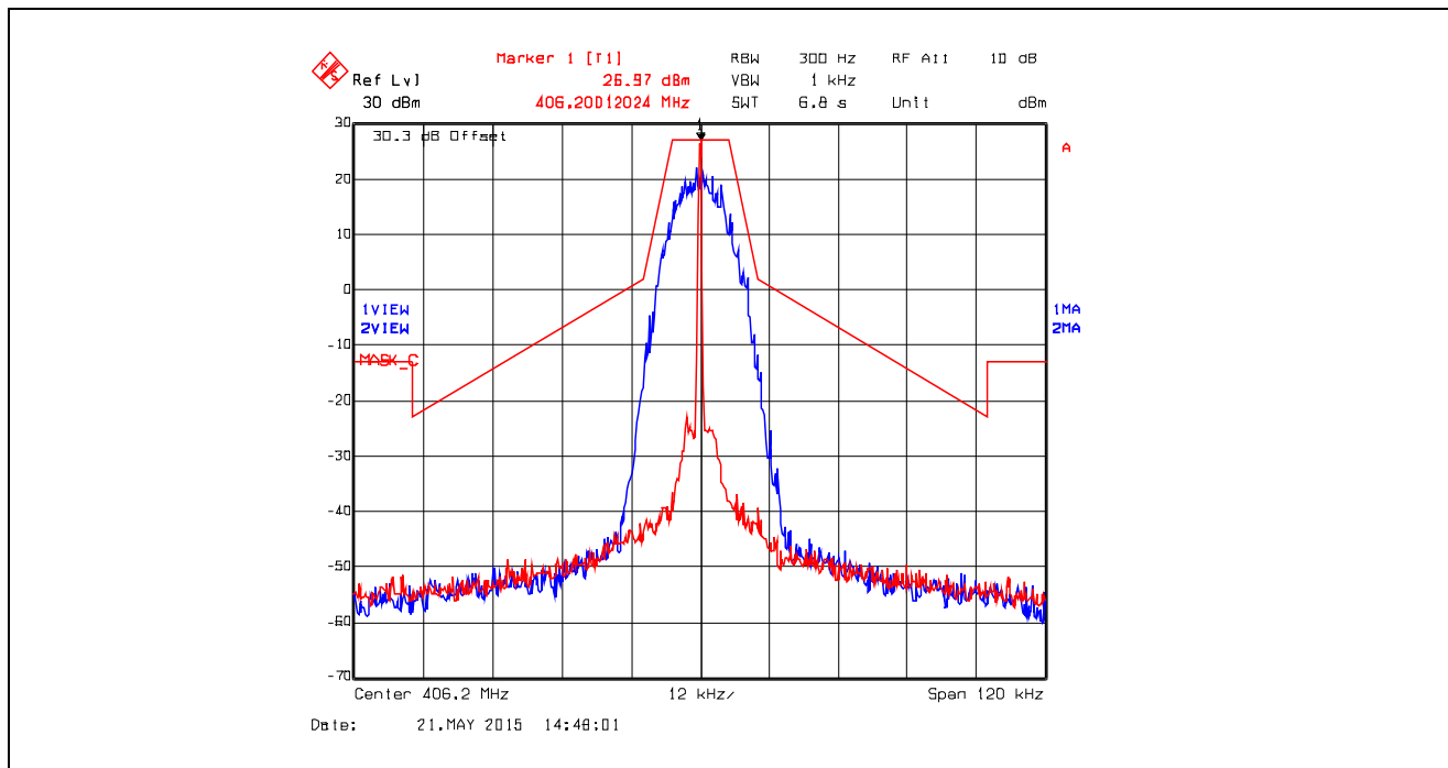
Plot 5.4.4.3.8. Emission Mask C, Digital at 19.2 kbps, 406.2 MHz, Low Power
