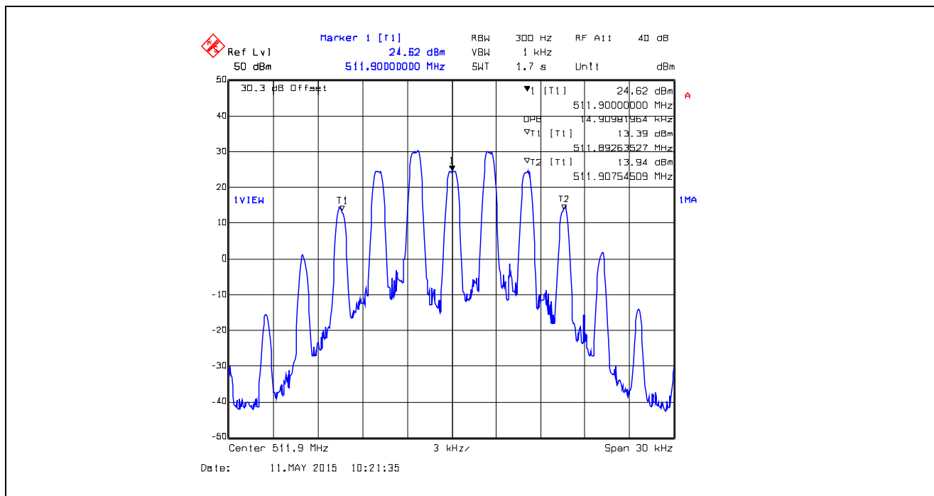
Plot 5.4.4.1.9. 99% Occupied Bandwidth, 25 kHz Channel Spacing, Analog, 511.9 MHz
