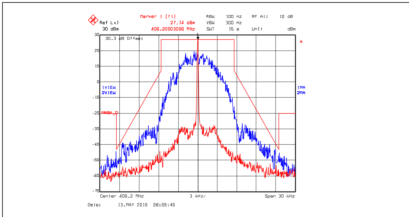
Plot 5.4.4.5.8. Emission Mask D, Digital at 9.6 kbps, 406.2 MHz, Low Power
