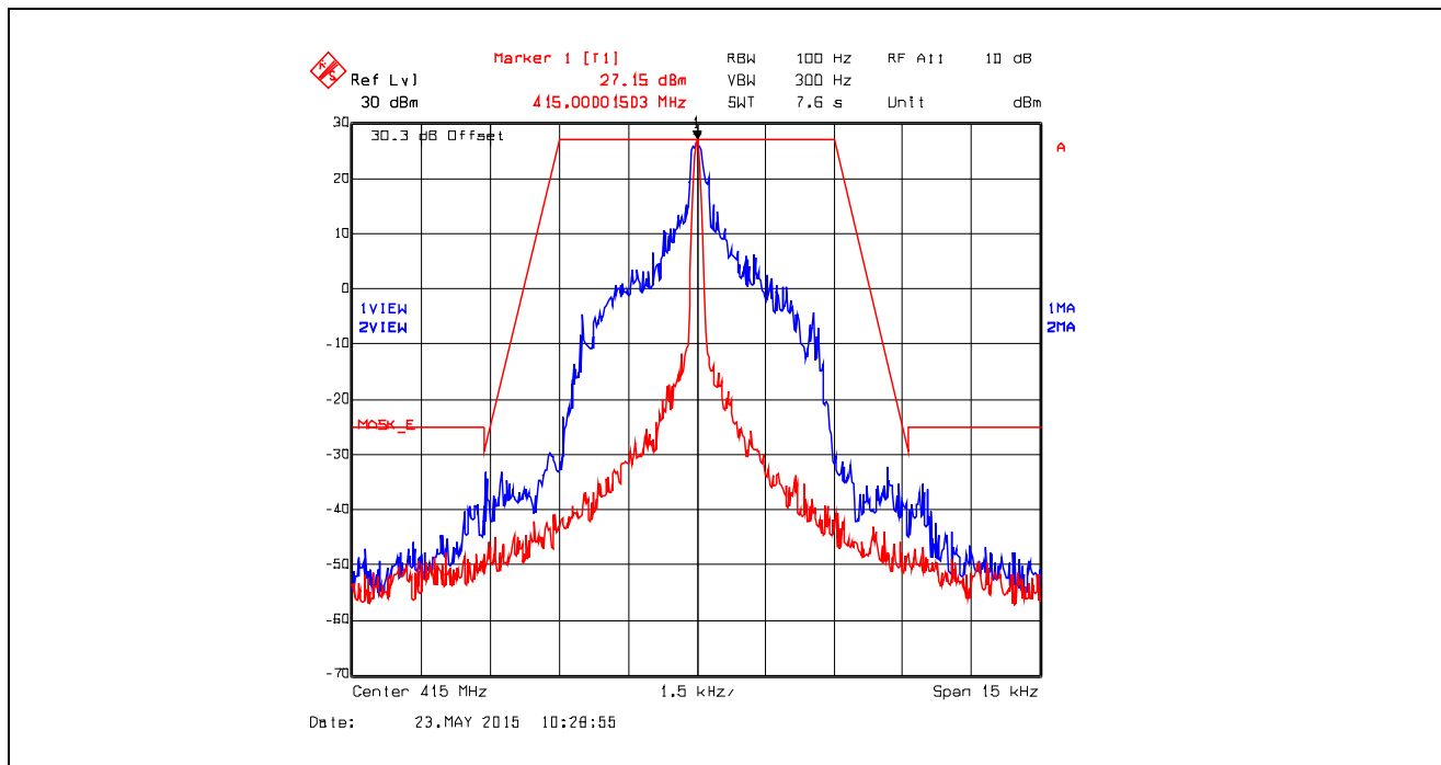
Plot 5.4.4.6.10. Emission Mask E, Digital at 4.8 kbps, 415.0 MHz, Low Power
