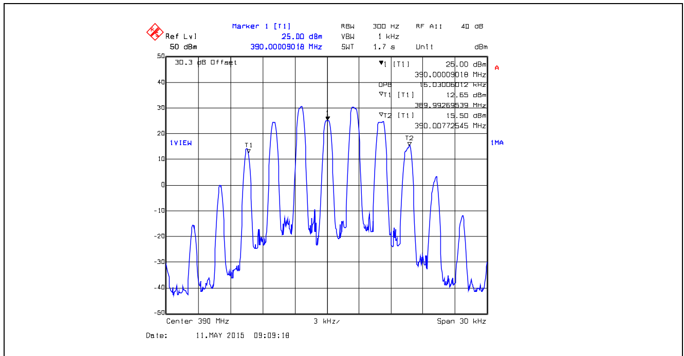
Plot 5.4.4.1.2. 99% Occupied Bandwidth, 25 kHz Channel Spacing, Analog, 390.0 MHz
