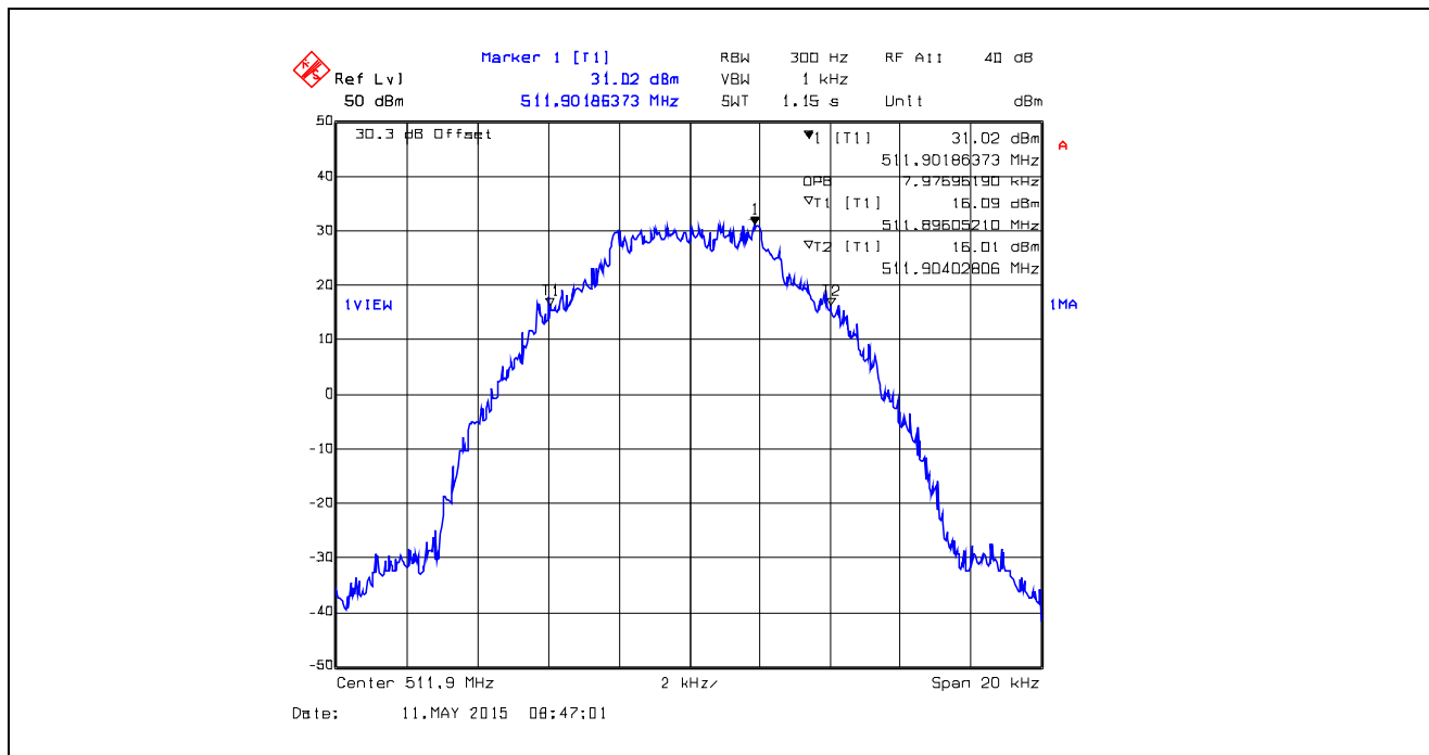
Plot 5.4.4.1.36. 99% Occupied Bandwidth, 12.5 kHz Channel Spacing, Digital 9.6 kbps, 511.9 MHz
