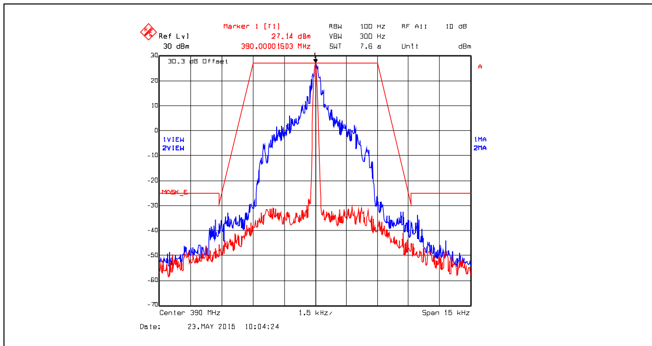
Plot 5.4.4.6.4. Emission Mask E, Digital at 4.8 kbps, 390.0 MHz, Low Power
