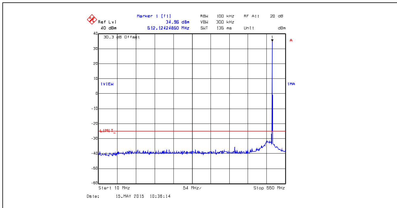
Plot 5.5.4.49. Conducted Transmitter Spurious Emissions, 511.9 MHz, High Power, 10 MHz – 550 MHz
