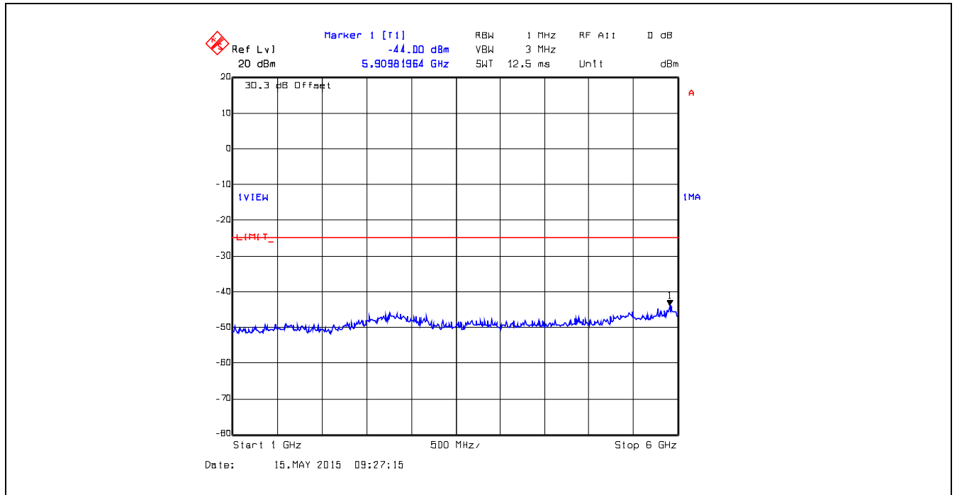
Plot 5.5.4.9. Conducted Transmitter Spurious Emissions, 390.0 MHz, High Power, 1 GHz – 6 GHz
