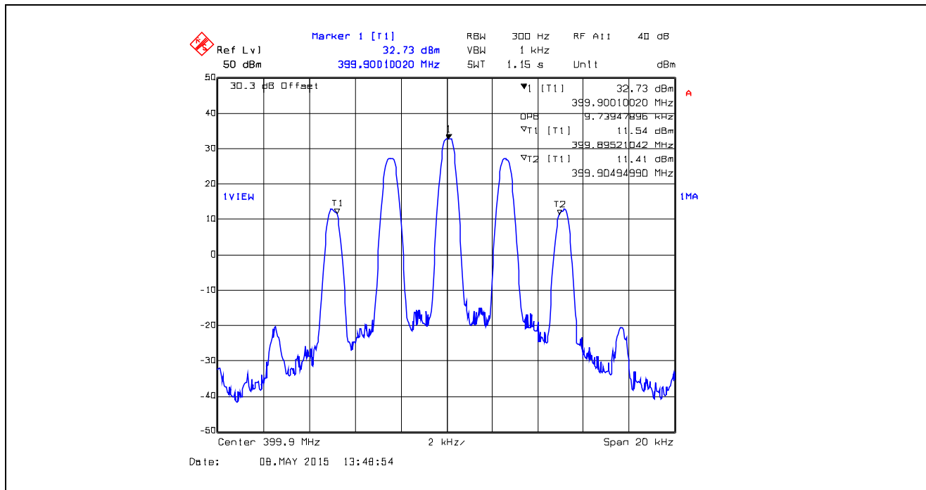
Plot 5.4.4.1.21. 99% Occupied Bandwidth, 12.5 kHz Channel Spacing, Analog, 399.9 MHz
