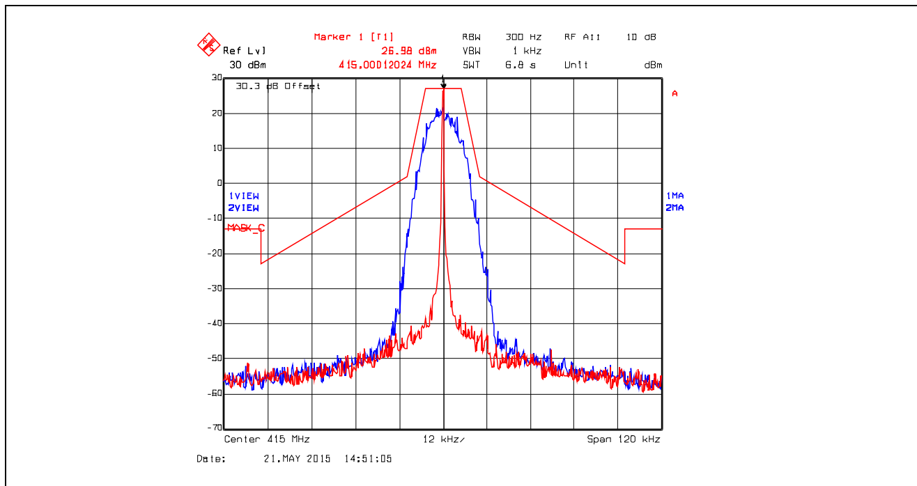
Plot 5.4.4.3.10. Emission Mask C, Digital at 19.2 kbps, 415.0 MHz, Low Power
