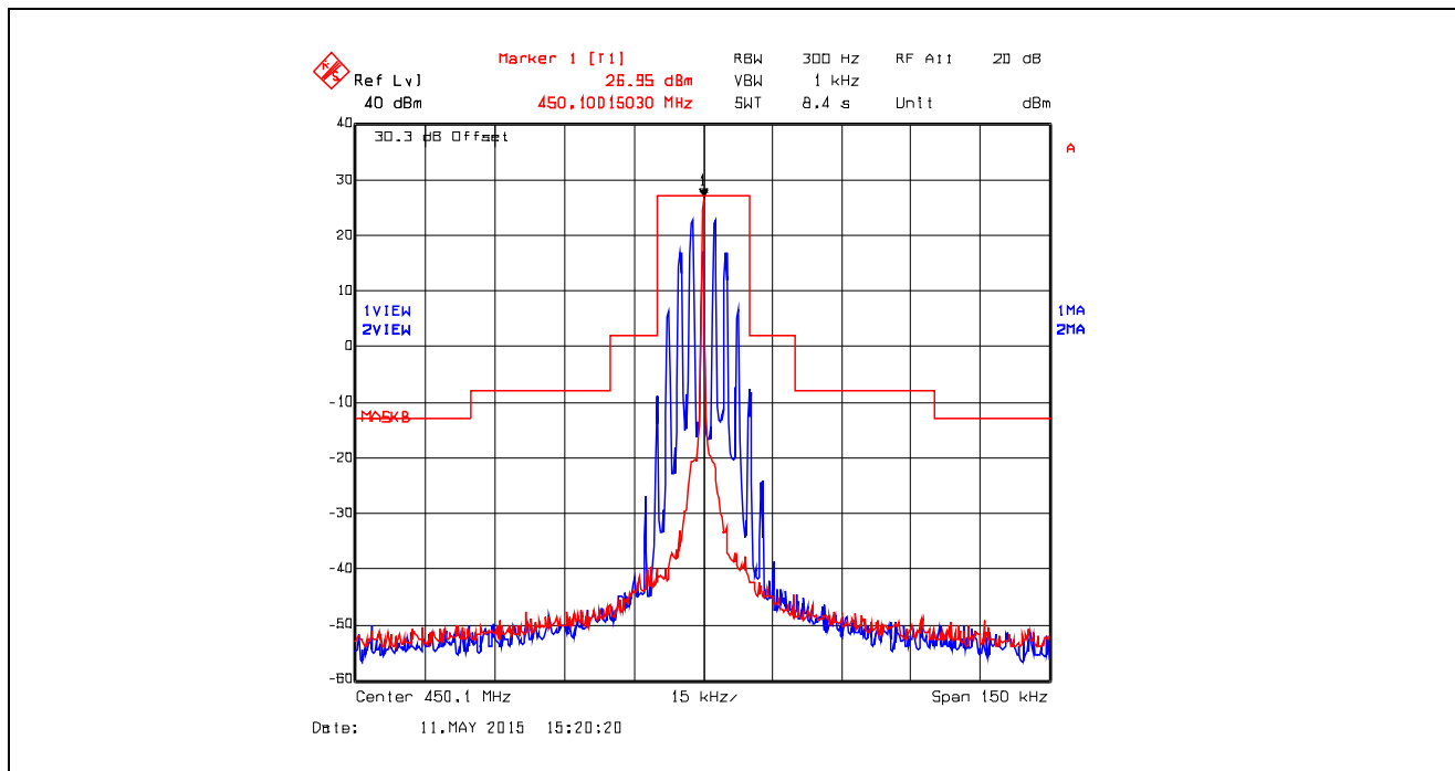
Plot 5.4.4.2.14. Emission Mask B, Analog, 450.1 MHz, Low Power
