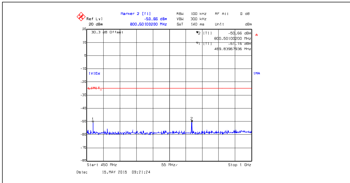
Plot 5.5.4.14. Conducted Transmitter Spurious Emissions, 399.9 MHz, High Power, 450 MHz – 1 GHz
