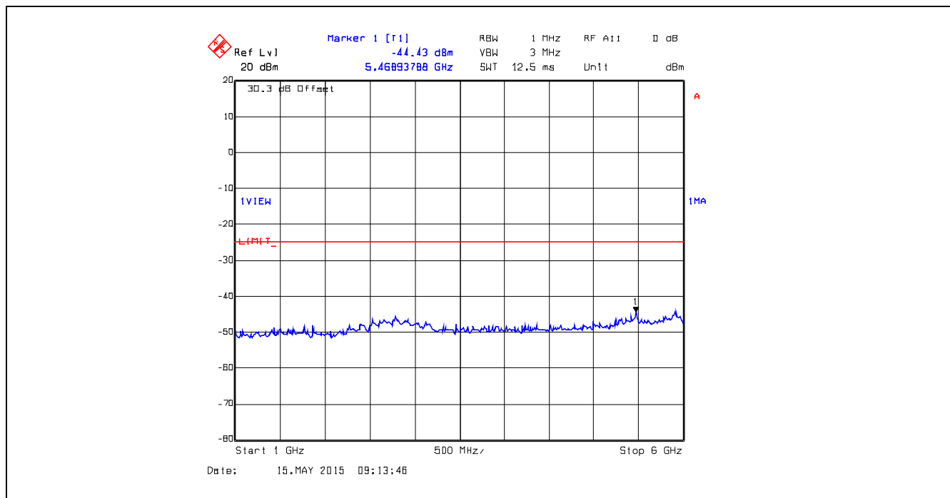
Plot 5.5.4.15. Conducted Transmitter Spurious Emissions, 399.9 MHz, High Power, 1 GHz – 6 GHz
