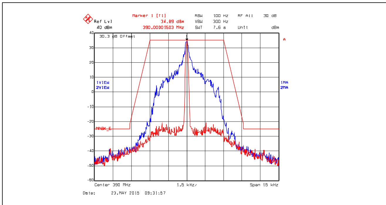
Plot 5.4.4.6.3. Emission Mask E, Digital at 4.8 kbps, 390.0 MHz, High Power
