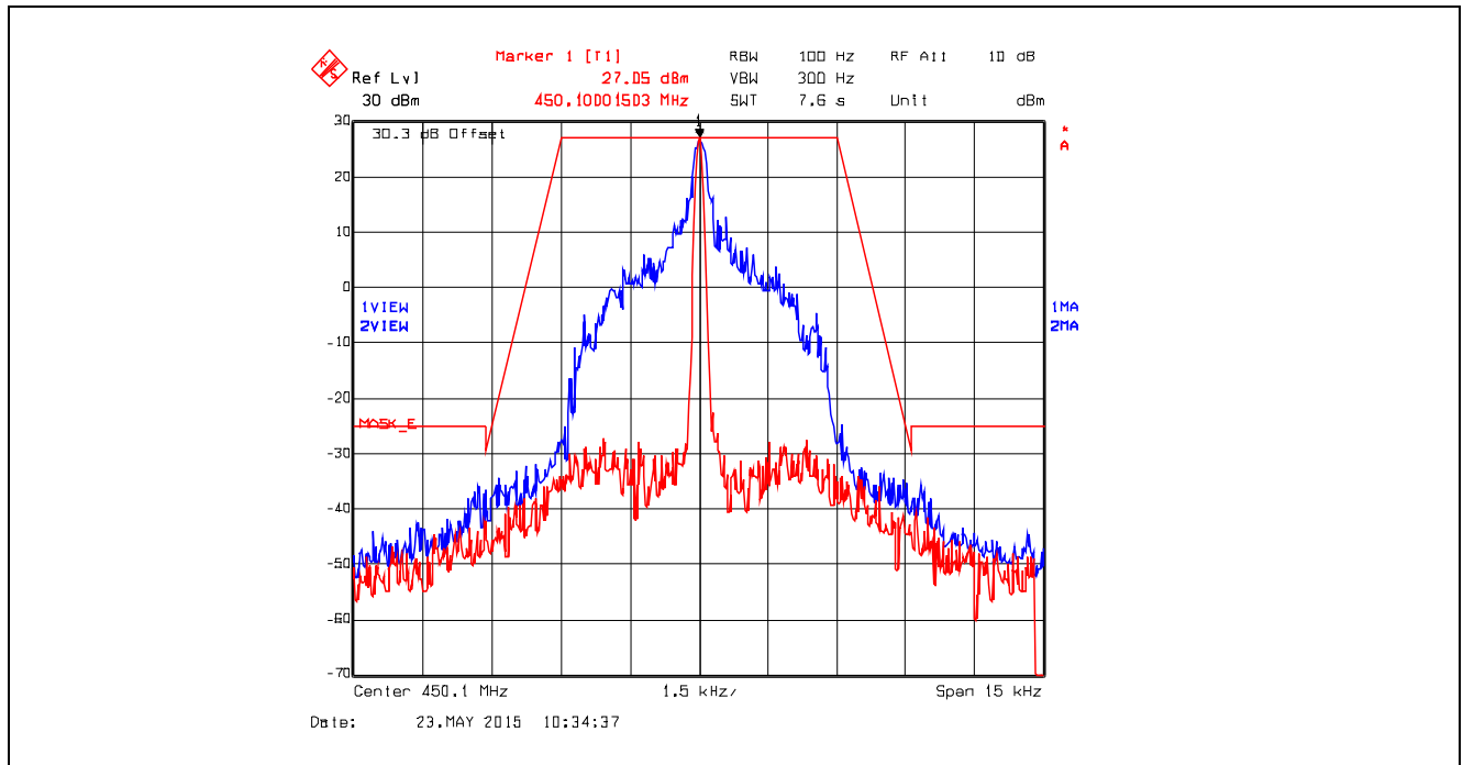
Plot 5.4.4.6.14. Emission Mask E, Digital at 4.8 kbps, 450.1 MHz, Low Power
