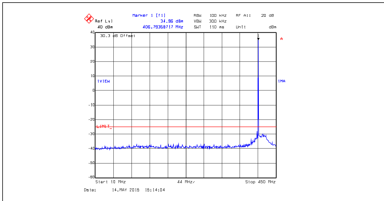
Plot 5.5.4.19. Conducted Transmitter Spurious Emissions, 406.2 MHz, High Power, 10 MHz – 450 MHz
