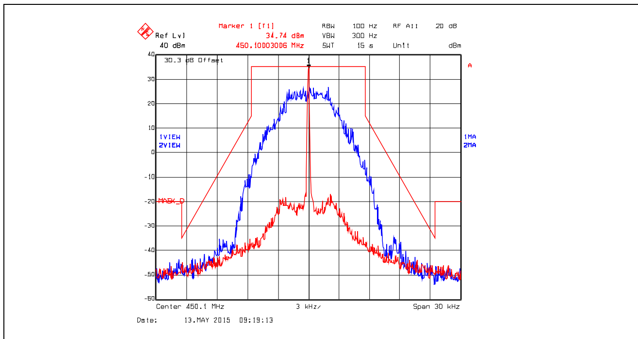
Plot 5.4.4.5.13. Emission Mask D, Digital at 9.6 kbps, 450.1 MHz, High Power
