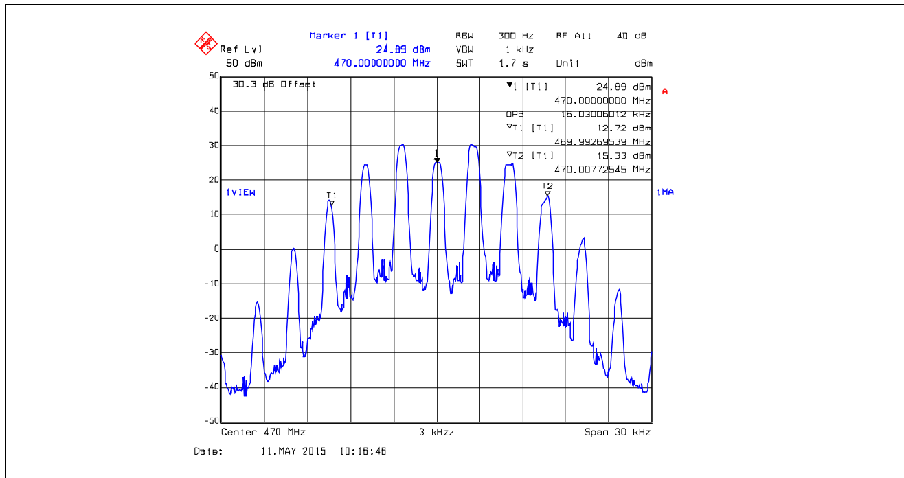
Plot 5.4.4.1.8. 99% Occupied Bandwidth, 25 kHz Channel Spacing, Analog, 470.0 MHz
