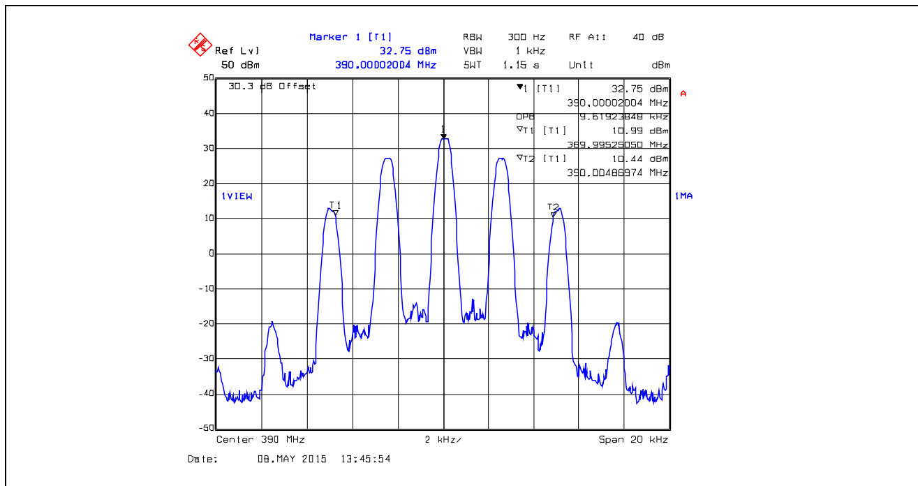
Plot 5.4.4.1.20. 99% Occupied Bandwidth, 12.5 kHz Channel Spacing, Analog, 390.0 MHz
