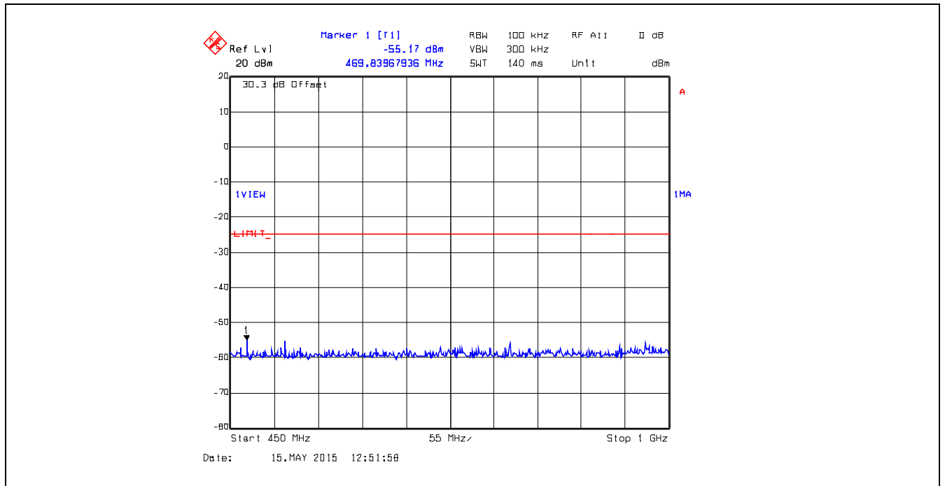
Plot 5.5.4.17. Conducted Transmitter Spurious Emissions, 399.9 MHz, Low Power, 450 MHz – 1 GHz
