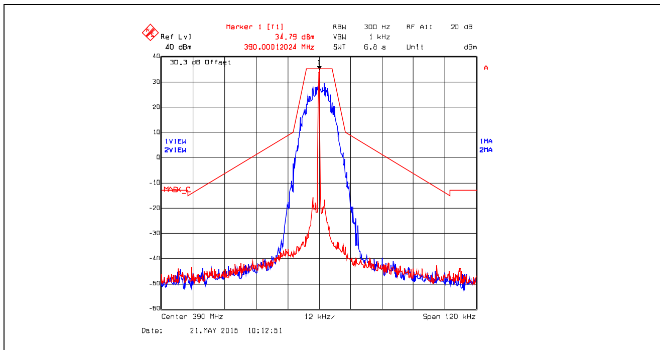
Plot 5.4.4.3.3. Emission Mask C, Digital at 19.2 kbps, 390.0 MHz, High Power
