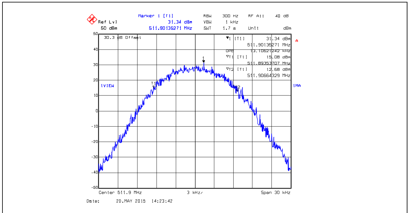
Plot 5.4.4.1.18. 99% Occupied Bandwidth, 25 kHz Channel Spacing, Digital 19.2 kbps, 511.9 MHz
