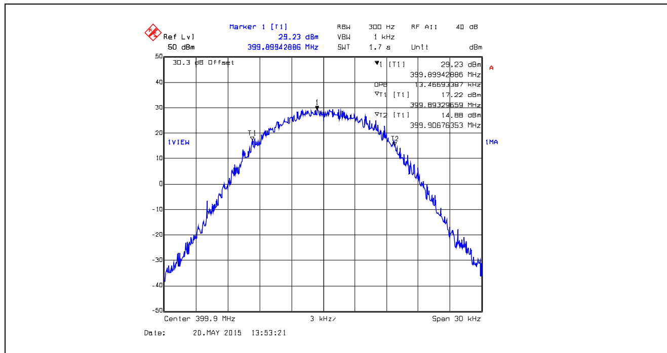
Plot 5.4.4.1.12. 99% Occupied Bandwidth, 25 kHz Channel Spacing, Digital 19.2 kbps, 399.9 MHz
