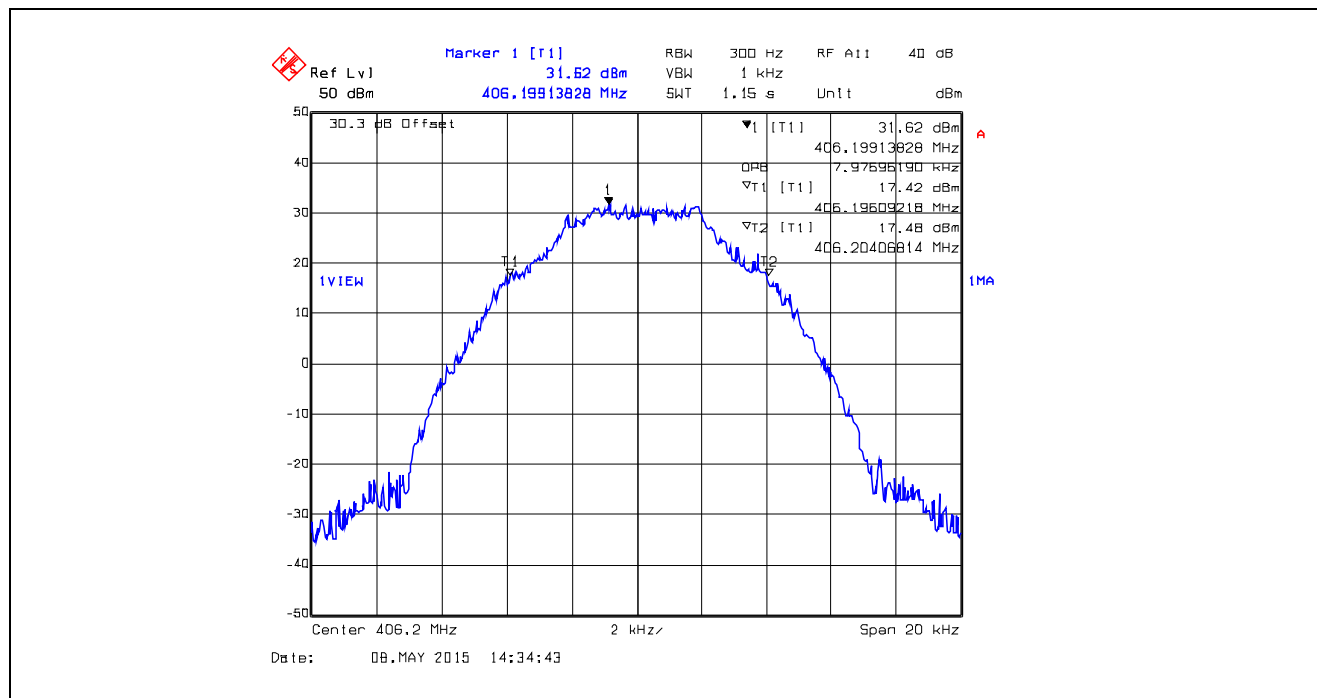
Plot 5.4.4.1.31. 99% Occupied Bandwidth, 12.5 kHz Channel Spacing, Digital 9.6 kbps, 406.2 MHz
