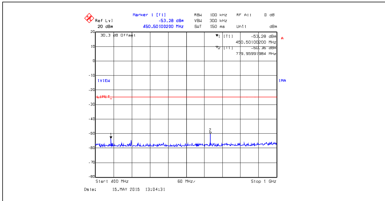
Plot 5.5.4.11. Conducted Transmitter Spurious Emissions, 390.0 MHz, Low Power, 400 MHz – 1 GHz
