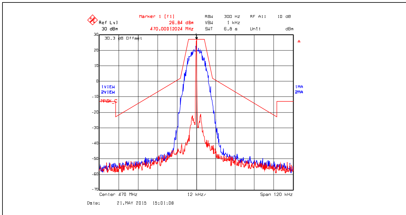
Plot 5.4.4.3.16. Emission Mask C, Digital at 19.2 kbps, 470.0 MHz, Low Power
