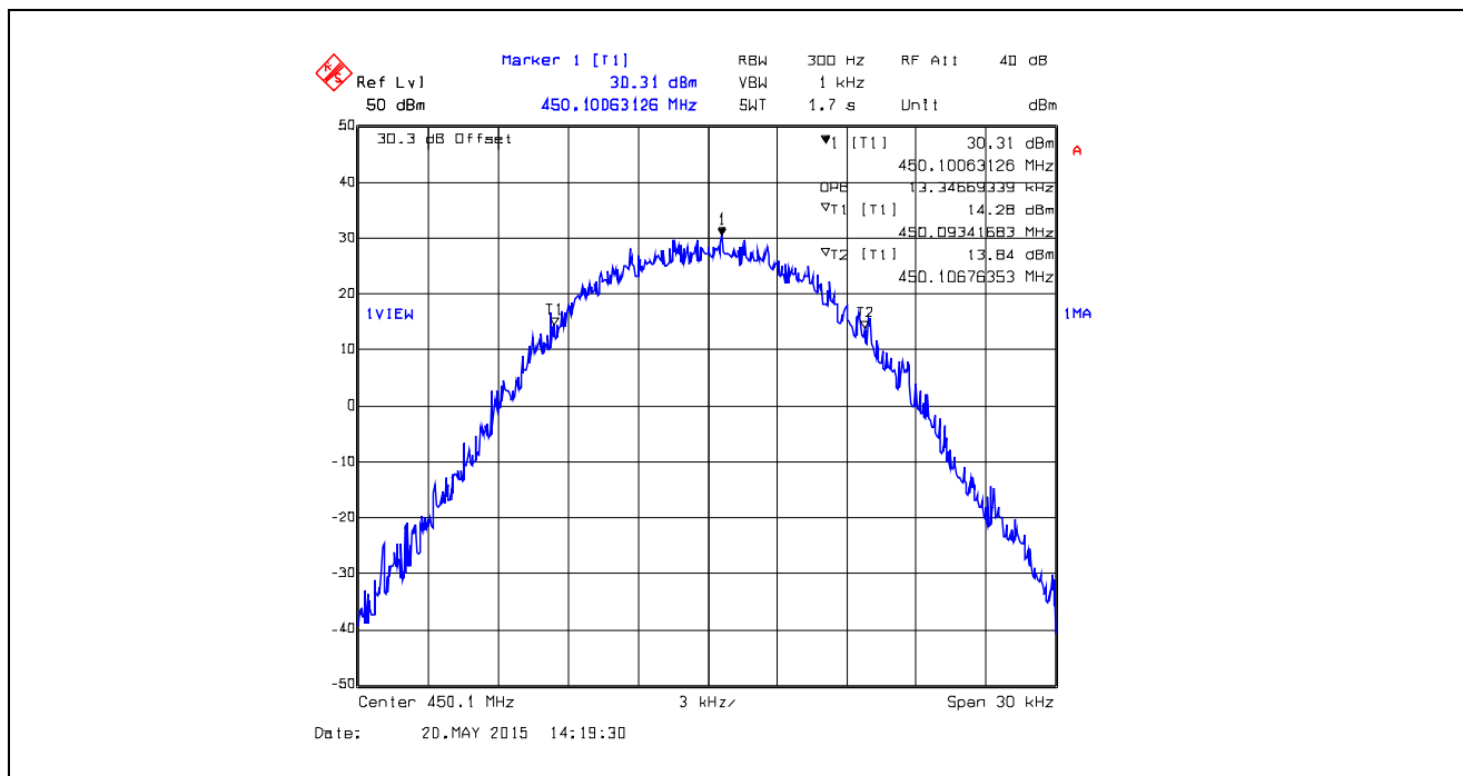
Plot 5.4.4.1.16. 99% Occupied Bandwidth, 25 kHz Channel Spacing, Digital 19.2 kbps, 450.1 MHz
