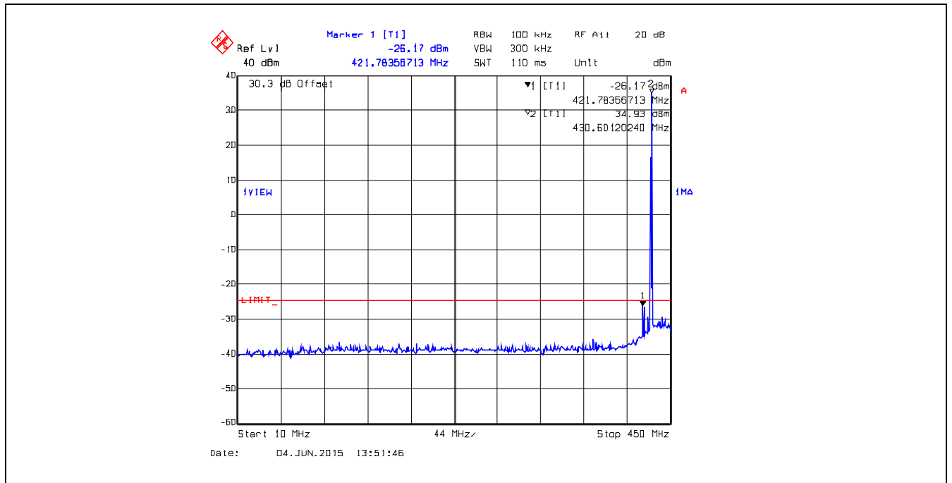
Plot 5.5.4.31. Conducted Transmitter Spurious Emissions, 429.9 MHz, High Power, 10 MHz – 450 MHz
