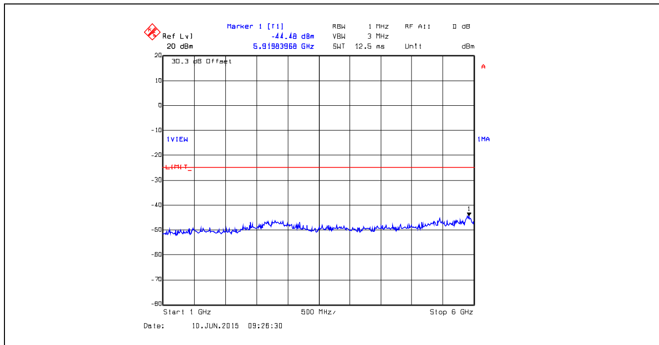
Plot 5.5.4.42. Conducted Transmitter Spurious Emissions, 450.1 MHz, Low Power, 1 GHz – 6 GHz
