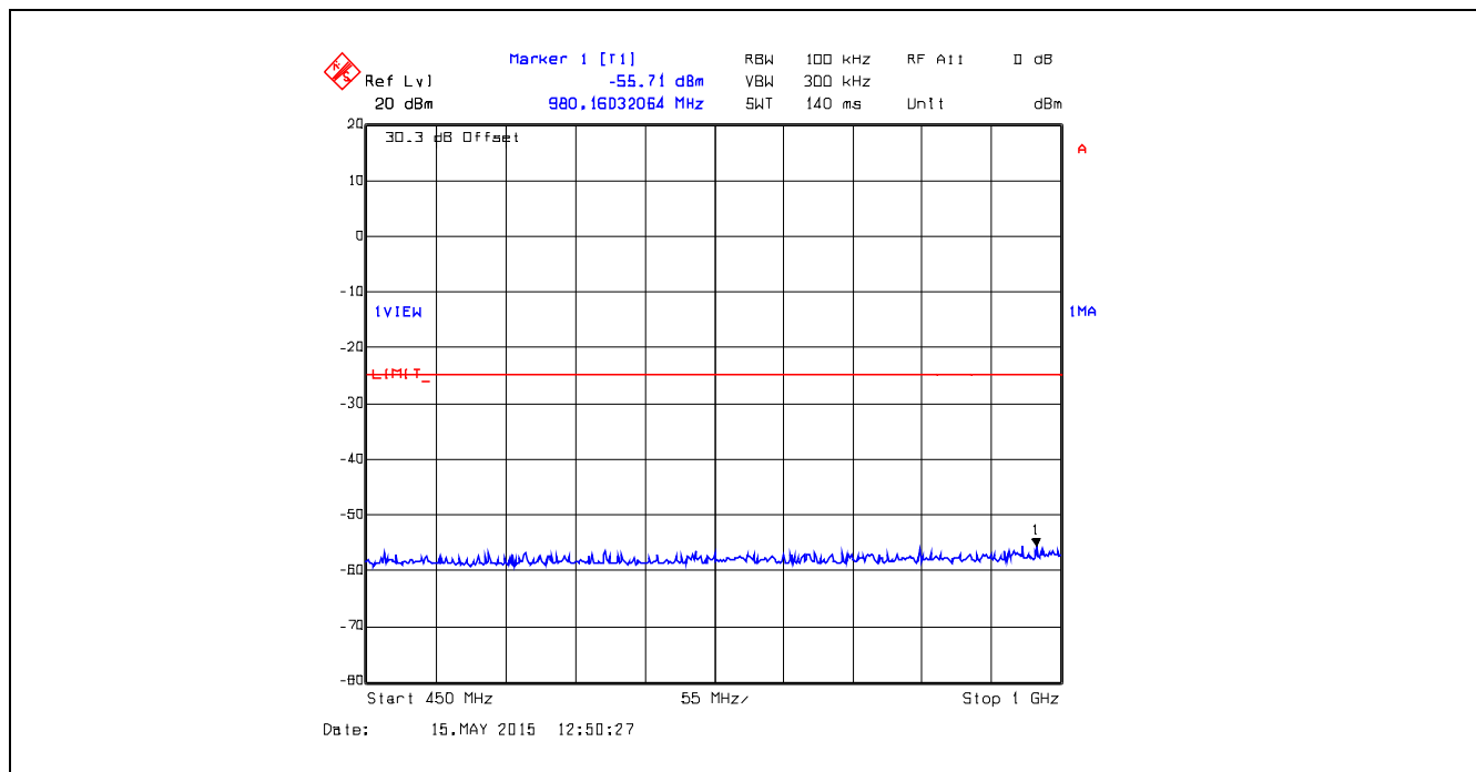
Plot 5.5.4.23. Conducted Transmitter Spurious Emissions, 406.2 MHz, Low Power, 450 MHz – 1 GHz
