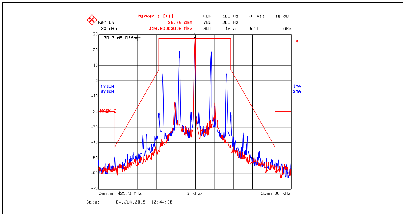
Plot 5.4.4.4.12. Emission Mask D, Analog, 429.9 MHz, Low Power
