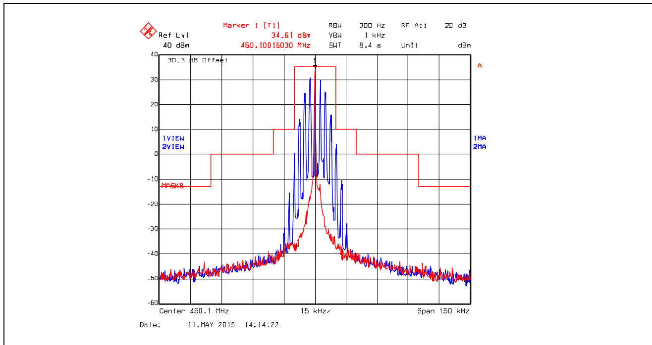
Plot 5.4.4.2.13. Emission Mask B, Analog, 450.1 MHz, High Power
