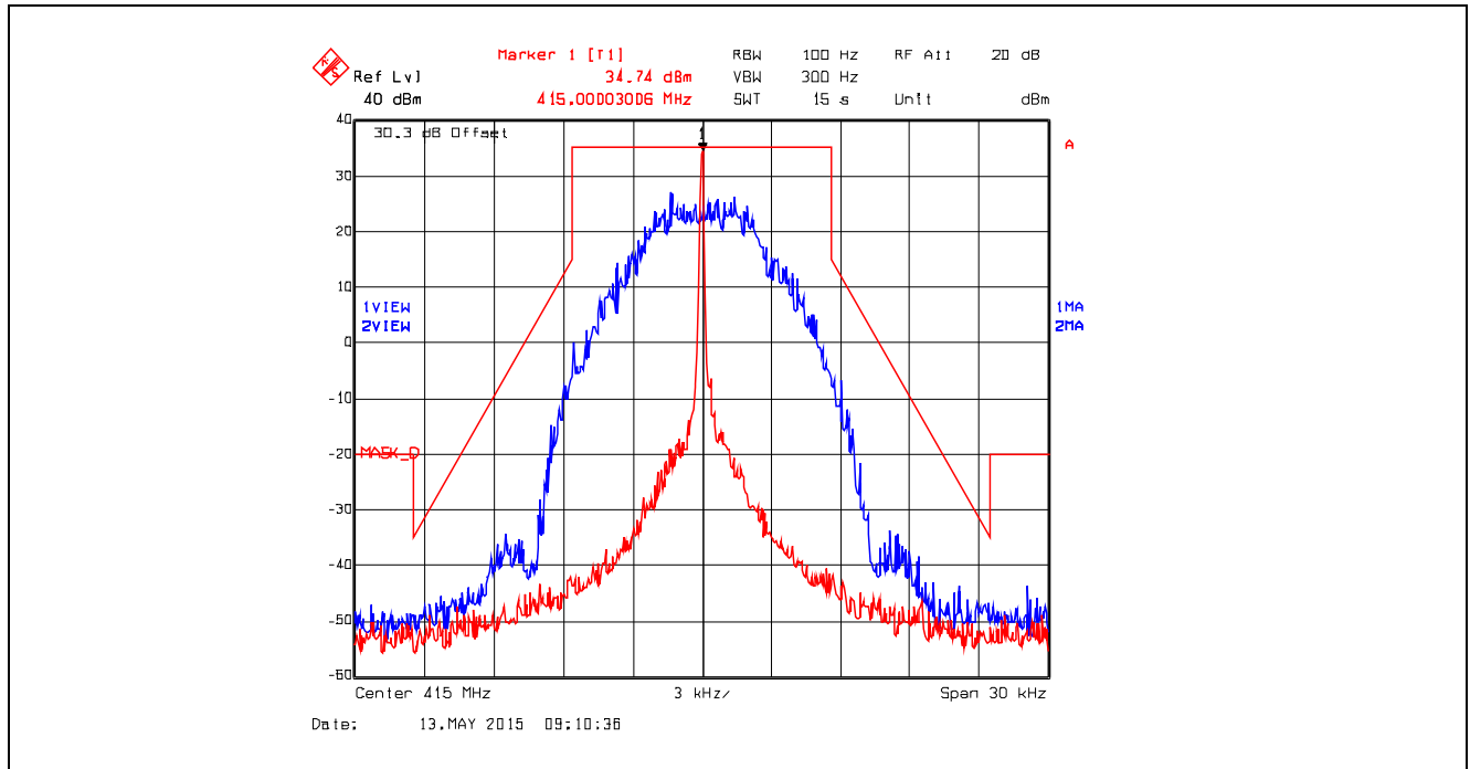
Plot 5.4.4.5.9. Emission Mask D, Digital at 9.6 kbps, 415.0 MHz, High Power
