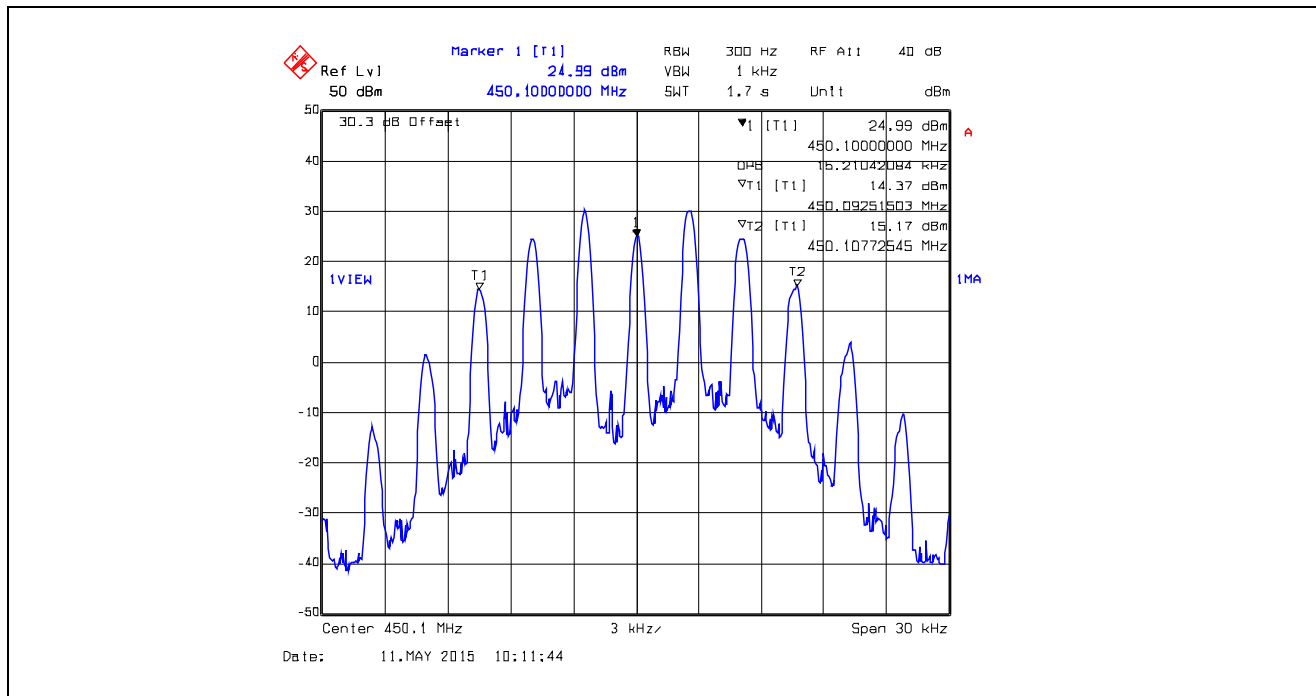
Plot 5.4.4.1.7. 99% Occupied Bandwidth, 25 kHz Channel Spacing, Analog, 450.1 MHz
