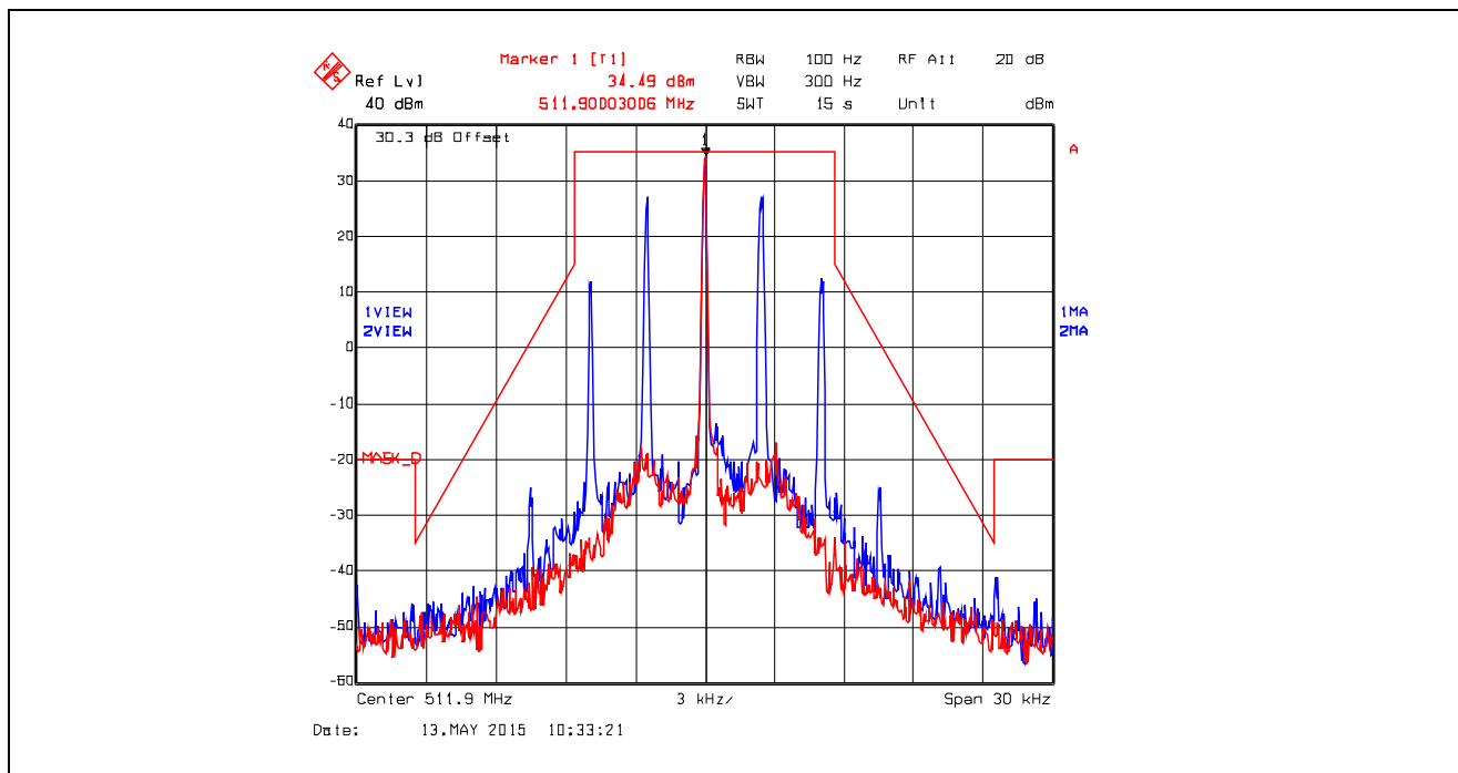
Plot 5.4.4.4.17. Emission Mask D, Analog, 511.9 MHz, High Power
