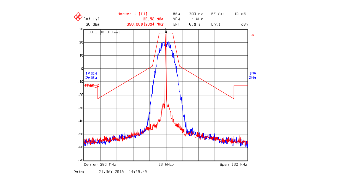
Plot 5.4.4.3.4. Emission Mask C, Digital at 19.2 kbps, 390.0 MHz, Low Power
