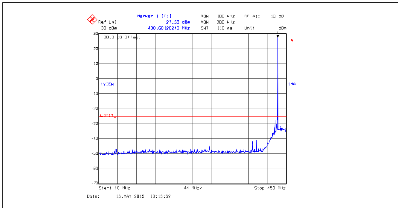
Plot 5.5.4.34. Conducted Transmitter Spurious Emissions, 429.9 MHz, Low Power, 10 MHz – 450 MHz
