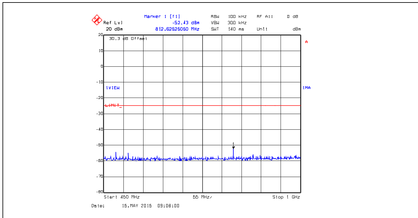
Plot 5.5.4.20. Conducted Transmitter Spurious Emissions, 406.2 MHz, High Power, 450 MHz – 1 GHz
