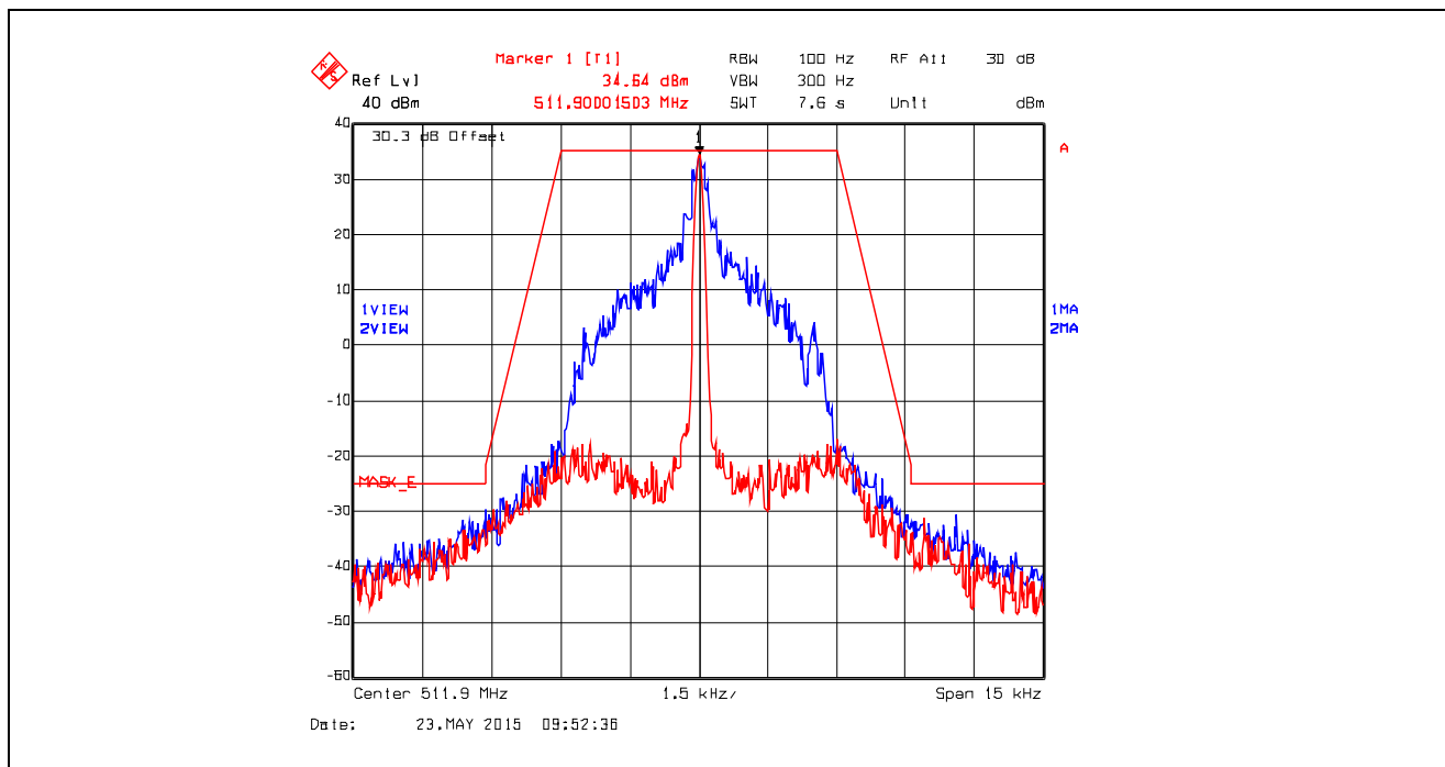
Plot 5.4.4.6.17. Emission Mask E, Digital at 4.8 kbps, 511.9 MHz, High Power
