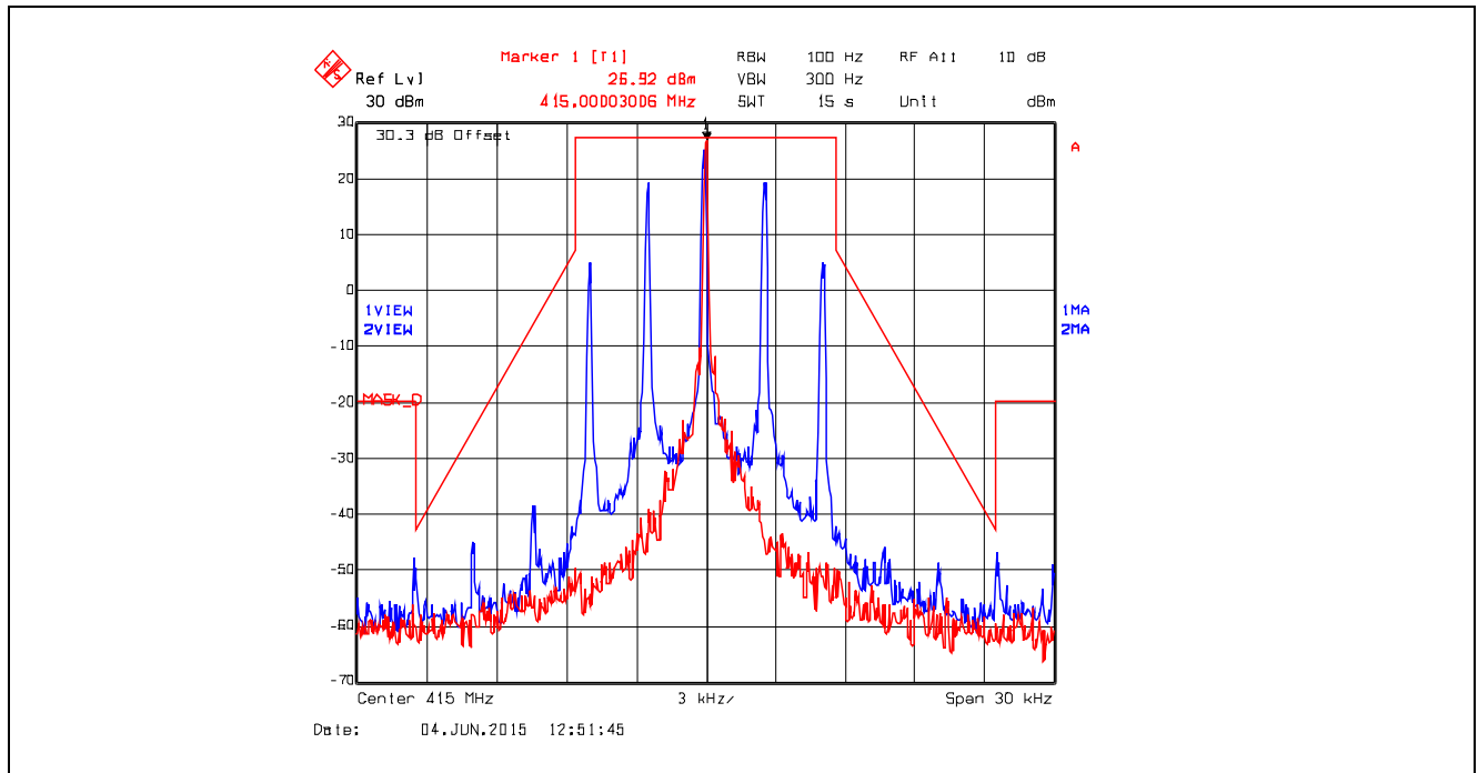
Plot 5.4.4.4.10. Emission Mask D, Analog, 415.0 MHz, Low Power
