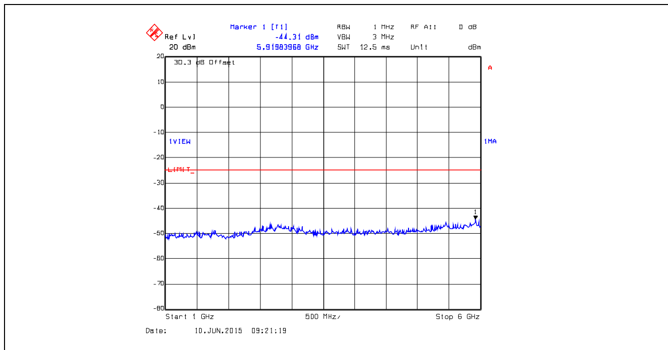
Plot 5.5.4.39. Conducted Transmitter Spurious Emissions, 450.1 MHz, High Power, 1 GHz – 6 GHz
