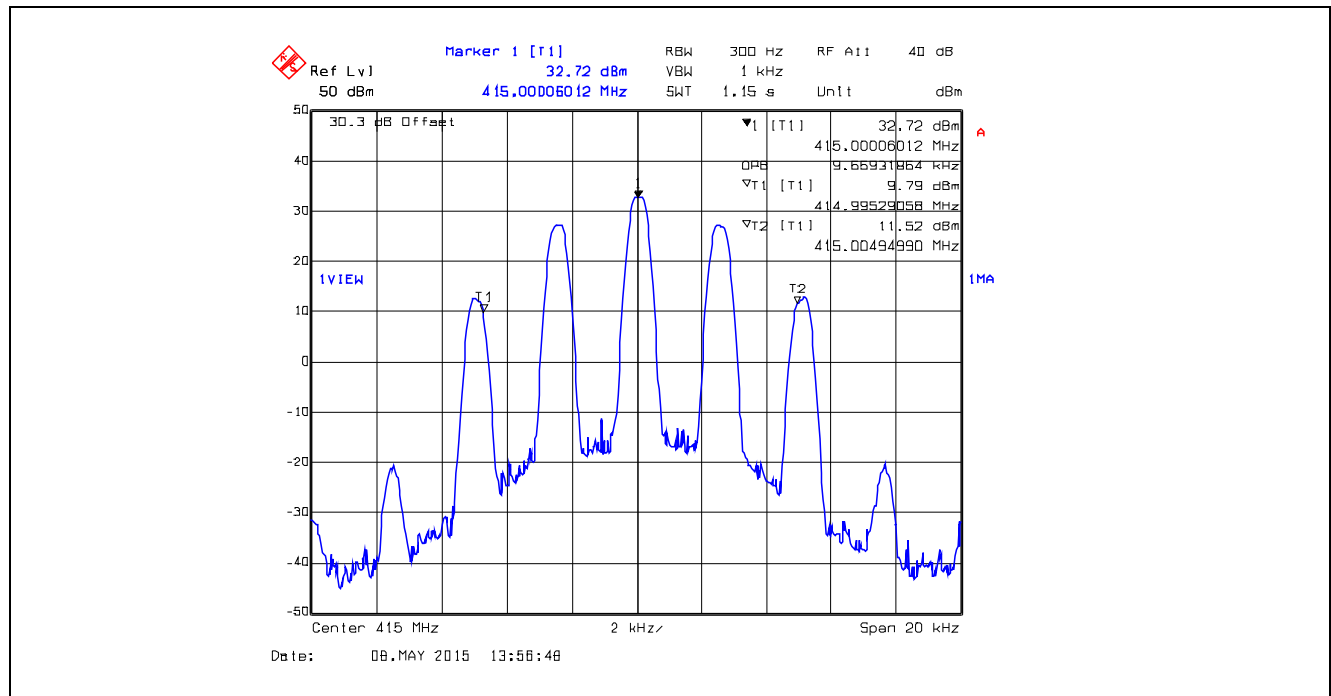
Plot 5.4.4.1.23. 99% Occupied Bandwidth, 12.5 kHz Channel Spacing, Analog, 415.0 MHz
