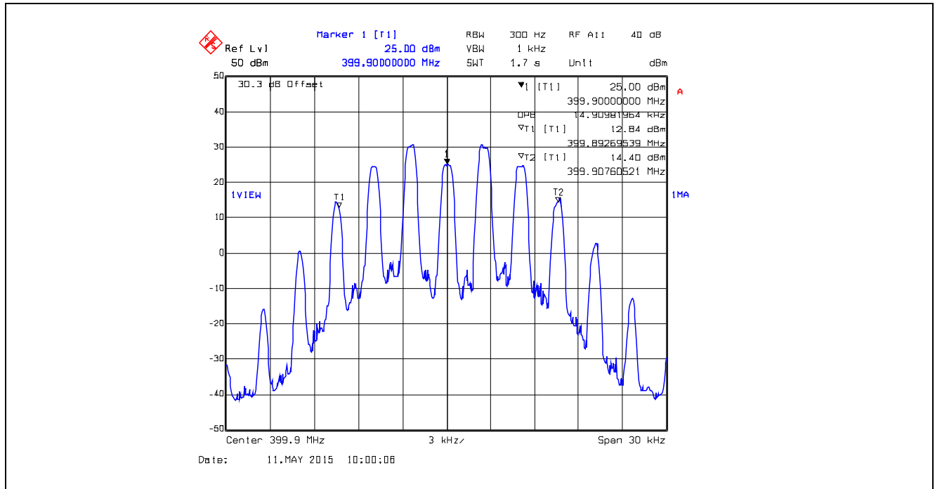
Plot 5.4.4.1.3. 99% Occupied Bandwidth, 25 kHz Channel Spacing, Analog, 399.9 MHz
