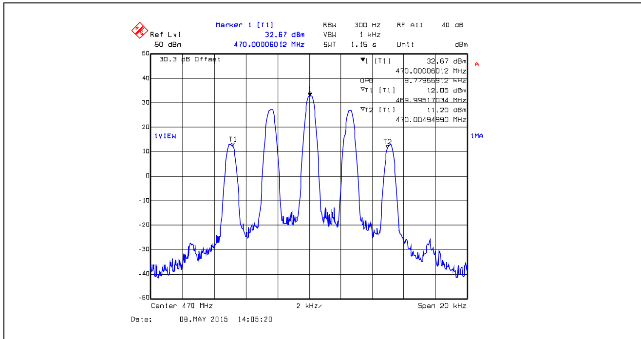
Plot 5.4.4.1.26. 99% Occupied Bandwidth, 12.5 kHz Channel Spacing, Analog, 470.0 MHz
