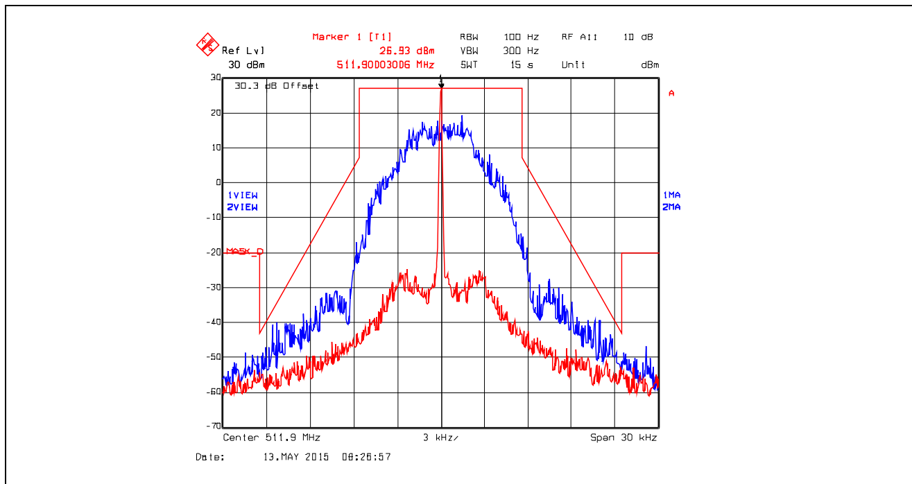
Plot 5.4.4.5.18. Emission Mask D, Digital at 9.6 kbps, 511.9 MHz, Low Power
