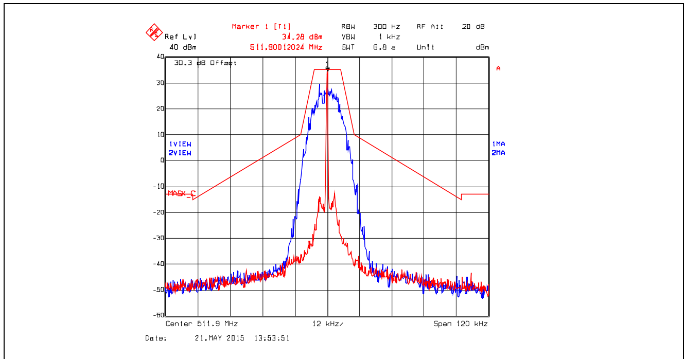
Plot 5.4.4.3.17. Emission Mask C, Digital at 19.2 kbps, 511.9 MHz, High Power
