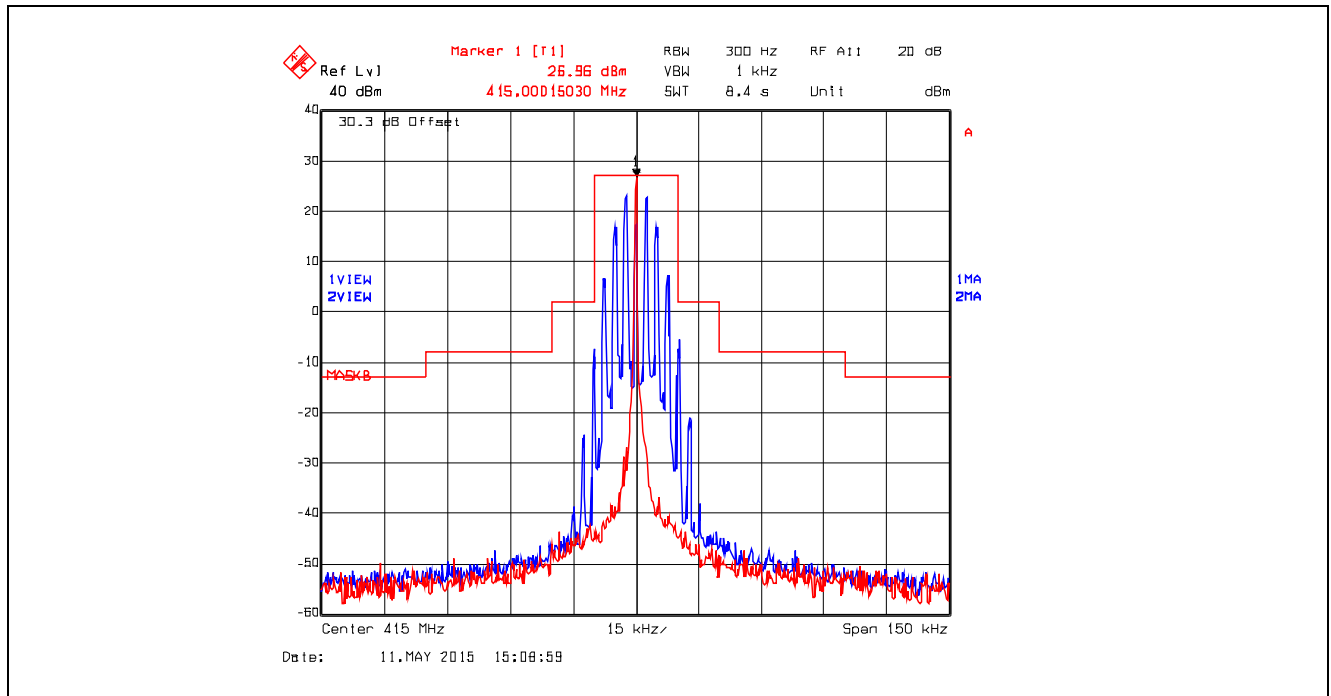
Plot 5.4.4.2.10. Emission Mask B, Analog, 415.0 MHz, Low Power
