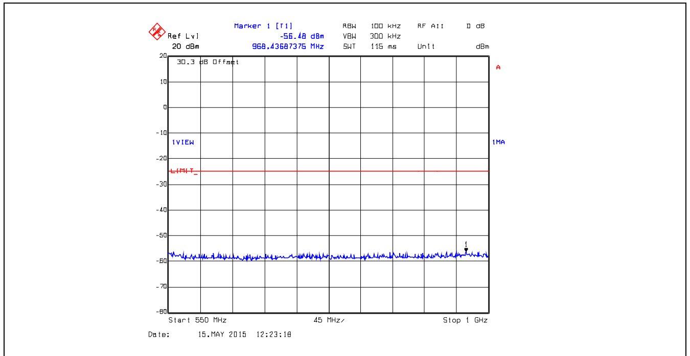
Plot 5.5.4.47. Conducted Transmitter Spurious Emissions, 470.0 MHz, Low Power, 550 MHz – 1 GHz
