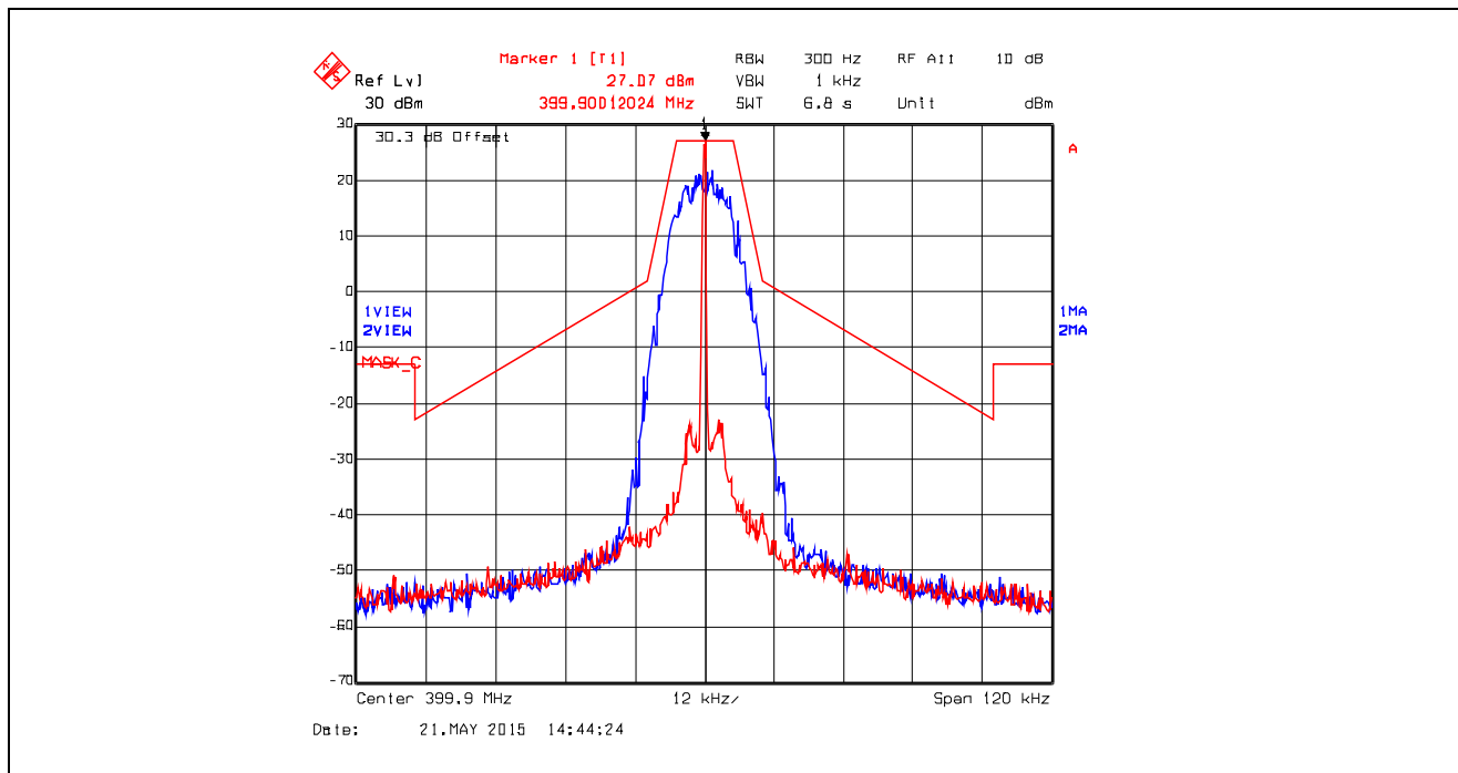
Plot 5.4.4.3.6. Emission Mask C, Digital at 19.2 kbps, 399.9 MHz, Low Power
