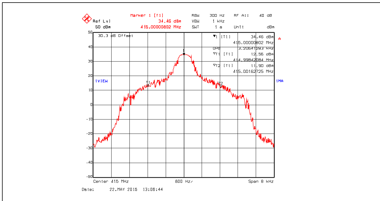
Plot 5.4.4.1.41. 99% Occupied Bandwidth, 6.25 kHz Channel Spacing, Digital 4.8 kbps, 415.0 MHz
