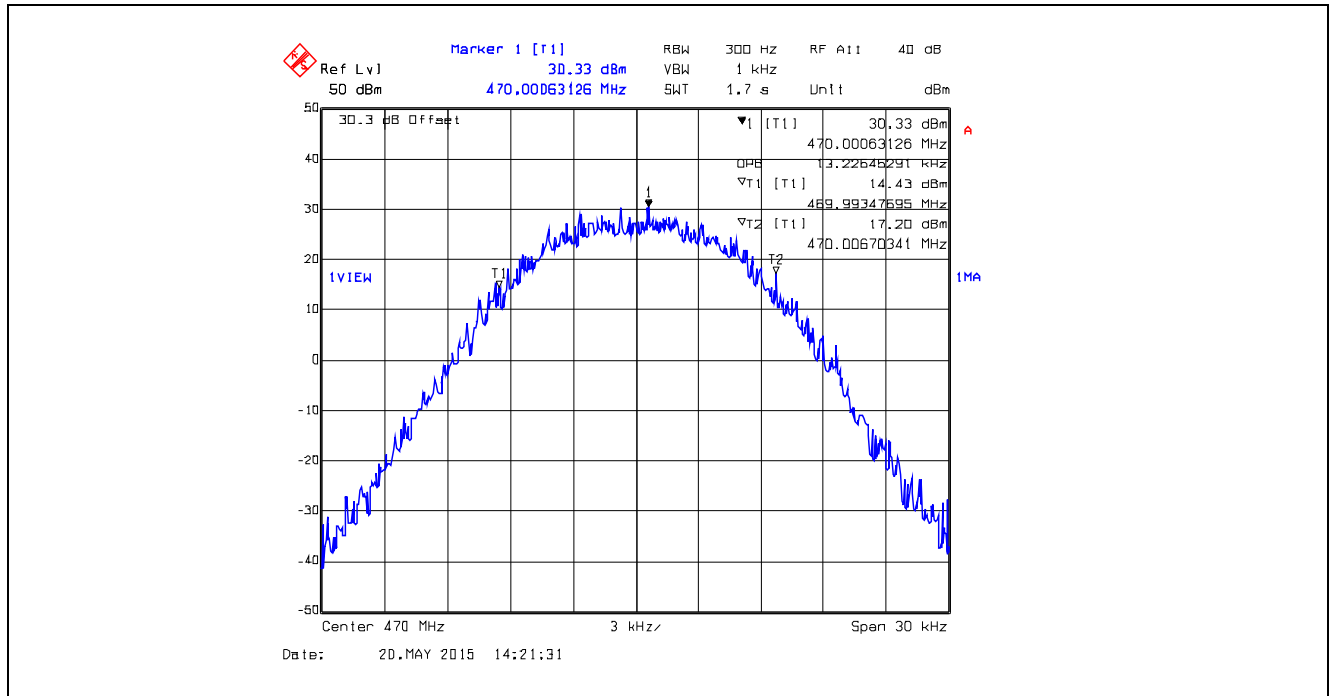
Plot 5.4.4.1.17. 99% Occupied Bandwidth, 25 kHz Channel Spacing, Digital 19.2 kbps, 470.0 MHz
