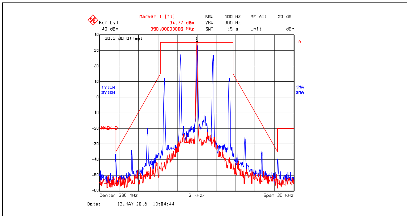
Plot 5.4.4.4.3. Emission Mask D, Analog, 390.0 MHz, High Power
