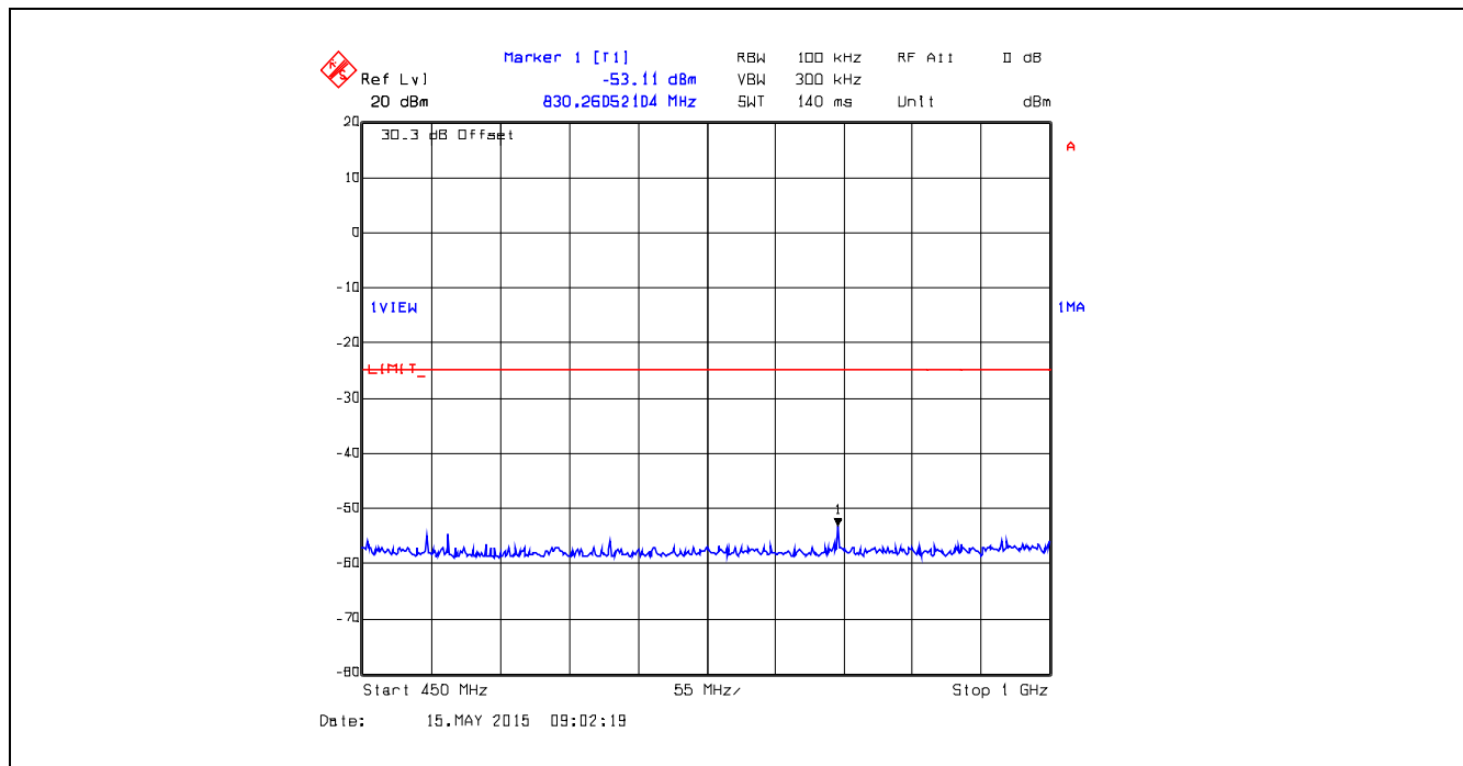
Plot 5.5.4.26. Conducted Transmitter Spurious Emissions, 415.0 MHz, High Power, 450 MHz – 1 GHz
