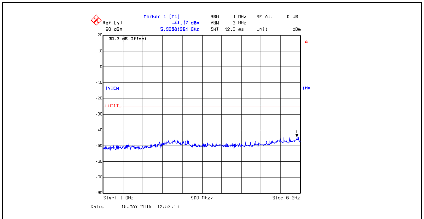
Plot 5.5.4.18. Conducted Transmitter Spurious Emissions, 399.9 MHz, Low Power, 1 GHz – 6 GHz
