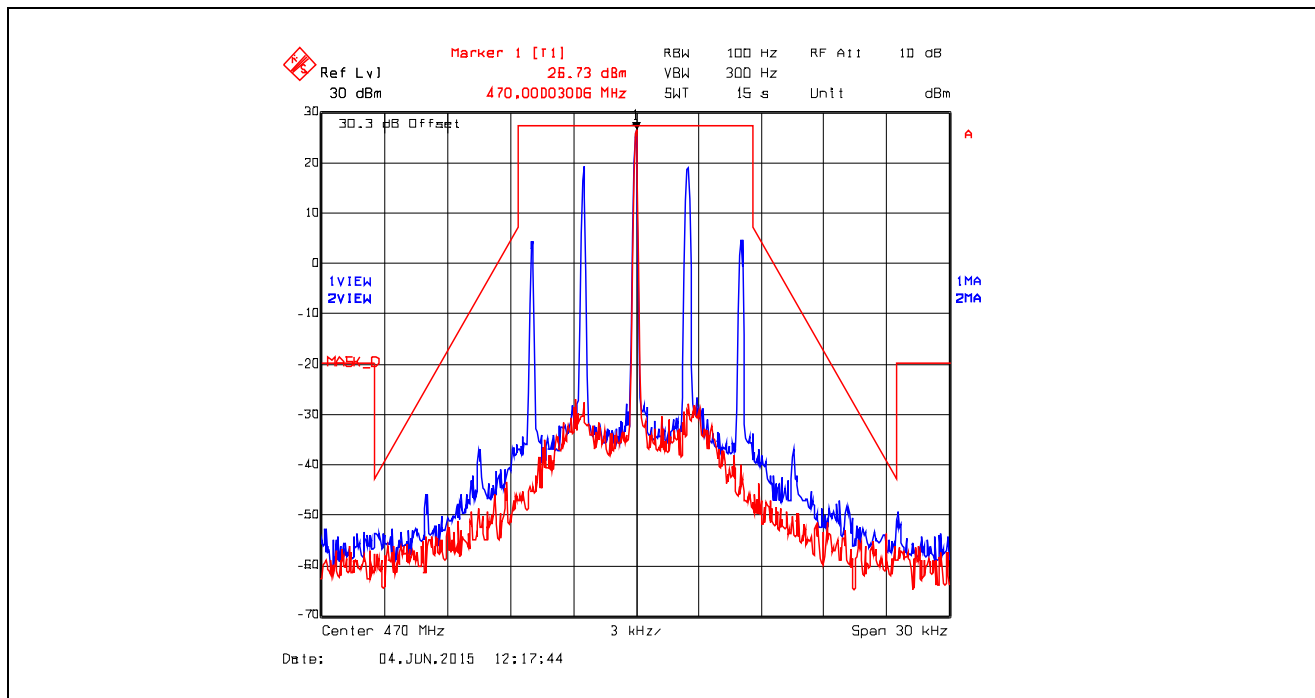
Plot 5.4.4.4.16. Emission Mask D, Analog, 470.0 MHz, Low Power
