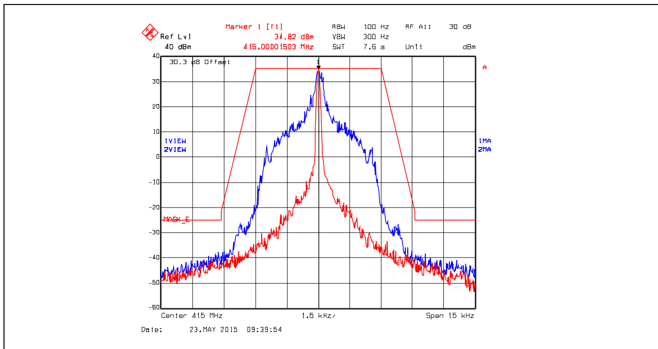
Plot 5.4.4.6.9. Emission Mask E, Digital at 4.8 kbps, 415.0 MHz, High Power
