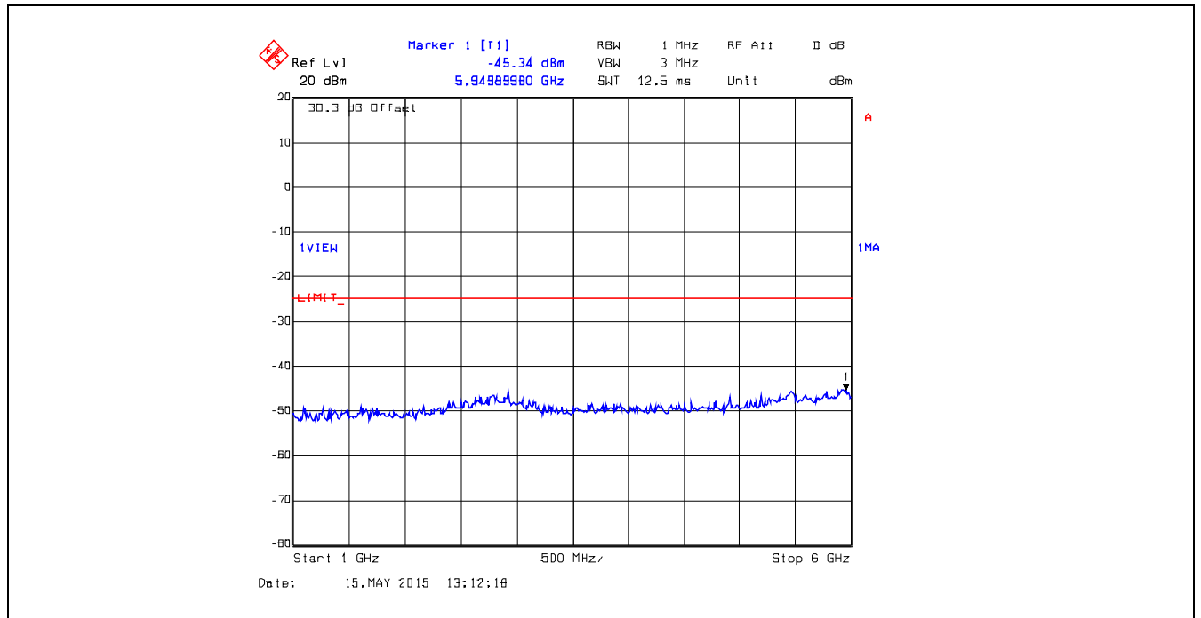
Plot 5.5.4.6. Conducted Transmitter Spurious Emissions, 380.1 MHz, Low Power, 1 GHz – 6 GHz
