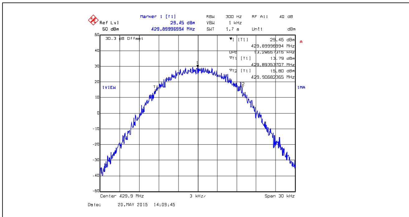
Plot 5.4.4.1.15. 99% Occupied Bandwidth, 25 kHz Channel Spacing, Digital 19.2 kbps, 429.9 MHz
