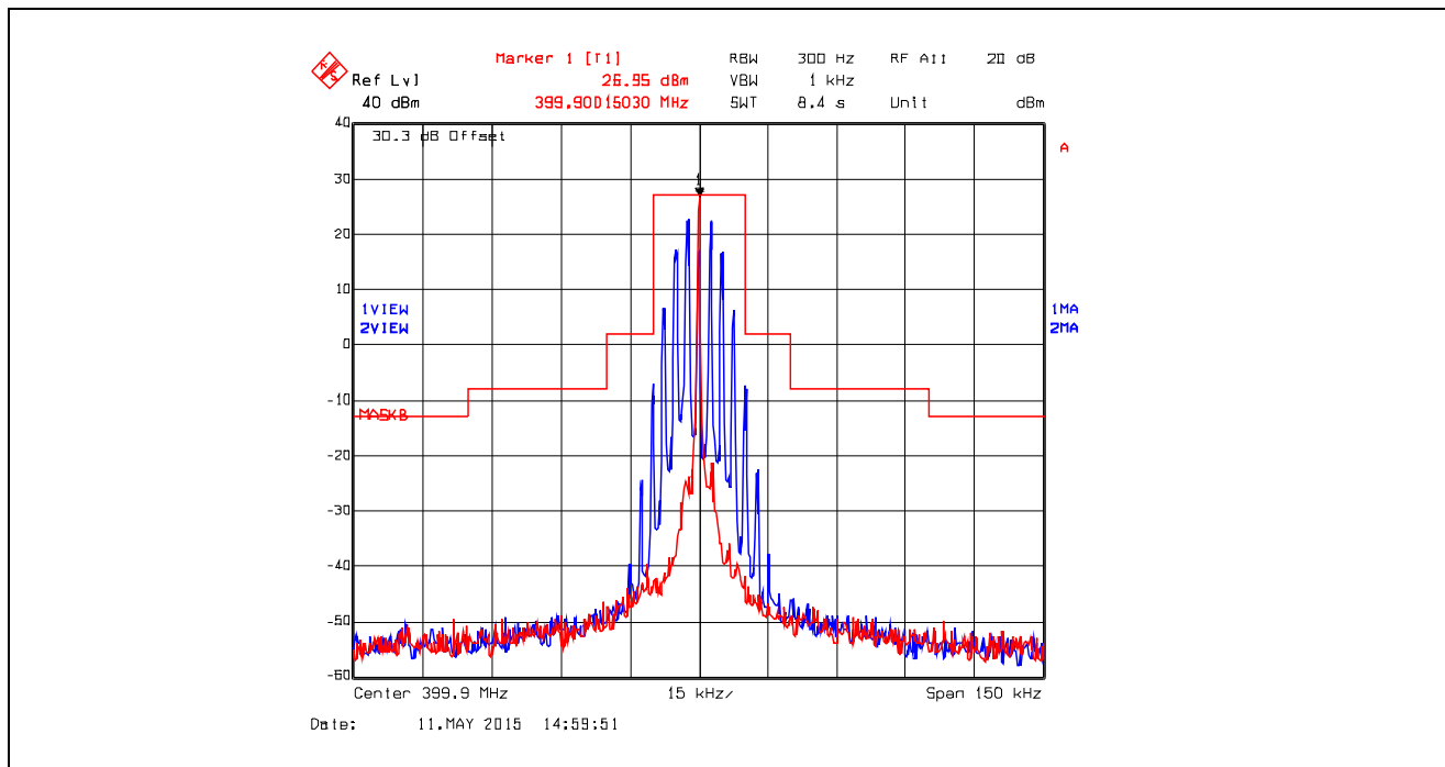
Plot 5.4.4.2.6. Emission Mask B, Analog, 399.9 MHz, Low Power
