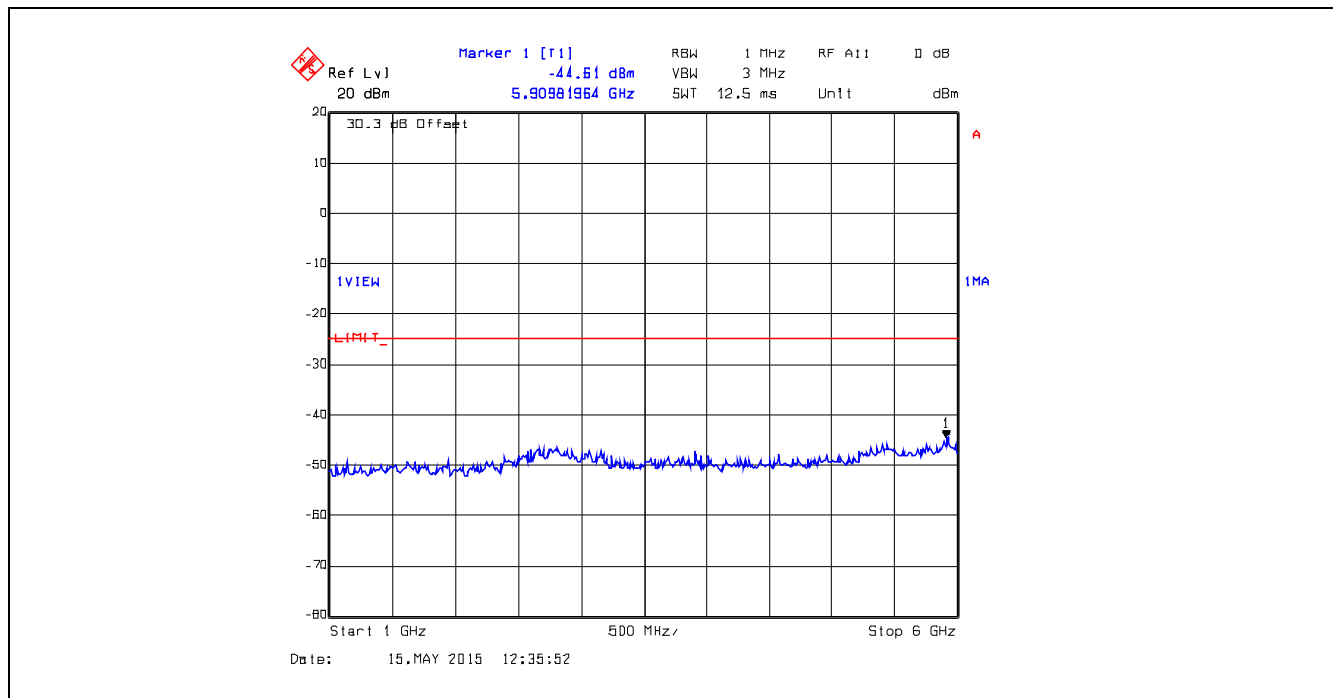
Plot 5.5.4.36. Conducted Transmitter Spurious Emissions, 429.9 MHz, Low Power, 1 GHz – 6 GHz
