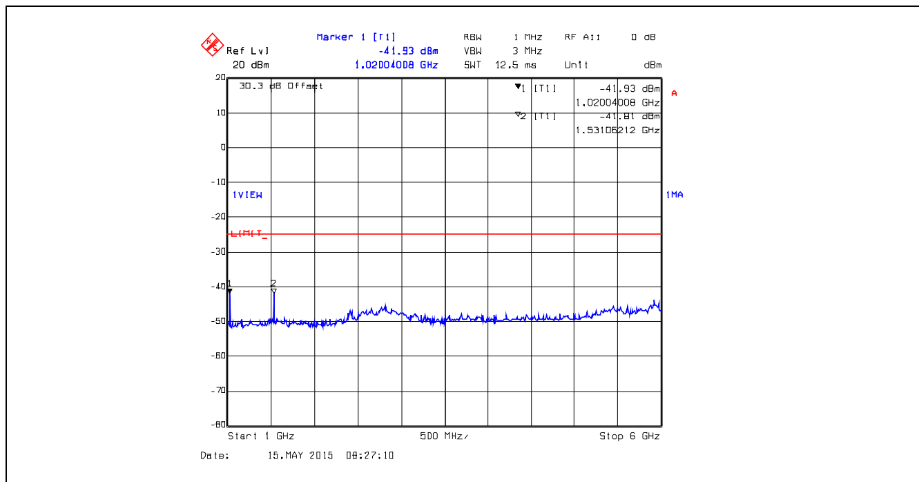
Plot 5.5.4.51. Conducted Transmitter Spurious Emissions, 511.9 MHz, High Power, 1 GHz – 6 GHz
