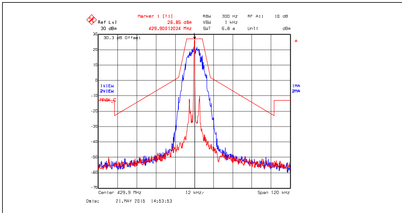
Plot 5.4.4.3.12. Emission Mask C, Digital at 19.2 kbps, 429.9 MHz, Low Power
