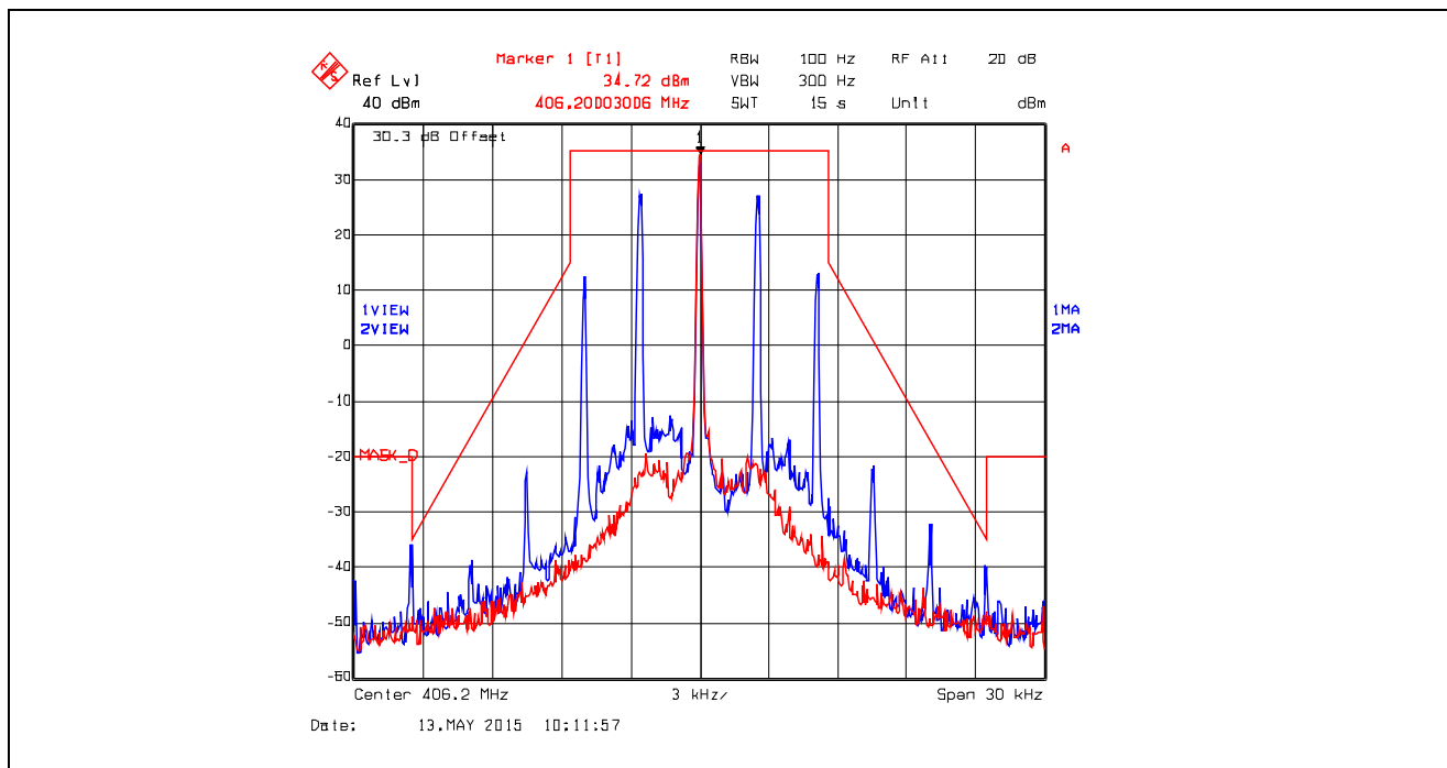
Plot 5.4.4.4.7. Emission Mask D, Analog, 406.2 MHz, High Power
