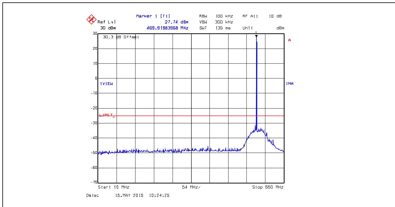
Plot 5.5.4.46. Conducted Transmitter Spurious Emissions, 470.0 MHz, Low Power, 10 MHz – 550 MHz
