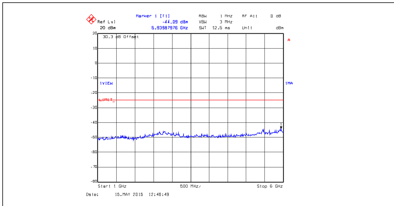
Plot 5.5.4.24. Conducted Transmitter Spurious Emissions, 406.2 MHz, Low Power, 1 GHz – 6 GHz
