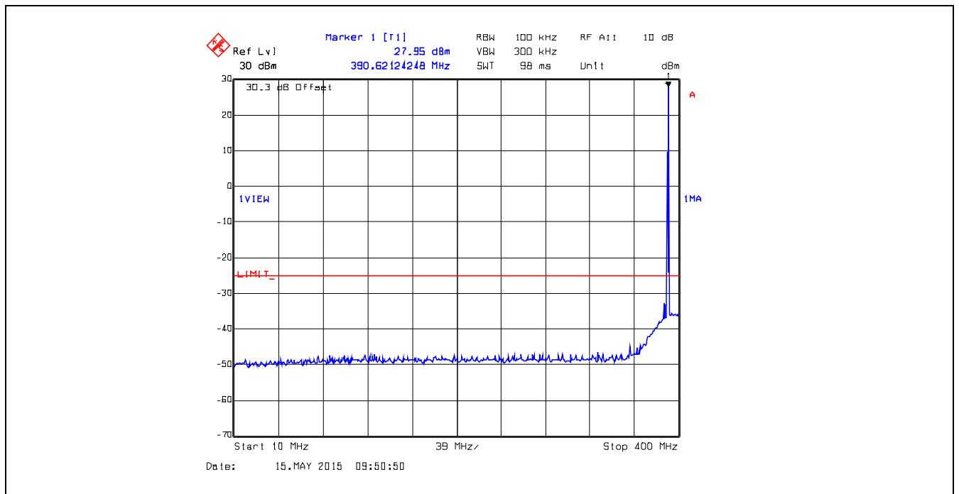
Plot 5.5.4.10. Conducted Transmitter Spurious Emissions, 390.0 MHz, Low Power, 10 MHz – 400 MHz
