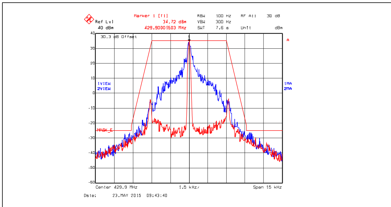
Plot 5.4.4.6.11. Emission Mask E, Digital at 4.8 kbps, 429.9 MHz, High Power
