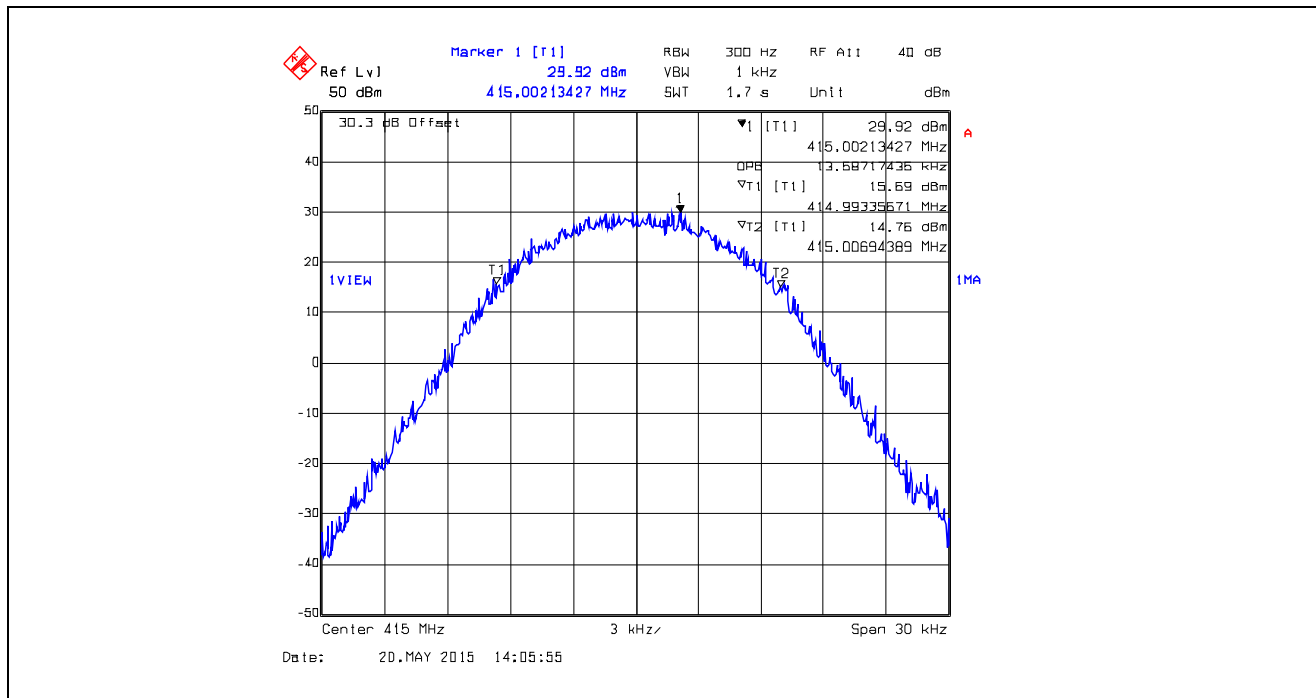
Plot 5.4.4.1.14. 99% Occupied Bandwidth, 25 kHz Channel Spacing, Digital 19.2 kbps, 415.0 MHz
