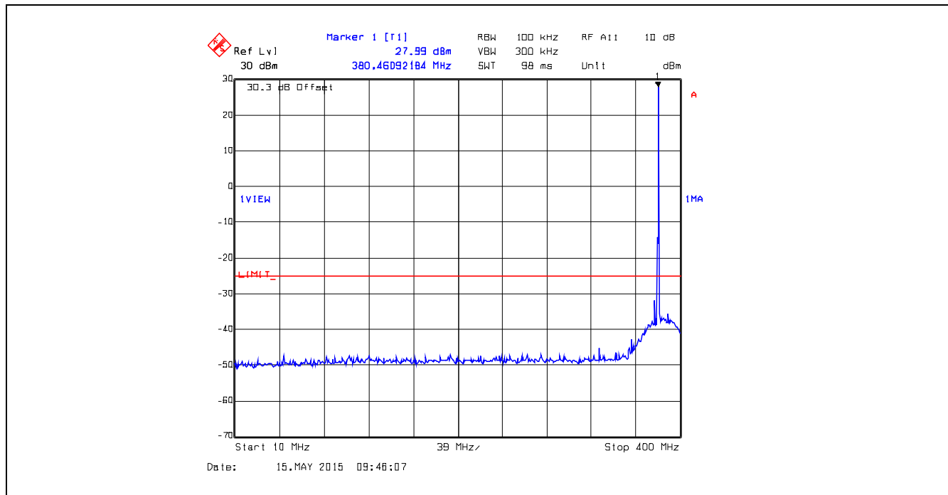
Plot 5.5.4.4. Conducted Transmitter Spurious Emissions, 380.1 MHz, Low Power, 10 MHz – 400 MHz
