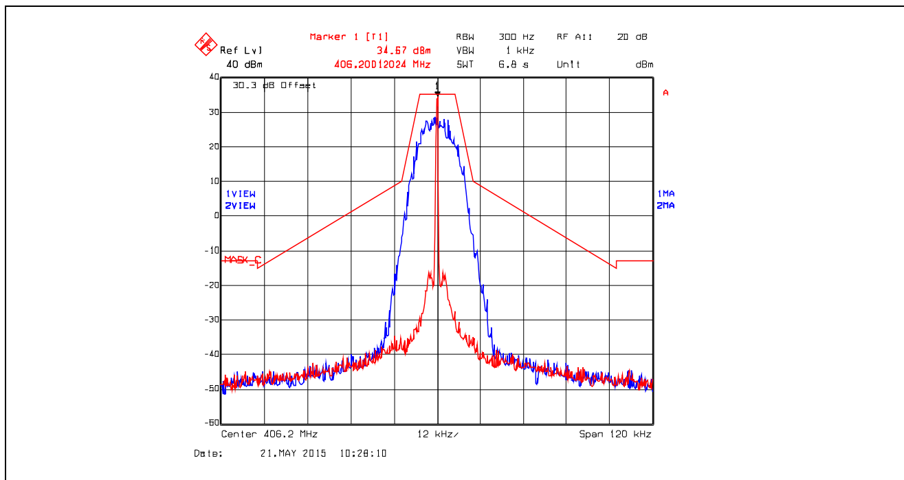
Plot 5.4.4.3.7. Emission Mask C, Digital at 19.2 kbps, 406.2 MHz, High Power
