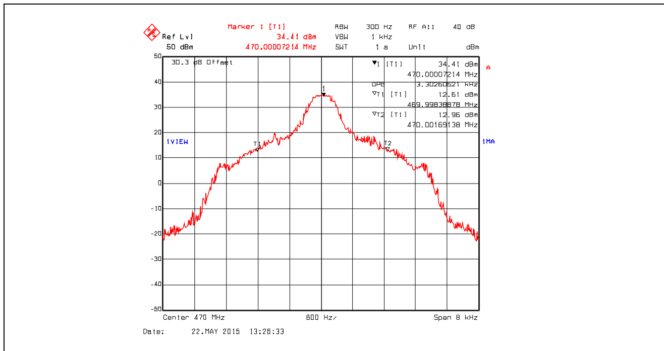
Plot 5.4.4.1.44. 99% Occupied Bandwidth, 6.25 kHz Channel Spacing, Digital 4.8 kbps, 470.0 MHz
