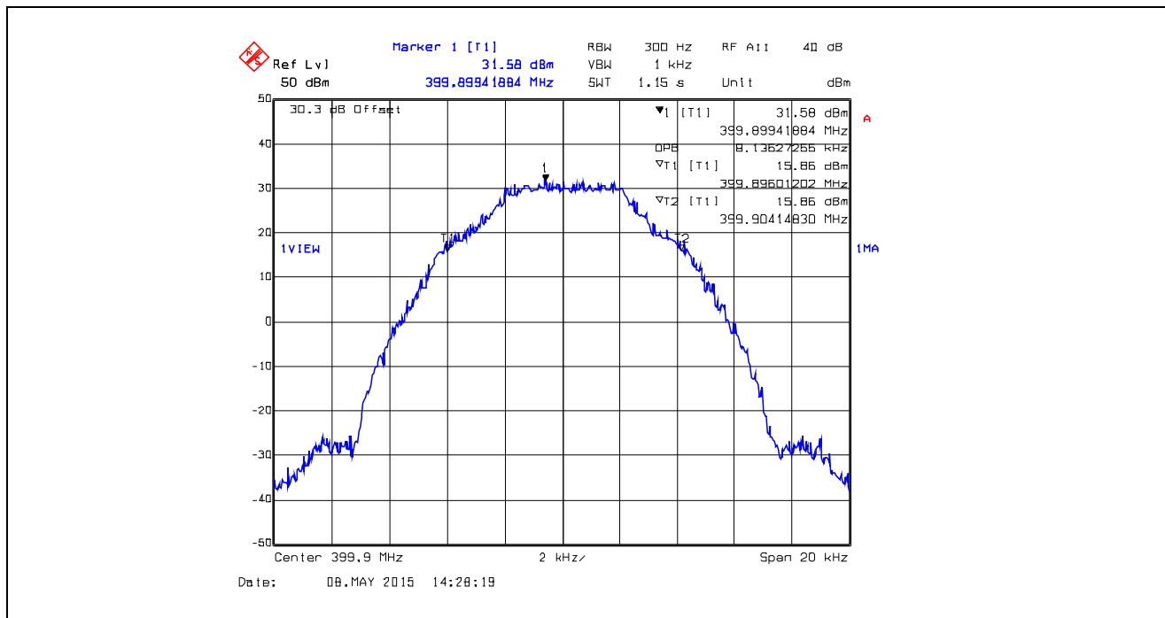
Plot 5.4.4.1.30. 99% Occupied Bandwidth, 12.5 kHz Channel Spacing, Digital 9.6 kbps, 399.9 MHz
