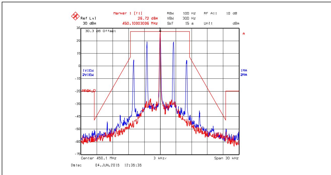
Plot 5.4.4.4.14. Emission Mask D, Analog, 450.1 MHz, Low Power
