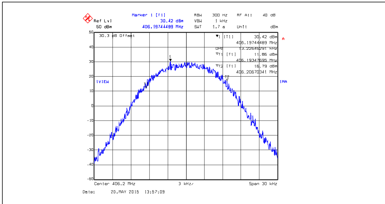
Plot 5.4.4.1.13. 99% Occupied Bandwidth, 25 kHz Channel Spacing, Digital 19.2 kbps, 406.2 MHz
