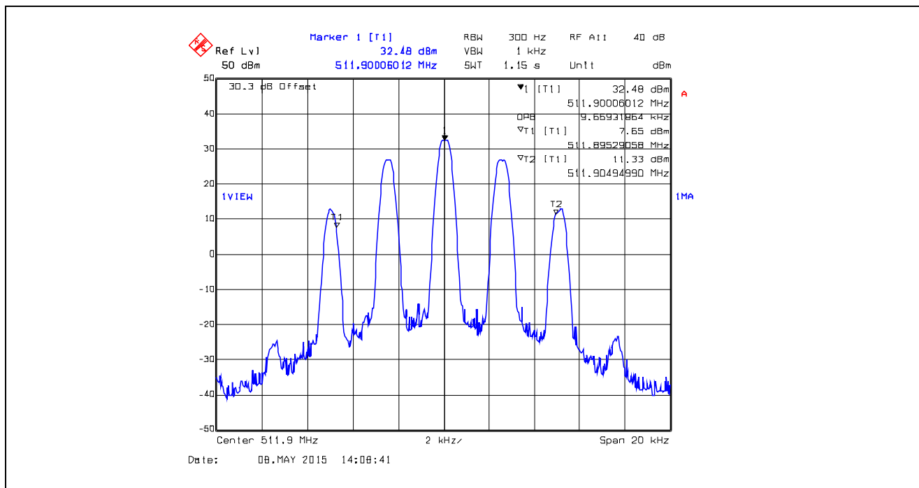
Plot 5.4.4.1.27. 99% Occupied Bandwidth, 12.5 kHz Channel Spacing, Analog, 511.9 MHz
