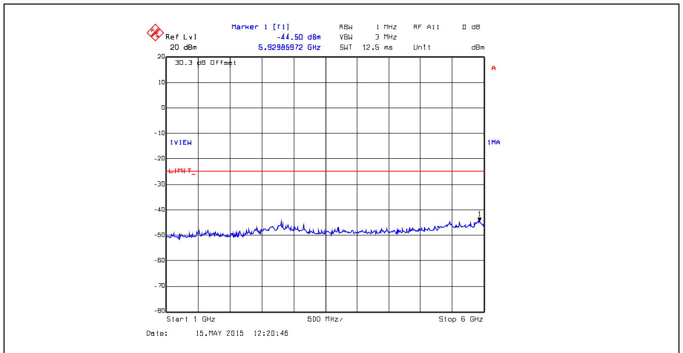
Plot 5.5.4.48. Conducted Transmitter Spurious Emissions, 470.0 MHz, Low Power, 1 GHz – 6 GHz
