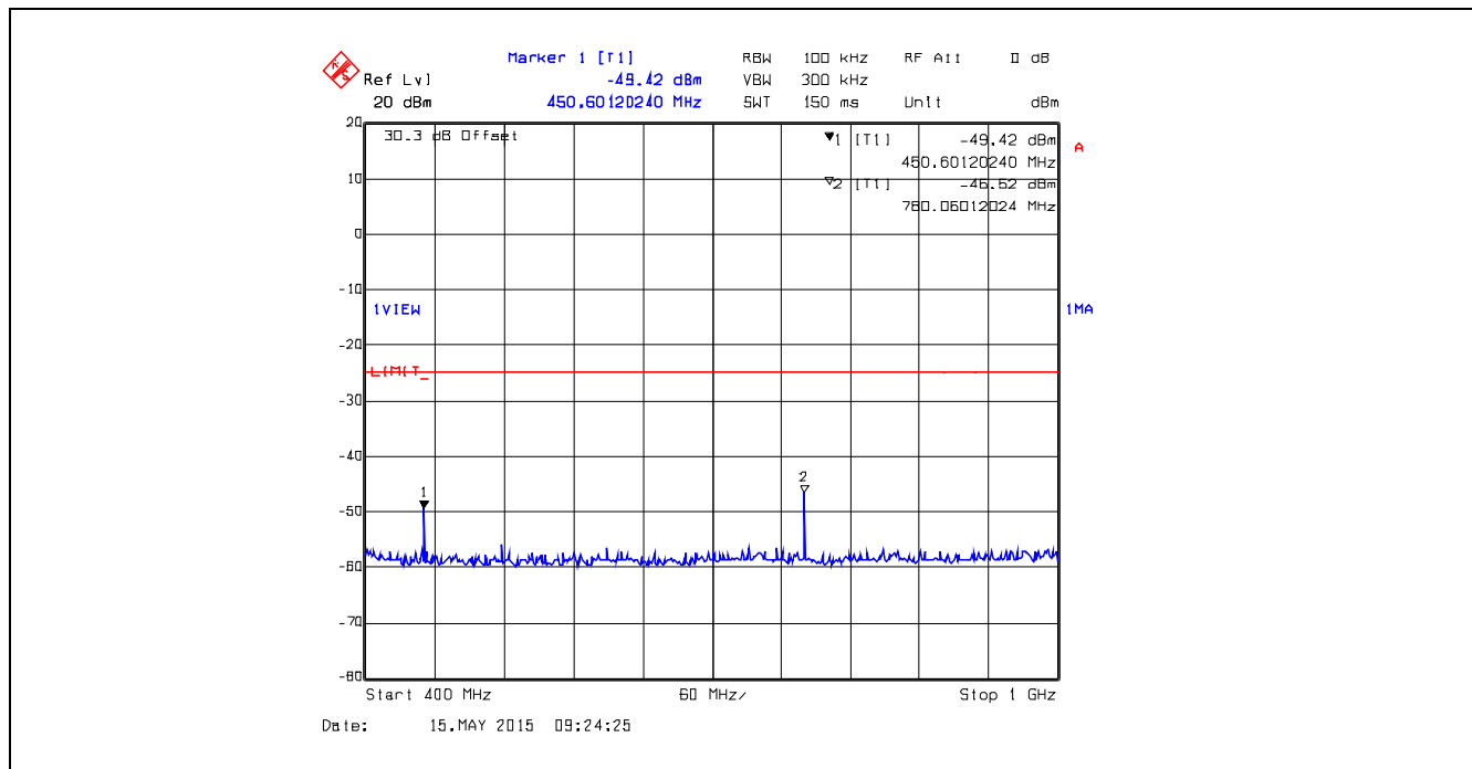
Plot 5.5.4.8. Conducted Transmitter Spurious Emissions, 390.0 MHz, High Power, 400 MHz – 1 GHz
