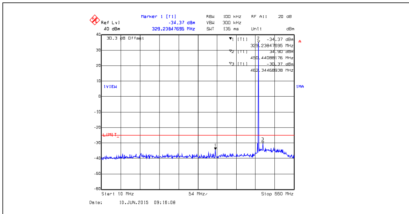
Plot 5.5.4.37. Conducted Transmitter Spurious Emissions, 450.1 MHz, High Power, 10 MHz – 550 MHz
