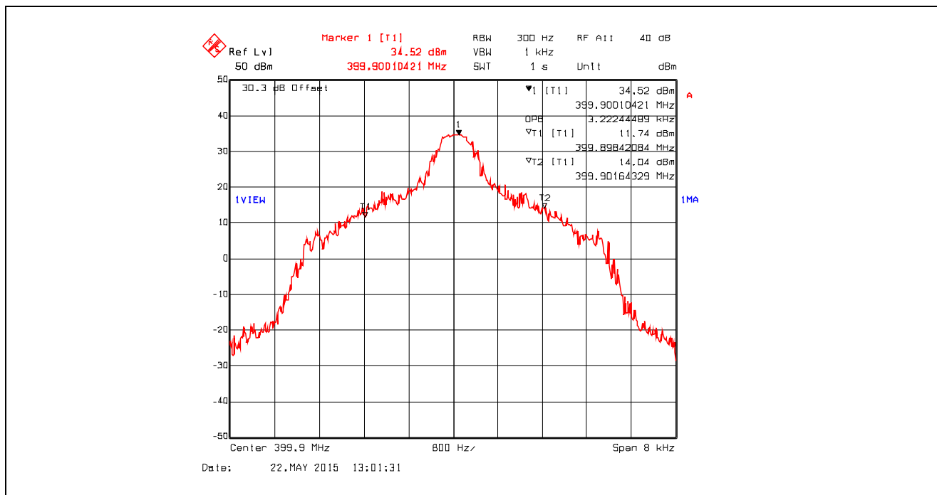
Plot 5.4.4.1.39. 99% Occupied Bandwidth, 6.25 kHz Channel Spacing, Digital 4.8 kbps, 399.9 MHz
