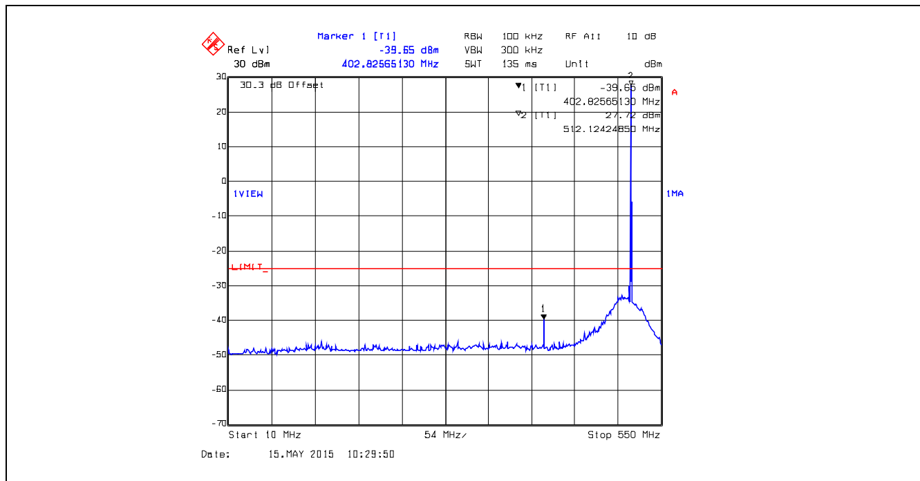
Plot 5.5.4.52. Conducted Transmitter Spurious Emissions, 511.9 MHz, Low Power, 10 MHz – 550 MHz
