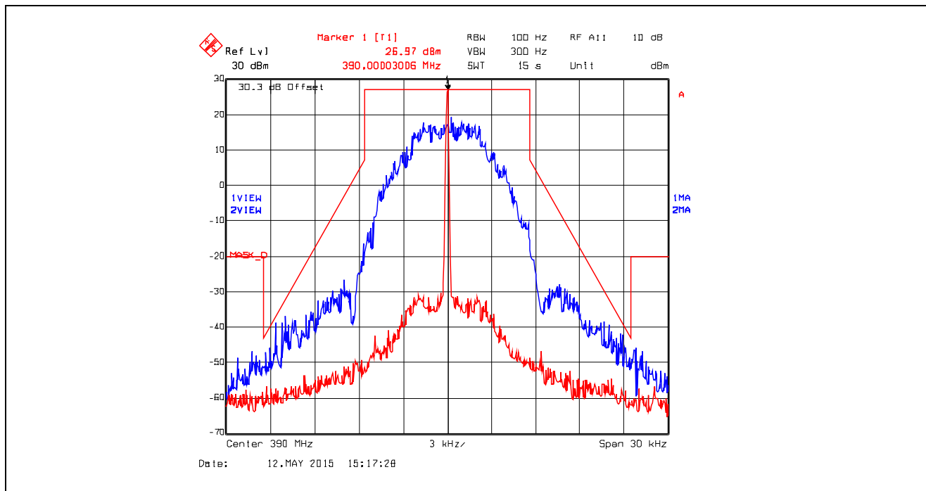
Plot 5.4.4.5.4. Emission Mask D, Digital at 9.6 kbps, 390.0 MHz, Low Power
