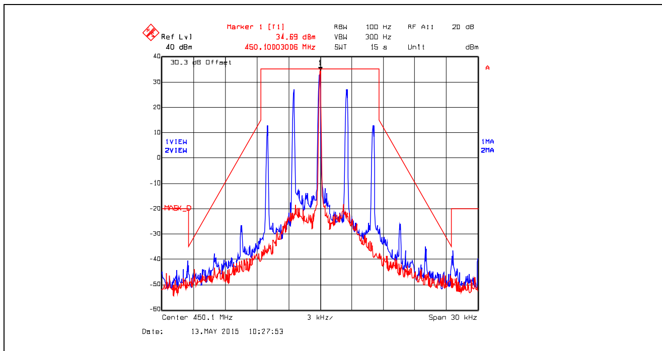
Plot 5.4.4.4.13. Emission Mask D, Analog, 450.1 MHz, High Power
