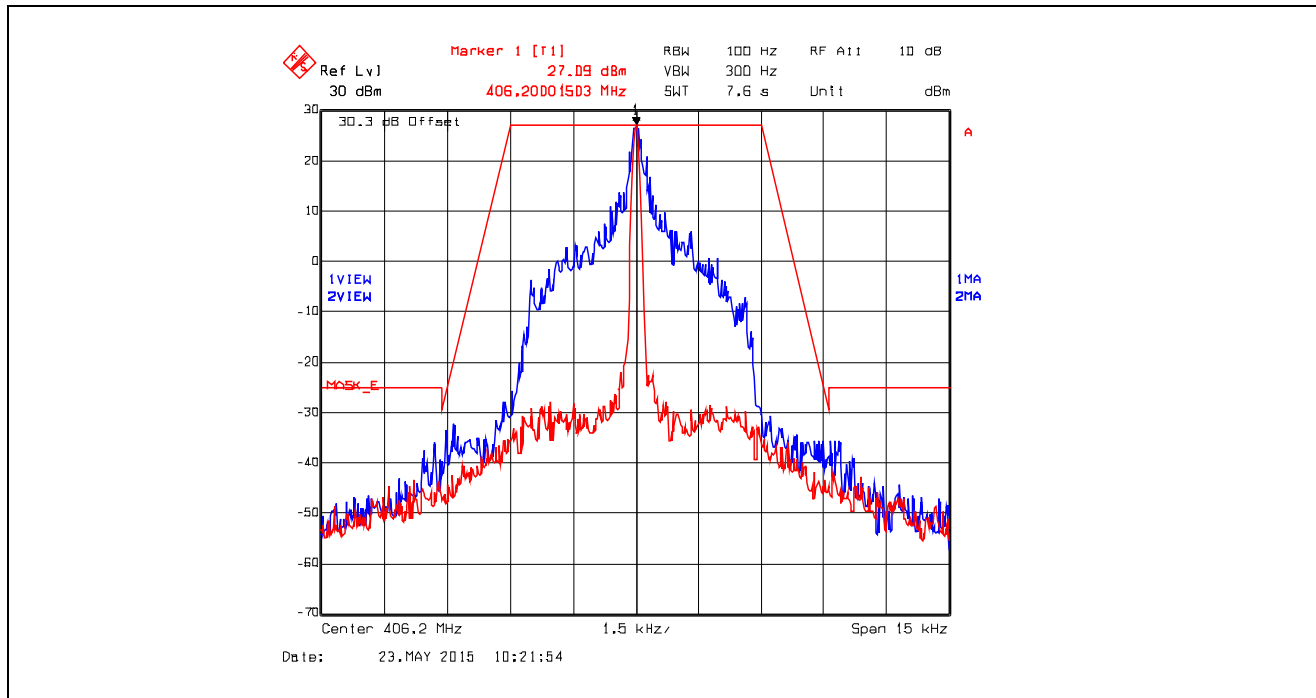
Plot 5.4.4.6.8. Emission Mask E, Digital at 4.8 kbps, 406.2 MHz, Low Power
