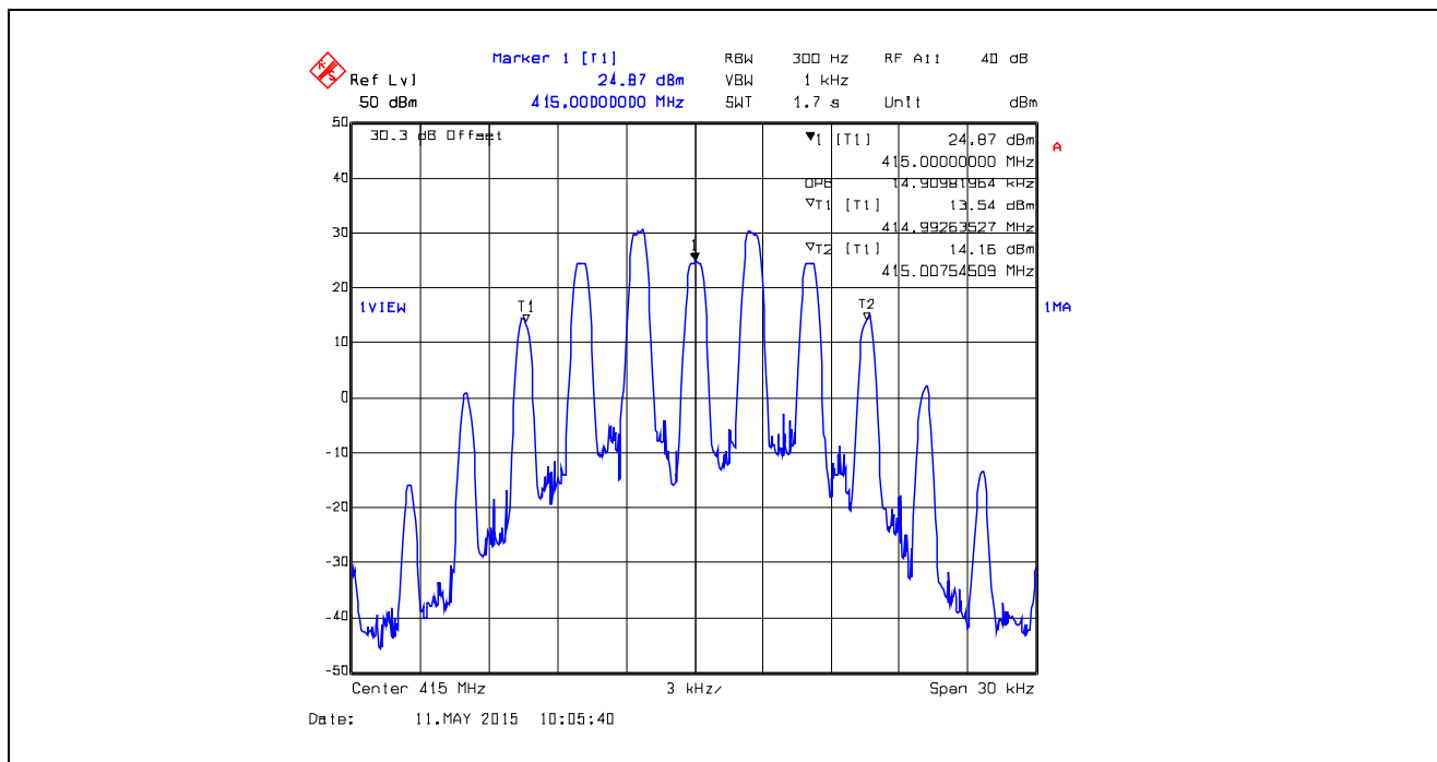
Plot 5.4.4.1.5. 99% Occupied Bandwidth, 25 kHz Channel Spacing, Analog, 415.0 MHz
