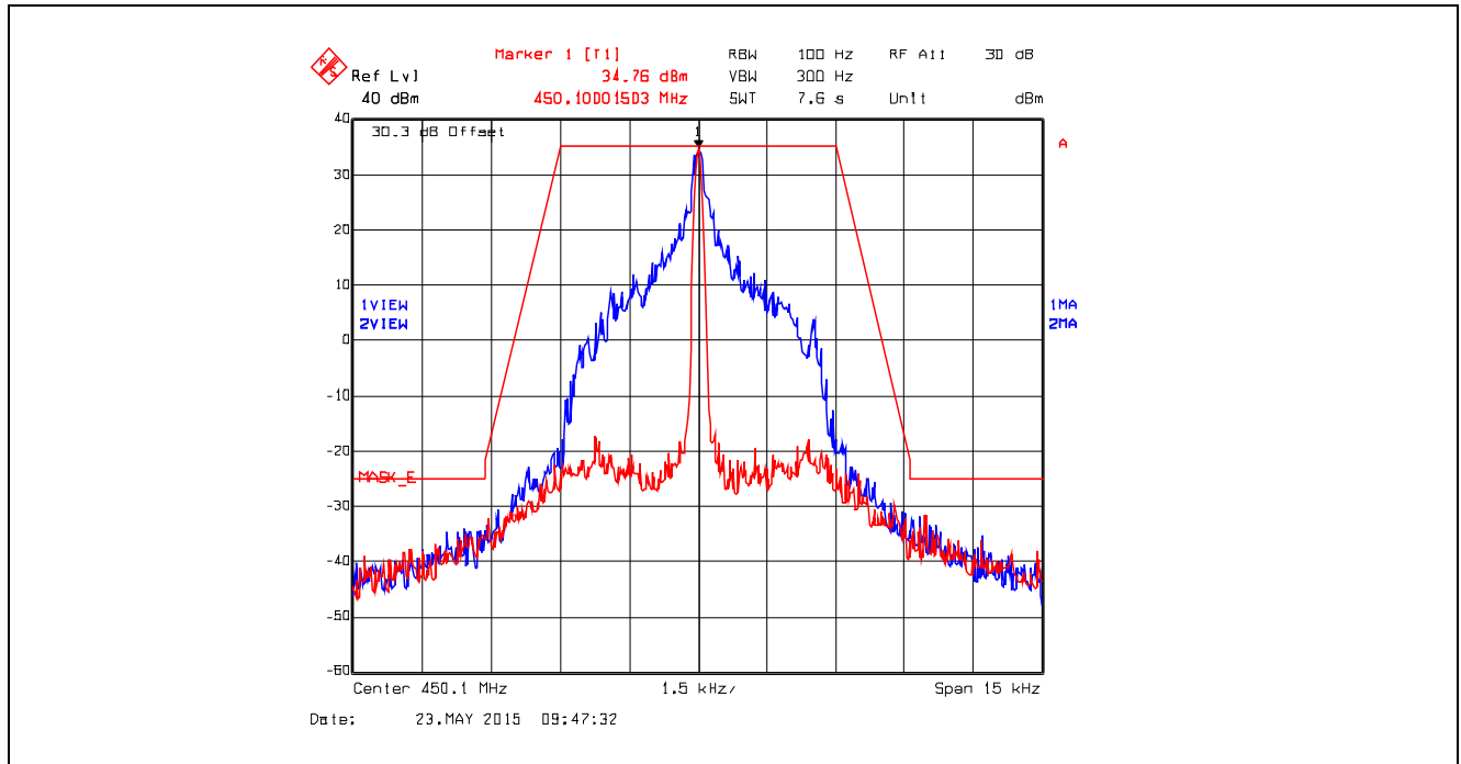
Plot 5.4.4.6.13. Emission Mask E, Digital at 4.8 kbps, 450.1 MHz, High Power
