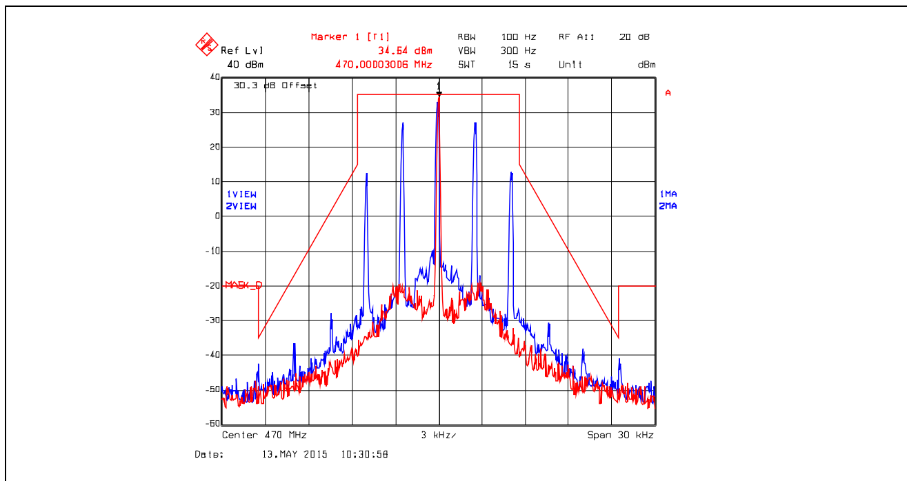
Plot 5.4.4.4.15. Emission Mask D, Analog, 470.0 MHz, High Power
