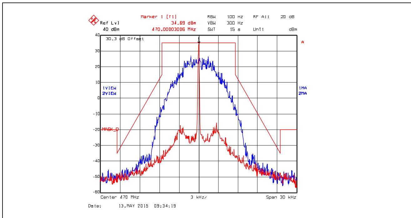
Plot 5.4.4.5.15. Emission Mask D, Digital at 9.6 kbps, 470.0 MHz, High Power
