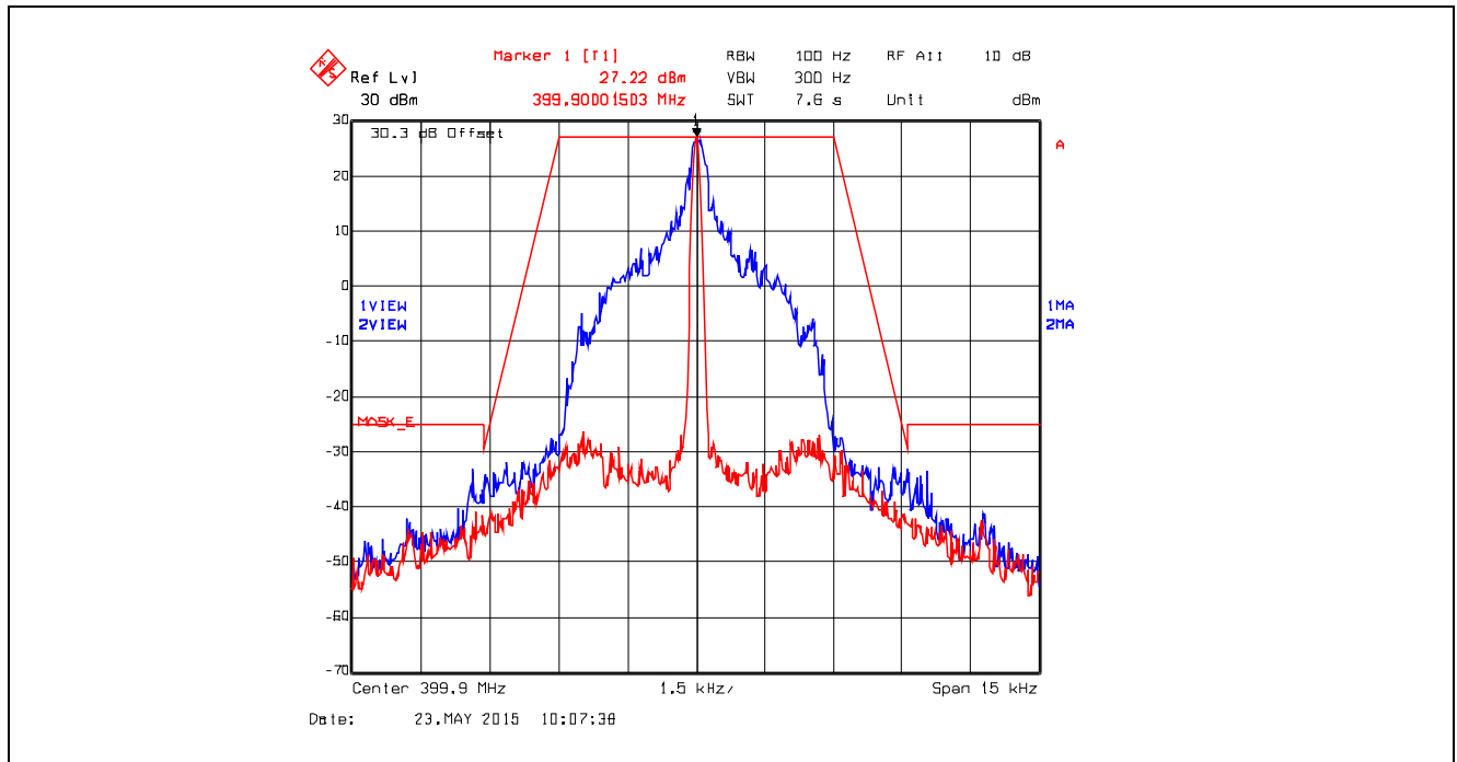
Plot 5.4.4.6.6. Emission Mask E, Digital at 4.8 kbps, 399.9 MHz, Low Power
