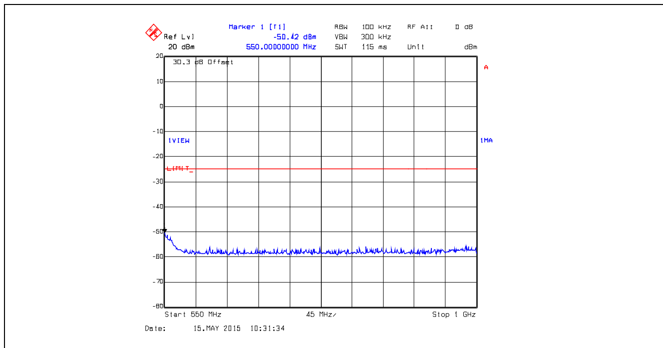
Plot 5.5.4.53. Conducted Transmitter Spurious Emissions, 511.9 MHz, Low Power, 550 MHz – 1 GHz
