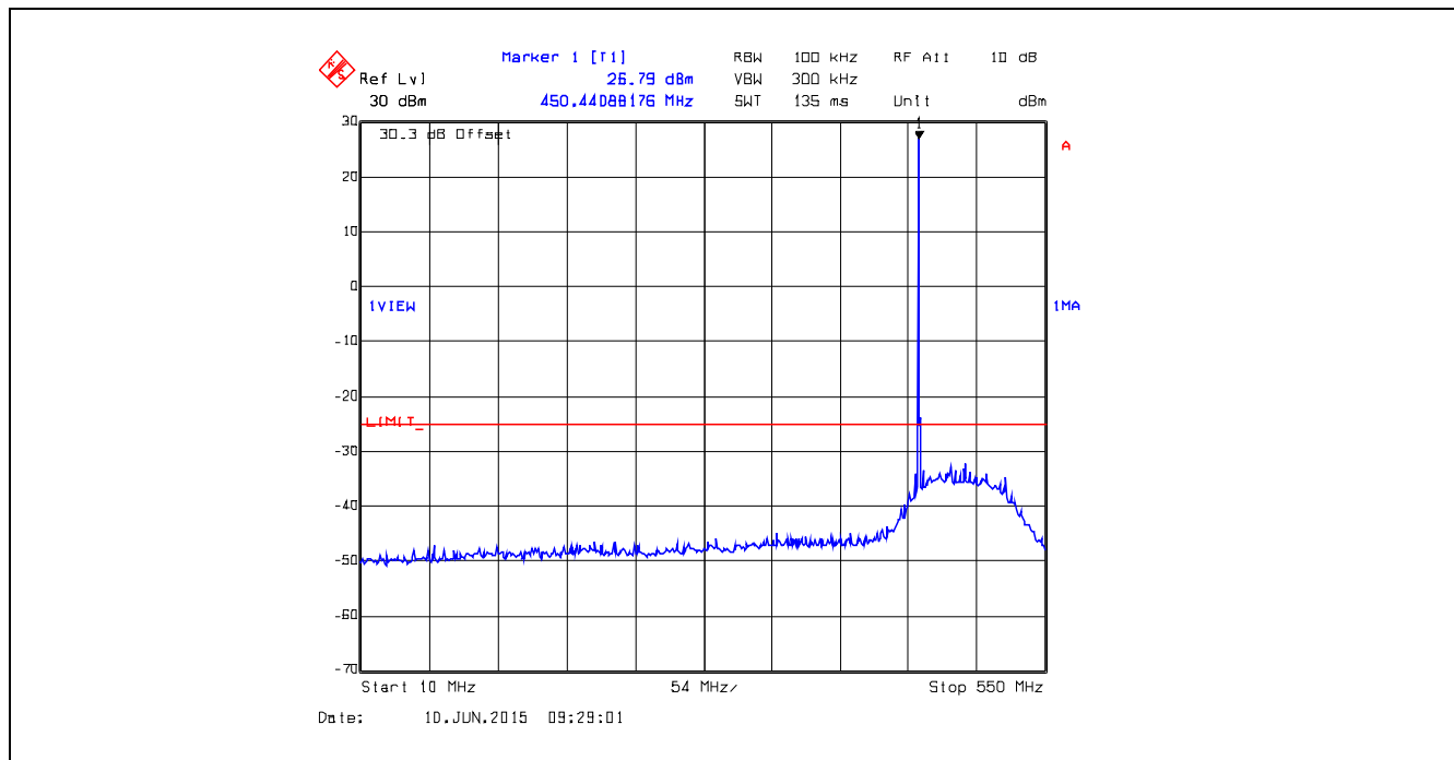
Plot 5.5.4.40. Conducted Transmitter Spurious Emissions, 450.1 MHz, Low Power, 10 MHz – 550 MHz
