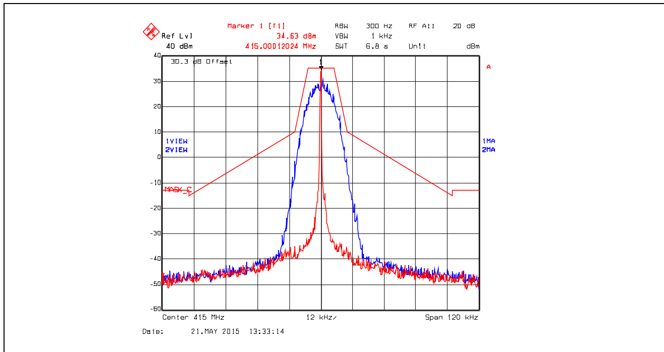
Plot 5.4.4.3.9. Emission Mask C, Digital at 19.2 kbps, 415.0 MHz, High Power
