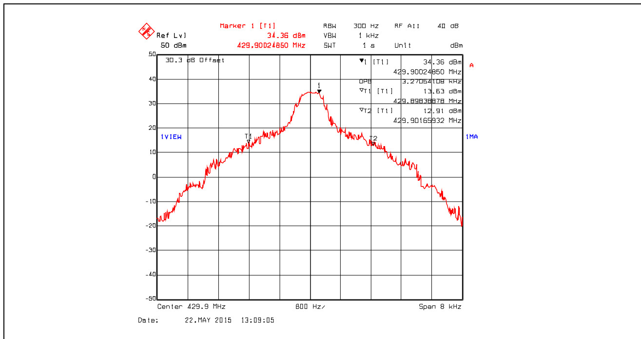
Plot 5.4.4.1.42. 99% Occupied Bandwidth, 6.25 kHz Channel Spacing, Digital 4.8 kbps, 429.9 MHz
