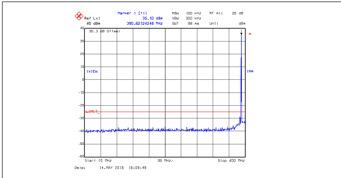
Plot 5.5.4.7. Conducted Transmitter Spurious Emissions, 390.0 MHz, High Power, 10 MHz – 400 MHz
