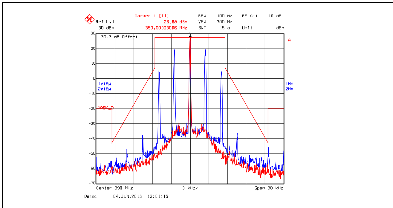
Plot 5.4.4.4.4. Emission Mask D, Analog, 390.0 MHz, Low Power
