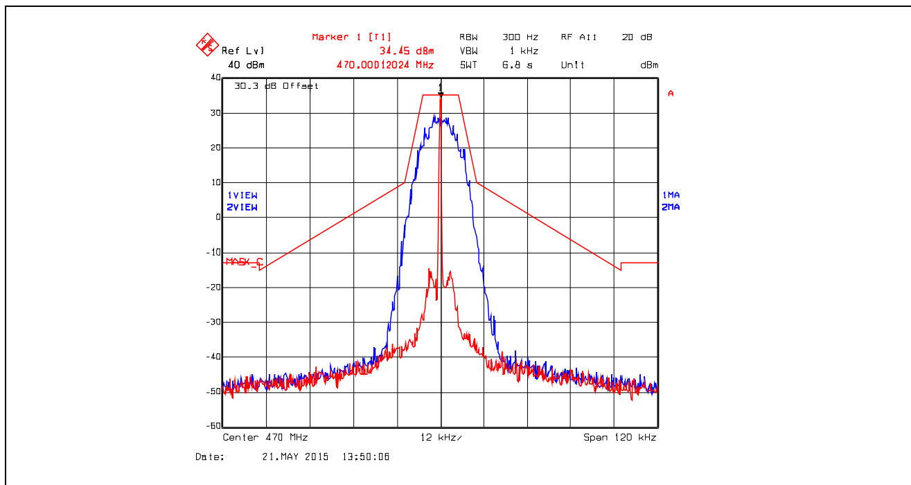
Plot 5.4.4.3.15. Emission Mask C, Digital at 19.2 kbps, 470.0 MHz, High Power
