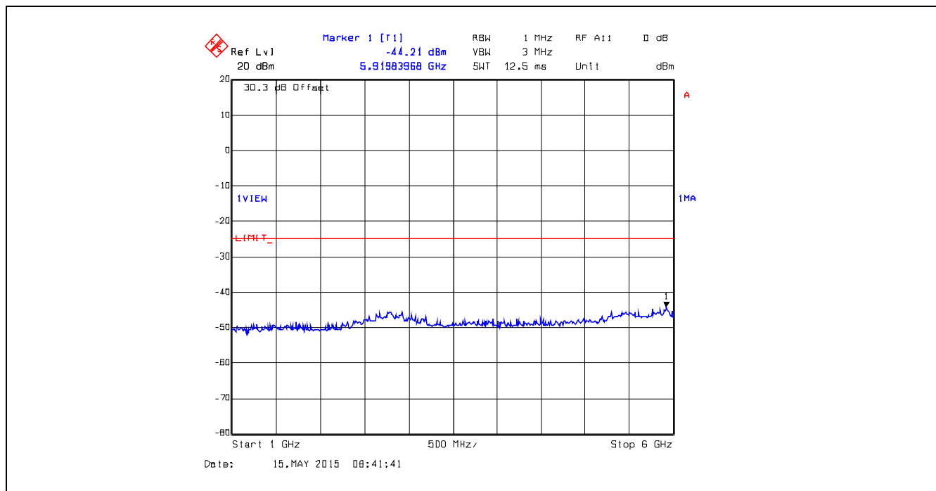
Plot 5.5.4.45. Conducted Transmitter Spurious Emissions, 470.0 MHz, High Power, 1 GHz – 6 GHz
