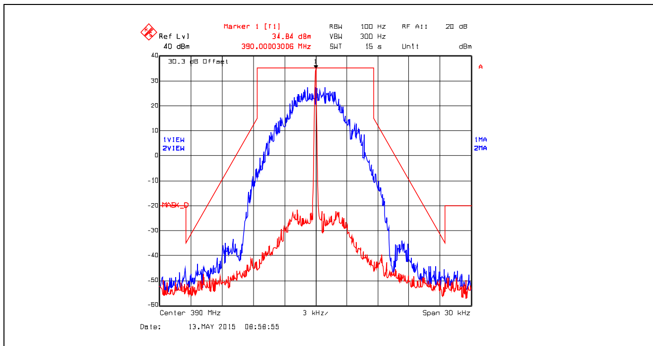
Plot 5.4.4.5.3. Emission Mask D, Digital at 9.6 kbps, 390.0 MHz, High Power
