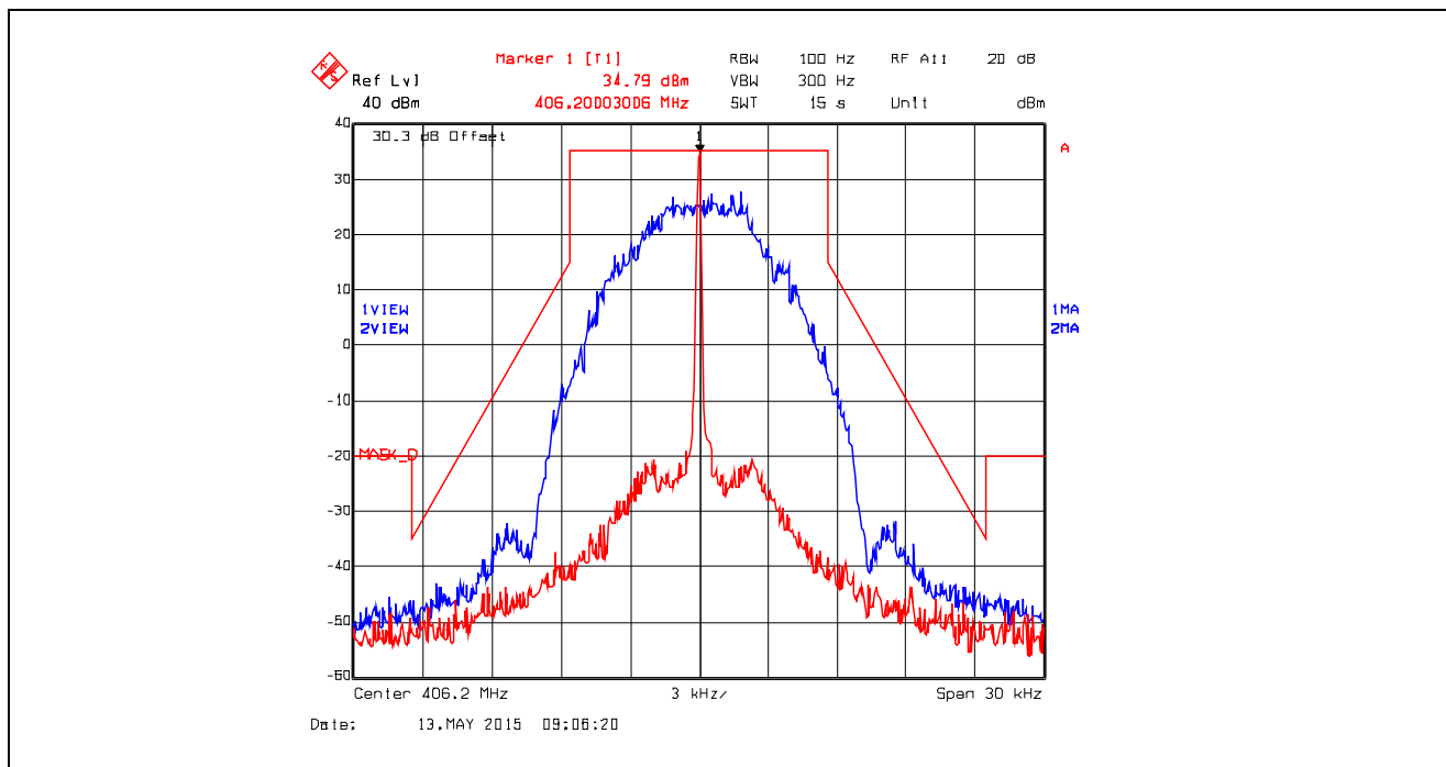
Plot 5.4.4.5.7. Emission Mask D, Digital at 9.6 kbps, 406.2 MHz, High Power
