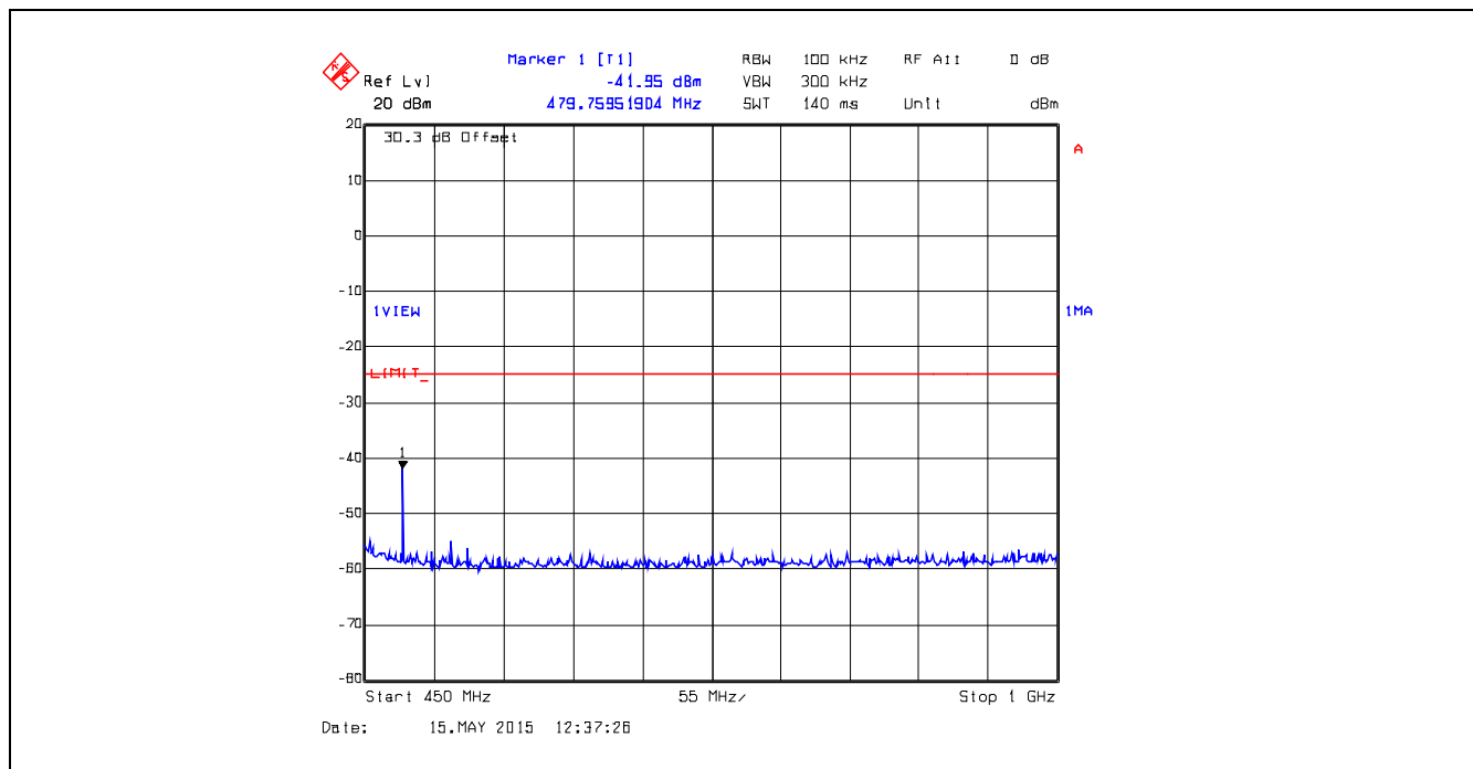
Plot 5.5.4.35. Conducted Transmitter Spurious Emissions, 429.9 MHz, Low Power, 450 MHz – 1 GHz
