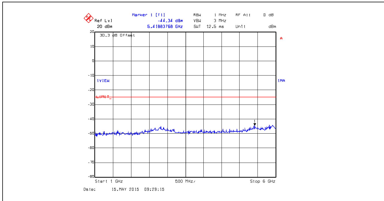
Plot 5.5.4.3. Conducted Transmitter Spurious Emissions, 380.1 MHz, High Power, 1 GHz – 6 GHz
