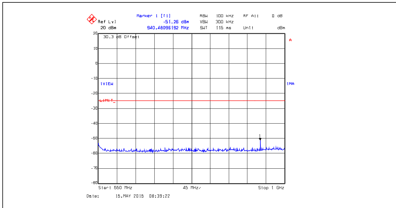
Plot 5.5.4.44. Conducted Transmitter Spurious Emissions, 470.0 MHz, High Power, 550 MHz – 1 GHz
