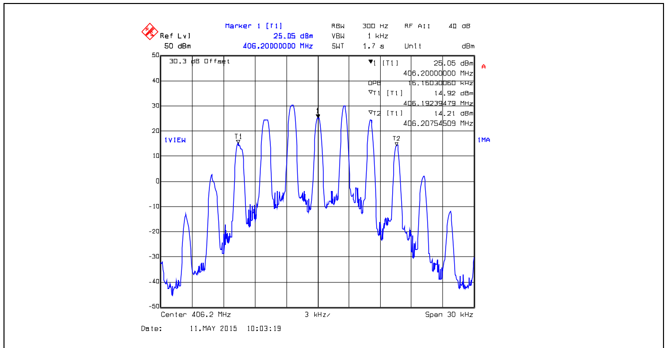
Plot 5.4.4.1.4. 99% Occupied Bandwidth, 25 kHz Channel Spacing, Analog, 406.2 MHz
