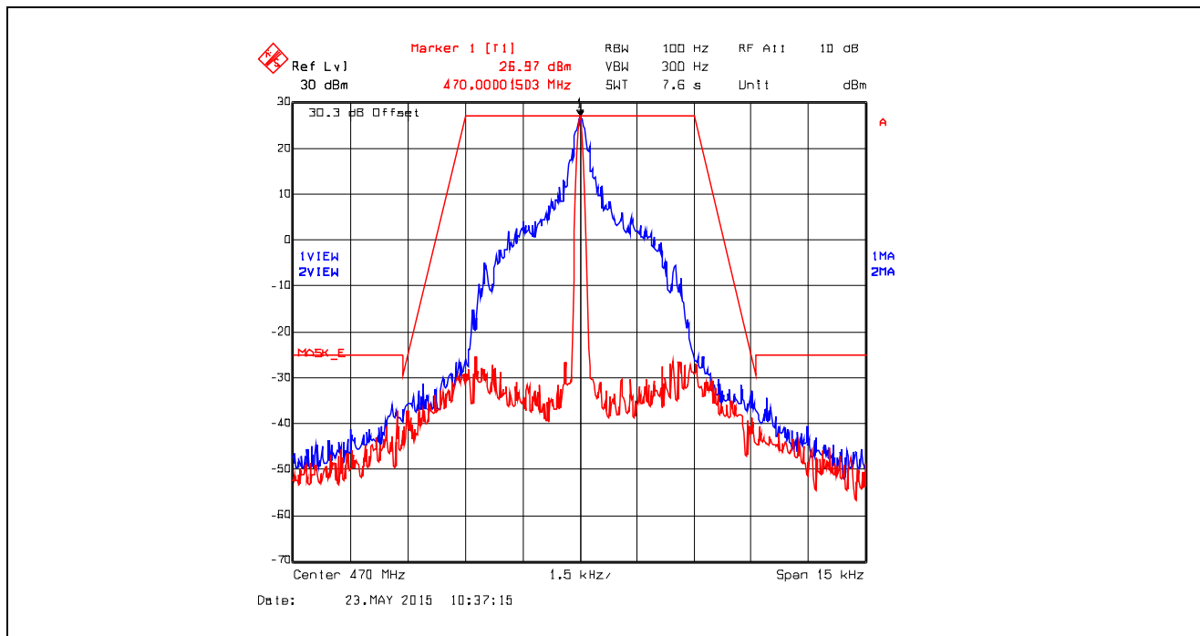
Plot 5.4.4.6.16. Emission Mask E, Digital at 4.8 kbps, 470.0 MHz, Low Power
