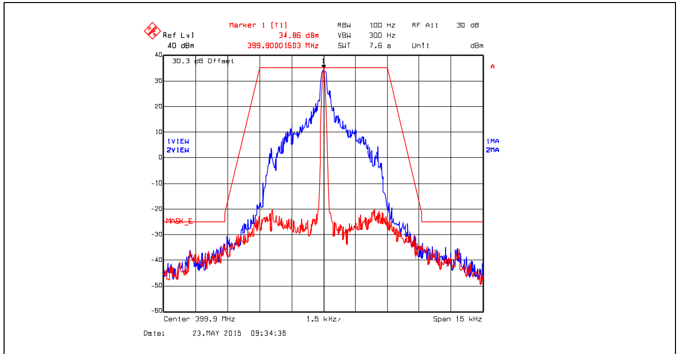
Plot 5.4.4.6.5. Emission Mask E, Digital at 4.8 kbps, 399.9 MHz, High Power
