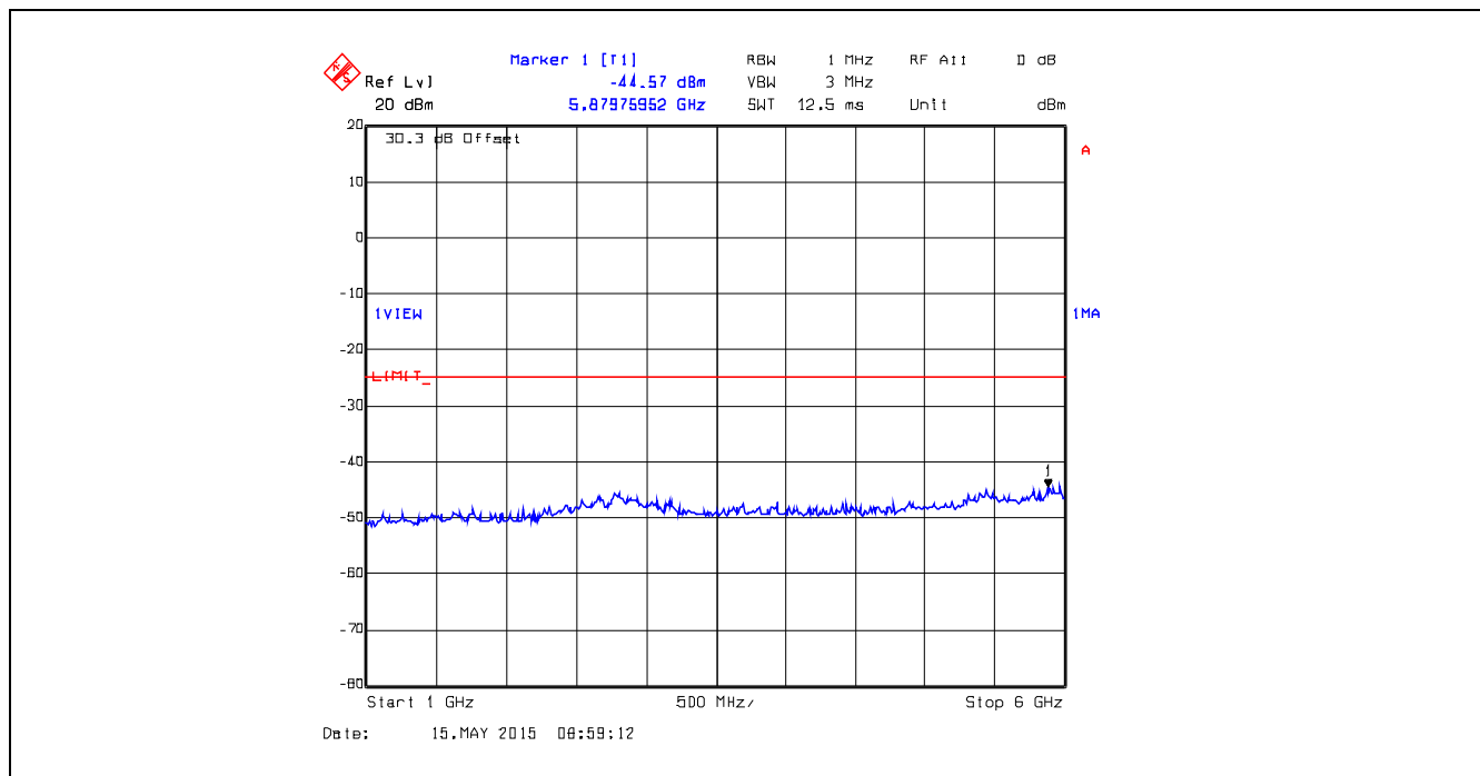
Plot 5.5.4.27. Conducted Transmitter Spurious Emissions, 415.0 MHz, High Power, 1 GHz – 6 GHz
