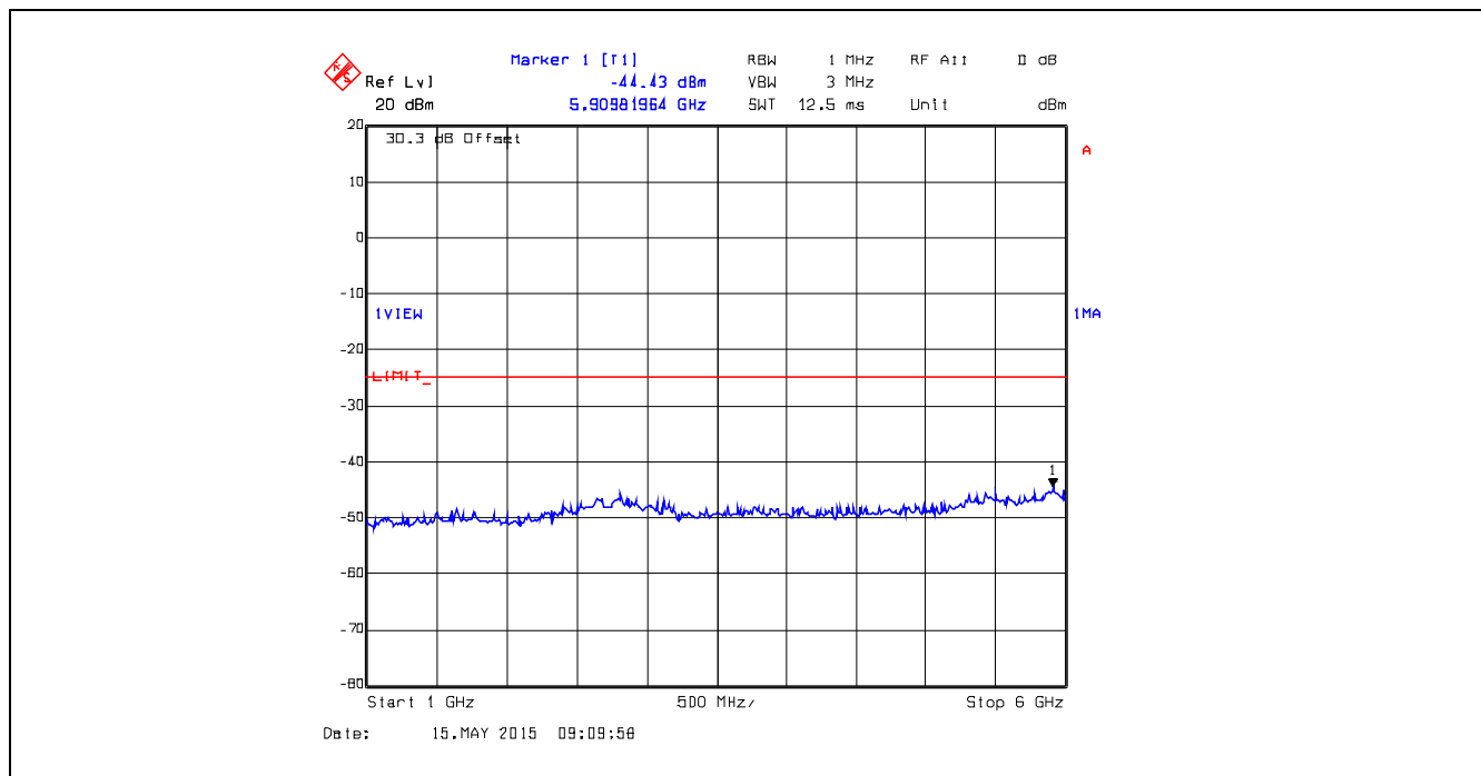
Plot 5.5.4.21. Conducted Transmitter Spurious Emissions, 406.2 MHz, High Power, 1 GHz – 6 GHz
