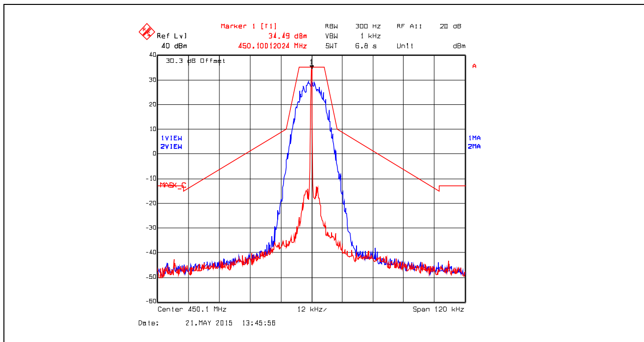
Plot 5.4.4.3.13. Emission Mask C, Digital at 19.2 kbps, 450.1 MHz, High Power
