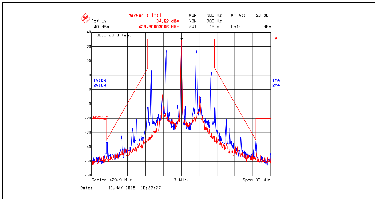
Plot 5.4.4.4.11. Emission Mask D, Analog, 429.9 MHz, High Power
