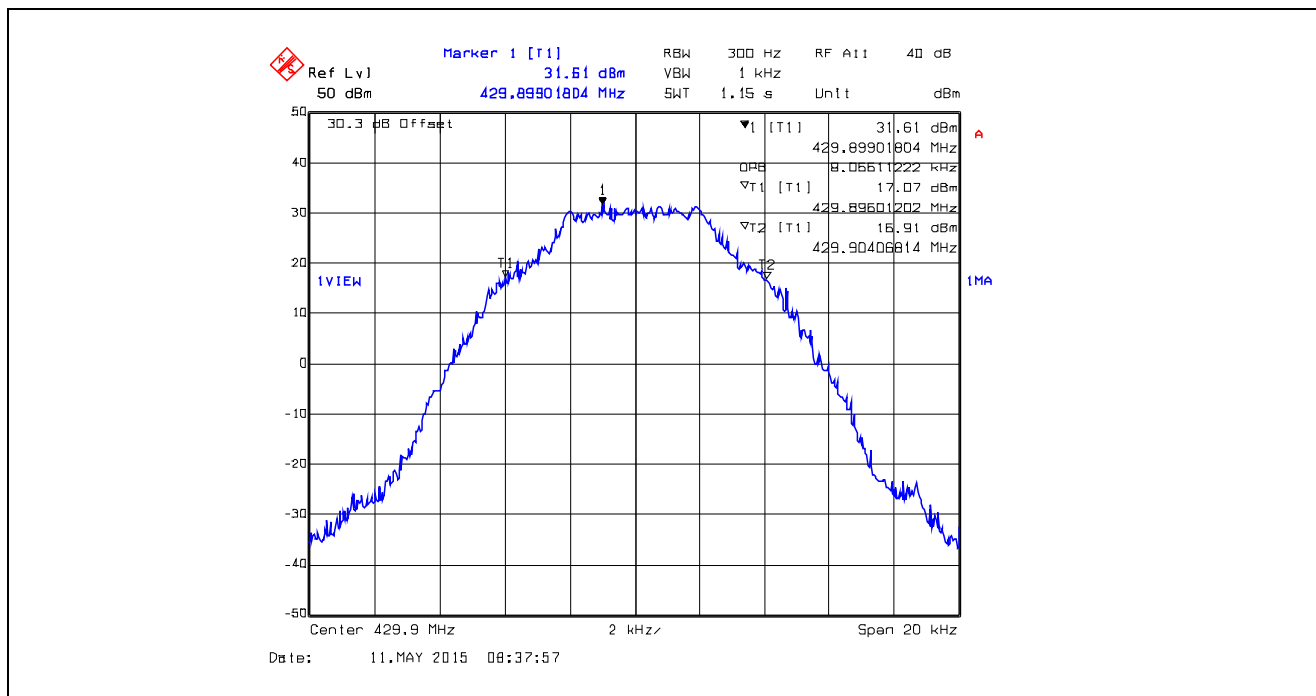
Plot 5.4.4.1.33. 99% Occupied Bandwidth, 12.5 kHz Channel Spacing, Digital 9.6 kbps, 429.9 MHz
