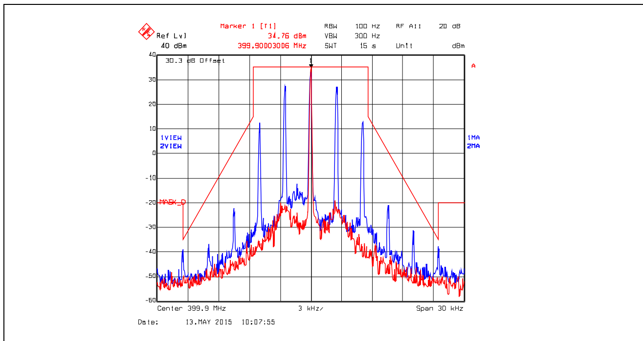
Plot 5.4.4.4.5. Emission Mask D, Analog, 399.9 MHz, High Power
