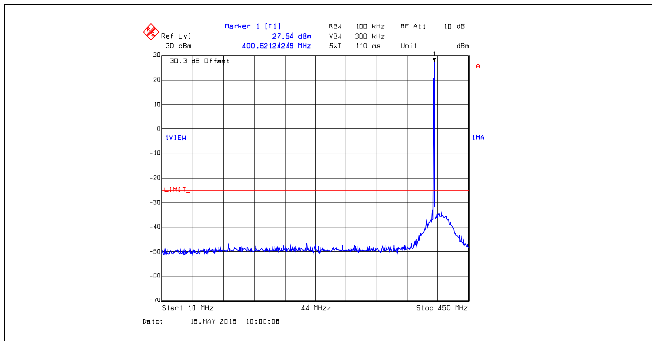
Plot 5.5.4.16. Conducted Transmitter Spurious Emissions, 399.9 MHz, Low Power, 10 MHz – 450 MHz
