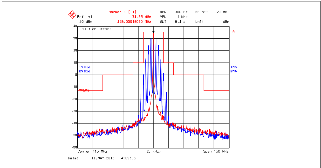
Plot 5.4.4.2.9. Emission Mask B, Analog, 415.0 MHz, High Power
