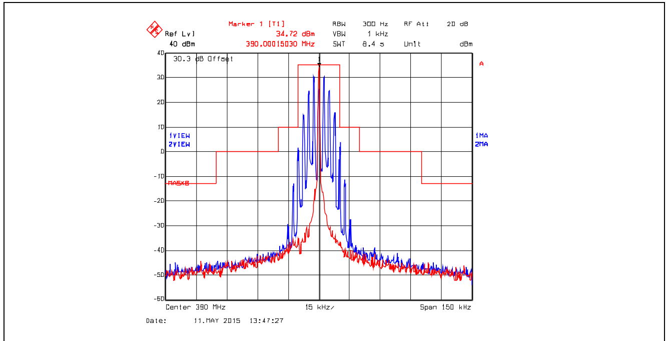
Plot 5.4.4.2.3. Emission Mask B, Analog, 390.0 MHz, High Power
