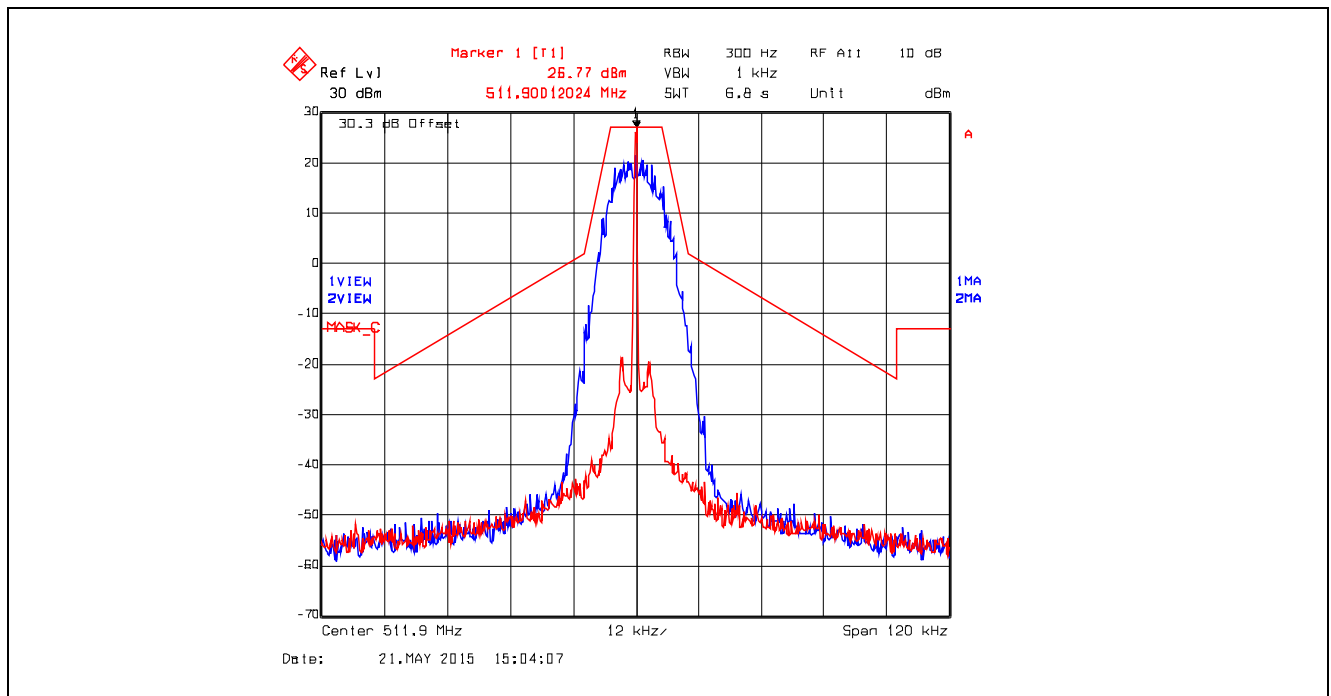
Plot 5.4.4.3.18. Emission Mask C, Digital at 19.2 kbps, 511.9 MHz, Low Power
