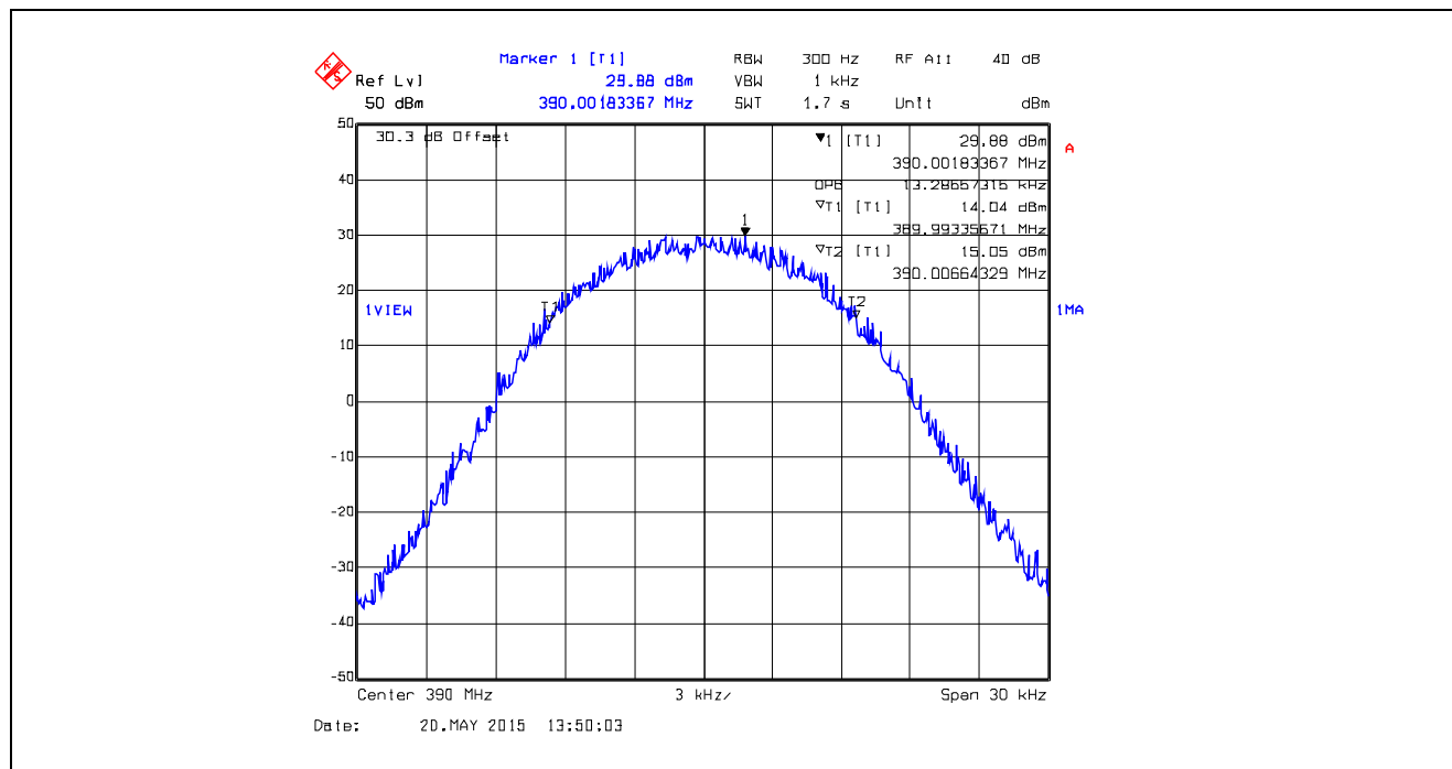
Plot 5.4.4.1.11. 99% Occupied Bandwidth, 25 kHz Channel Spacing, Digital 19.2 kbps, 390.0 MHz
