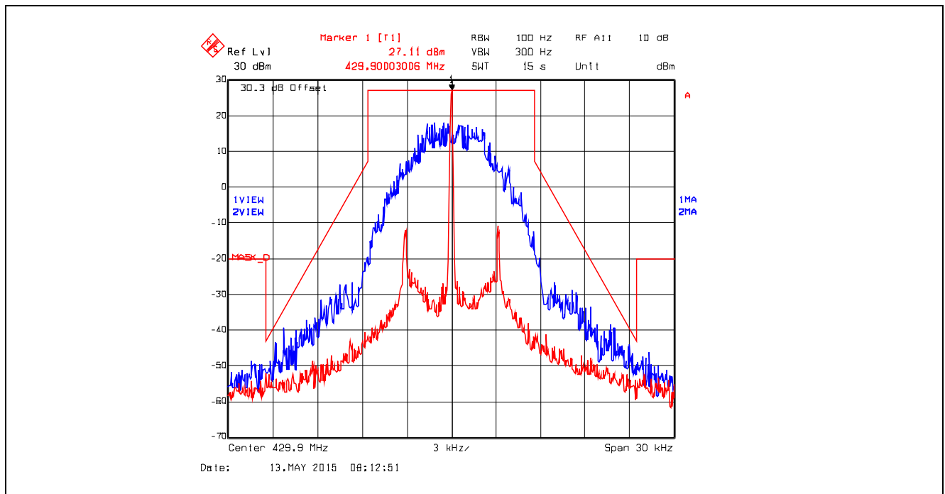
Plot 5.4.4.5.12. Emission Mask D, Digital at 9.6 kbps, 429.9 MHz, Low Power
