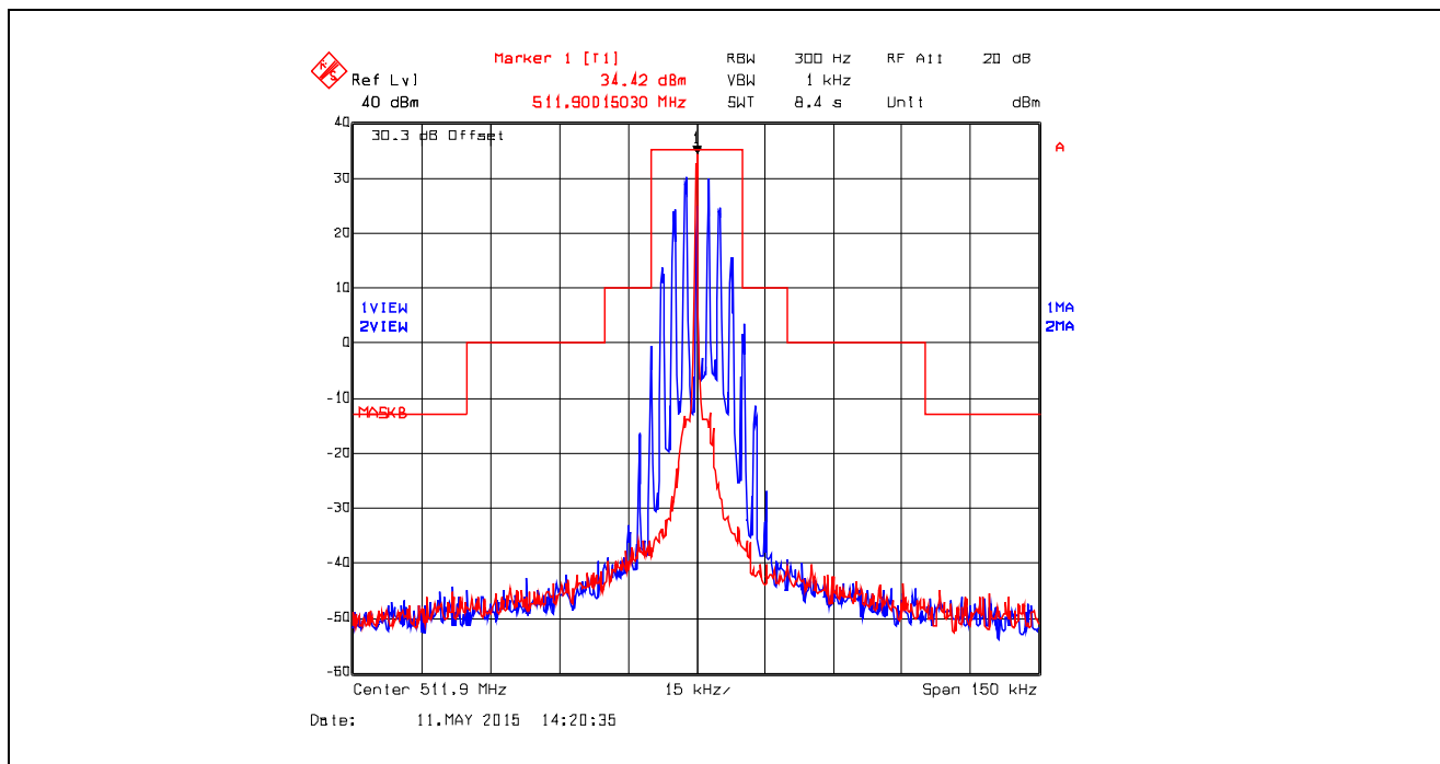
Plot 5.4.4.2.17. Emission Mask B, Analog, 511.9 MHz, High Power
