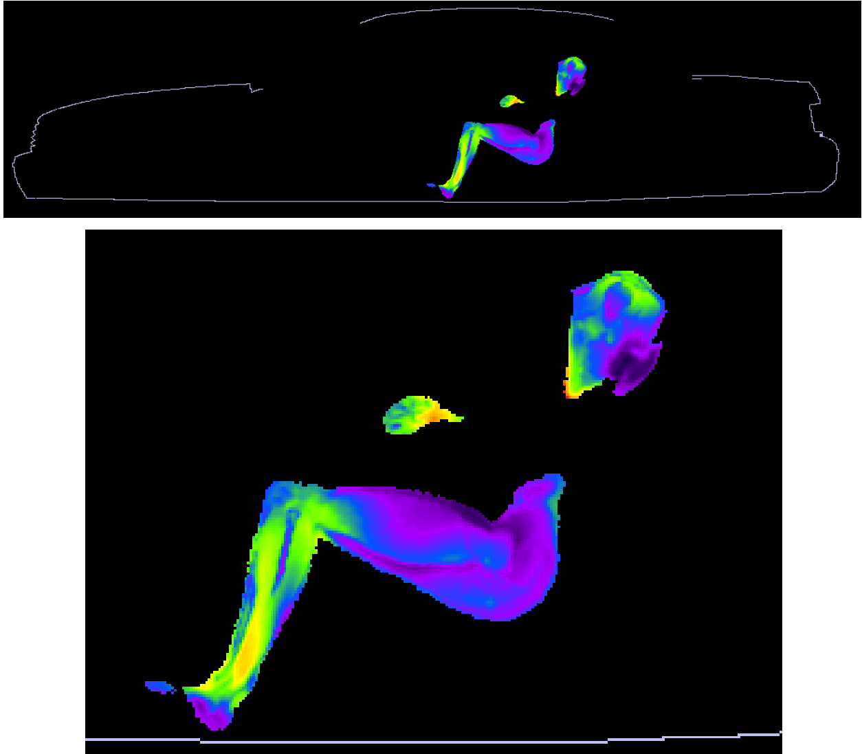
Figure 5. SAR distribution at 173.4000 MHz in the passenger model located on the side of the back seat, produced by the roof-mount HAD4022A antenna. The contour plot is relative to the plane where the peak 1-g average SAR for this exposure condition occurs.
