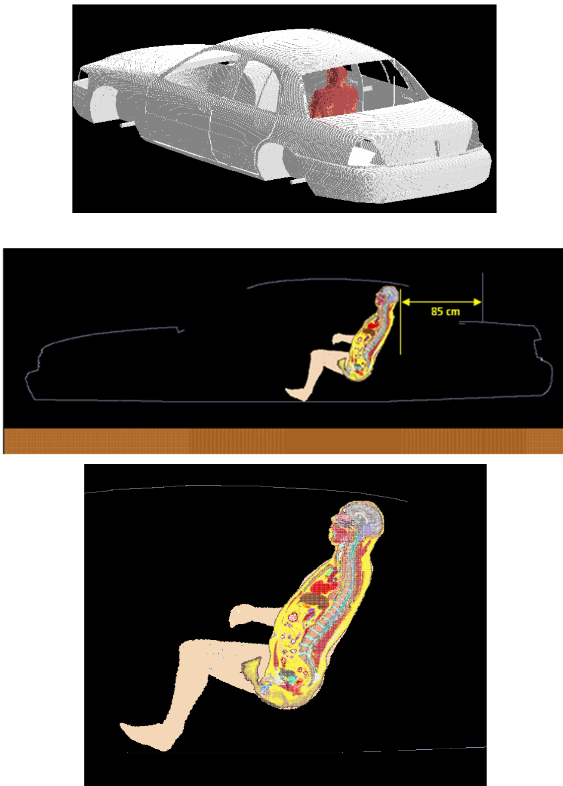
Figure 2: Passenger (back seat) model exposed to a trunk-mount antenna: XFDTD geometry. The antenna is mounted at 85 cm from the passenger located in the center of the back seat.
