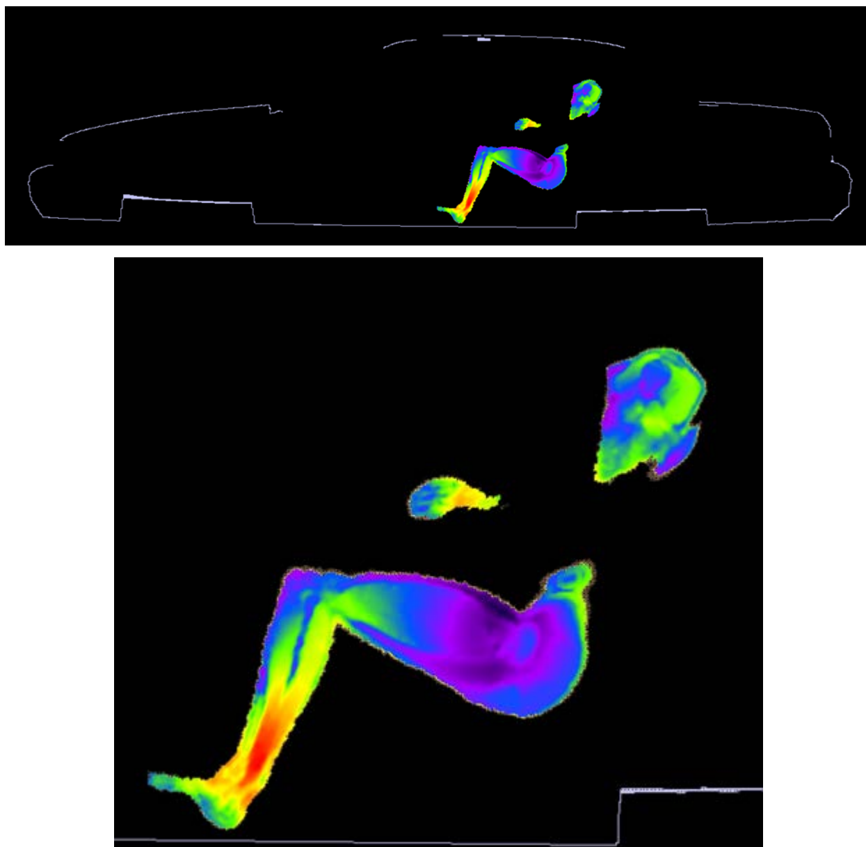
Figure 3. SAR distribution at 167.7000 MHz in the passenger model located on the side of the back seat, produced by the trunk-mount HAD4009A antenna. The contour plot is relative to the plane where the peak 1-g average SAR for this exposure condition occurs.
