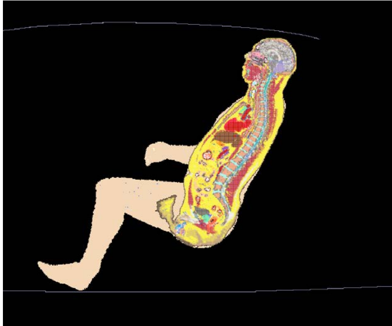
Figure 2: Passenger model exposed to a trunk-mount antenna: XFDTD geometry.
