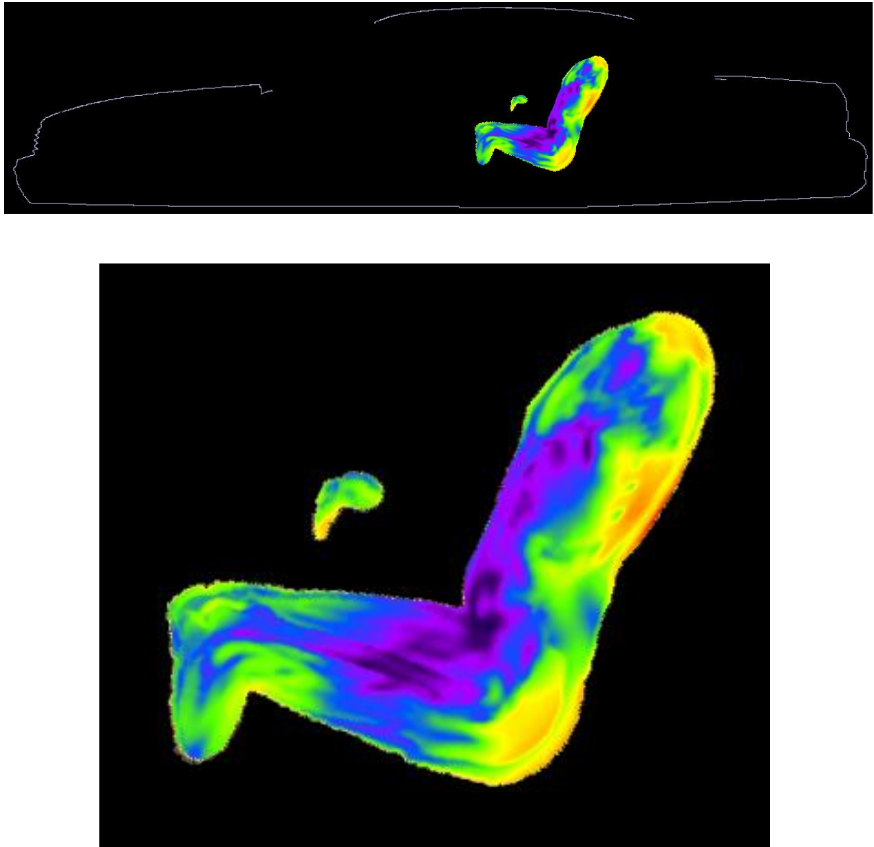
Figure 3. SAR distribution at 775.0000 MHz in the passenger model located on the side of the back seat, produced by the trunk-mount HAF4016A antenna. The contour plot is relative to the plane where the peak 1-g average SAR for this exposure condition occurs.
