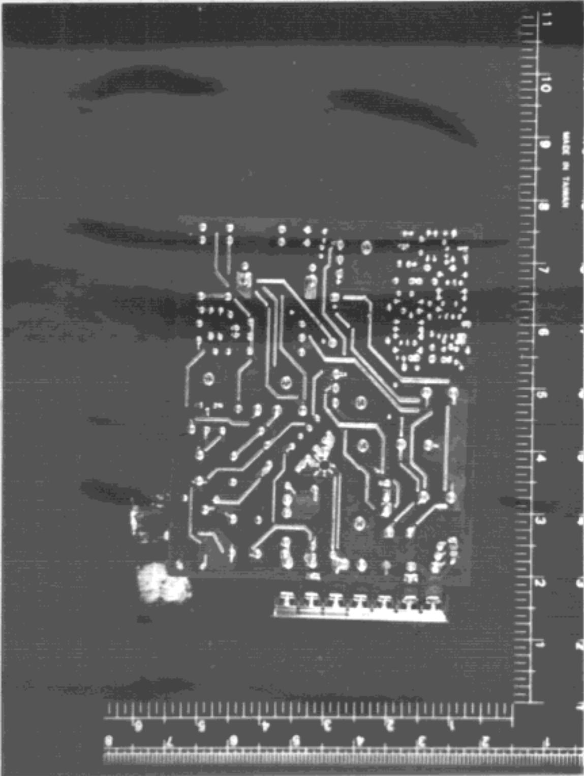
58. SOLDER SIDE OF S.P.S. MAIN BOARD
