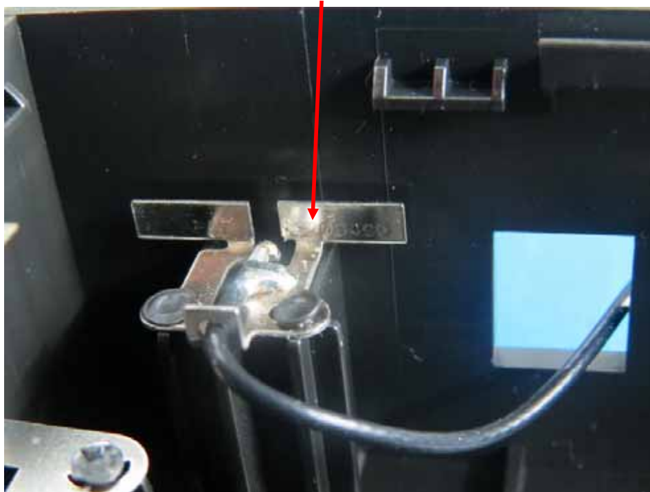
5G WIFI Antenna 1 – Top View
