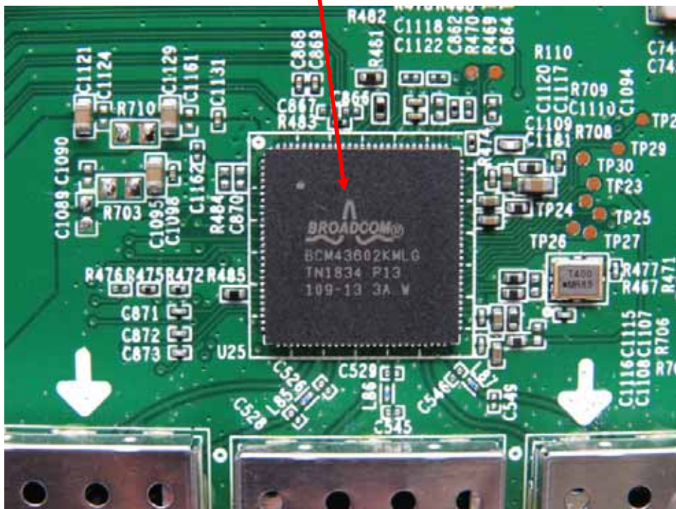
2.4G WIFI RF Chip IC – Top View
