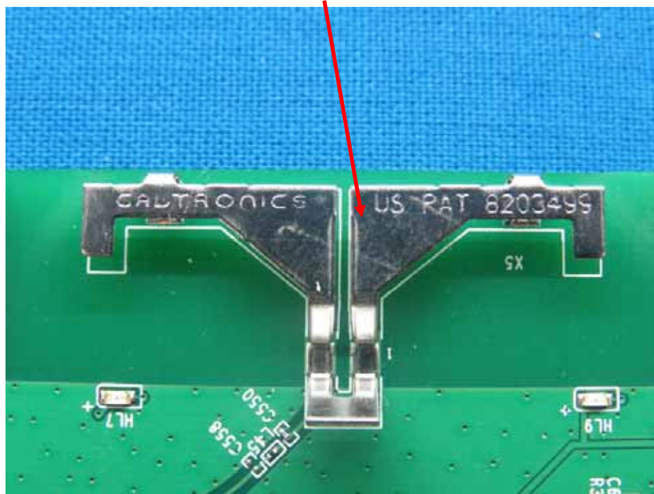
2.4G WIFI Antenna 3 – Top View
