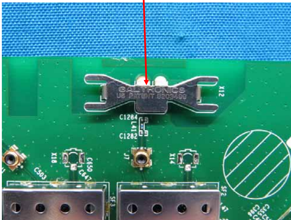
5G WIFI Antenna 3 – Top View
