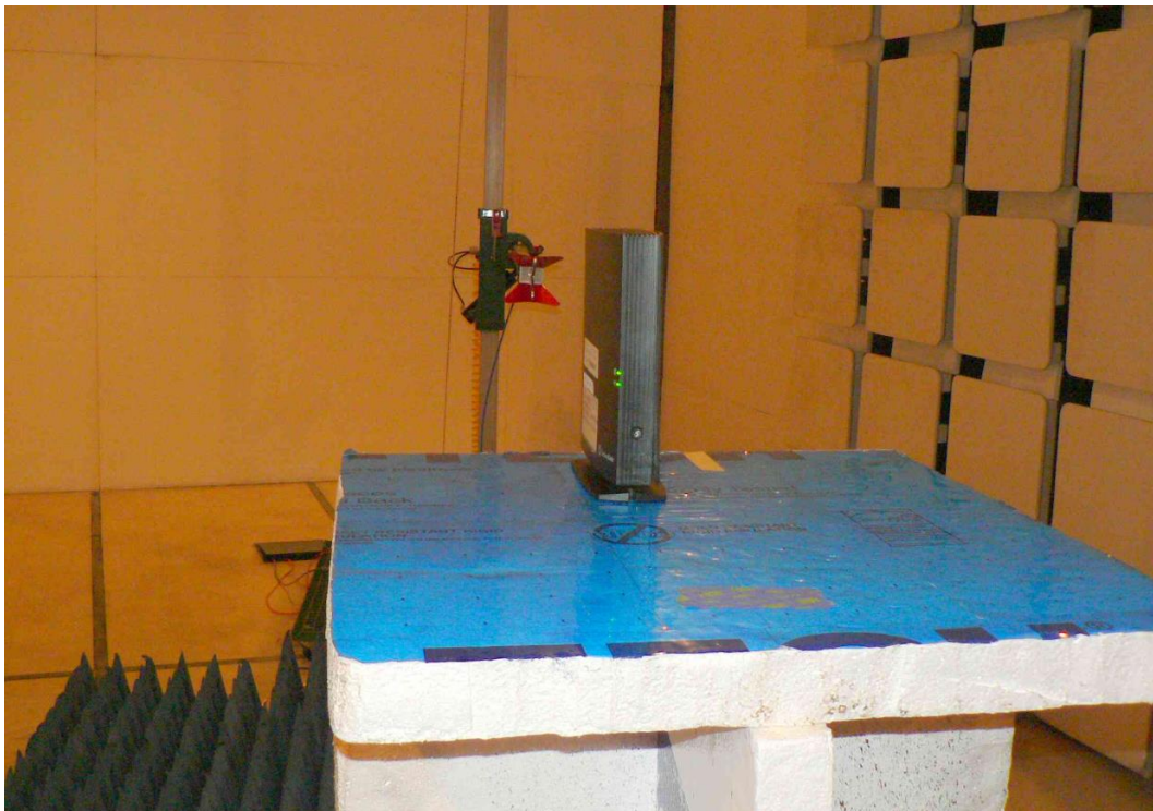
TX Spurious Emissions 1-18 GHz Back
