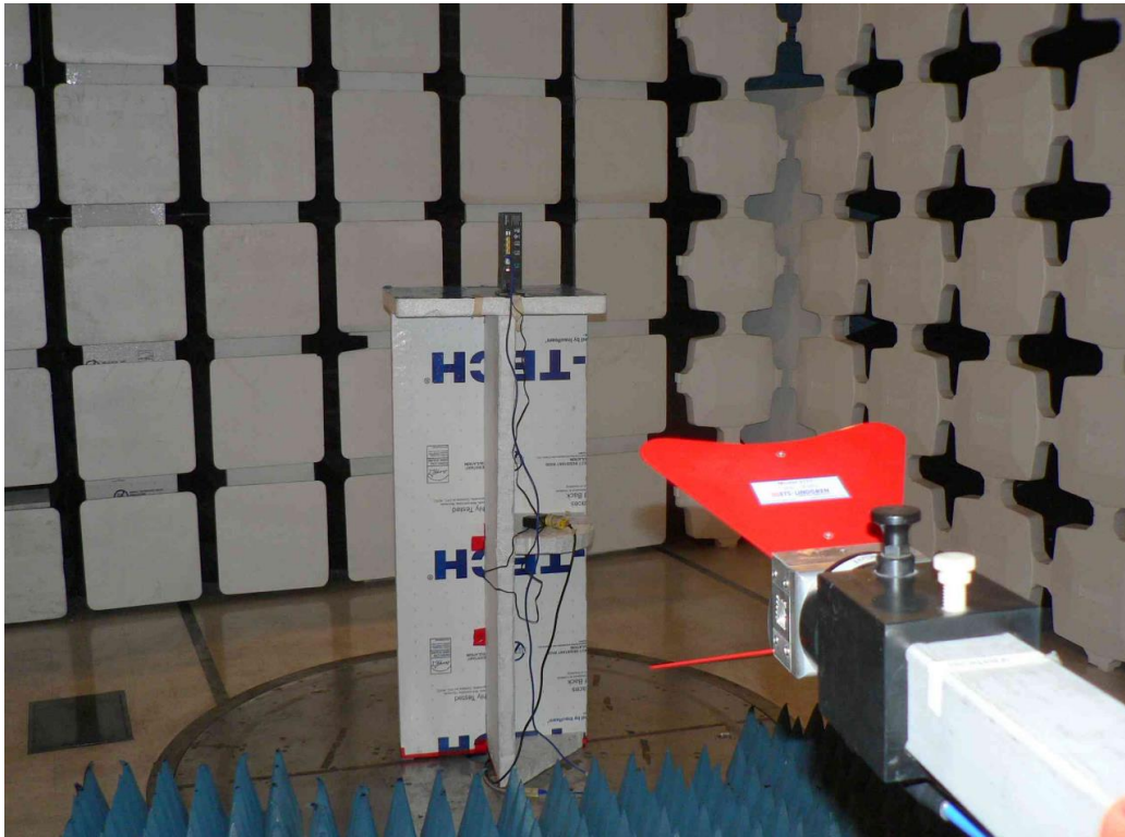
TX Spurious Emissions 1-18 GHz Back
