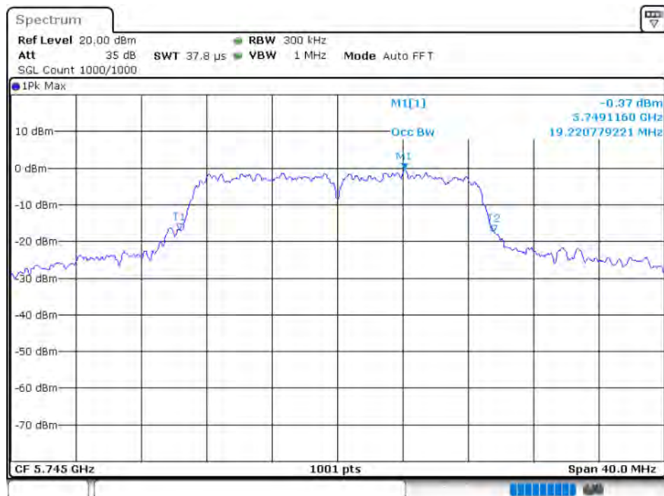
OBW NVNT 802.11n(HT20) 5745MHz Ant 4
