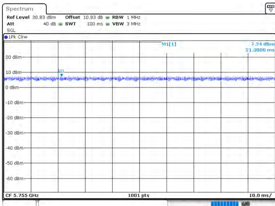
Duty Cycle NVNT 802.11n(HT40) 5755MHz Ant 4
