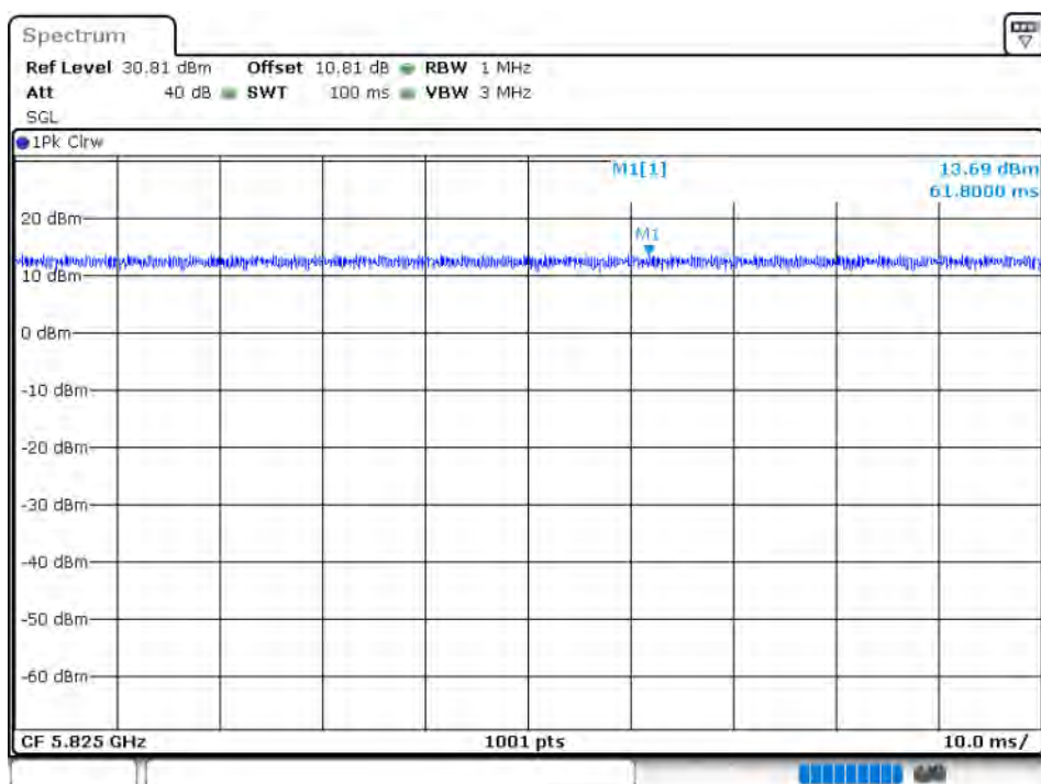
Duty Cycle NVNT 802.11n(HT20) 5825MHz Ant 4
