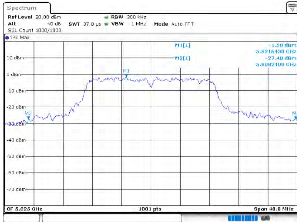
-26 dB BW NVNT 802.11n(HT20) 5825MHz Ant 3
