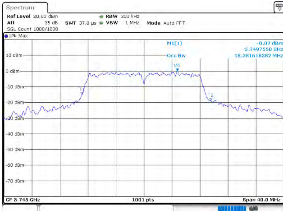
OBW NVNT 802.11a 5745MHz Ant 3
