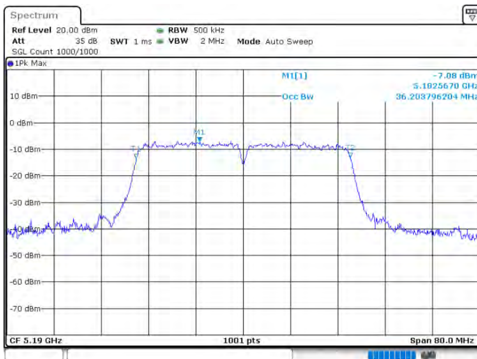
OBW NVNT 802.11n(HT40) 5190MHz Ant 4
