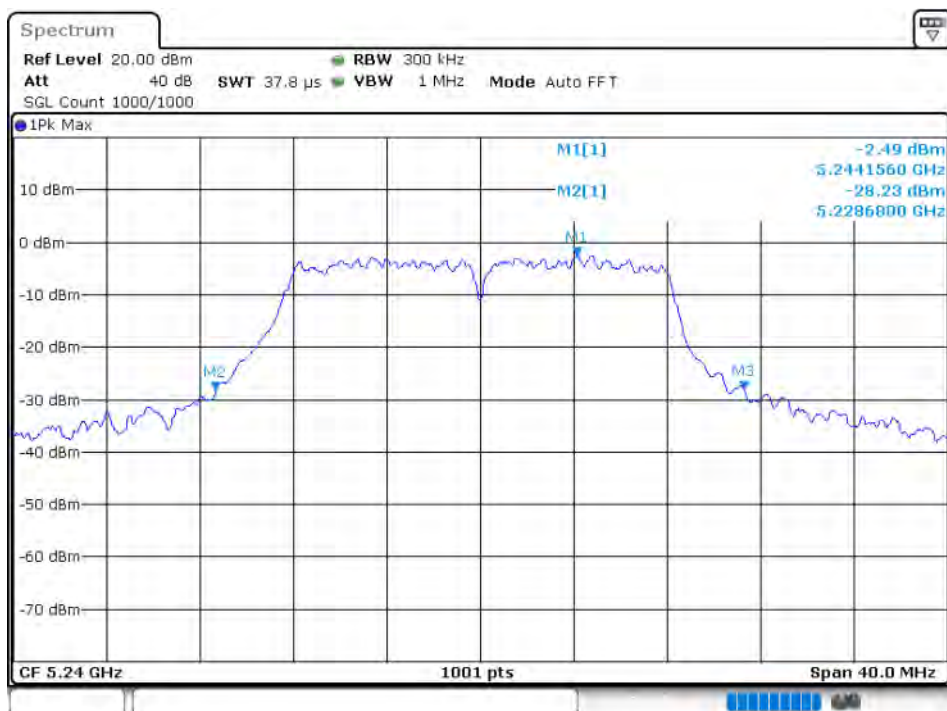
-26 dB BW NVNT 802.11a 5240MHz Ant 4
