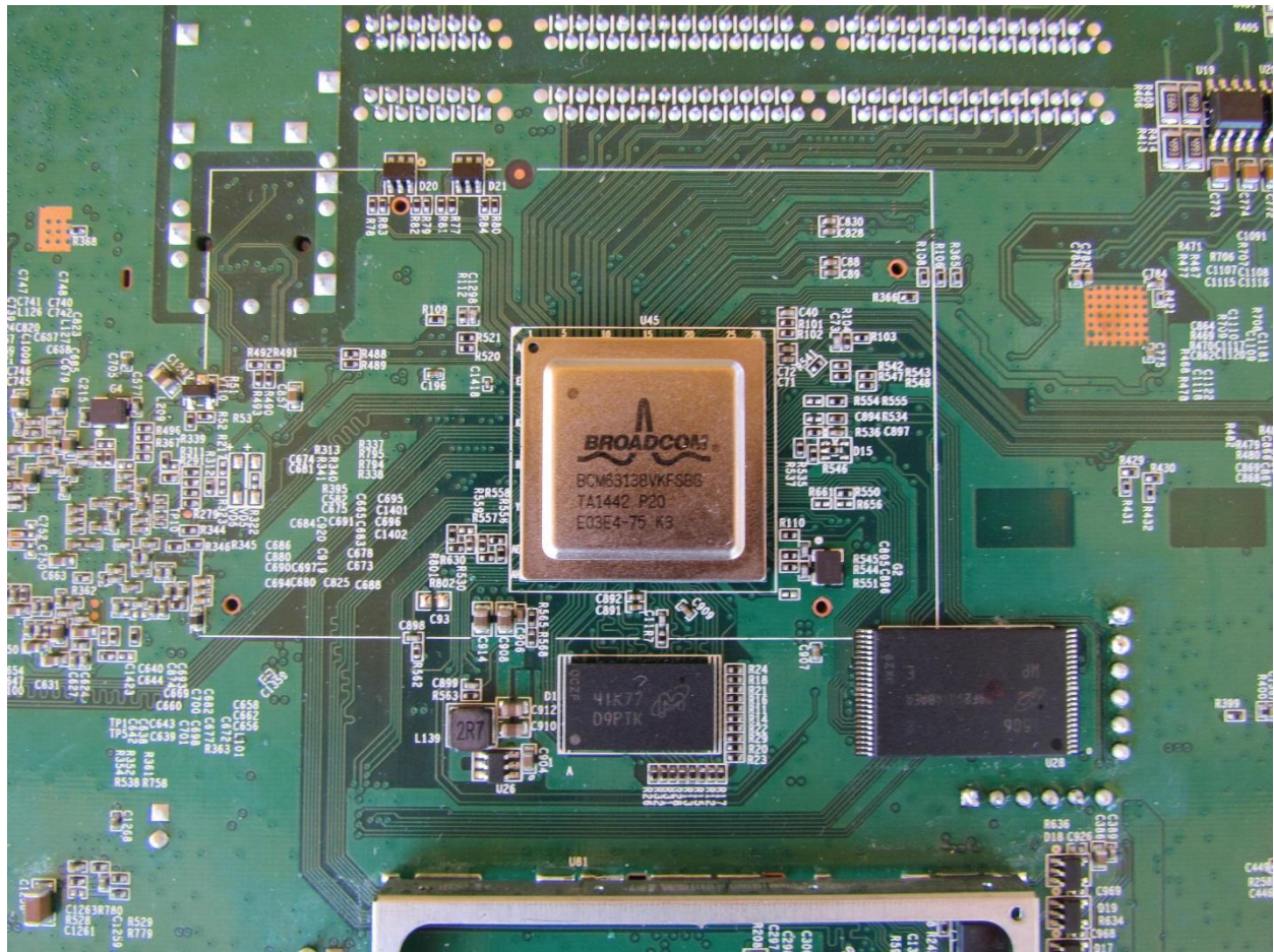
EUT - Radio 1 View
