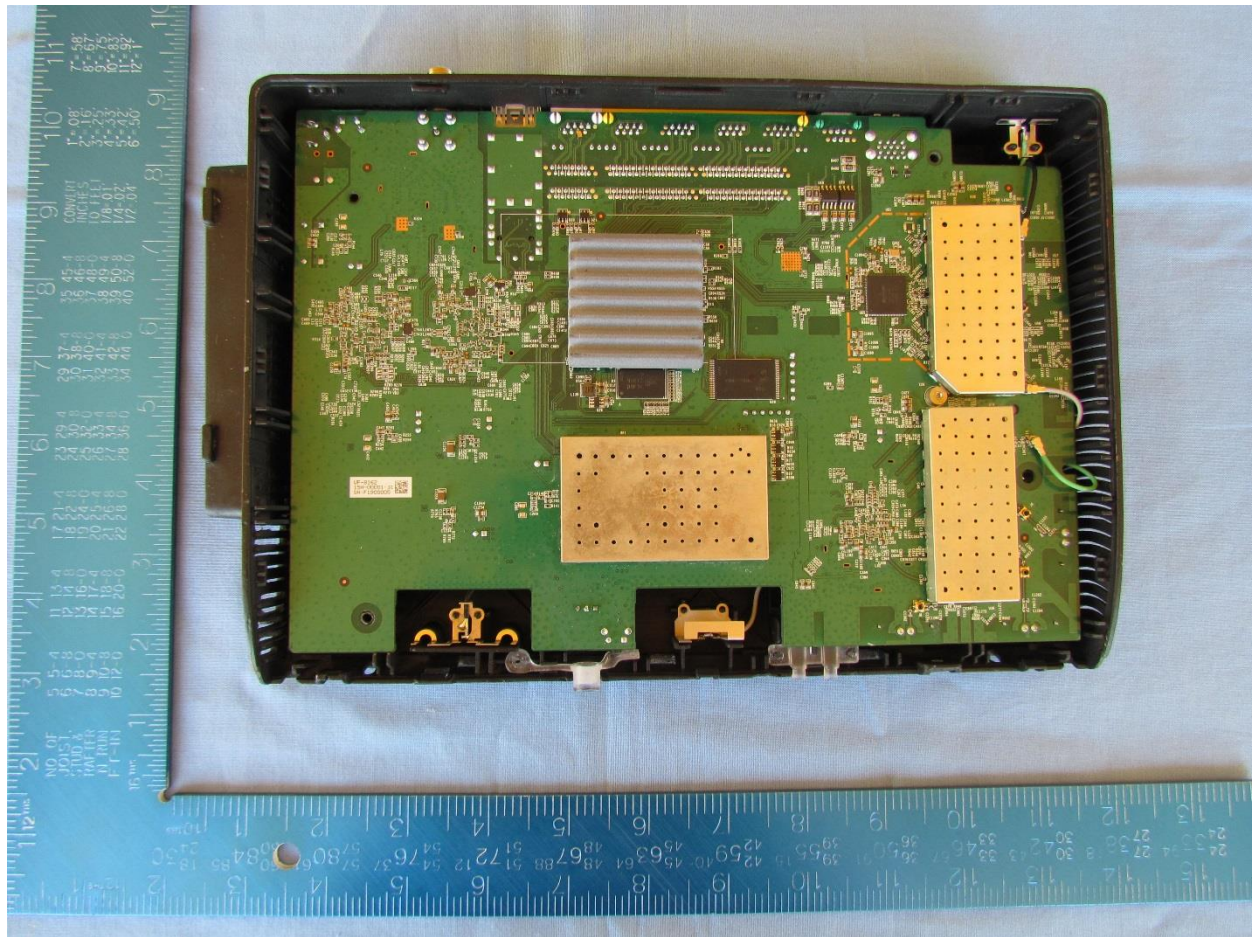
EUT - Internal View Shielding & Housing
