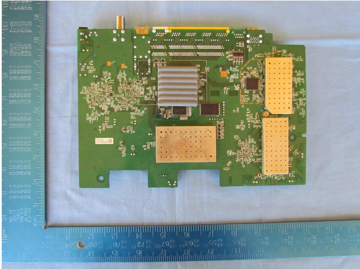
EUT - Top View Shielding
