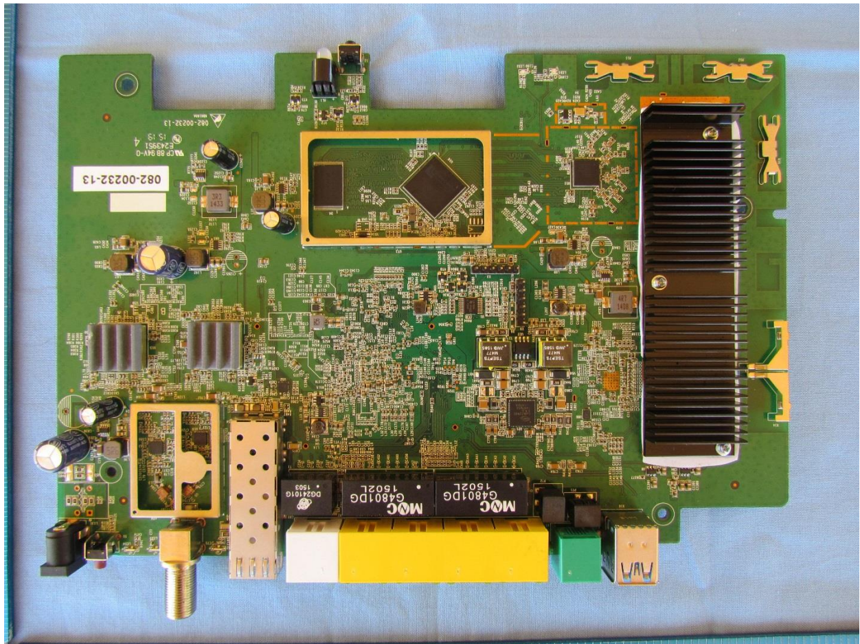
EUT - Bottom View No Shielding
