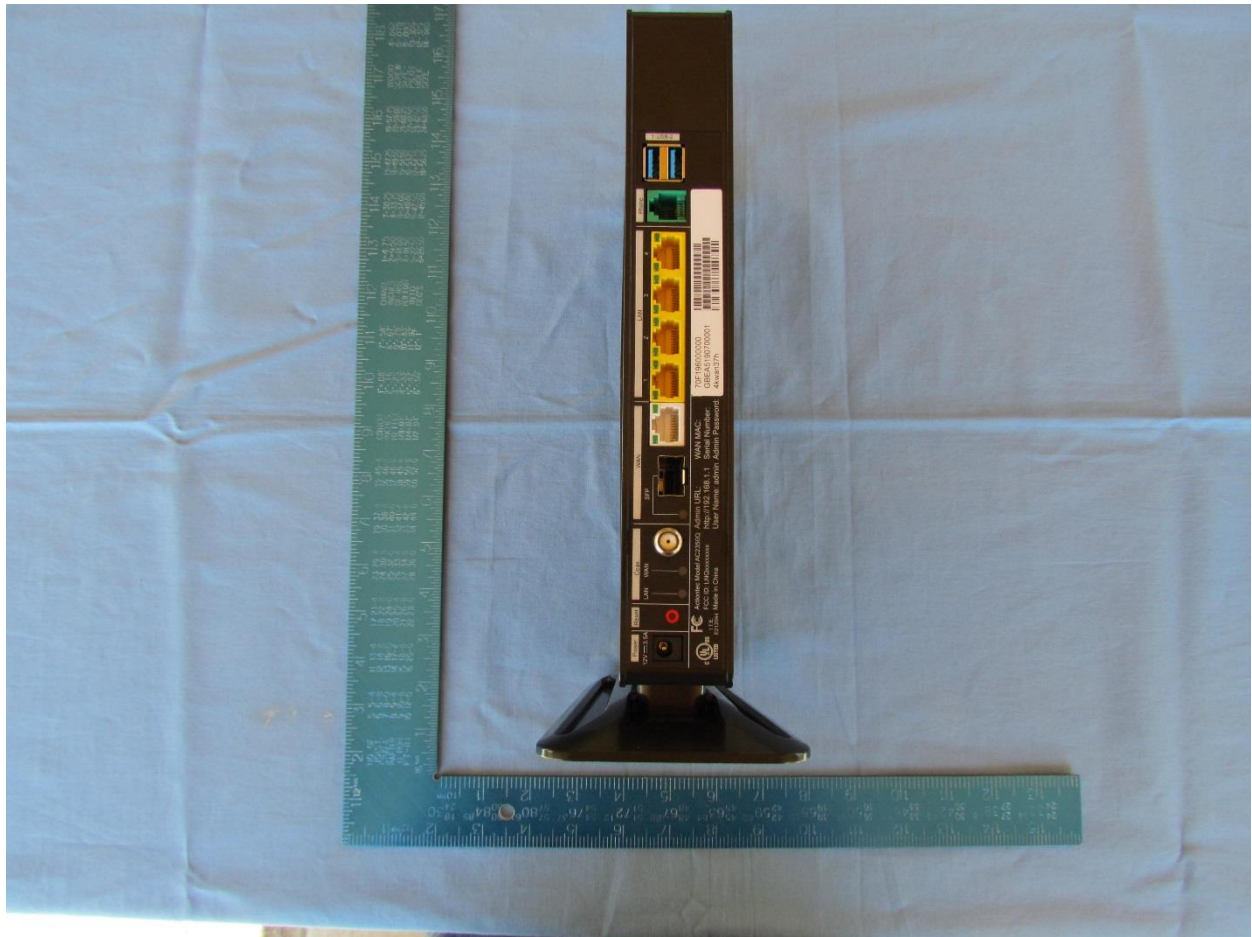
EUT - Port View
