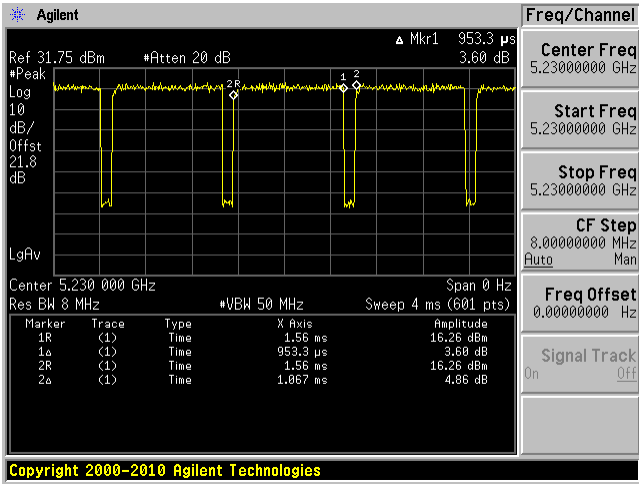
802.11HT/VHT40 mode
