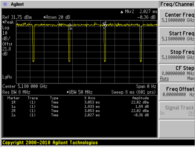
802.11HT/VHT20 mode
