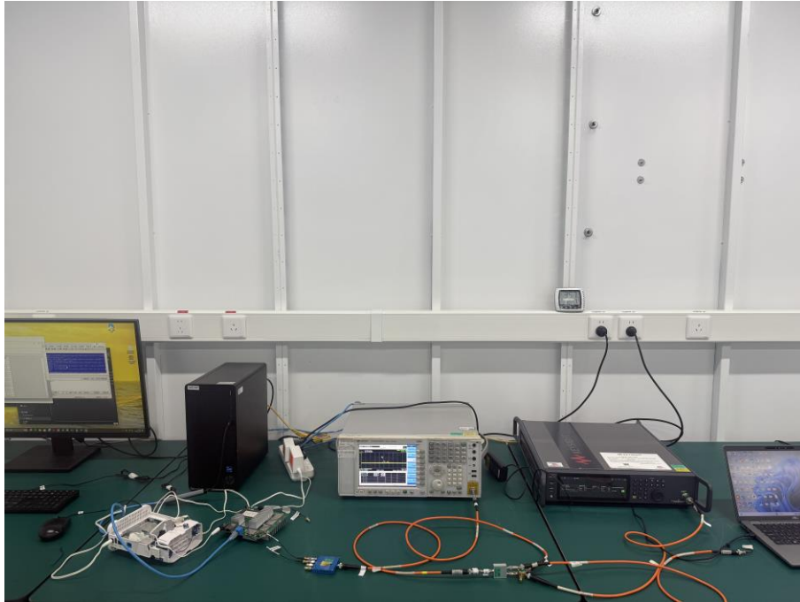
Description: DFS Test Setup - Mesh Mode
