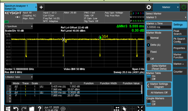
802.11be-EHT20 (T = 5.425ms)
