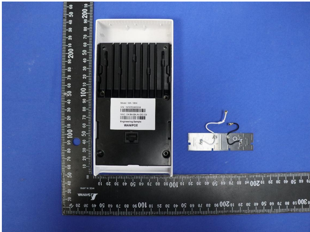
(2) EUT Photo (WF-189W)
