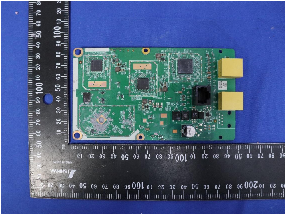
(24) EUT Photo (WF-189H)
