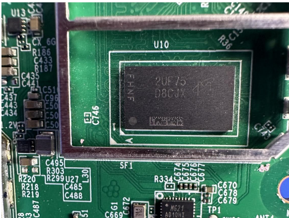
(10) EUT Photo (WF-189W)
