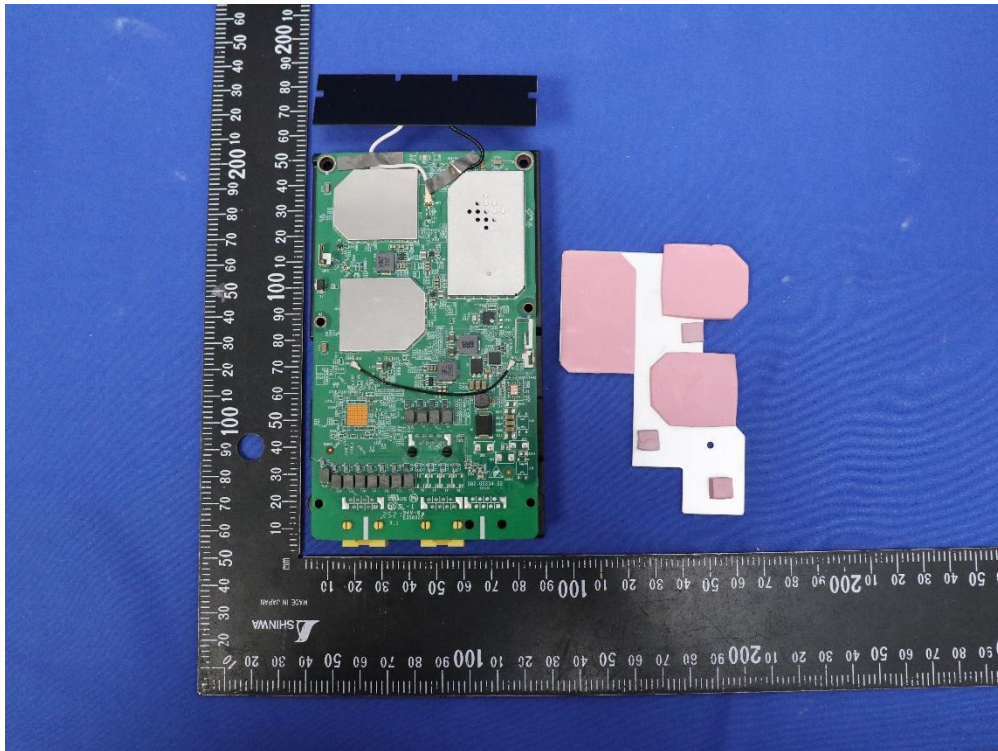
(18) EUT Photo (WF-189H)
