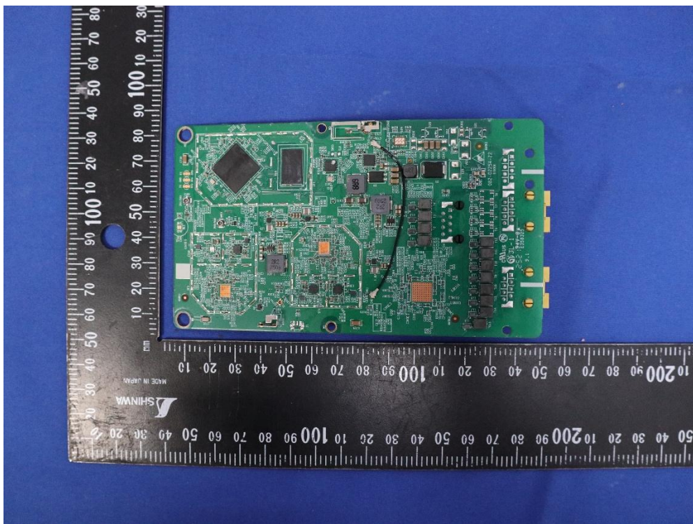
(22) EUT Photo (WF-189H)
