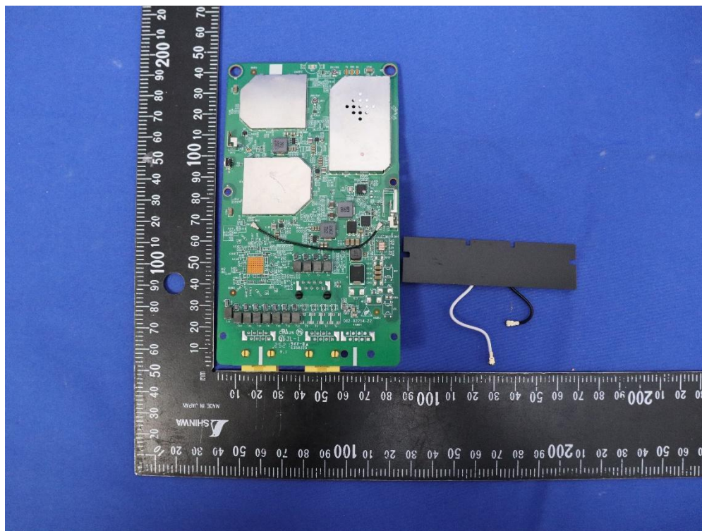
(20) EUT Photo (WF-189H)
