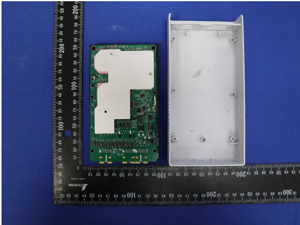
(4) EUT Photo (WF-189W)
