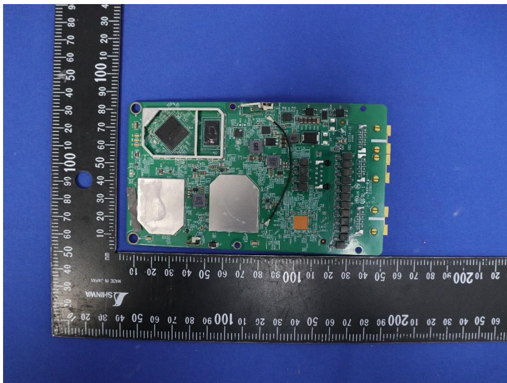
(8) EUT Photo (WF-189W)
