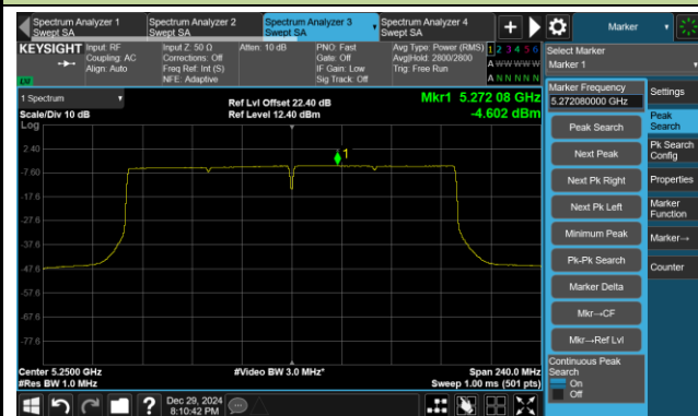
Channel 50 (5250MHz)
