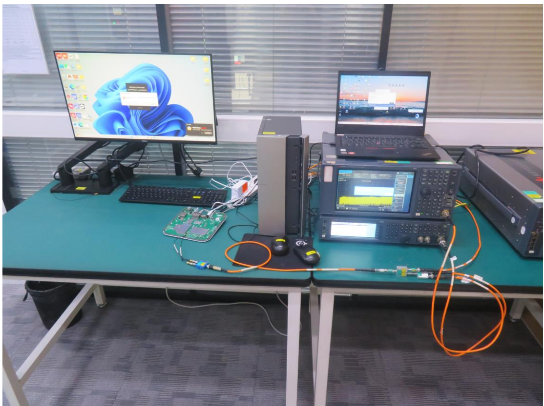
Description: DFS Test Setup
