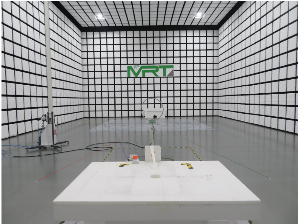
Description: Radiated Emissions Test Setup for 9kHz ~ 30MHz
