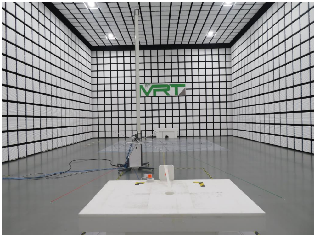
Description: Radiated Emissions Test Setup for 30MHz ~ 1000MHz
