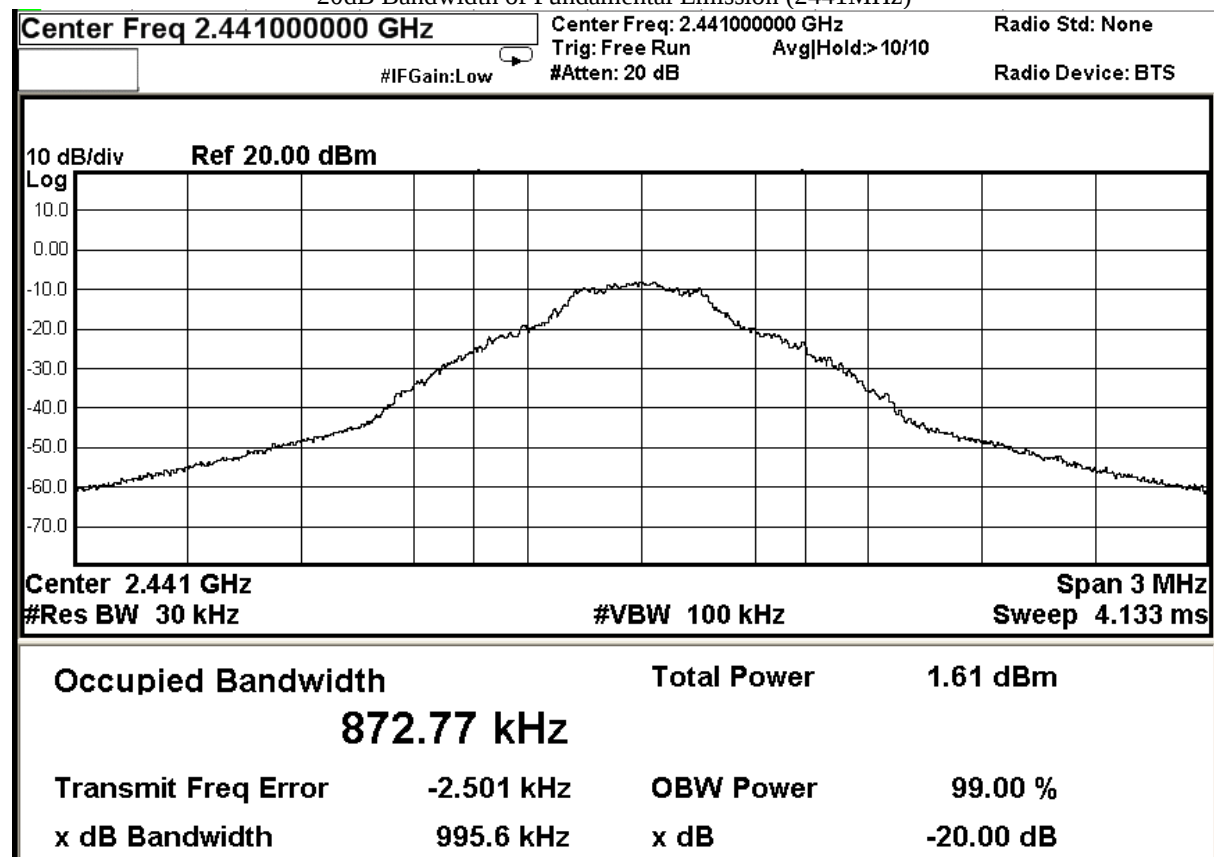
20dB Bandwidth of Fundamental Emission (2441MHz)
