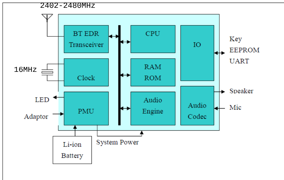
IS1681S Bluetooth RF IC
