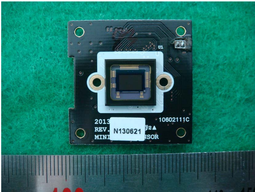
Camera module board
