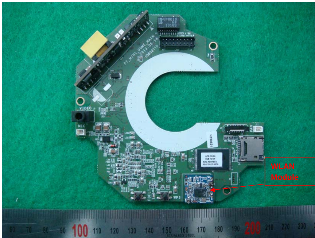
Main board
