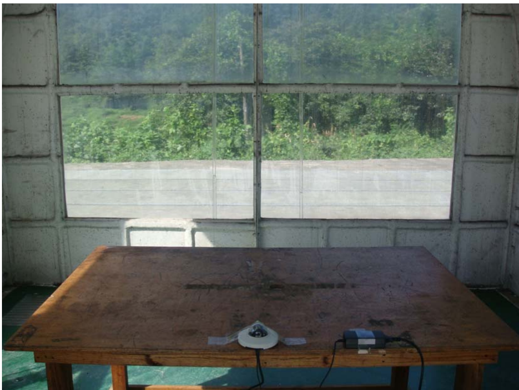
Radiated emissions - rear view (AC adapter)
