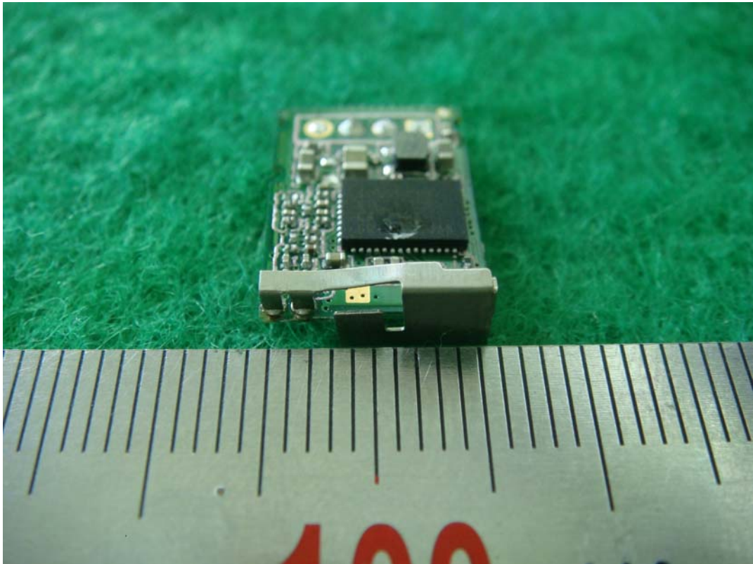
WLAN Antenna
