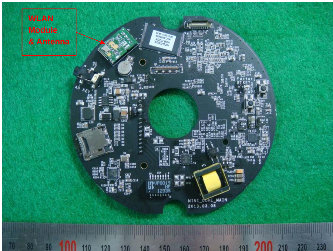
Main board
