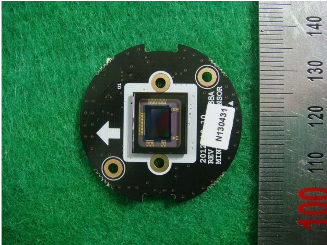
Sensor board
