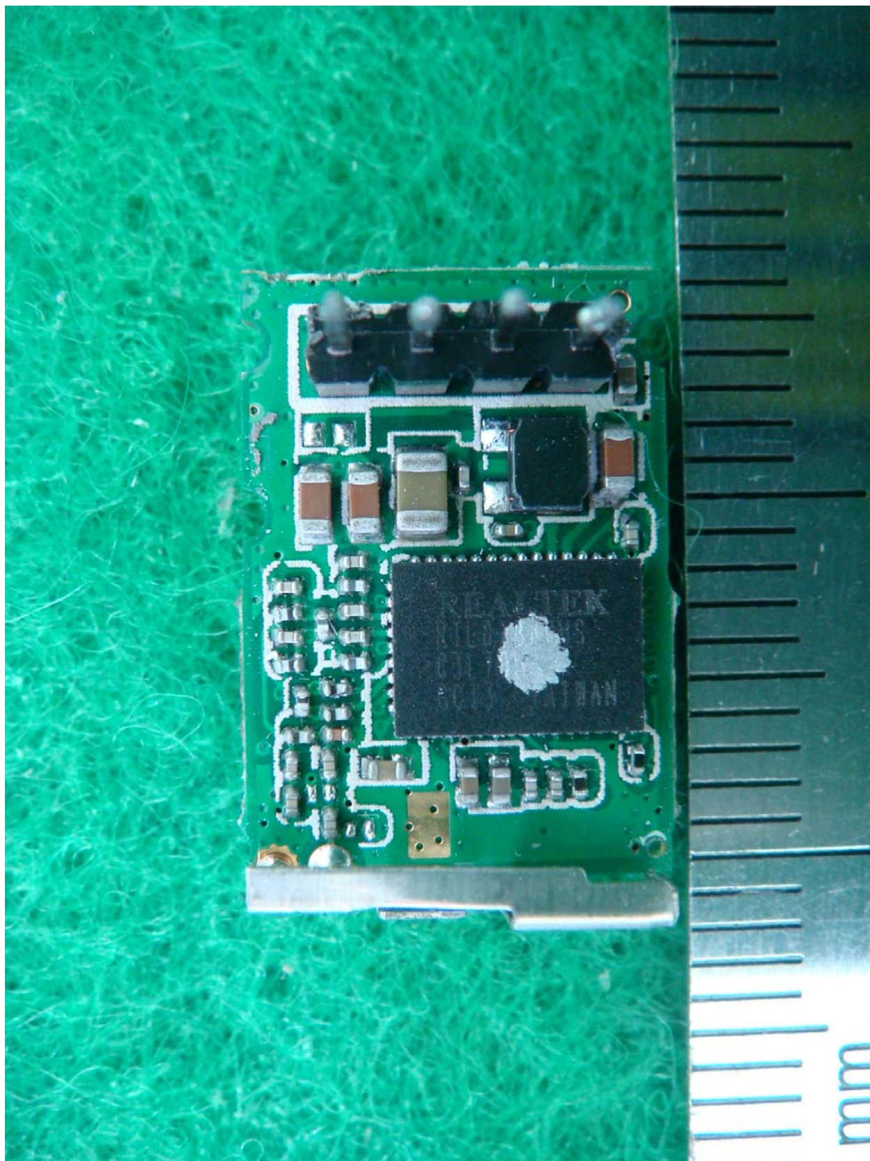
<Photograph 5: WLAN module - Rear view>
