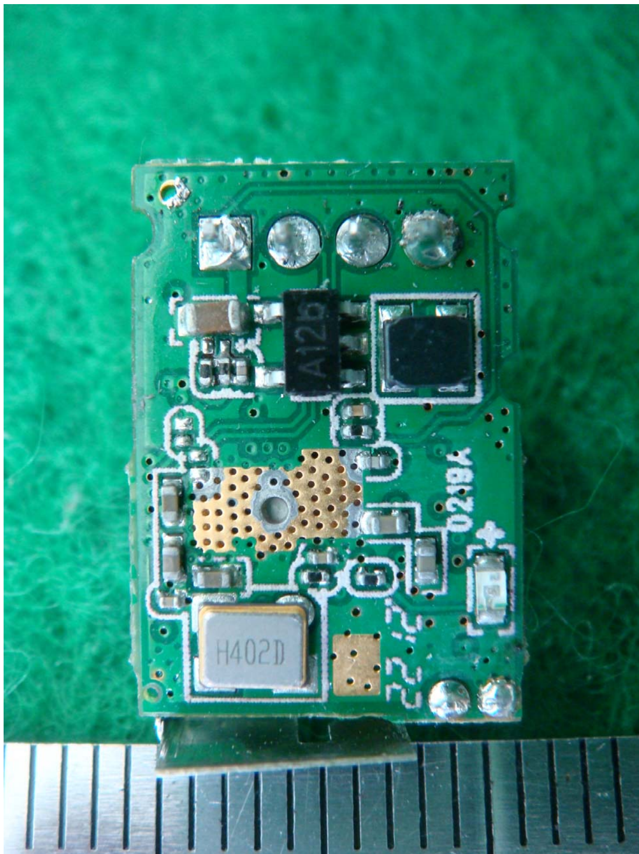
<Photograph 5: WLAN module - Front view>
