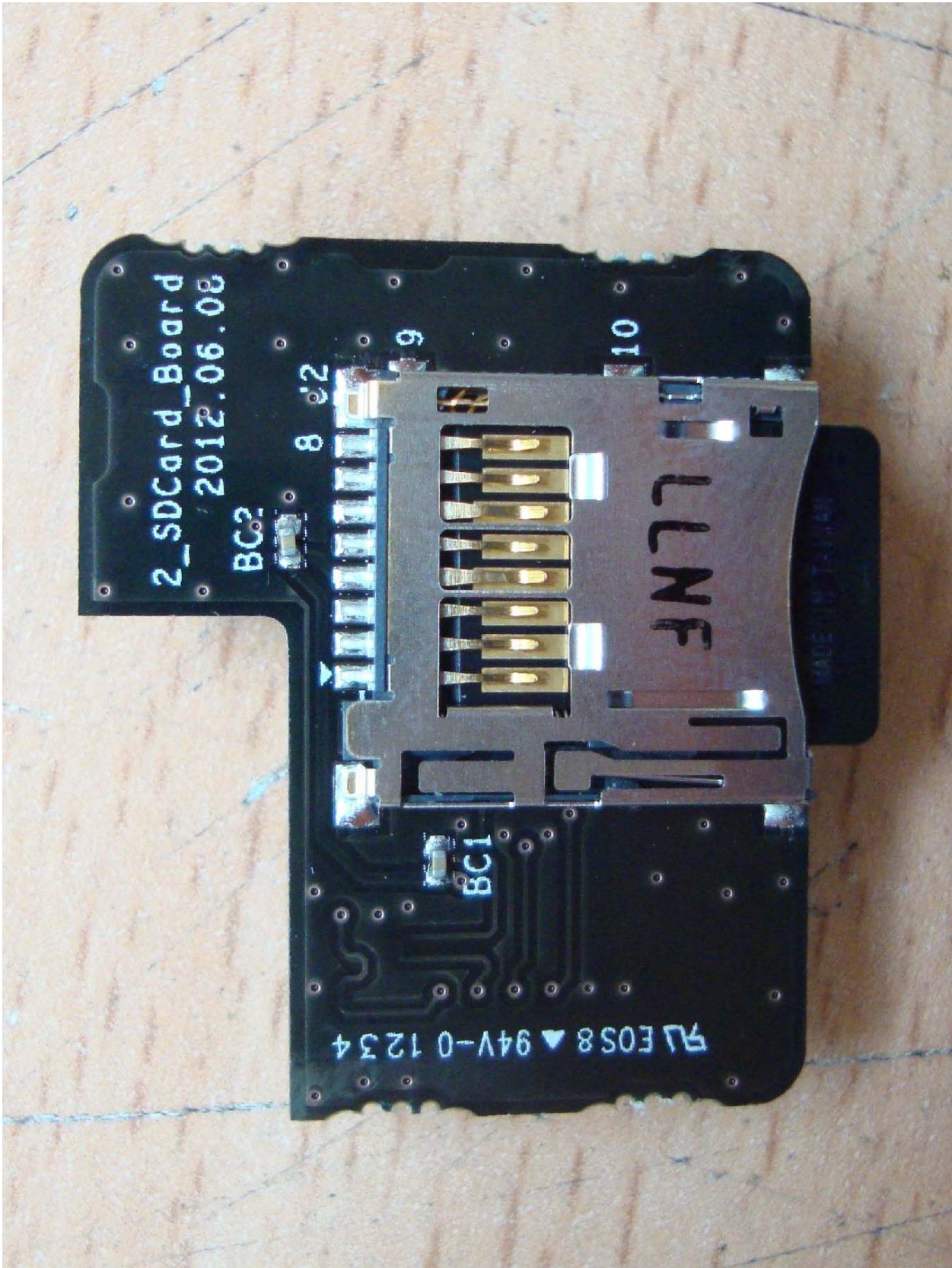
<Photograph 7: Micro SD Card board - Front view>
