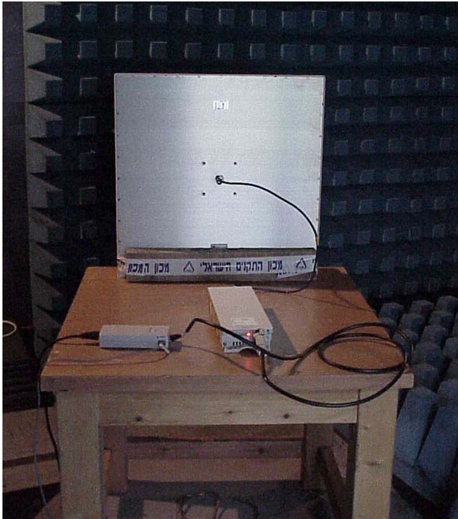
Photo# 7. Radiated spurious emission test . Antenna P/N AN1230
