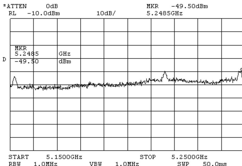
Plot # 52. Subscriber unit out of band emission low band zoom into 5150-5250 band limit.
