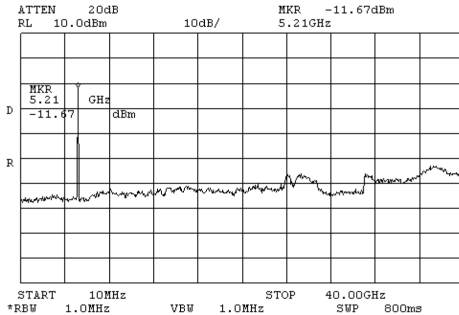
Plot # 30. Base station out of band emissions low band
