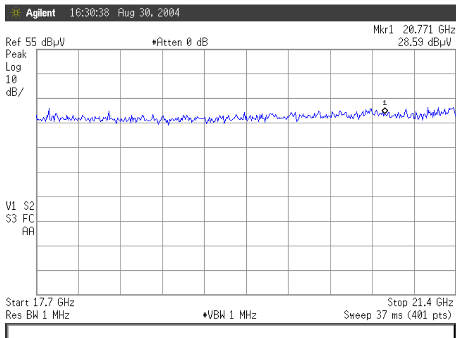
Plot # 18. Antenna: P/N AN1230, high frequency
