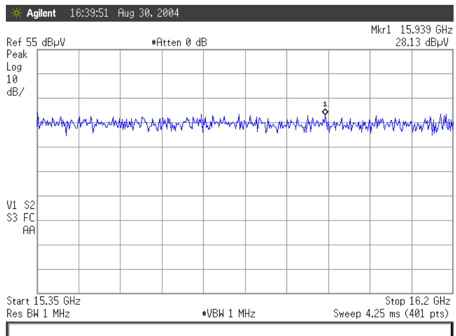
Plot # 10. Antenna : P/N AN1152, high frequency
