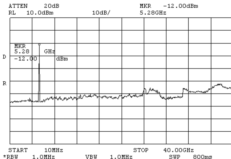
Plot # 32. Base station out of band emission high band
