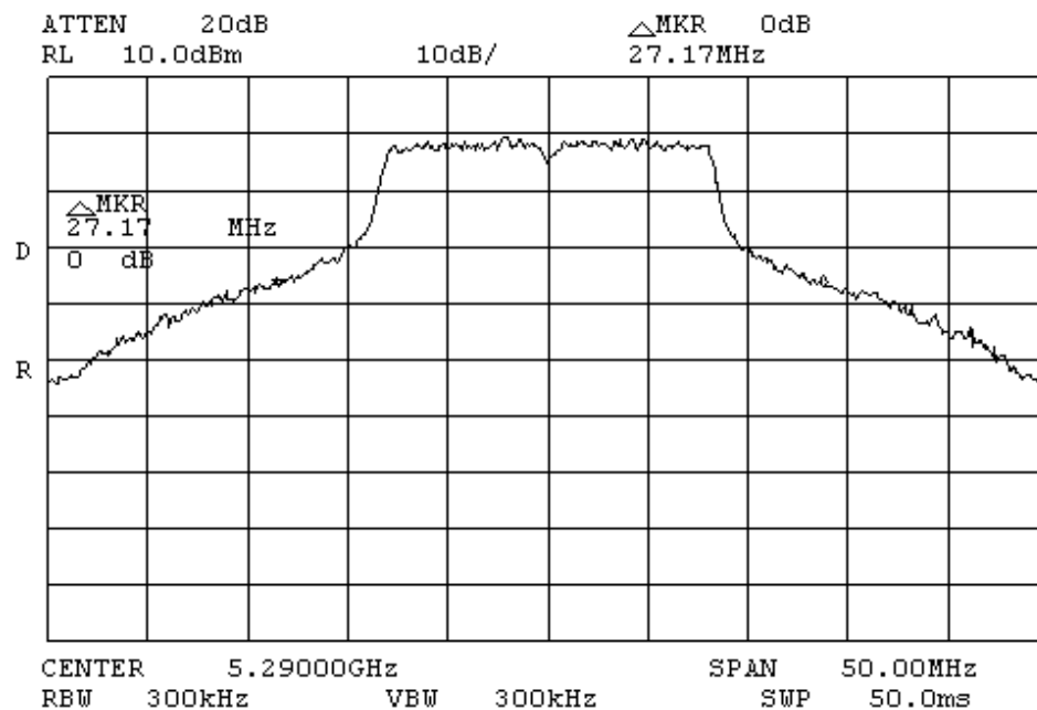
Plot # 55. Subscriber unit 26dB bandwidth middle band
