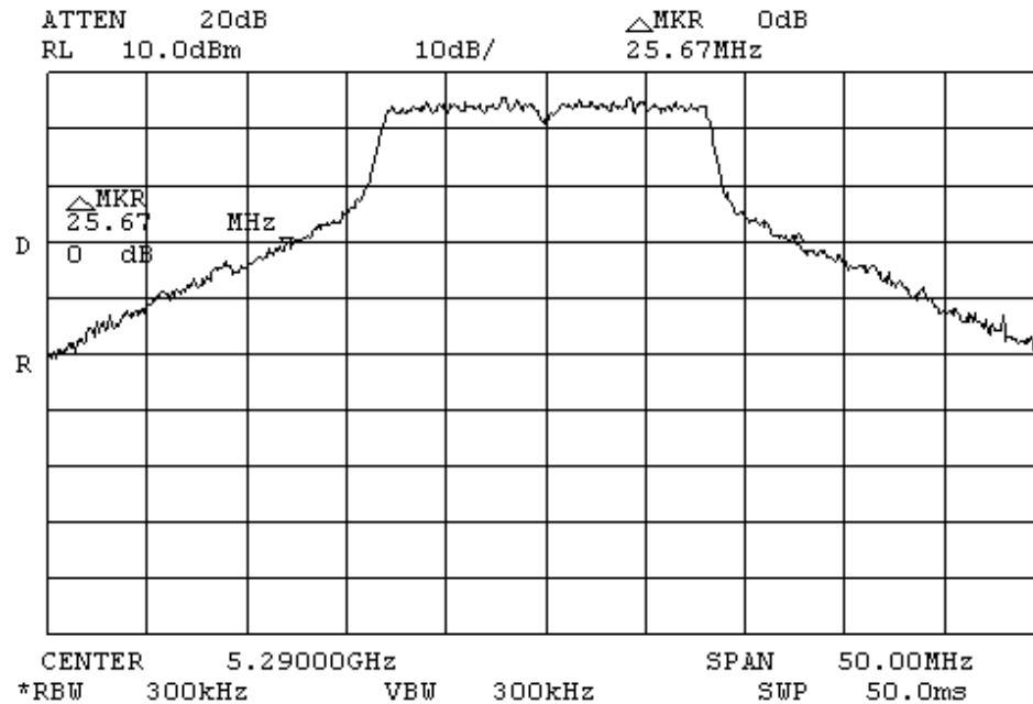
Plot # 37. Base station 26dB bandwidth middle channel
