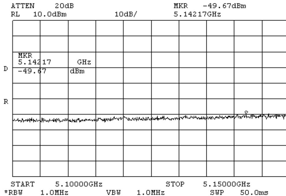
Plot # 35. Base station low band out of band emission zoom to 5100-5150MHz band
