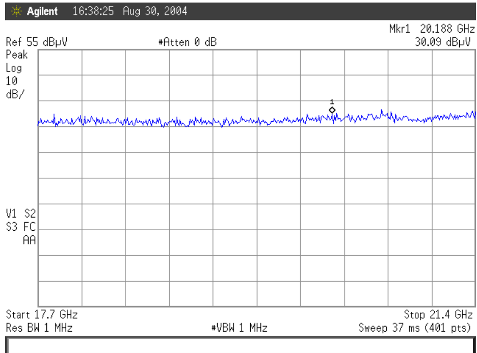
Plot # 9. Antenna : P/N AN1152, high frequency
