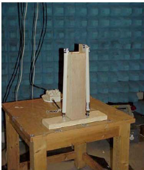
Photo #2. Test setup in anechoic chamber. Antenna Omni.
