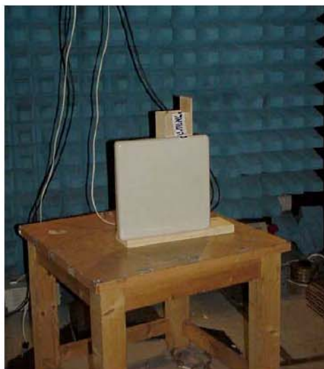
Photo #3. Test setup in anechoic chamber. Antenna Flat panel.
