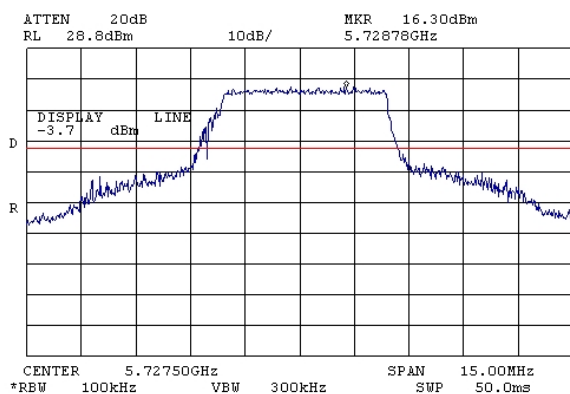
Plot # 19. Carrier frequency 5727.5 MHz
