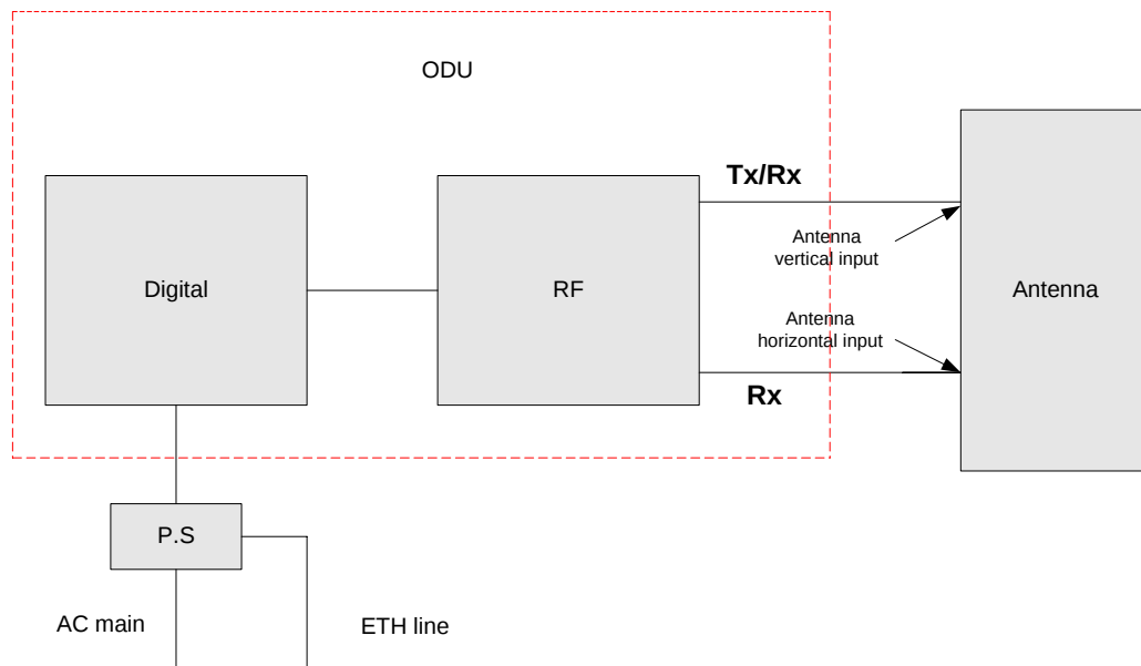
Fig. 1. EUT block diagram.
