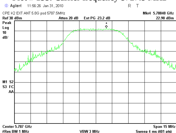
Plot # 135. Carrier frequency 5787.5 MHz
