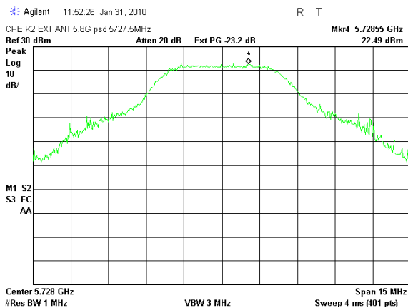
Plot # 133. Carrier frequency 5727.5 MHz
