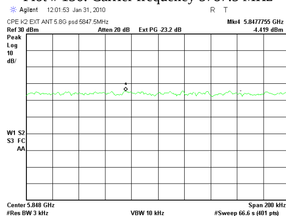
Plot # 138. Carrier frequency 5847.5 MHz
