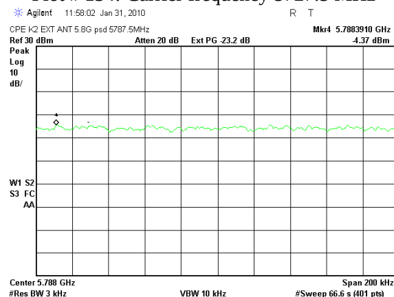
Plot # 136. Carrier frequency 5787.5 MHz
