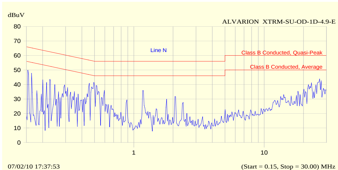
Plot # 146. Conducted emissions test. Line Neutral .
