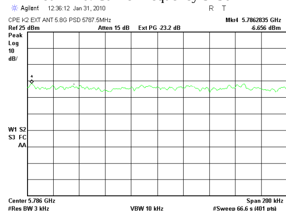
Plot # 142. Carrier frequency 5787.5 MHz
