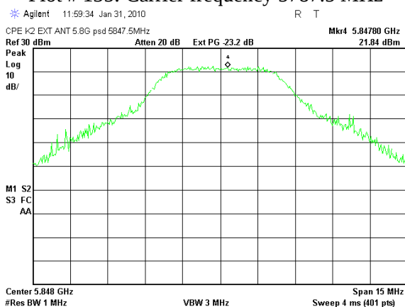
Plot # 137. Carrier frequency 5847.5 MHz
