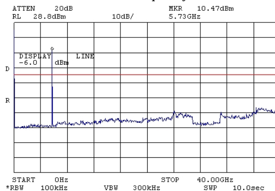
Plot # 26. Carrier frequency 5730 MHz
