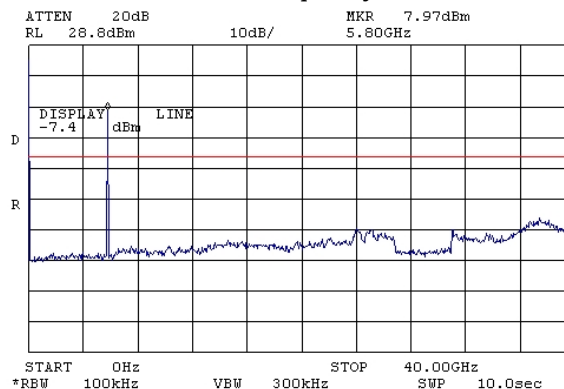
Plot # 28. Carrier frequency 5787.5 MHz
