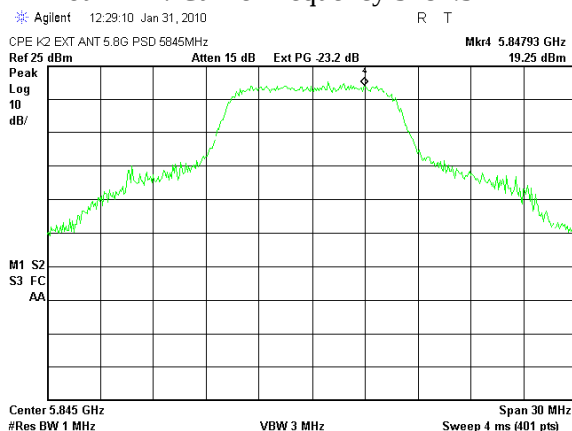
Plot # 143. Carrier frequency 5845 MHz
