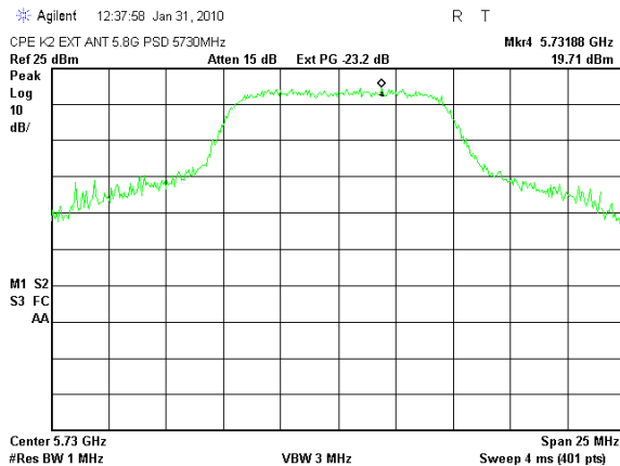
Plot # 139. Carrier frequency 5730 MHz
