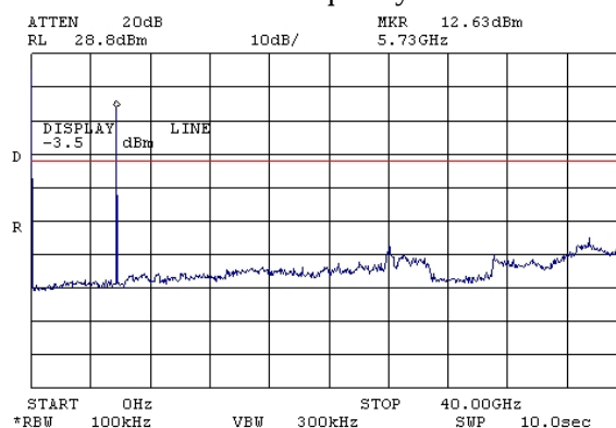
Plot # 20. Carrier frequency 5727.5 MHz
