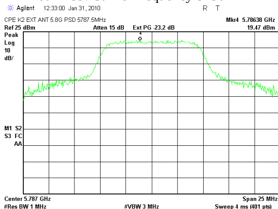
Plot # 141. Carrier frequency 5787.5 MHz
