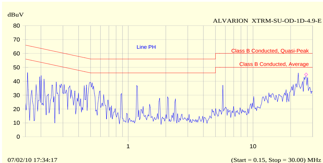
Plot # 145. Conducted emissions test. Line Phase .
