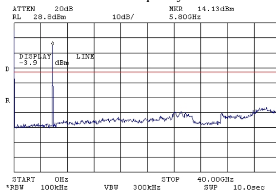
Plot # 22. Carrier frequency 5787.5 MHz
