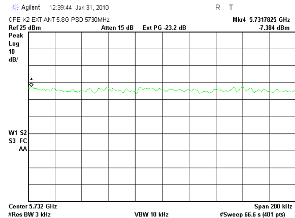
Plot # 140. Carrier frequency 5730 MHz
