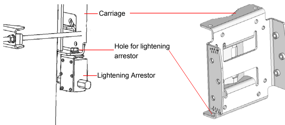
Figure 2-3: Installing the Lightning Arrestor on the Carriage
