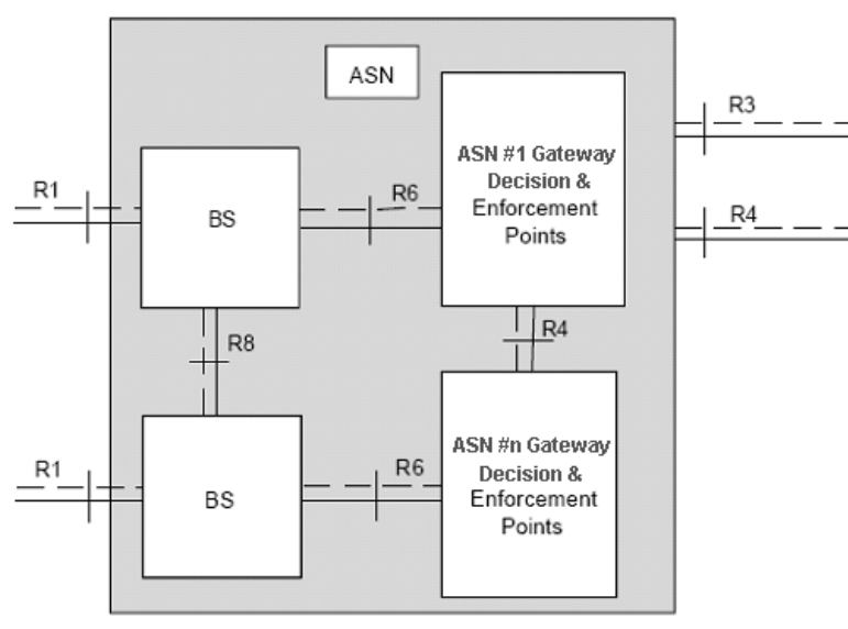
Figure 1-2: ASN Reference Model containing Multiple ASN-GWs
