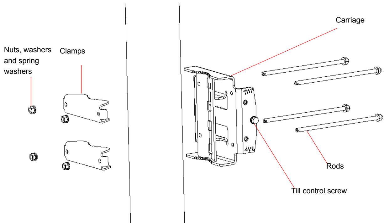
Figure 2-5: Assembling BTS Carriage and Clamps
