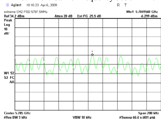
Plot # 166. Carrier frequency 5787.5 MHz.
