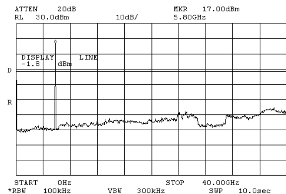
Plot # 36. Carrier frequency 5847.5 MHz
