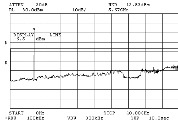
Plot # 38. Carrier frequency 5730 MHz.
