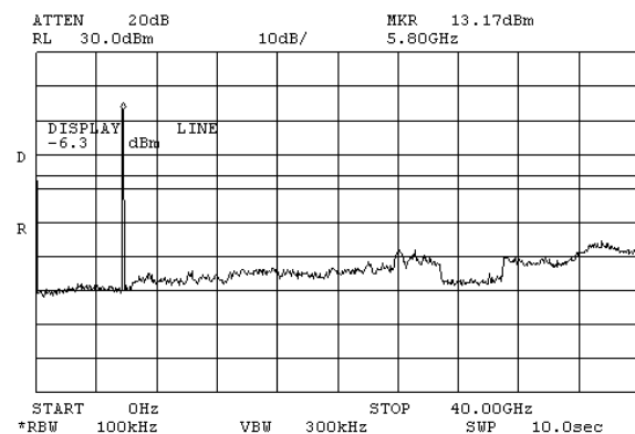
Plot # 40. Carrier frequency 5787.5 MHz
