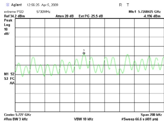
Plot # 152. Carrier frequency 5730 MHz.
