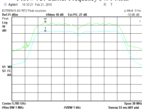
Plot # 95. Carrier Frequency 5705 MHz
