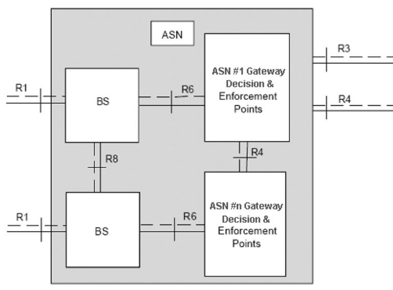
Figure 1-2: ASN Reference Model containing Multiple ASN-GWs
