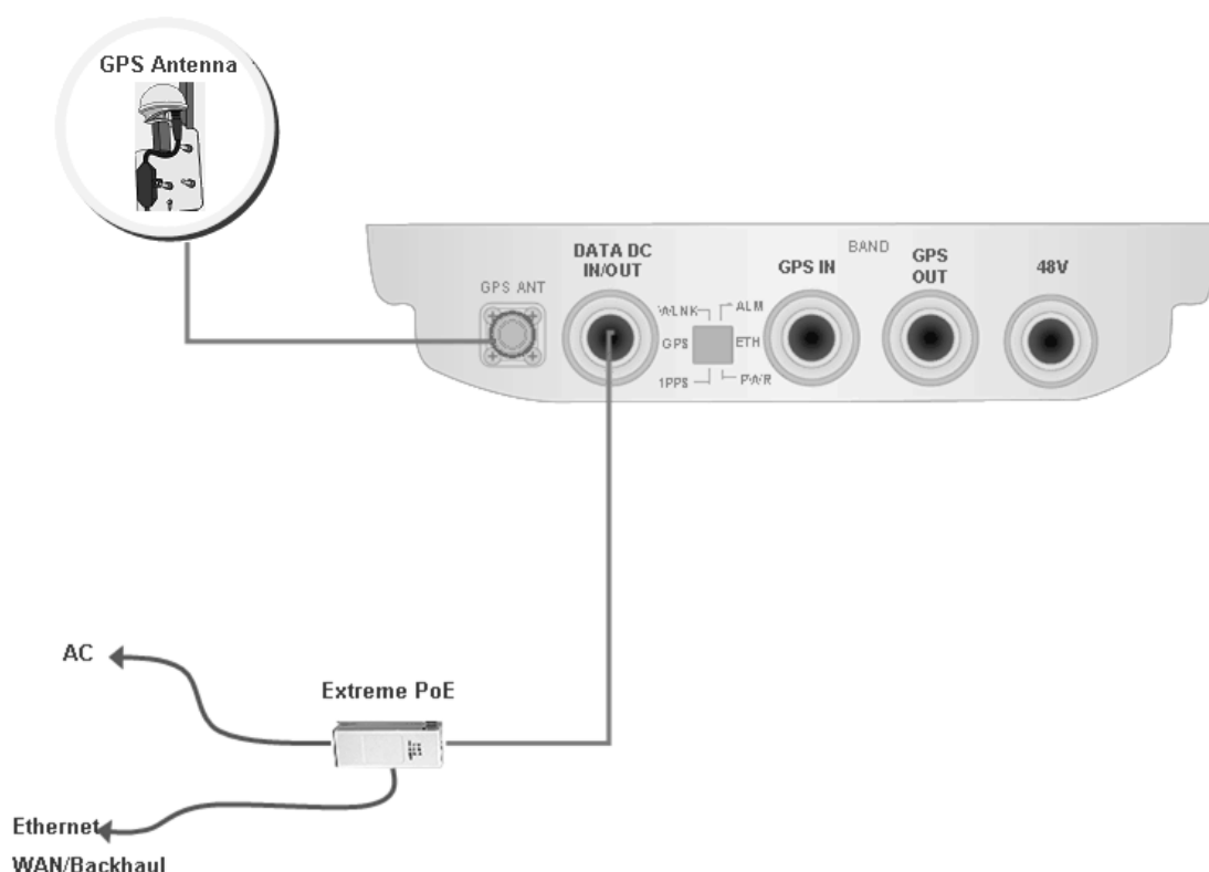
Figure 2-1: PoE Power Feeding Option
