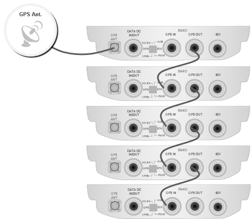
Figure 2-17: GPS Chaining
