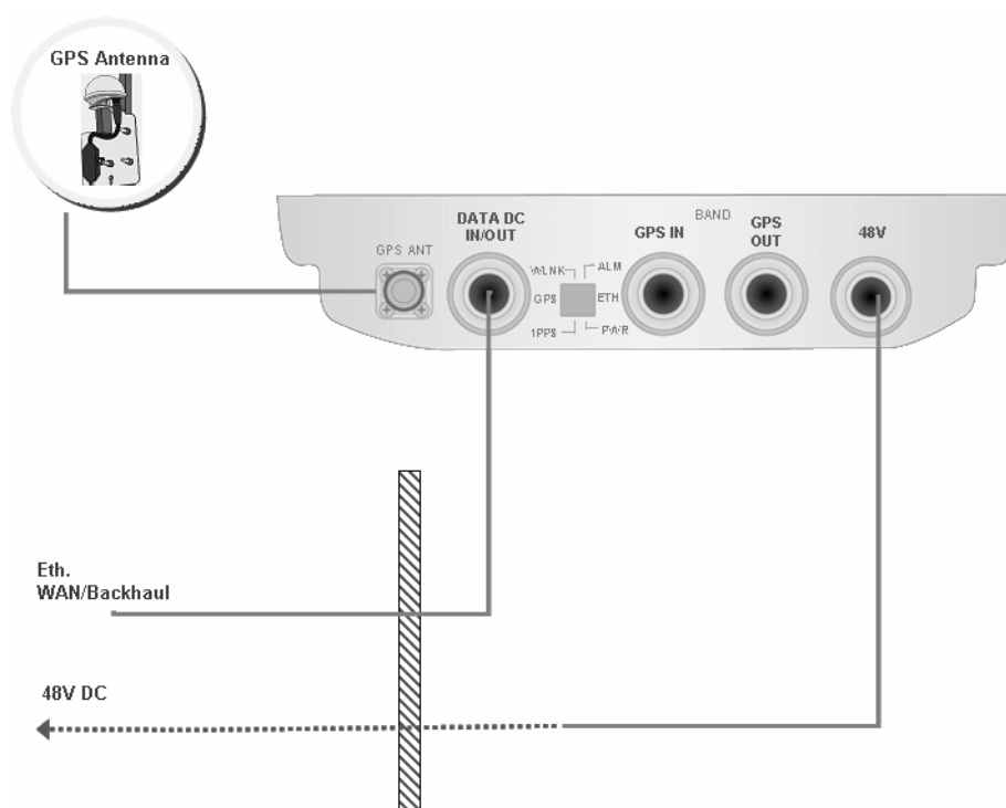
Figure 2-2: 48VDC Power Feeding Option
