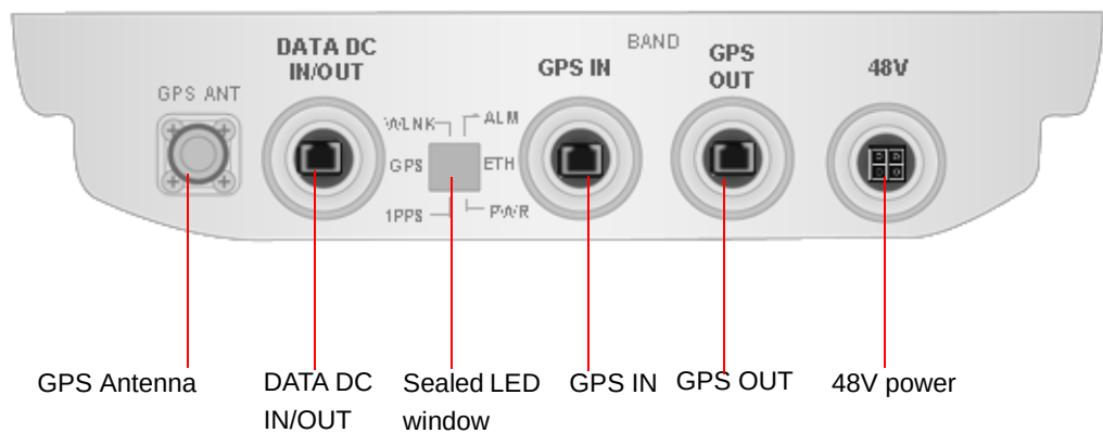
Figure 2-20: BTS Connectors (Bottom View)
