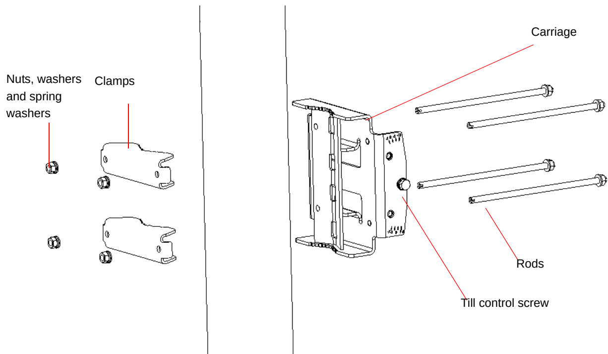
Figure 2-9: Assembling BTS Carriage and Clamps
