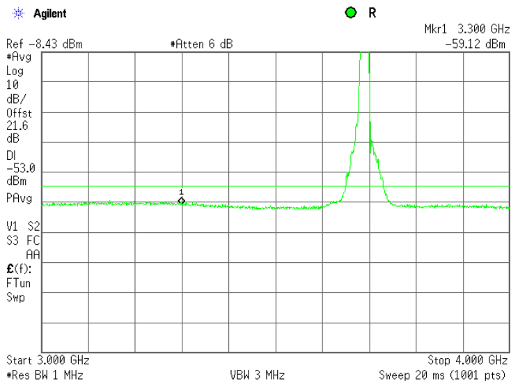
Plot 9.1.3 Conducted spurious emission measurements 3000 - 4000 MHz
