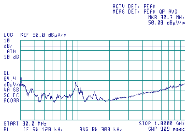
Plot 7.6.8 Radiated emission measurements in 30 - 1000 MHz range
