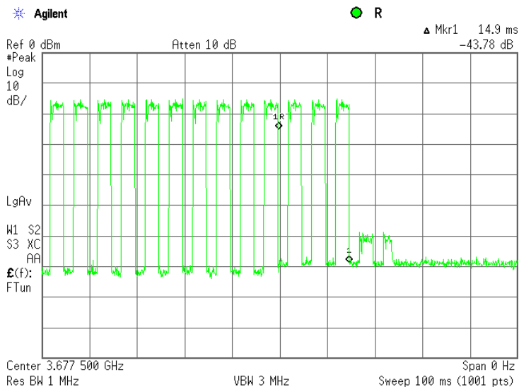
Plot 8.2.2 Tx off example, shut-off time
