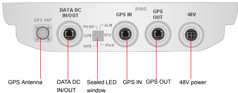
Figure 2-21: BTS Connectors (Bottom View)
