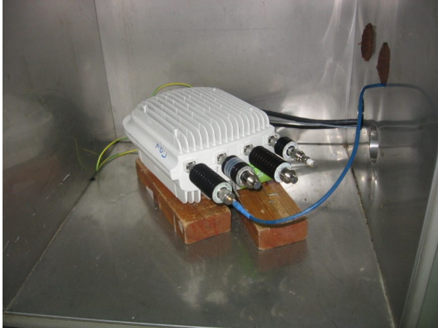
Photograph No.9 Frequency stability measurement setup
