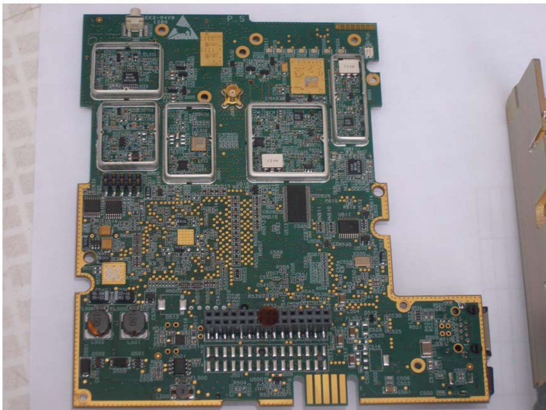
Photo3. CPE Si internal view , CS
