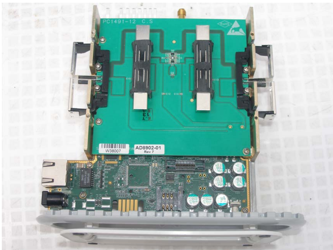
Photo7. CPE Si internal view, antennas
