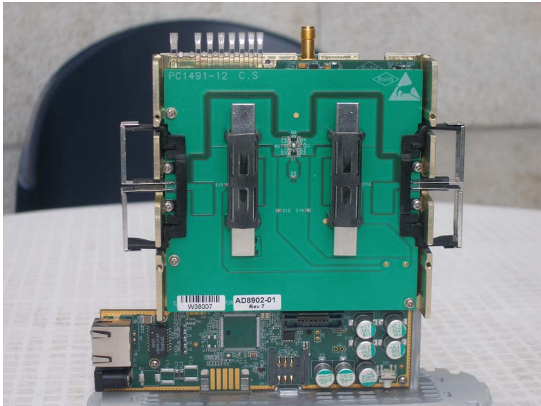
Photo 6. CPE Si internal view antennas
