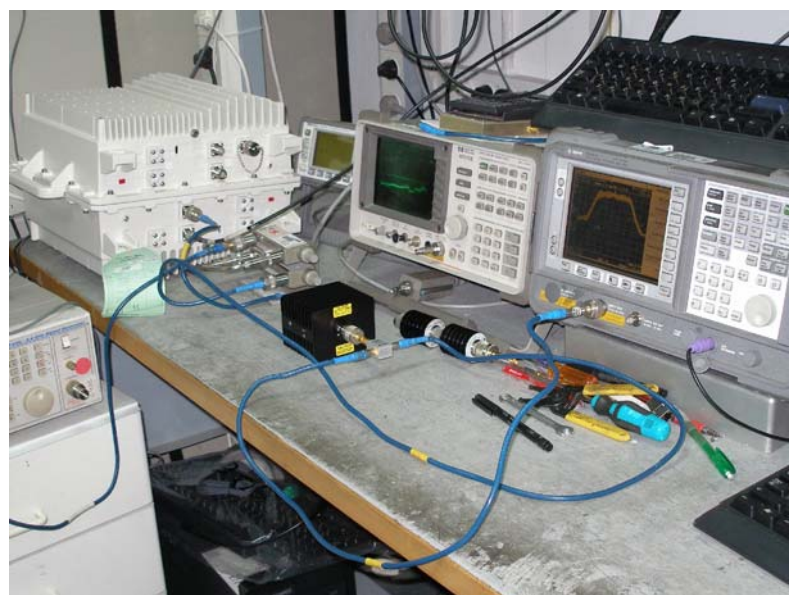
Photo 2. Test setup for conducted measurements.
