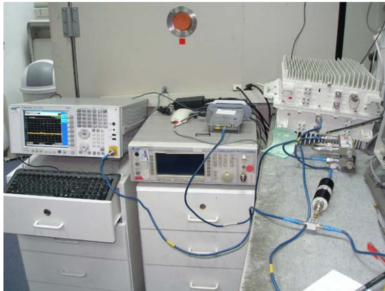
Photo 1. Test setup for conducted measurements.
