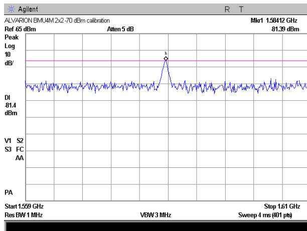
Plot # 12. Wide band limit calibration -70 dBm/MHz.
