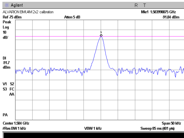
Plot # 14. Narrow band limit calibration -80 dBm/kHz
