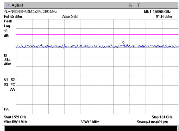
Plot # 13. Wide band power density.
