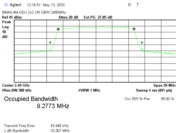
Plot # 1. 99% power emission bandwidth.
