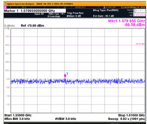
Plot # 11. Narrow band power density
