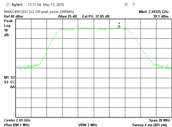
Plot # 2. Peak of emission envelope.
