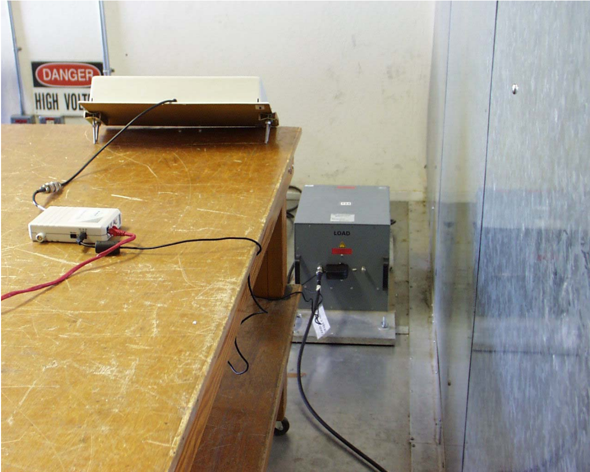
AC line conducted, subscriber unit configuration
