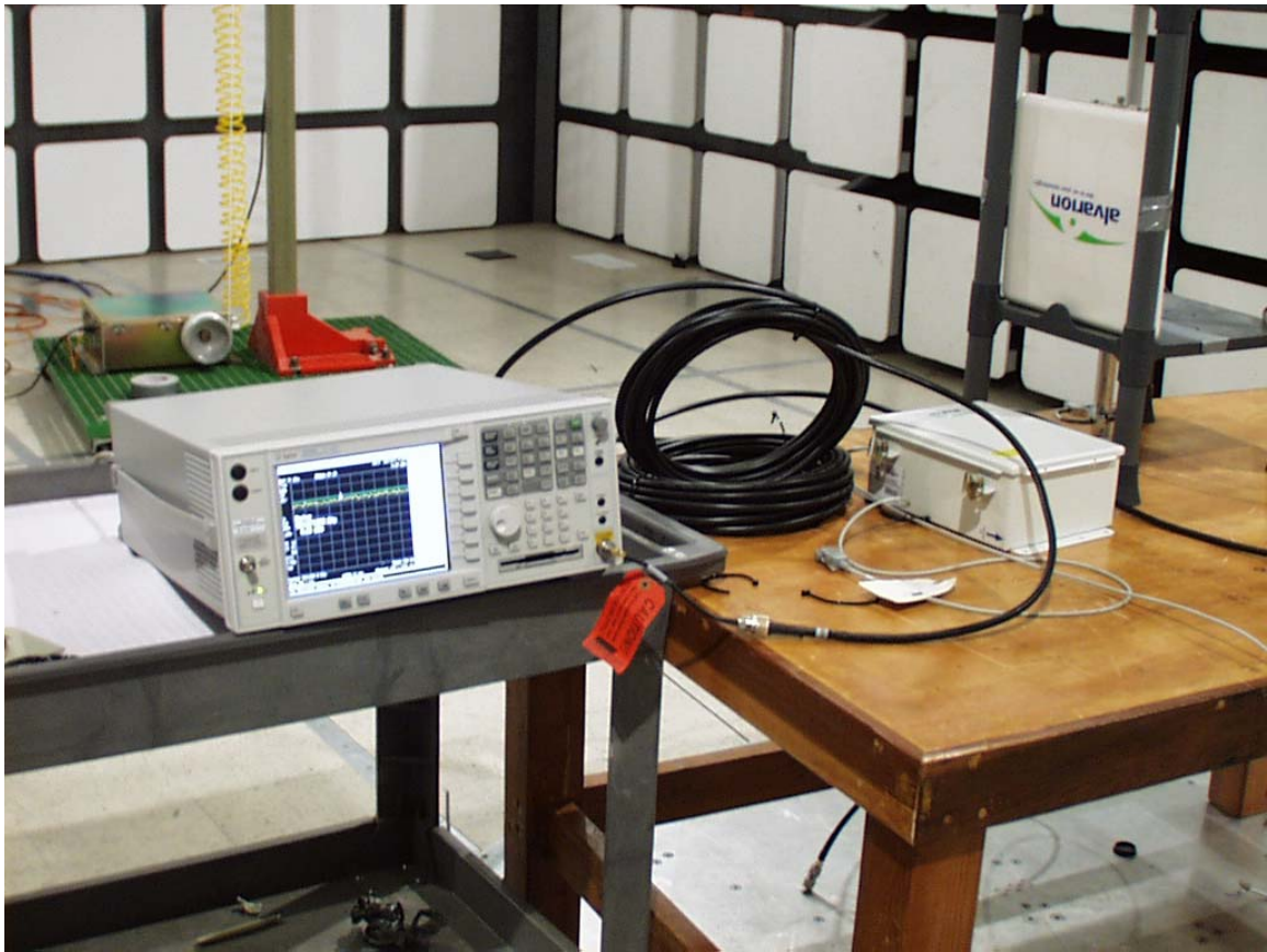
Antenna port output conducted test set-up
