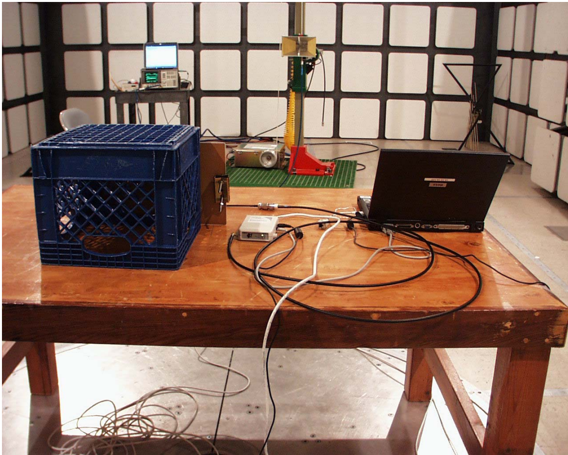
Radiated setup, subscriber unit configuration 14.6 dBi panel antenna
