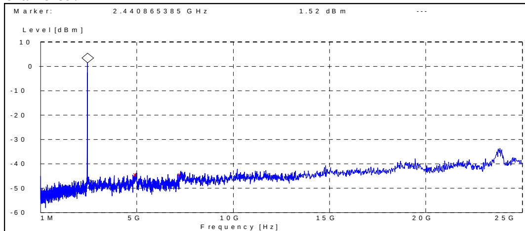
Channel 39 / 2441 MHz
