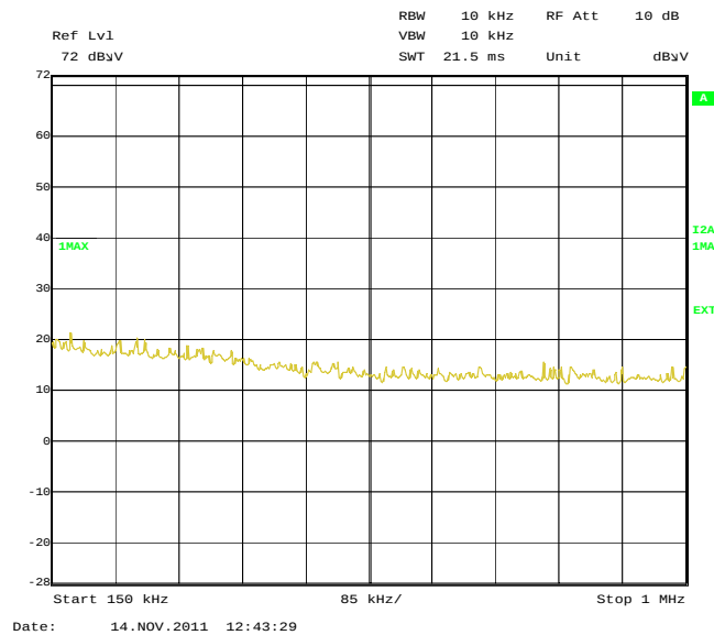
Figure 2 Radiated Emission 150 kHz to 1 MHz
