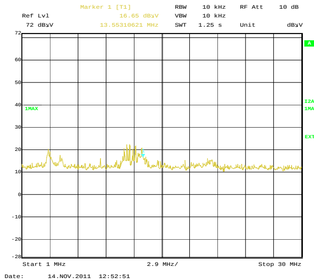
Figure 4 Radiated Emission 1 MHz to 30 MHz, Noise Floor (Background) No EUT's inside the Anechoic Chamber. Peaks are coming from the Magnetic Loop Antennas Pre-Amplifier.
