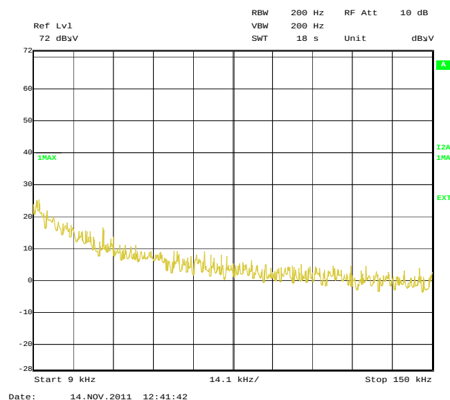
Figure 1 Radiated Emission 9 kHz to 150 kHz
