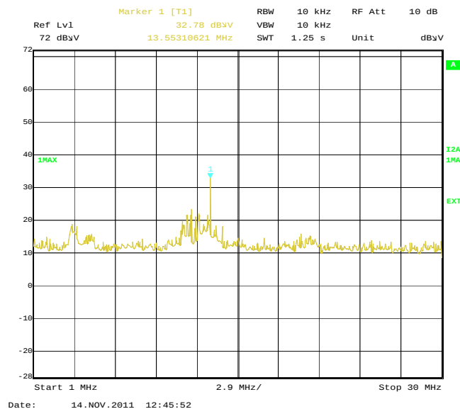
Figure 3 Radiated Emission 1 MHz to 30 MHz
