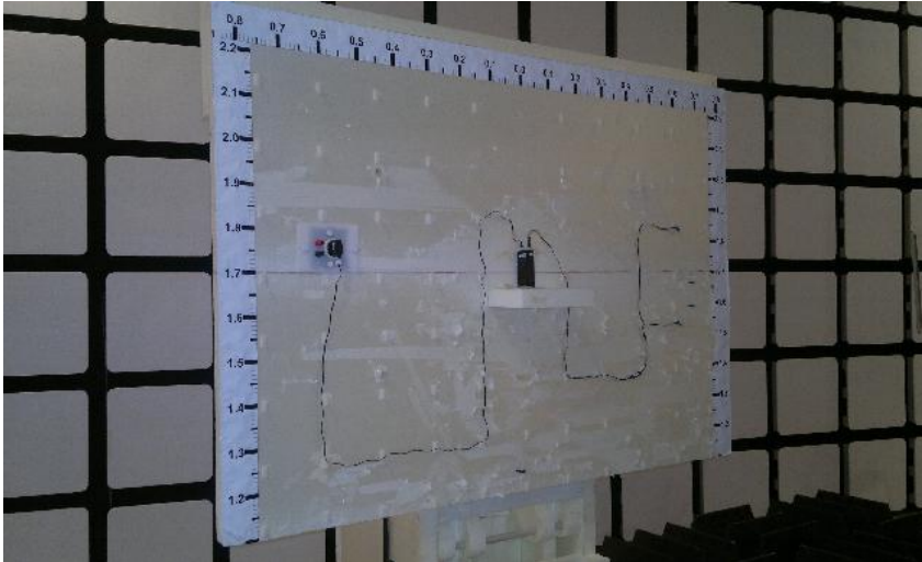
Picture 2. FCC Part 15B Radiated emissions
