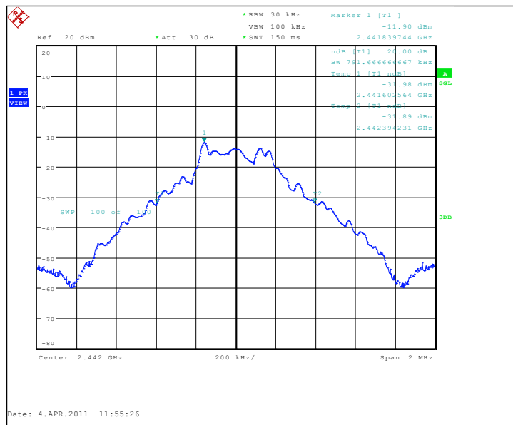
Channel 40 / 2442 MHz
