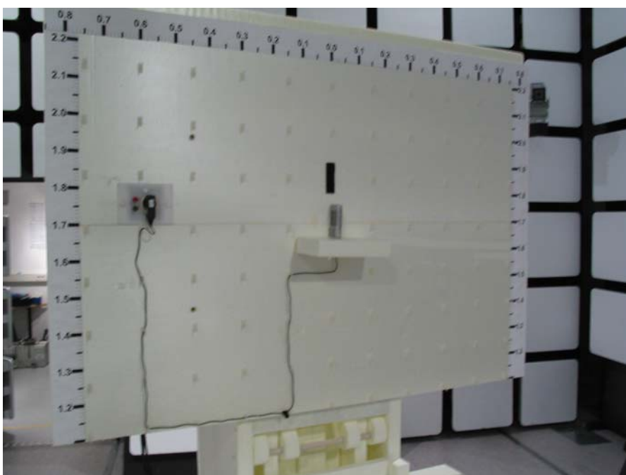
Picture 2 Spurious radiated emissions
