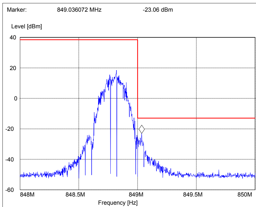
Picture 6 Upper bandedge, EGPRS 850 channel 251
