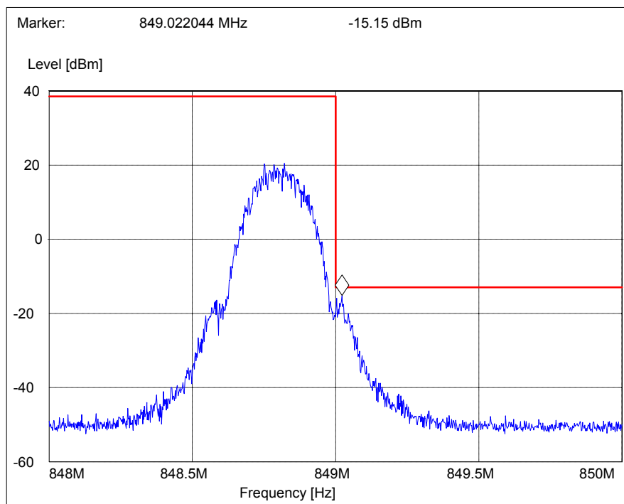
Picture 4 Upper bandedge, GSM 850 channel 251
