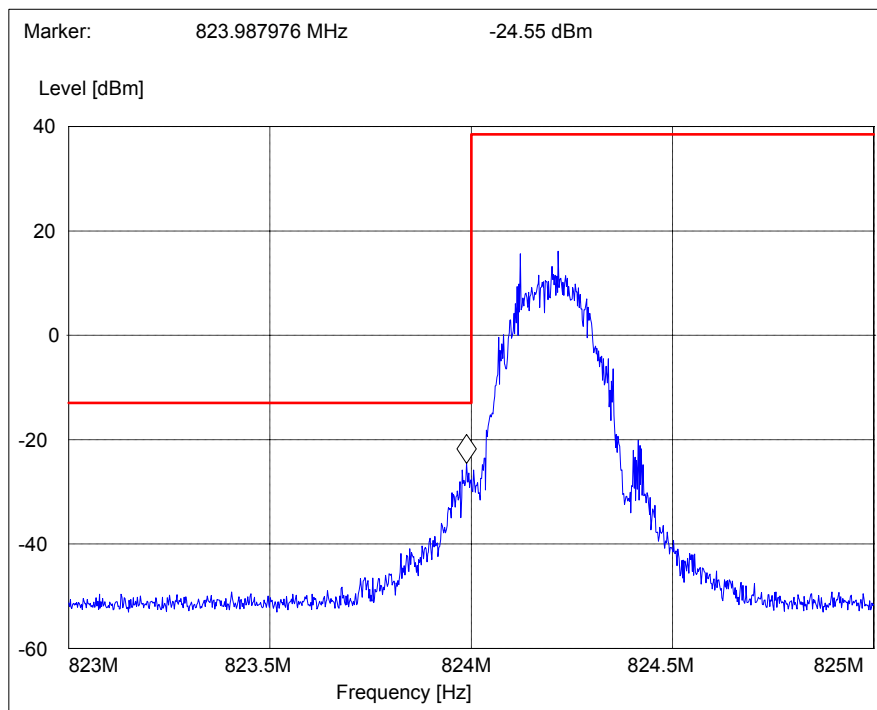
Picture 5 Lower bandedge, EGPRS 850 channel 128
