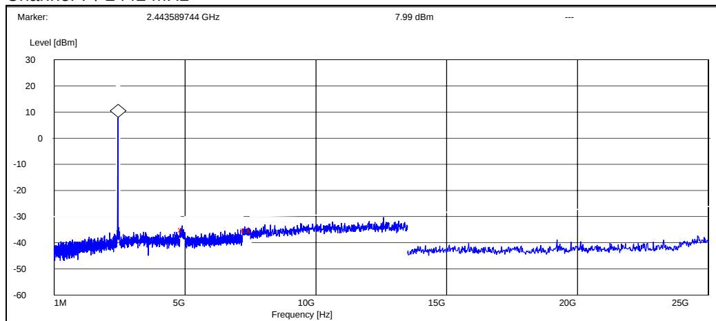
Channel 7 / 2442 MHz
